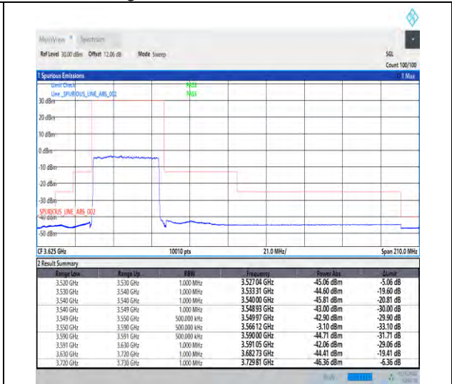
1-N48-30-40-L-3-DFT-PI2BPSK-Outer_Full-100@0-Ant3-1--PASS-see graph
