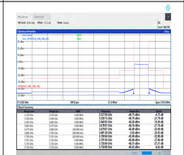
1-N48-30-20-H-6-CP-QPSK-Outer_Full-51@0-Ant3-1--PASS-see graph
