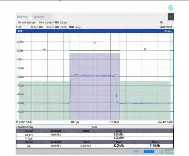
NTVN_N48_PC3_30_40_H_TID1_#1_-40_40
