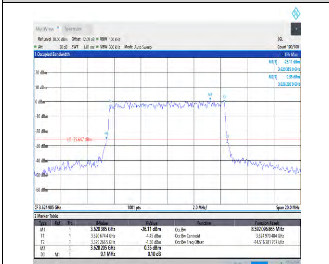
1-N48-30-10-M-7-CP-16QAM-Outer_Full-24@0-Ant3 -8.592-9.100≤10-PASS
