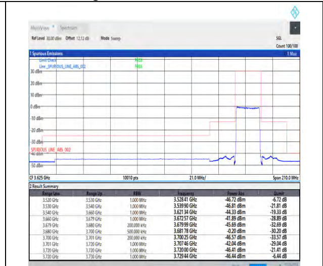
1-N48-30-20-H-3-DFT-PI2BPSK-Outer_Full-50@0-Ant3-1--PASS-see graph
