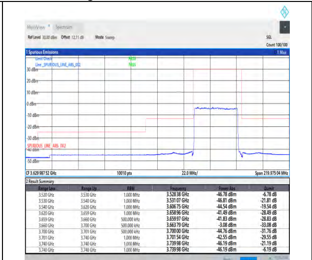
1-N48-30-40-H-3-DFT-PI2BPSK-Outer_Full-100@0-Ant3-1--PASS-see graph
