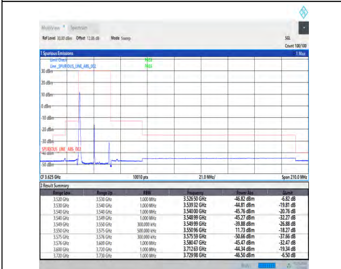
1-N48-30-25-L-4-CP-QPSK-Edge_1RB_Left-1@0-Ant3-1--PASS-see graph
