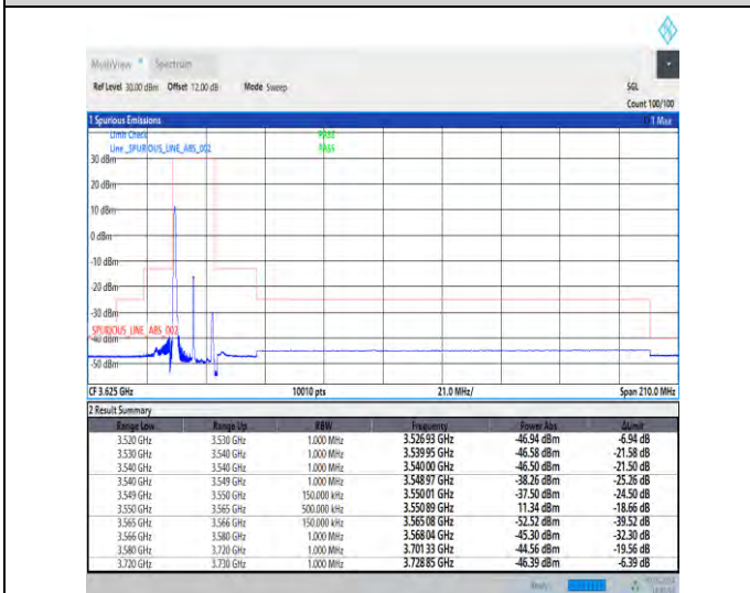
1-N48-30-15-L-4-CP-QPSK-Edge_1RB_Left-1@0-Ant3-1--PASS-see graph
