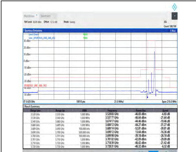
1-N48-30-10-H-2-DFT-PI2BPSK-Edge_1RB_Right-1@23-Ant3-1--PASS-see graph
