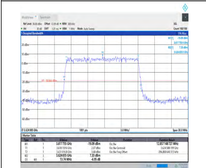
1-N48-30-15-M-2-DFT-PI2BPSK-Outer_Full-36@0-A nt3-12.857-13.740-≤15-PASS
