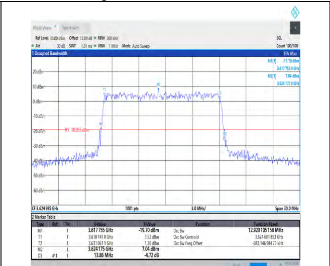
1-N48-30-15-M-1-DFT-QPSK-Outer_Full-36@0-Ant3 -12.92-13.860-≤15-PASS
