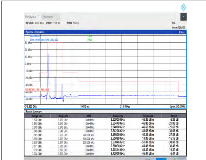
1-N48-30-20-L-1-DFT-PI2BPSK-Edge_1RB_Left-1@0-Ant3-1--PASS-see graph
