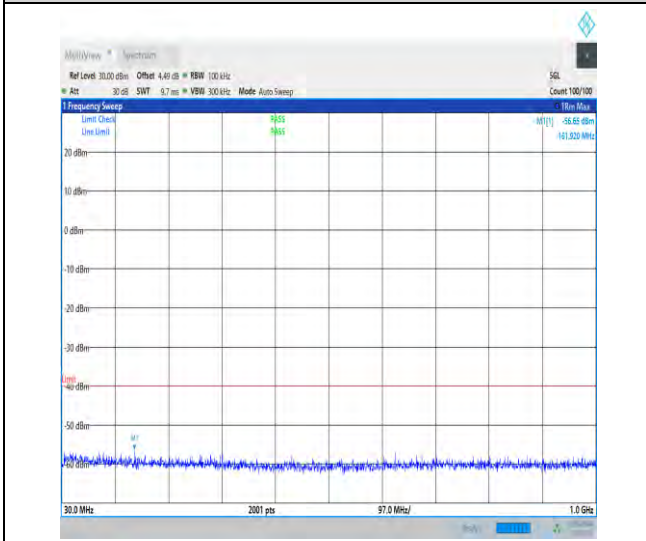
1-N48-30-40-H-1-DFT-PI2BPSK-Inner_1RB_Left-1 @ 1-30-1000-Ant3-90.14--56.65--40-PASS
