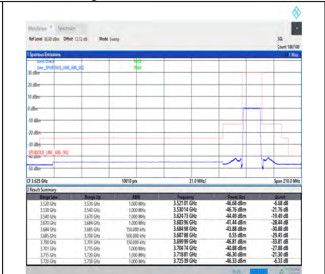
1-N48-30-15-H-3-DFT-PI2BPSK-Outer_Full-36@0-Ant3-1--PASS-see graph
