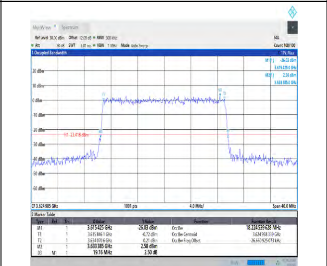
1-N48-30-20-M-6-CP-QPSK-Outer_Full-51@0-Ant3 18.225-19.160-≤20-PASS
