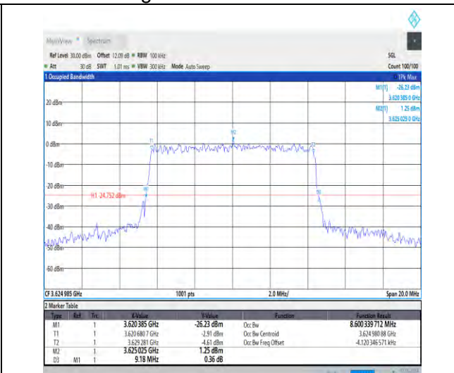
1-N48-30-10-M-6-CP-QPSK-Outer_Full-24@0-Ant3- 8.6-9.180≤10-PASS
