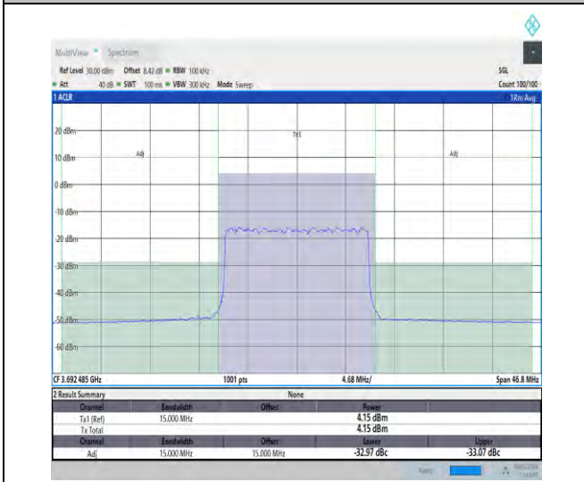
NTVN_N48_PC3_30_15_H_TID16_#1_-15_15
