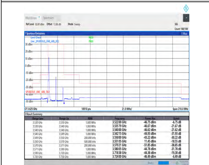
1-N48-30-20-L-4-CP-QPSK-Edge_1RB_Left-1@0-Ant3-1--PASS-see graph
