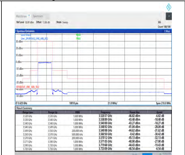
1-N48-30-20-L-3-DFT-PI2BPSK-Outer_Full-50@0-Ant3-1--PASS-see graph
