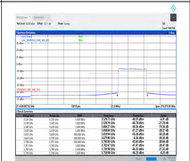
1-N48-30-40-H-6-CP-QPSK-Outer_Full-106@0-Ant3-1--PASS-see graph
