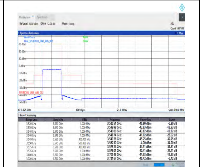
1-N48-30-25-L-6-CP-QPSK-Outer_Full-65@0-Ant3-1--PASS-see graph
