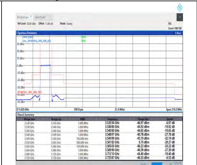
1-N48-30-15-L-3-DFT-PI2BPSK-Outer_Full-36@0-Ant3-1--PASS-see graph
