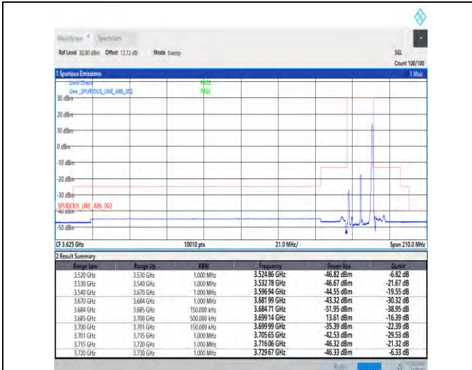
1-N48-30-15-H-2-DFT-PI2BPSK-Edge_1RB_Right-1@37-Ant3-1--PASS-see graph
