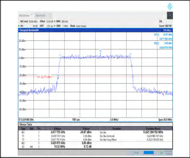
1-N48-30-15-M-7-CP-16QAM-Outer_Full-38@0-Ant 3-13.621-14.520-≤15-PASS
