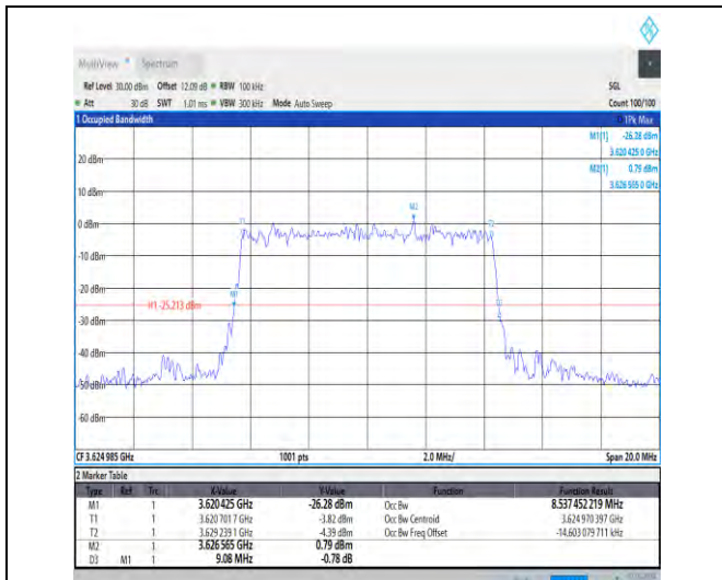
1-N48-30-10-M-5-DFT-256QAM-Outer_Full-24@0-A nt3-8.537-9.080≤10-PASS
