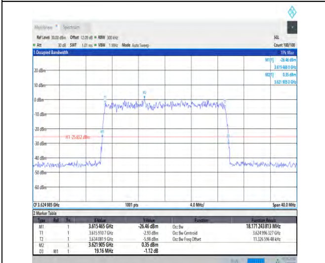
1-N48-30-20-M-9-CP-256QAM-Outer_Full-51@0-Ant 3-18.171-19.160-≤20-PASS
