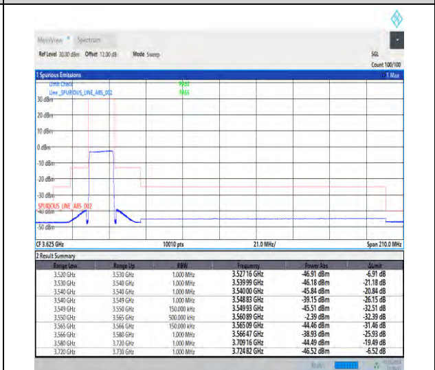
1-N48-30-15-L-6-CP-QPSK-Outer_Full-38@0-Ant3-1--PASS-see graph
