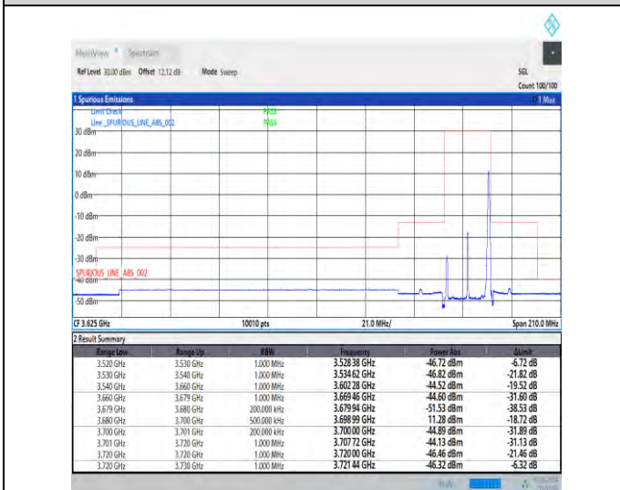
1-N48-30-20-H-5-CP-QPSK-Edge_1RB_Right-1@50-Ant3-1--PASS-see graph
