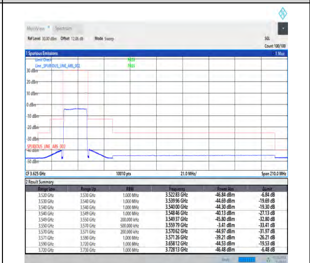
1-N48-30-20-L-6-CP-QPSK-Outer_Full-51@0-Ant3-1--PASS-see graph
