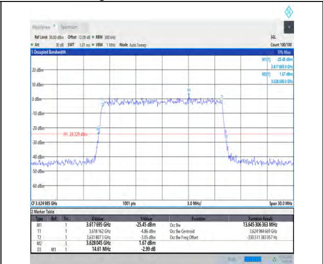
1-N48-30-15-M-9-CP-256QAM-Outer_Full-38@0-Ant3 -13.645-14.610-≤15-PASS
