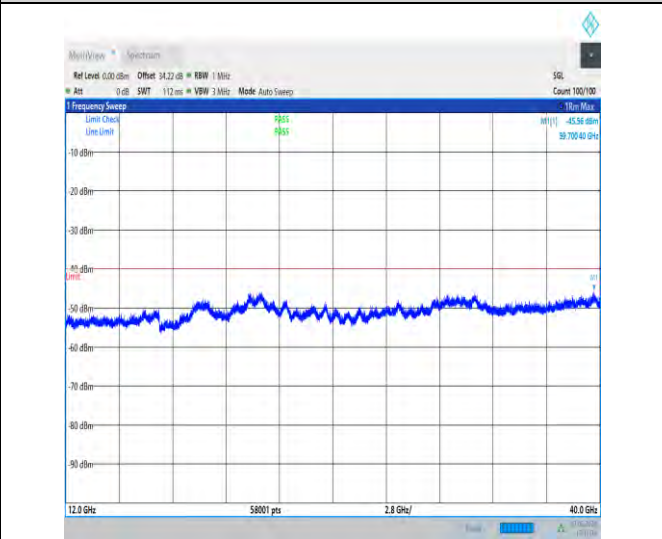
1-N48-30-40-M-1-DFT-PI2BPSK-Inner_1RB_Left-1 @ 1-12000-40000-Ant3-39713.00--45.56--40-PASS
