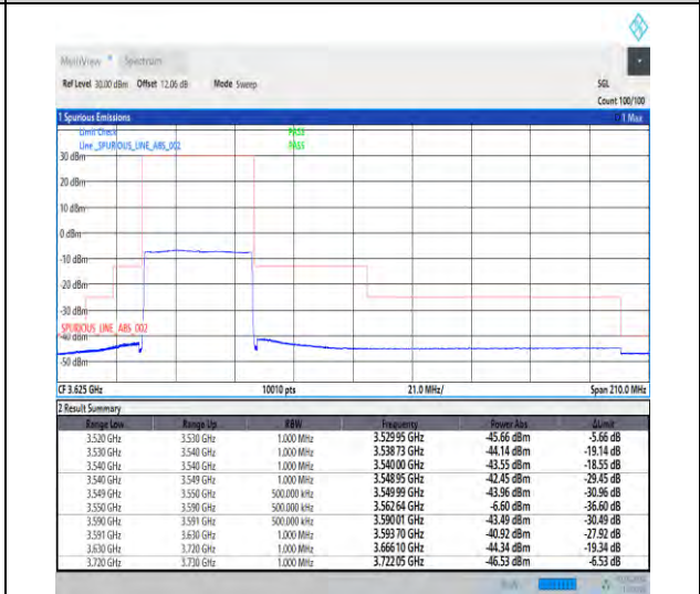
1-N48-30-40-L-6-CP-QPSK-Outer_Full-106@0-Ant3-1--PASS-see graph
