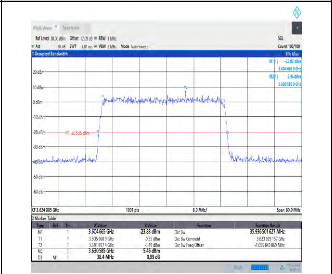
1-N48-30-40-M-5-DFT-256QAM-Outer_Full-100@0-Ant3-35.937-38.400-≤40-PASS
