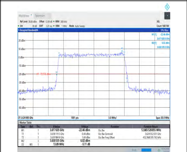
1-N48-30-15-M-3-DFT-16QAM-Outer_Full-36@0-Ant 3-12.866-13.890-≤15-PASS
