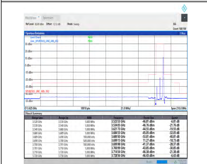
1-N48-30-10-H-5-CP-QPSK-Edge_1RB_Right-1@23-Ant3-1--PASS-see graph
