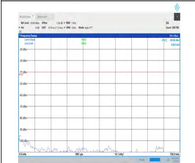
1-N48-30-40-M-1-DFT-PI2BPSK-Inner_1RB_Left-1 @ 1-0.009-0.15-Ant3-0.01--99.38--40-PASS
