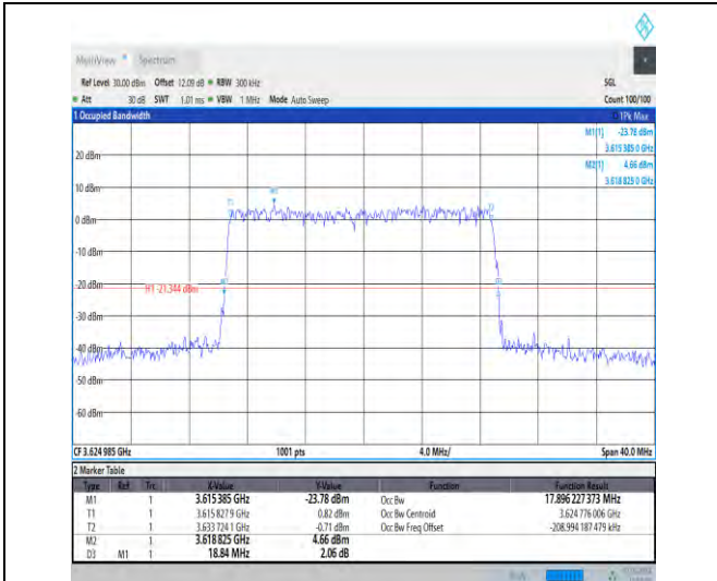
1-N48-30-20-M-3-DFT-16QAM-Outer_Full-50@0-Ant 3-17.896-18.840-≤20-PASS
