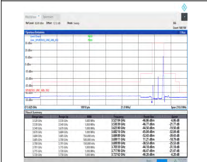
1-N48-30-15-H-5-CP-QPSK-Edge_1RB_Right-1@37-Ant3-1--PASS-see graph
