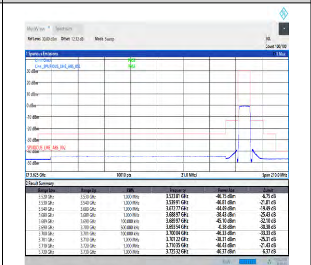
1-N48-30-10-H-6-CP-QPSK-Outer_Full-24@0-Ant3-1--PASS-see graph
