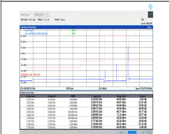
1-N48-30-40-H-5-CP-QPSK-Edge_1RB_Right-1@105-Ant3-1--PASS-see graph
