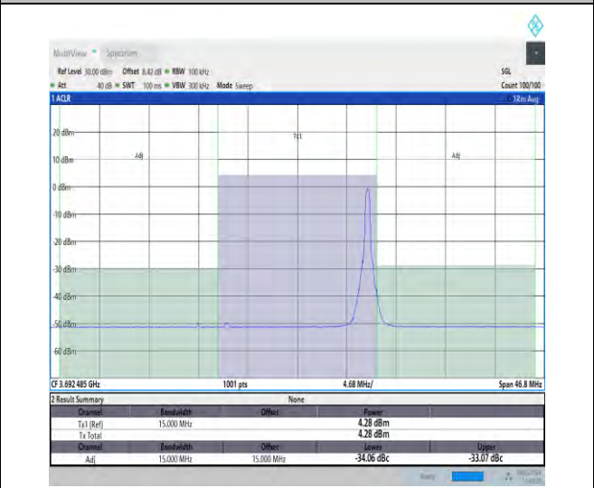
NTVN_N48_PC3_30_15_H_TID18_#1_-15_15
