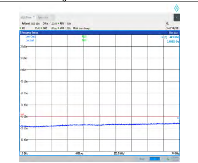
1-N48-30-40-M-1-DFT-PI2BPSK-Inner_1RB_Left-1 @ 1-1000-3000-Ant3-2963.50--44.98--40-PASS
