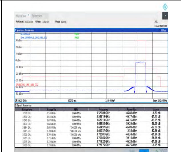
1-N48-30-15-H-6-CP-QPSK-Outer_Full-38@0-Ant3-1--PASS-see graph
