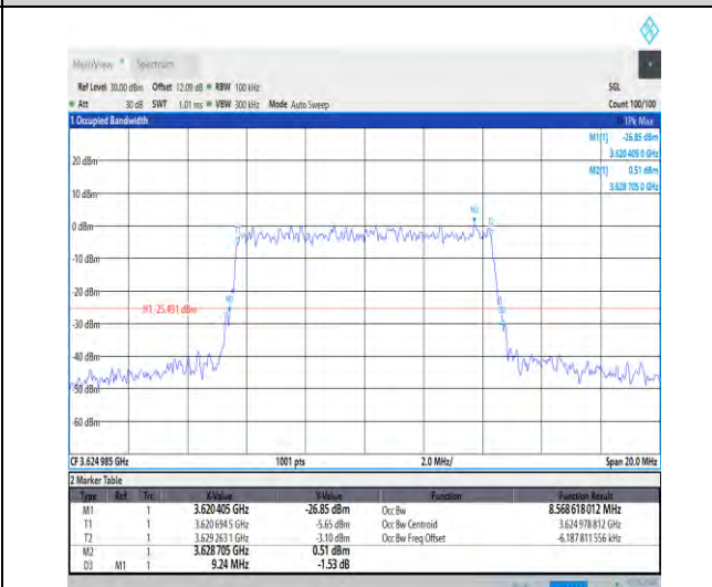
1-N48-30-10-M-8-CP-64QAM-Outer_Full-24@0-Ant 3-8.569-9.240≤10-PASS
