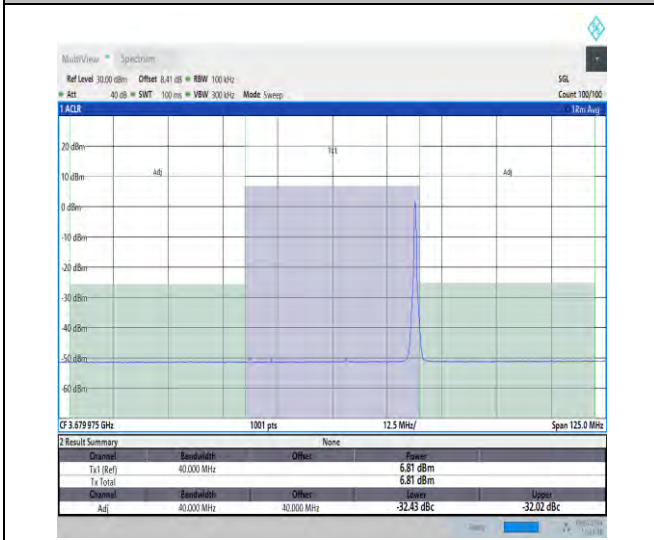
NTVN_N48_PC3_30_40_H_TID3_#1_-40_40
