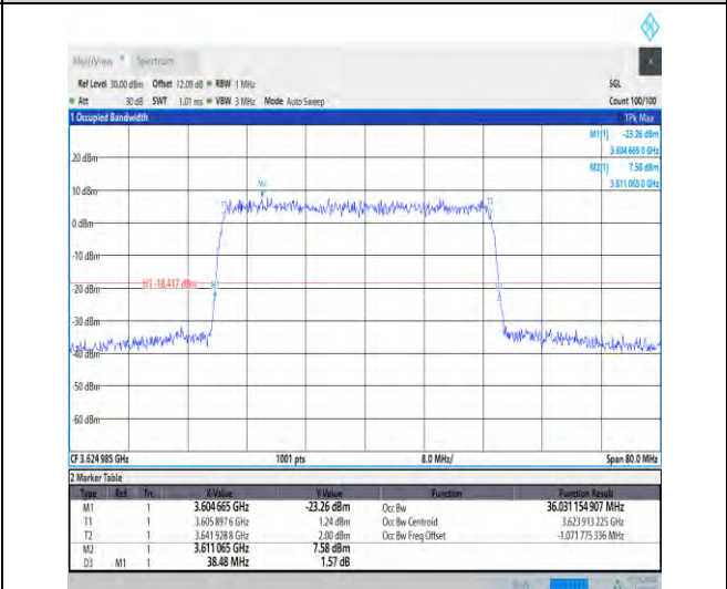
1-N48-30-40-M-1-DFT-QPSK-Outer_Full-100@0-Ant 3-36.031-38.480-≤40-PASS
