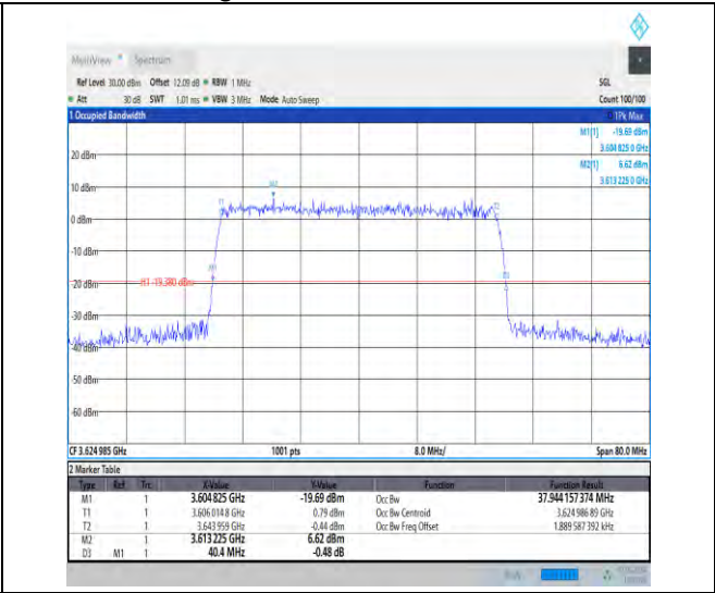
1-N48-30-40-M-7-CP-16QAM-Outer_Full-106@0-Ant3 -37.944-40.400-≤40-PASS
