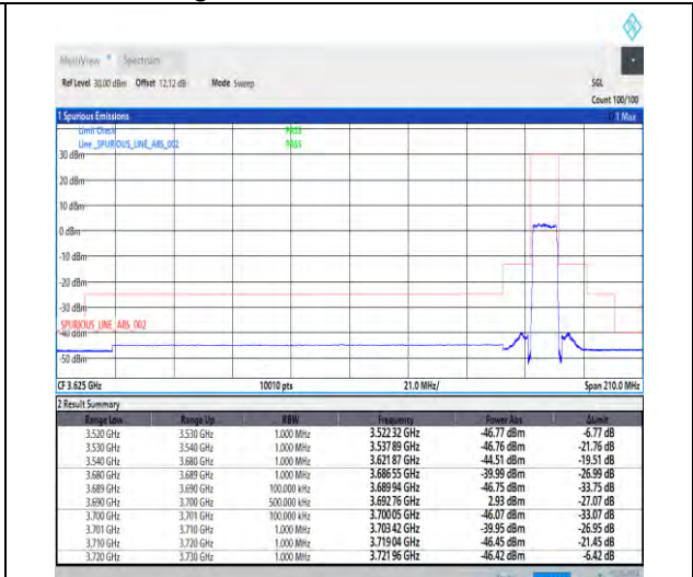
1-N48-30-10-H-3-DFT-PI2BPSK-Outer_Full-24@0-Ant3-1--PASS-see graph
