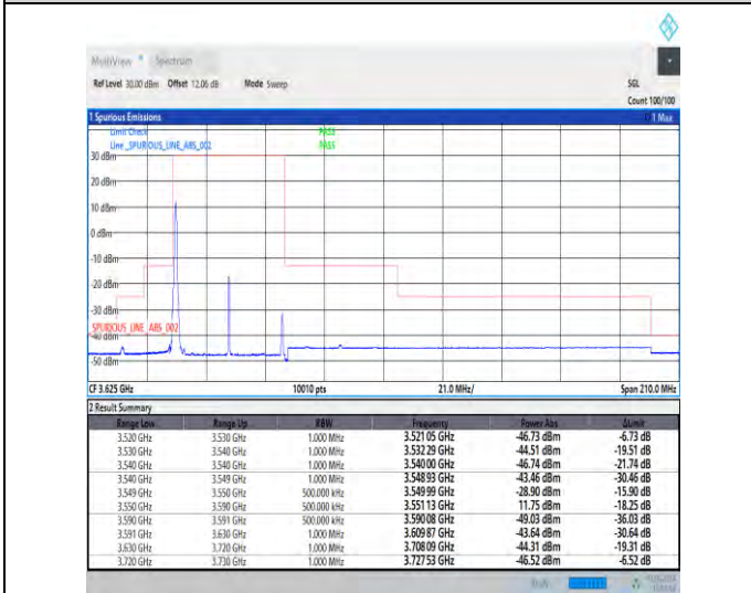
1-N48-30-40-L-4-CP-QPSK-Edge_1RB_Left-1@0-Ant3-1--PASS-see graph
