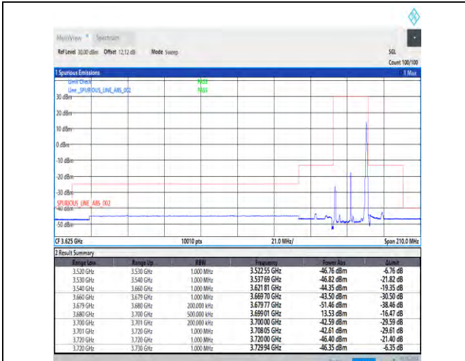
1-N48-30-20-H-2-DFT-PI2BPSK-Edge_1RB_Right-1@50-Ant3-1--PASS-see graph
