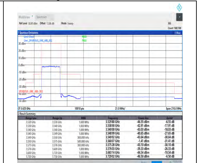
1-N48-30-25-L-3-DFT-PI2BPSK-Outer_Full-64@0-Ant3-1--PASS-see graph
