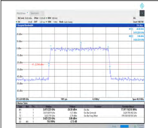
1-N48-30-20-M-5-DFT-256QAM-Outer_Full-50@0-A nt3-17.911-19.000-≤20-PASS
