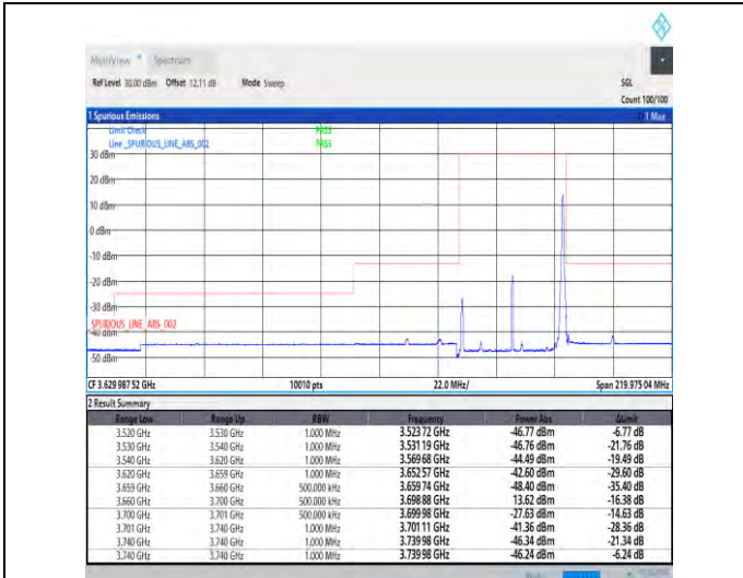
1-N48-30-40-H-2-DFT-PI2BPSK-Edge_1RB_Right-1@105-Ant3-1--PASS-see graph
