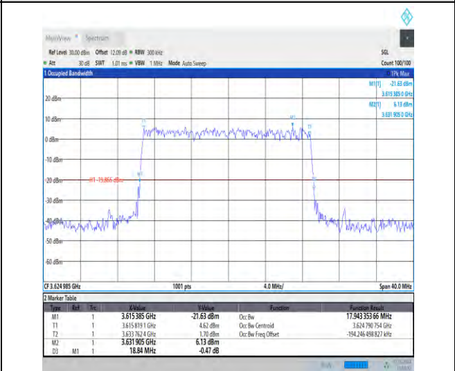
1-N48-30-20-M-2-DFT-PI2BPSK-Outer_Full-50@0-Ant3 -17.943-18.840-≤20-PASS
