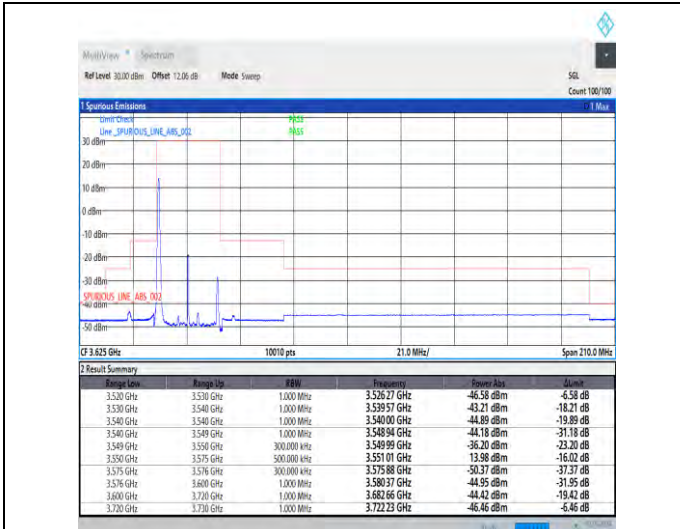
1-N48-30-25-L-1-DFT-PI2BPSK-Edge_1RB_Left-1@0-Ant3-1--PASS-see graph
