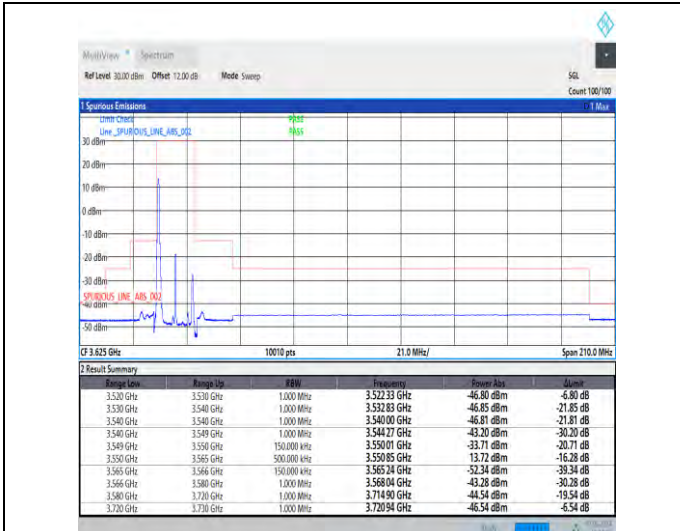
1-N48-30-15-L-1-DFT-PI2BPSK-Edge_1RB_Left-1@0-Ant3-1--PASS-see graph
