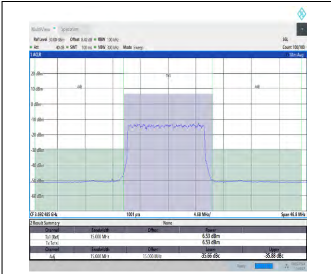
NTVN_N48_PC3_30_15_H_TID1_#1_-15_15
