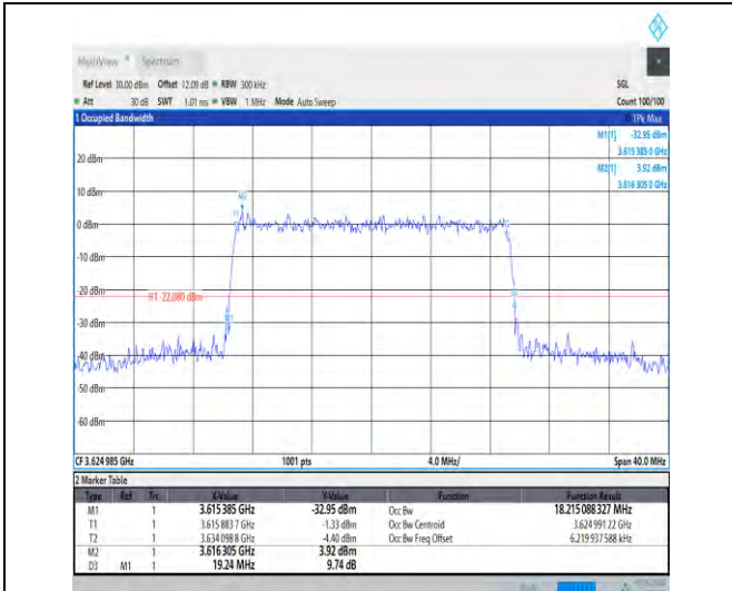
1-N48-30-20-M-7-CP-16QAM-Outer_Full-51@0-Ant3 -18.215-19.240-≤20-PASS
