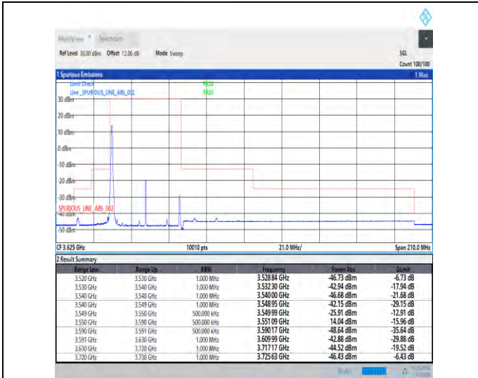
1-N48-30-40-L-1-DFT-PI2BPSK-Edge_1RB_Left-1@0-Ant3-1--PASS-see graph
