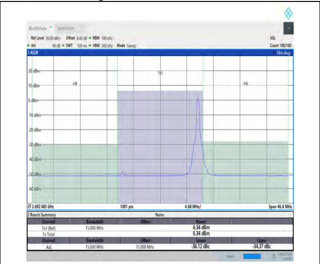
NTVN_N48_PC3_30_15_H_TID3_#1_-15_15
