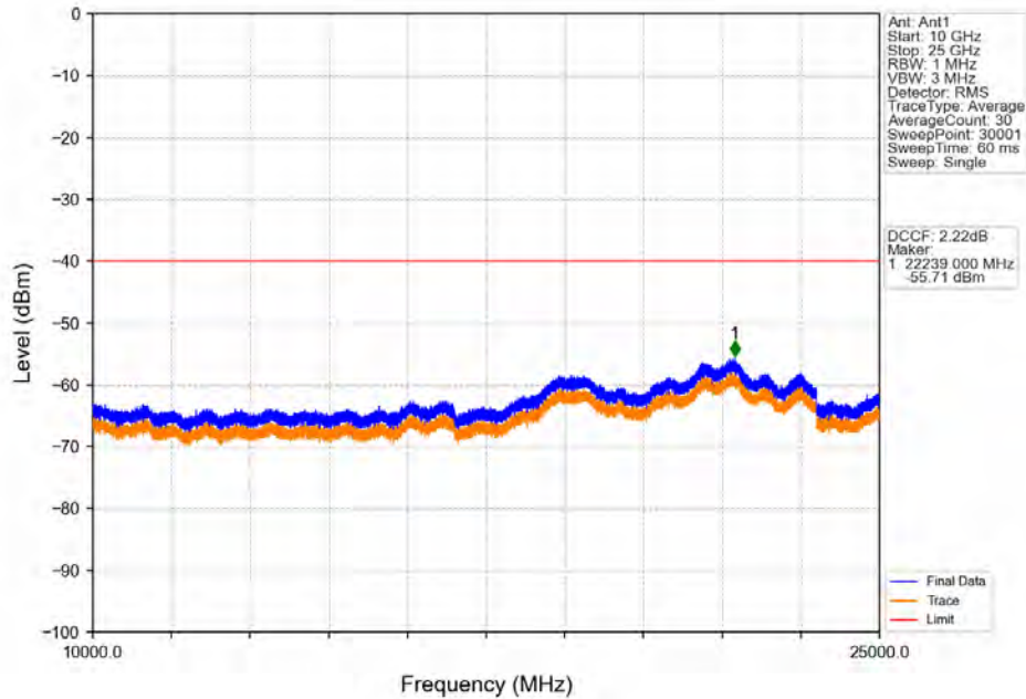
Band48_5MHz_QPSK_LCH_3552.5MHz_RB_1_0_NTNV
