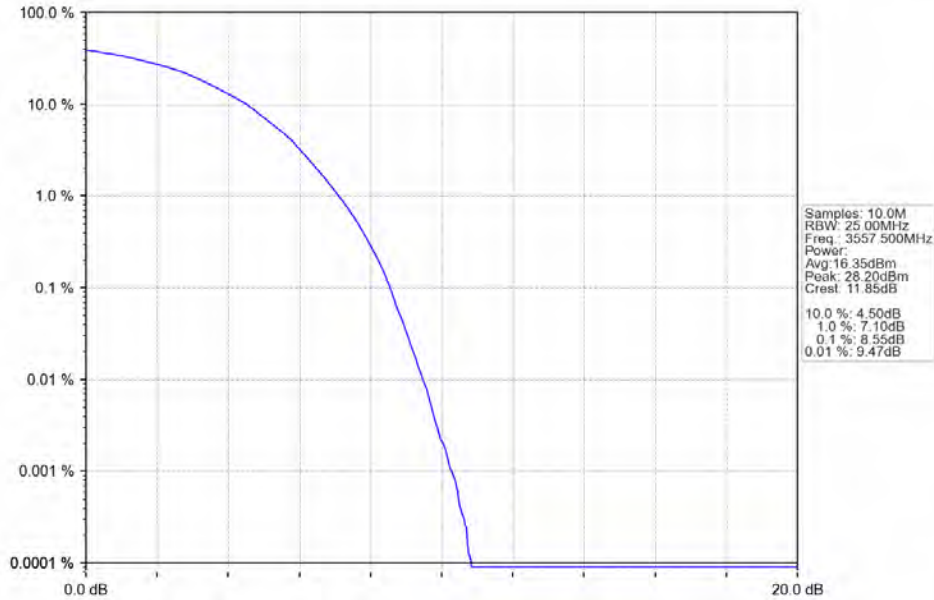
Band48_15MHz_64QAM_LCH_3557.5MHz_RB_75_0_NTNV
