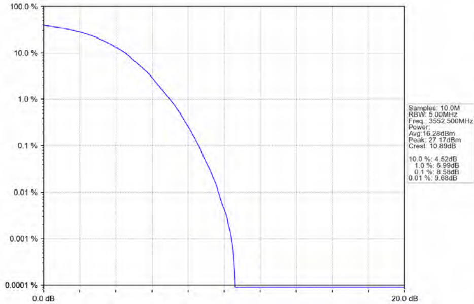
Band48_5MHz_64QAM_LCH_3552.5MHz_RB_25_0_NTNV
