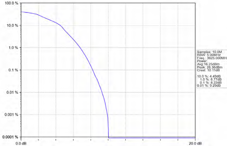
Band48_5MHz_16QAM_MCH_3625MHz_RB_25_0_NTNV
