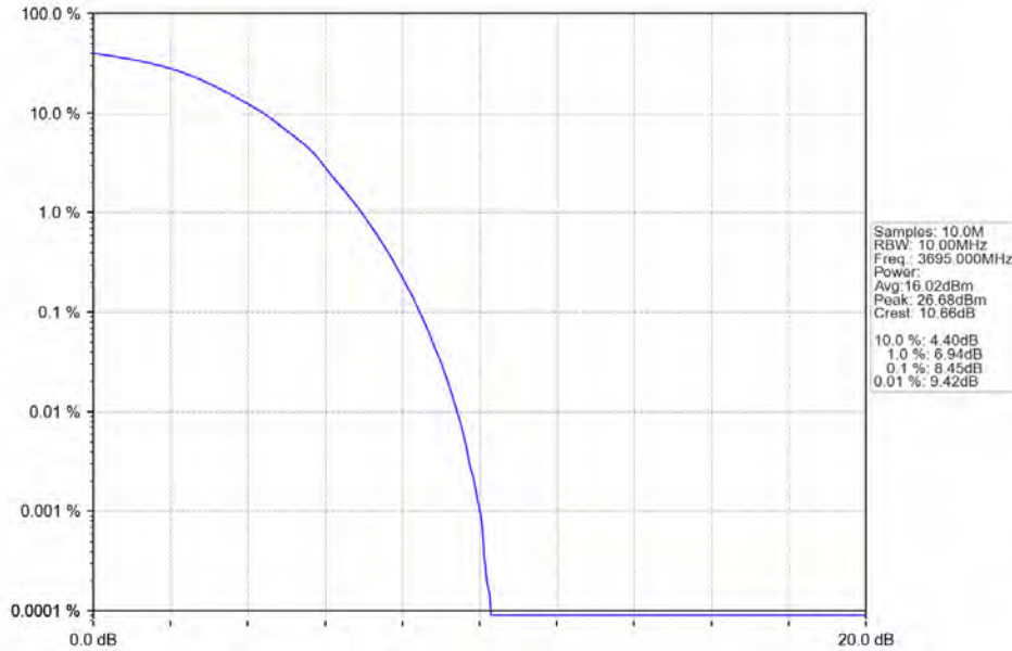
Band48_10MHz_64QAM_HCH_3695MHz_RB_50_0_NTNV
