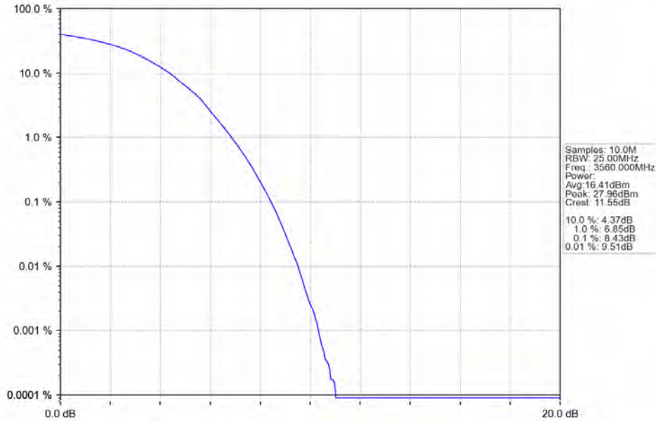
Band48_20MHz_64QAM_LCH_3560MHz_RB_100_0_NTNV
