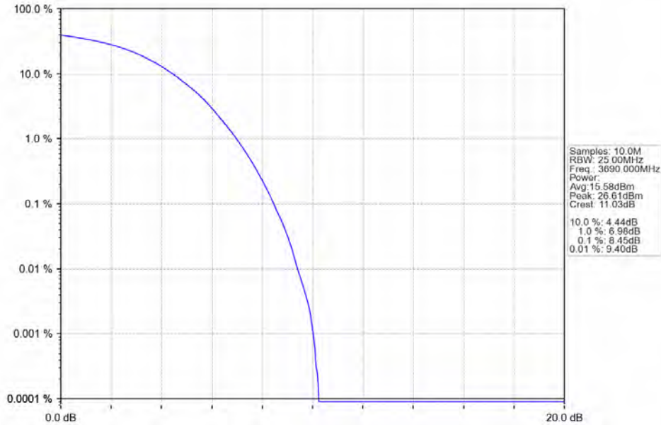
Band48_20MHz_64QAM_HCH_3690MHz_RB_100_0_NTNV
