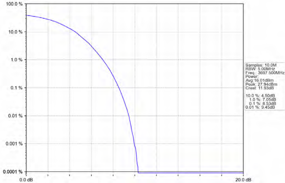
Band48_5MHz_64QAM_HCH_3697.5MHz_RB_25_0_NTNV
