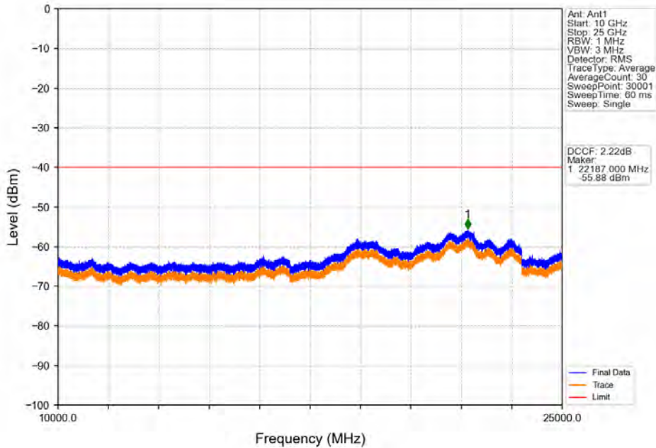
Band48_5MHz_QPSK_MCH_3625MHz_RB_1_0_NTNV
