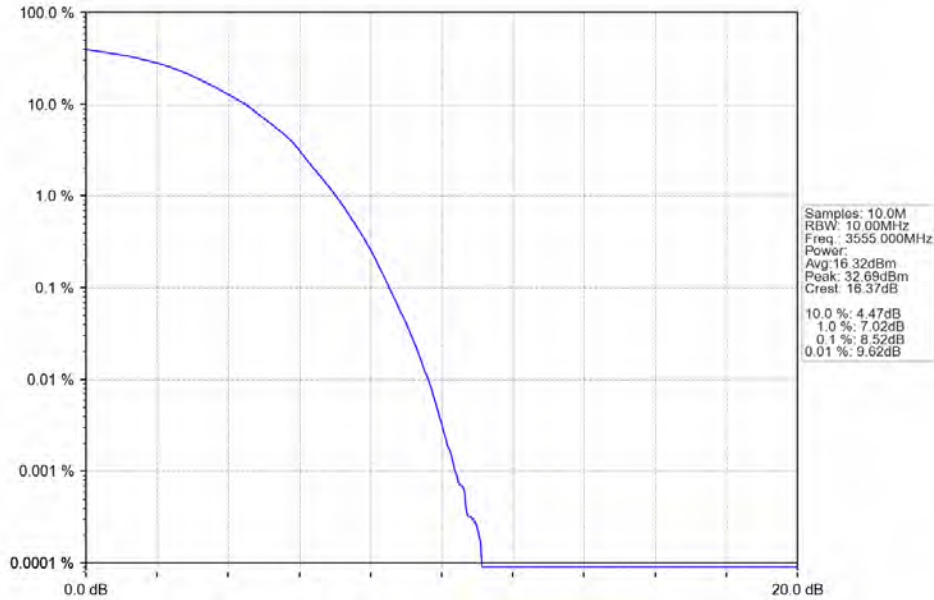
Band48_10MHz_64QAM_LCH_3555MHz_RB_50_0_NTNV
