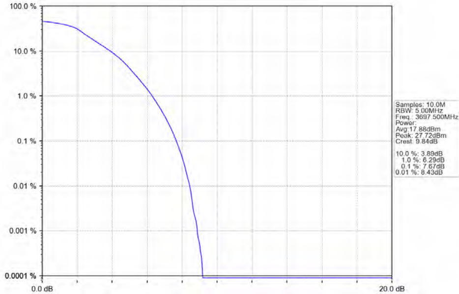
Band48_5MHz_QPSK_HCH_3697.5MHz_RB_25_0_NTNV
