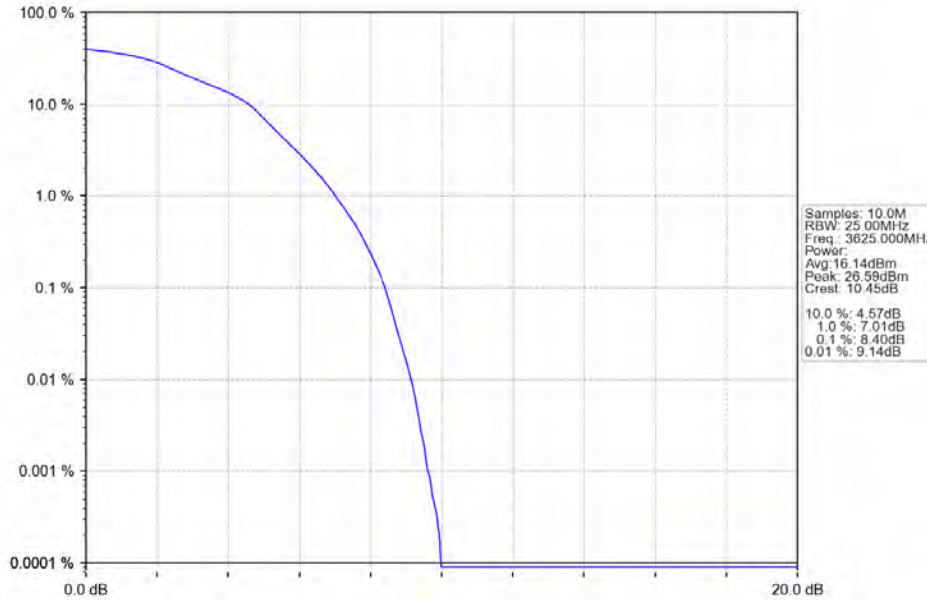
Band48_15MHz_16QAM_MCH_3625MHz_RB_75_0_NTNV
