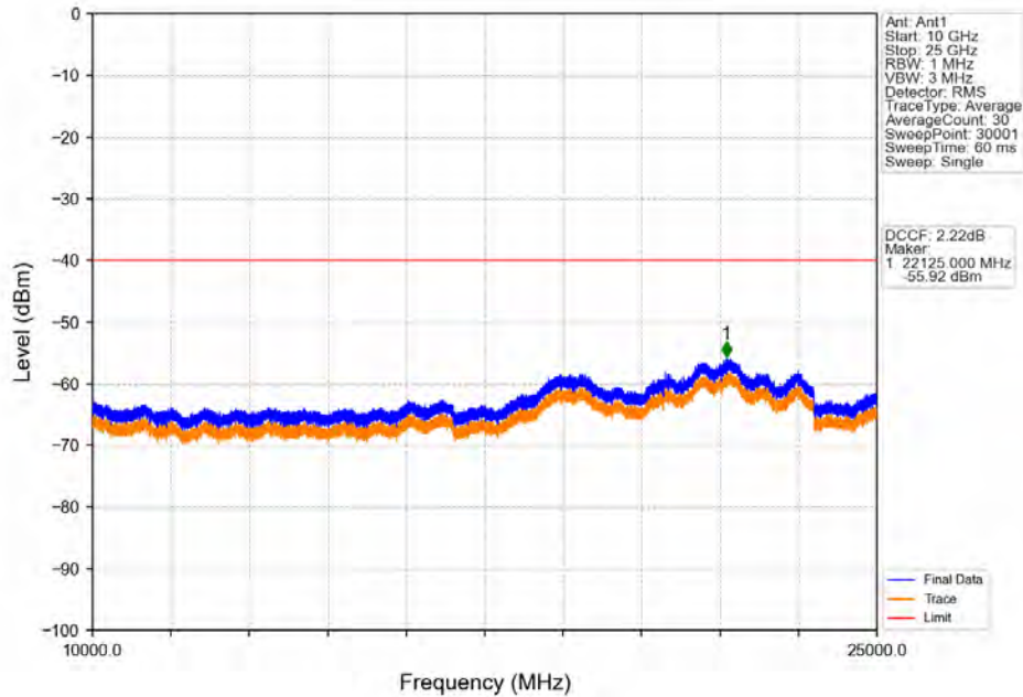
Band48_15MHz_QPSK_LCH_3557.5MHz_RB_1_0_NTNV
