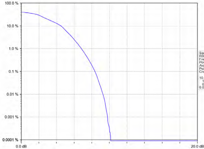
Band48_10MHz_16QAM_MCH_3625MHz_RB_50_0_NTNV
