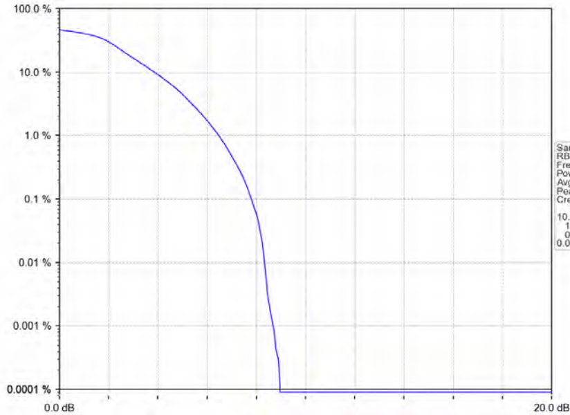
Band48_15MHz_QPSK_HCH_3692.5MHz_RB_75_0_NTNV
