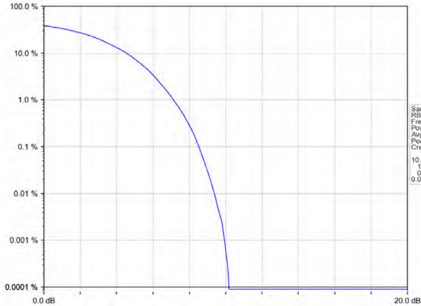
Band48_15MHz_64QAM_HCH_3692.5MHz_RB_75_0_NTNV
