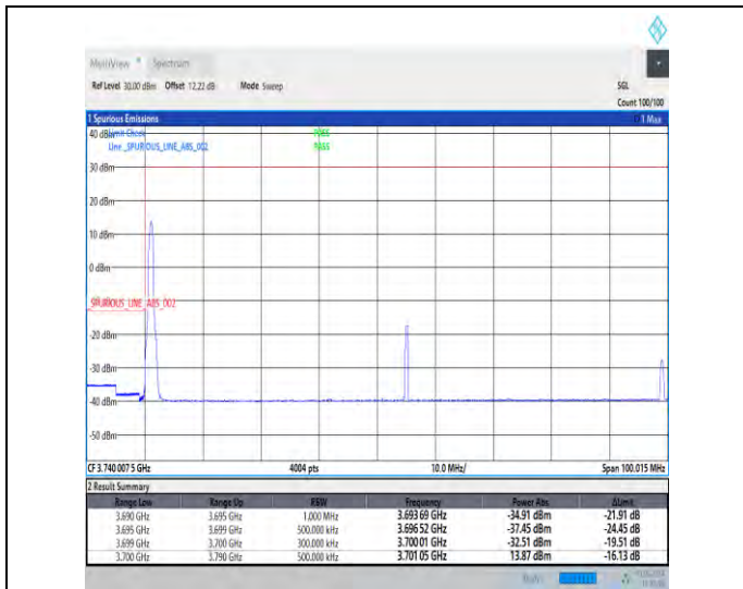
1-N77-3700-3980-30-90-L-1-DFT-PI2BPSK-Edge_1RB _Left-1@0-Ant3-1--PASS-see graph
