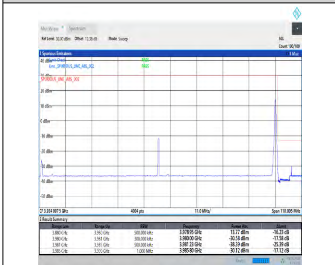
1-N77-3700-3980-30-100-H-5-CP-QPSK-Edge_1RB_Right-1@272-Ant3-1--PASS-see graph
