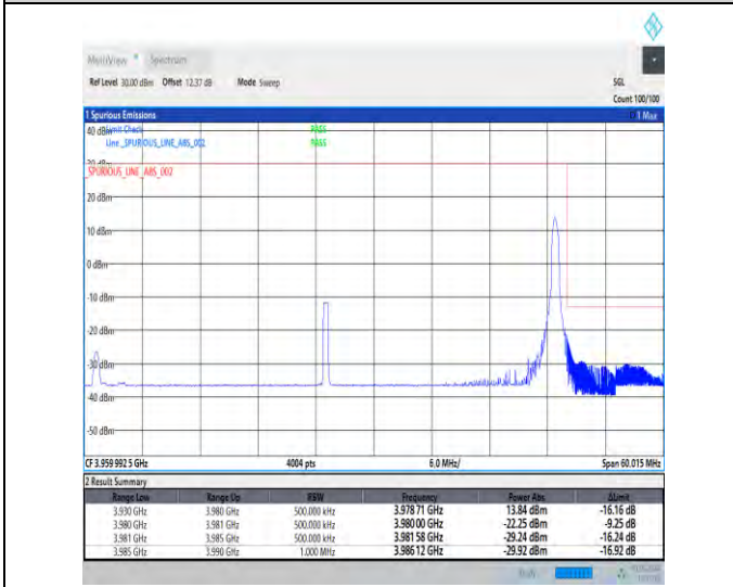
1-N77-3700-3980-30-50-H-5-CP-QPSK-Edge_1RB_Right-1@132-Ant3-1--PASS-see graph
