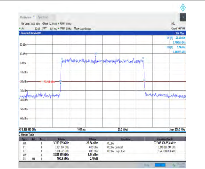
1-N77-3700-3980-30-100-M-7-CP-16QAM-Outer_Full-273@0-Ant3-97.305-100.800-≤100-PASS
