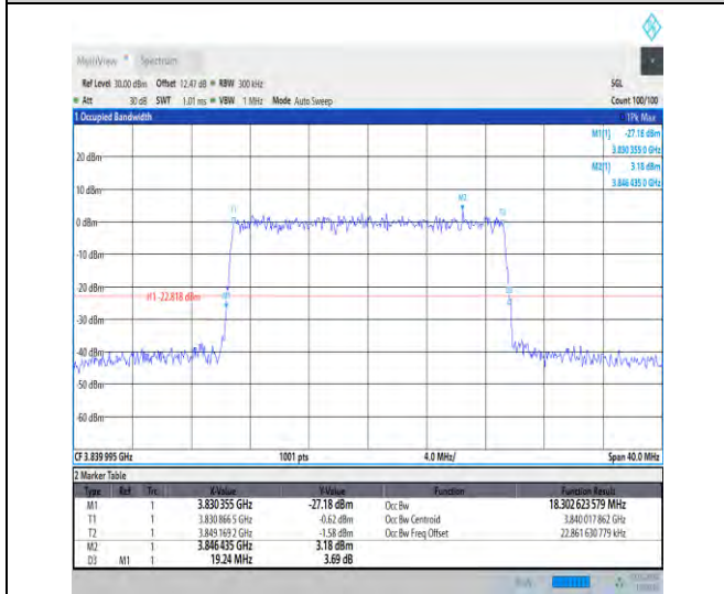
1-N77-3700-3980-30-20-M-9-CP-256QAM-Outer_Fu ll-51@0-Ant3-18.303-19.240-<=20-PASS
