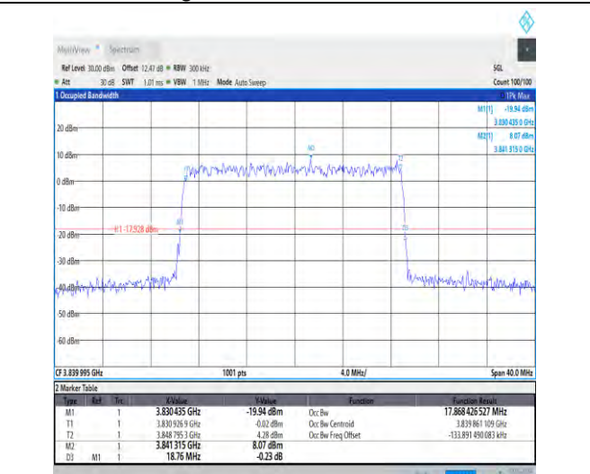
1-N77-3700-3980-30-20-M-4-DFT-64QAM-Outer_Ful I-50@0-Ant3-17.868-18.760-≤20-PASS
