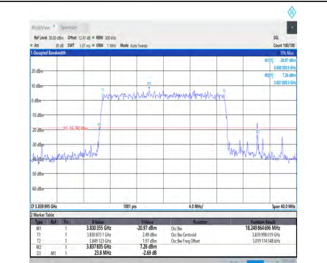
1-N77-3700-3980-30-20-M-6-CP-QPSK-Outer_Full-50@0-Ant3-18.25-23.800-≤20-PASS
