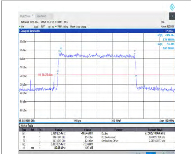
1-N77-3700-3980-30-80-M-6-CP-QPSK-Outer_Full-217@0-Ant3-77.502-80.480-≤80-PASS
