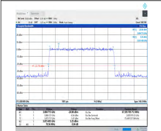
1-N77-3700-3980-30-70-M-9-CP-256QAM-Outer_Fu II-189@0-Ant3-67.596-70.560-≤70-PASS
