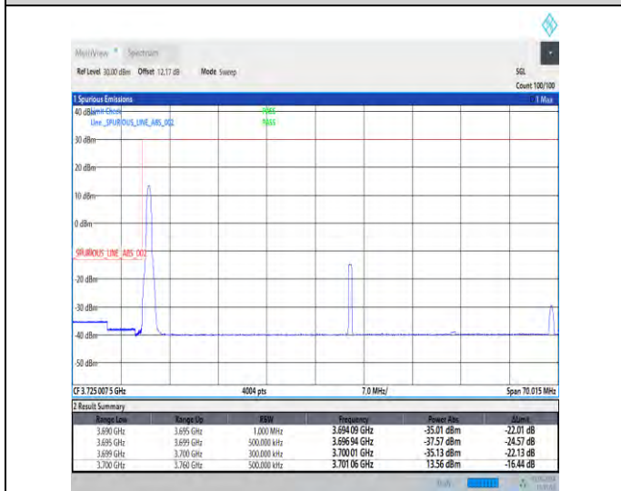
1-N77-3700-3980-30-60-L-4-CP-QPSK-Edge_1RB_Lef t-1@0-Ant3-1--PASS-see graph
