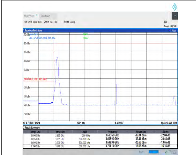
1-N77-3700-3980-30-40-L-4-CP-QPSK-Edge_1RB_Lef t-1@0-Ant3-1--PASS-see graph
