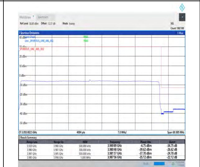
1-N77-3700-3980-30-60-H-6-CP-QPSK-Outer_Full-162@0-Ant3-1--PASS-see graph
