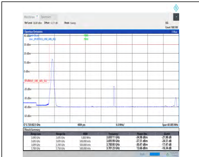
1-N77-3700-3980-30-50-L-1-DFT-PI2BPSK-Edge_1RB_Left-1@0-Ant3-1--PASS-see graph
