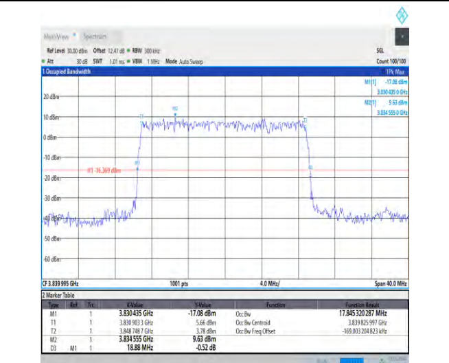
1-N77-3700-3980-30-20-M-2-DFT-PI2BPSK-Outer_F ull-50@0-Ant3-17.845-18.880-≤20-PASS
