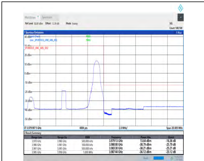
1-N77-3700-3980-30-10-H-2-DFT-PI2BPSK-Edge_1R_B_Right-1@23-Ant3-1--PASS-see graph
