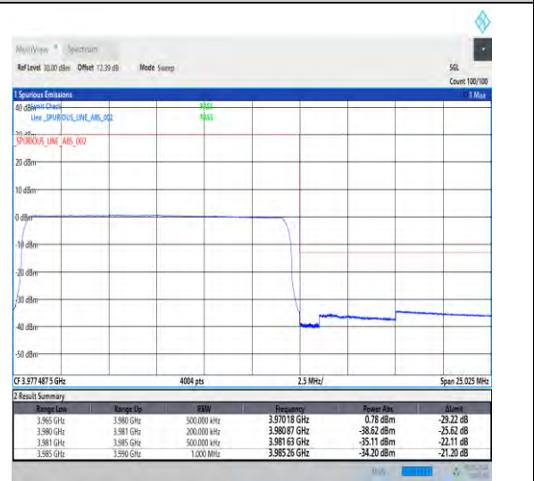
1-N77-3700-3980-30-15-H-6-CP-QPSK-Outer_Full-38@0-Ant3-1--PASS-see graph
