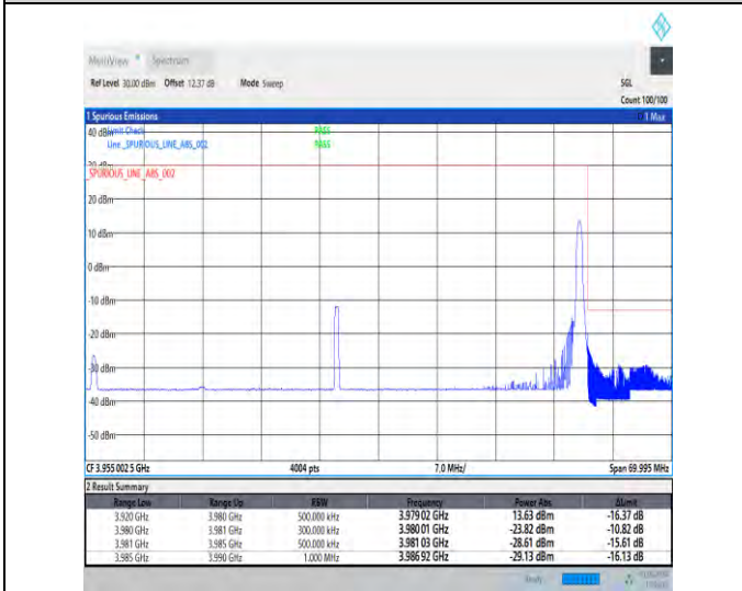
1-N77-3700-3980-30-60-H-5-CP-QPSK-Edge_1RB_Right-1@161-Ant3-1--PASS-see graph
