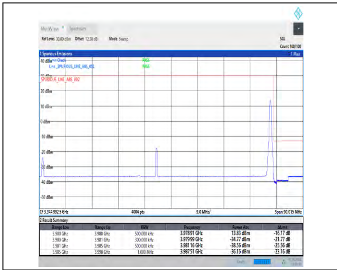
1-N77-3700-3980-30-80-H-2-DFT-PI2BPSK-Edge_1R_B_Right-1@216-Ant3-1--PASS-see graph
