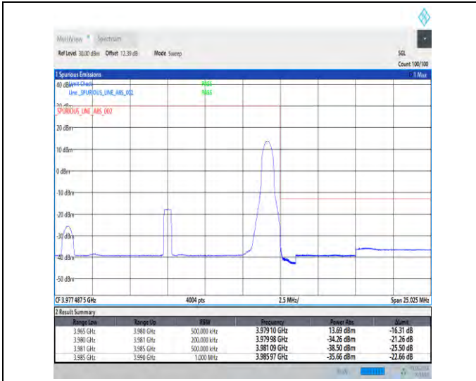
1-N77-3700-3980-30-15-H-2-DFT-PI2BPSK-Edge_1R_B_Right-1@37-Ant3-1--PASS-see graph
