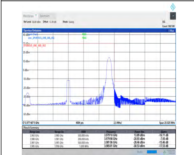
1-N77-3700-3980-30-15-H-5-CP-QPSK-Edge_1RB_Right-1@37-Ant3-1--PASS-see graph
