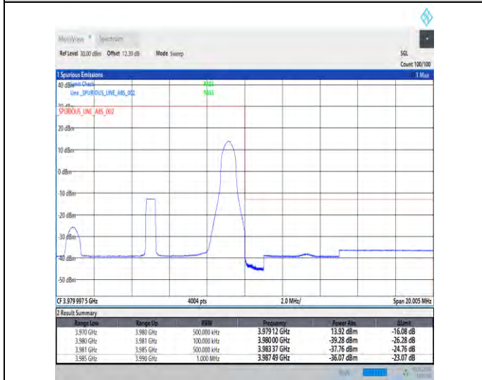
1-N77-3700-3980-30-10-H-5-CP-QPSK-Edge_1RB_Right-1@23-Ant3-1--PASS-see graph
