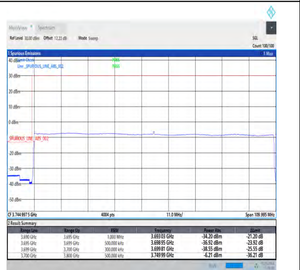
1-N77-3700-3980-30-100-L-6-CP-QPSK-Outer_Full-273@0-Ant3-1--PASS-see graph
