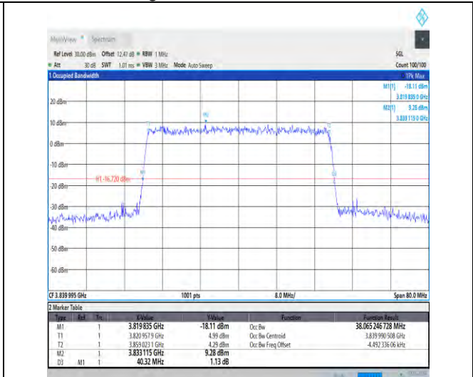
1-N77-3700-3980-30-40-M-7-CP-16QAM-Outer_Full-106@0-Ant3-38.065-40.320-<math>\leq 40</math>-PASS
