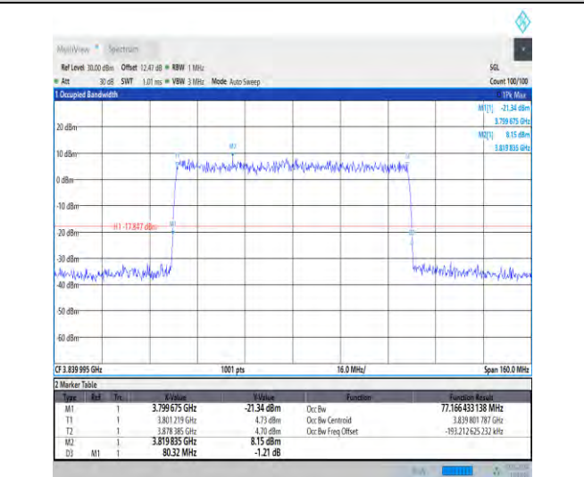
1-N77-3700-3980-30-80-M-1-DFT-QPSK-Outer_Full- 216@0-Ant3-77.166-80.320-≤80-PASS
