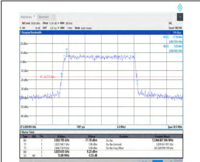
1-N77-3700-3980-30-15-M-4-DFT-64QAM-Outer_Fu II-36@0-Ant3-12.967-13.890-≤15-PASS
