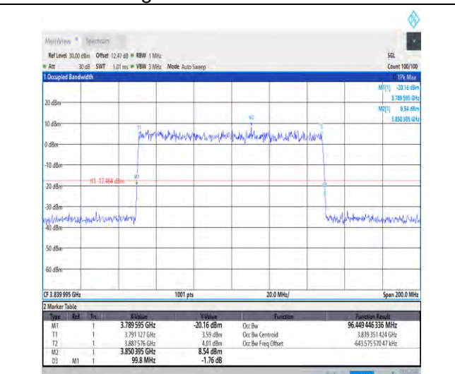
1-N77-3700-3980-30-100-M-1-DFT-QPSK-Outer_Ful I-270@0-Ant3-96.449-99.800-≤100-PASS
