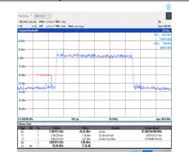
1-N77-3700-3980-30-90-M-6-CP-QPSK-Outer_Full-245@0-Ant3-87.38-95.940-≤90-PASS
