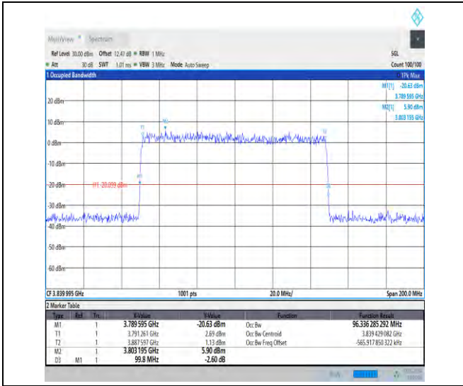
1-N77-3700-3980-30-100-M-4-DFT-64QAM-Outer_Full-270@0-Ant3-96.336-99.800-≤100-PASS
