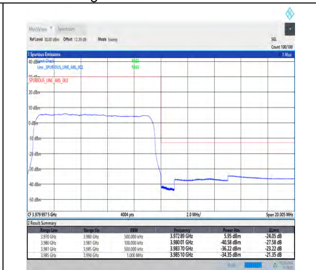
1-N77-3700-3980-30-10-H-3-DFT-PI2BPSK-Outer_Full-24@0-Ant3-1--PASS-see graph
