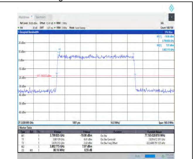
1-N77-3700-3980-30-80-M-3-DFT-16QAM-Outer_Full-216@0-Ant3-77.165-80.160-≤80-PASS
