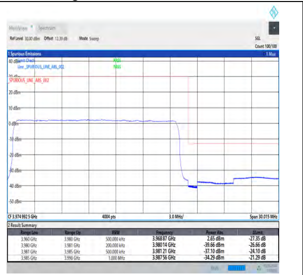
1-N77-3700-3980-30-20-H-3-DFT-PI2BPSK-Outer_Full-50@0-Ant3-1--PASS-see graph
