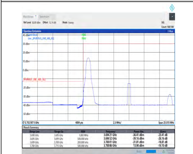
1-N77-3700-3980-30-15-L-4-CP-QPSK-Edge_1RB_Lef t-1@0-Ant3-1--PASS-see graph
