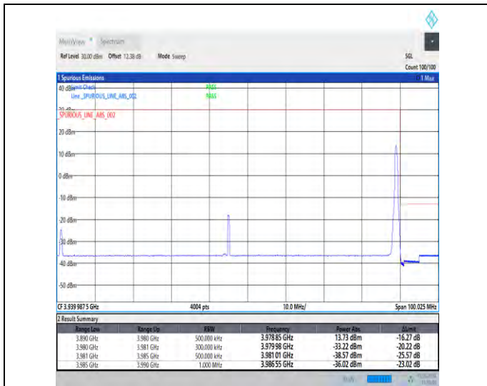
1-N77-3700-3980-30-90-H-2-DFT-PI2BPSK-Edge_1R_B_Right-1@244-Ant3-1--PASS-see graph
