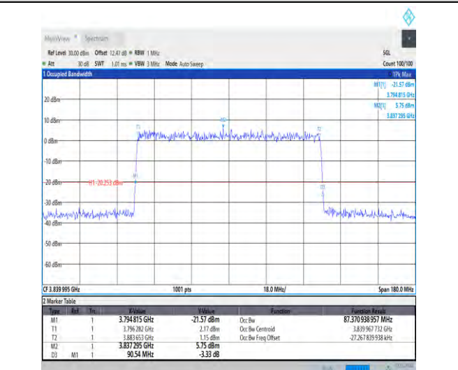
1-N77-3700-3980-30-90-M-8-CP-64QAM-Outer_Full-245@0-Ant3-87.371-90.540-≤90-PASS
