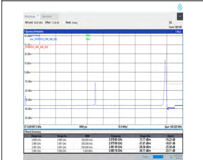
1-N77-3700-3980-30-90-H-5-CP-QPSK-Edge_1RB_Right-1@244-Ant3-1--PASS-see graph
