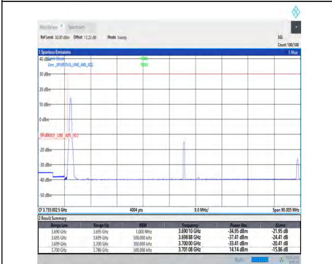
1-N77-3700-3980-30-80-L-4-CP-QPSK-Edge_1RB_Lef t-1@0-Ant3-1--PASS-see graph
