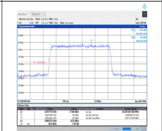
1-N77-3700-3980-30-40-M-5-DFT-256QAM-Outer_Full-100@0-Ant3-35.926-38.400-≤40-PASS
