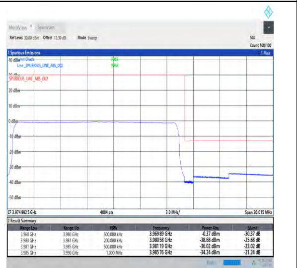
1-N77-3700-3980-30-20-H-6-CP-QPSK-Outer_Full-51@0-Ant3-1--PASS-see graph
