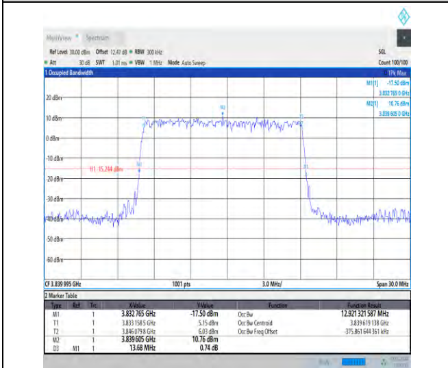
1-N77-3700-3980-30-15-M-2-DFT-P12BPSK-Outer_Full Full-36@0-Ant3-12.921-13.680-≤15-PASS
