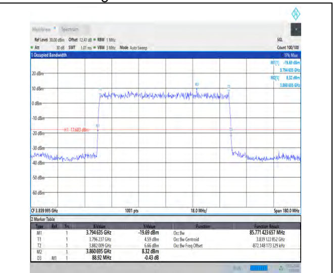
1-N77-3700-3980-30-90-M-2-DFT-PI2BPSK-Outer_Full-240@0-Ant3-85.771-88.920-≤90-PASS
