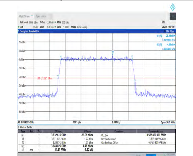
1-N77-3700-3980-30-15-M-9-CP-256QAM-Outer_Ful I-38@0-Ant3-13.587-14.610-≤15-PASS
