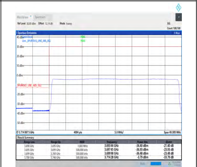
1-N77-3700-3980-30-40-L-6-CP-QPSK-Outer_Full -106@0-Ant3-1--PASS-see graph
