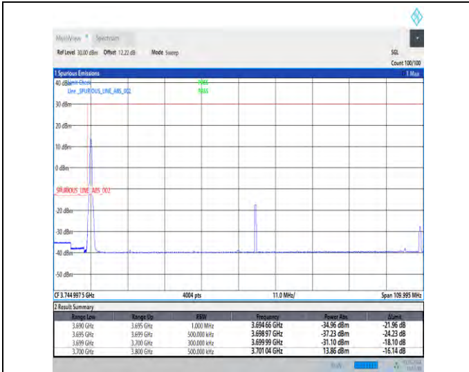
1-N77-3700-3980-30-100-L-1-DFT-PI2BPSK-Edge_1R_B_Left-1@0-Ant3-1--PASS-see graph
