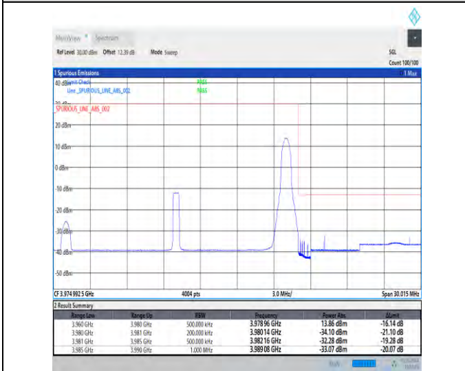
1-N77-3700-3980-30-20-H-5-CP-QPSK-Edge_1RB_Right-1@50-Ant3-1--PASS-see graph
