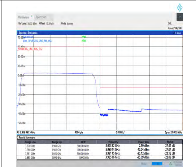
1-N77-3700-3980-30-10-H-6-CP-QPSK-Outer_Full-24@0-Ant3-1--PASS-see graph
