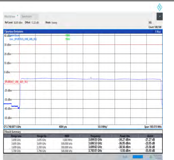
1-N77-3700-3980-30-90-L-6-CP-QPSK-Outer_Full -245@0-Ant3-1--PASS-see graph
