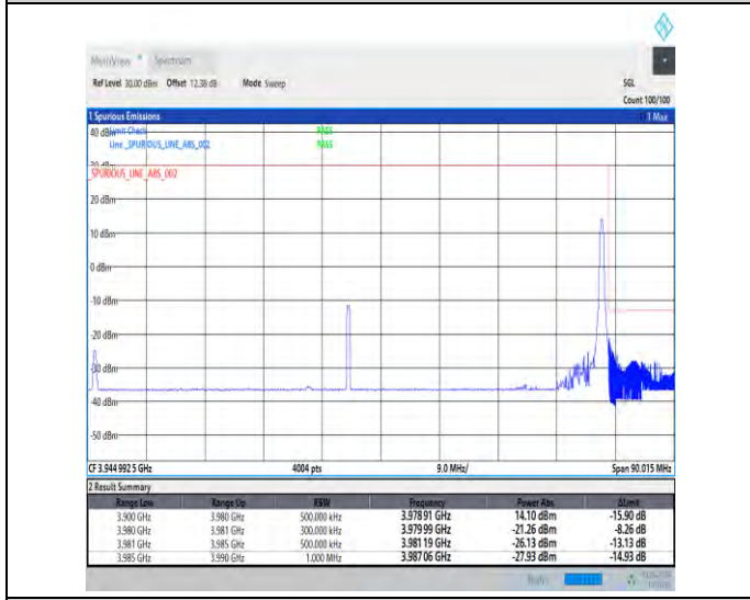
1-N77-3700-3980-30-80-H-5-CP-QPSK-Edge_1RB_Right-1@216-Ant3-1--PASS-see graph
