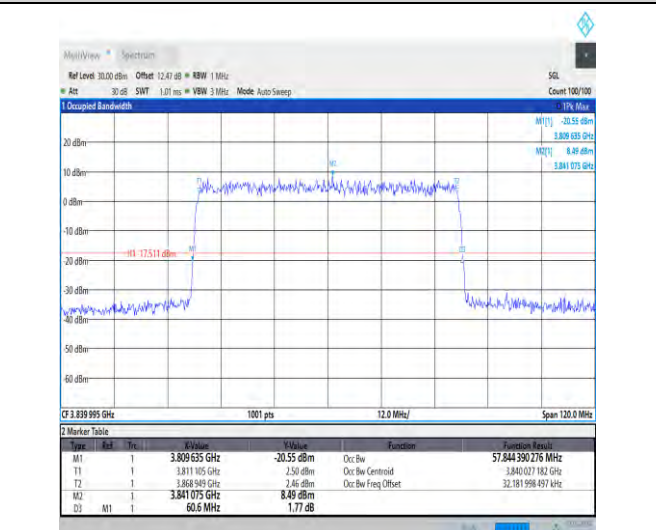
1-N77-3700-3980-30-60-M-3-DFT-16QAM-Outer_Full-162@0-Ant3-57.844-60.600-≤60-PASS
