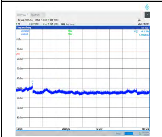
1-N77-3700-3980-30-100-M-1-DFT-PI2BPSK-Inner_1RB_Left-1@1-6000-18000-Ant3-7491.84--46.62--1 3-PASS
