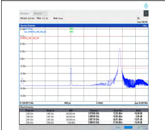
1-N77-3700-3980-30-40-H-5-CP-QPSK-Edge_1RB_Right-1@105-Ant3-1--PASS-see graph
