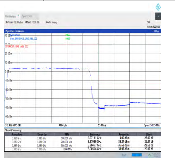
1-N77-3700-3980-30-15-H-3-DFT-PI2BPSK-Outer_Full-36@0-Ant3-1--PASS-see graph
