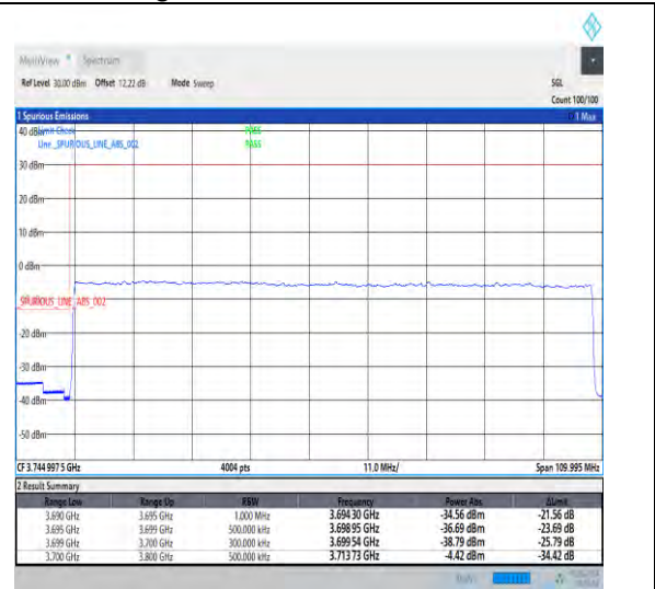
1-N77-3700-3980-30-100-L-3-DFT-PI2BPSK-Outer_Full-270@0-Ant3-1--PASS-see graph
