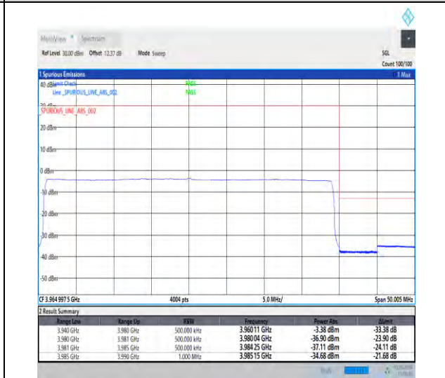
1-N77-3700-3980-30-40-H-6-CP-QPSK-Outer_Full-106@0-Ant3-1--PASS-see graph
