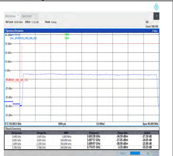
1-N77-3700-3980-30-80-L-3-DFT-PI2BPSK-Outer_Full-216@0-Ant3-1--PASS-see graph
