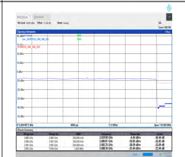
1-N77-3700-3980-30-100-H-6-CP-QPSK-Outer_Full-273@0-Ant3-1--PASS-see graph
