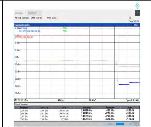
1-N77-3700-3980-30-50-H-6-CP-QPSK-Outer_Full-133@0-Ant3-1--PASS-see graph
