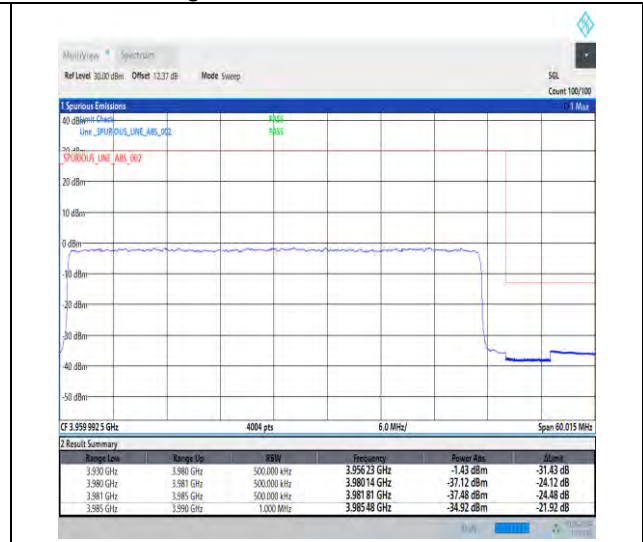
1-N77-3700-3980-30-50-H-3-DFT-PI2BPSK-Outer_Full-128@0-Ant3-1--PASS-see graph
