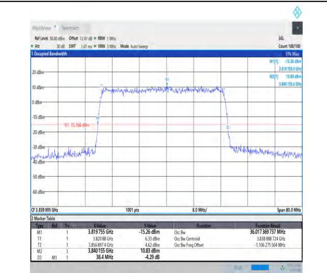
1-N77-3700-3980-30-40-M-1-DFT-QPSK-Outer_Full- 100@0-Ant3-36.017-38.400-<=40-PASS
