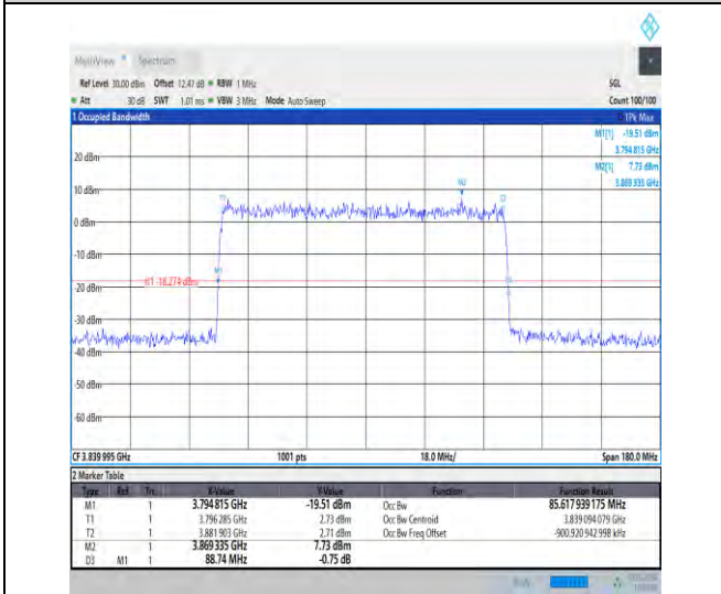
1-N77-3700-3980-30-90-M-3-DFT-16QAM-Outer_Full-240@0-Ant3-85.618-88.740-≤90-PASS
