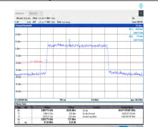
1-N77-3700-3980-30-70-M-4-DFT-64QAM-Outer_Ful I-180@0-Ant3-64.411-67.340-≤70-PASS
