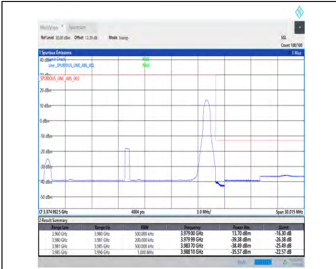
1-N77-3700-3980-30-20-H-2-DFT-PI2BPSK-Edge_1R_B_Right-1@50-Ant3-1--PASS-see graph
