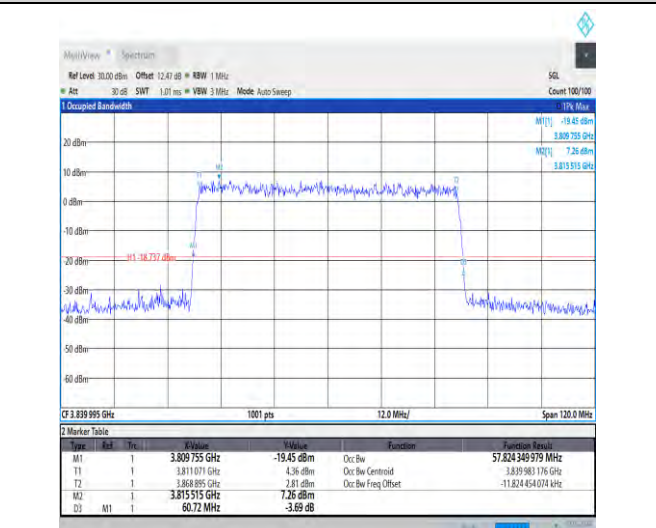
1-N77-3700-3980-30-60-M-7-CP-16QAM-Outer_Full-162@0-Ant3-57.824-60.720-≤60-PASS
