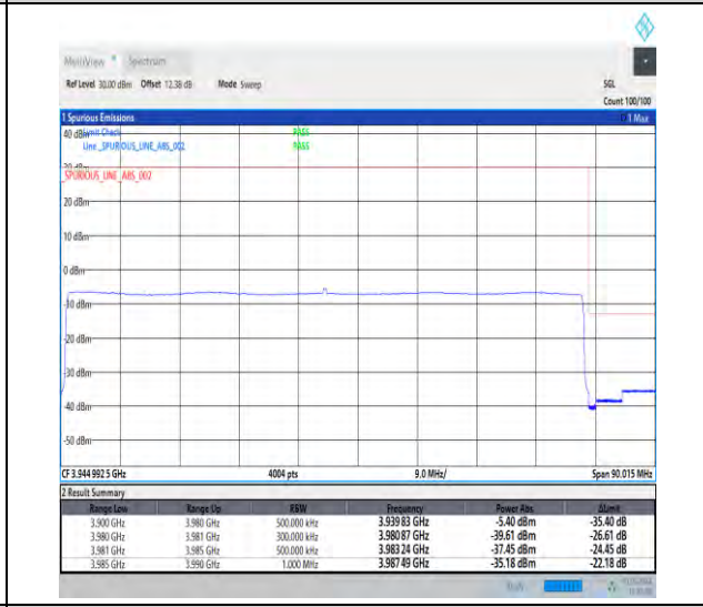
1-N77-3700-3980-30-80-H-6-CP-QPSK-Outer_Full-217@0-Ant3-1--PASS-see graph
