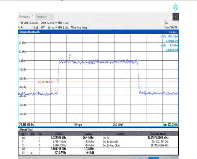
1-N77-3700-3980-30-100-M-9-CP-256QAM-Outer_F ull-273@0-Ant3-97.216-101.000≤100-PASS
