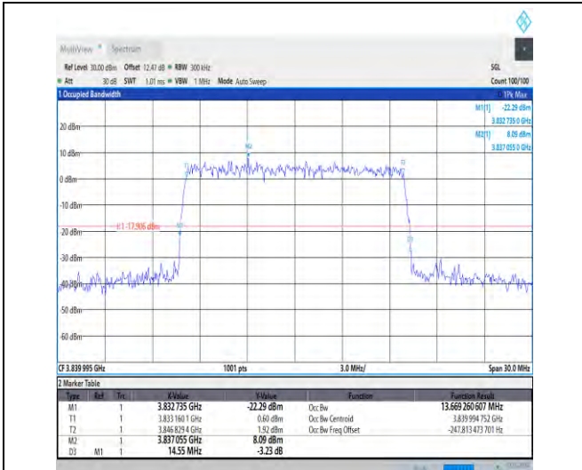
1-N77-3700-3980-30-15-M-8-CP-64QAM-Outer_Full -38@0-Ant3-13.669-14.550-≤15-PASS
