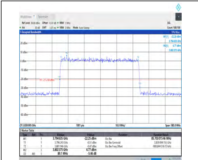
1-N77-3700-3980-30-90-M-5-DFT-256QAM-Outer_Full-240@0-Ant3-85.703-89.100-≤90-PASS
