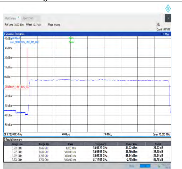
1-N77-3700-3980-30-60-L-3-DFT-PI2BPSK-Outer_Full-162@0-Ant3-1--PASS-see graph
