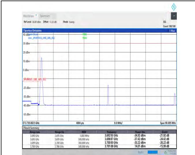
1-N77-3700-3980-30-80-L-1-DFT-PI2BPSK-Edge_1RB_Left-1@0-Ant3-1--PASS-see graph
