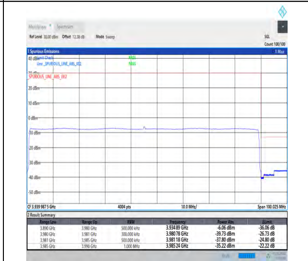
1-N77-3700-3980-30-90-H-6-CP-QPSK-Outer_Full-245@0-Ant3-1--PASS-see graph
