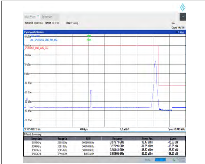
1-N77-3700-3980-30-50-H-2-DFT-PI2BPSK-Edge_1R B_Right-1@132-Ant3-1--PASS-see graph
