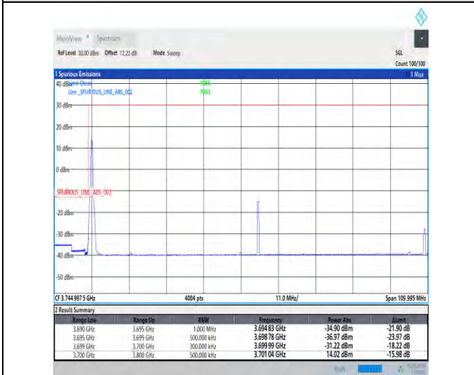
1-N77-3700-3980-30-100-L-4-CP-QPSK-Edge_1RB_Left-1@0-Ant3-1--PASS-see graph
