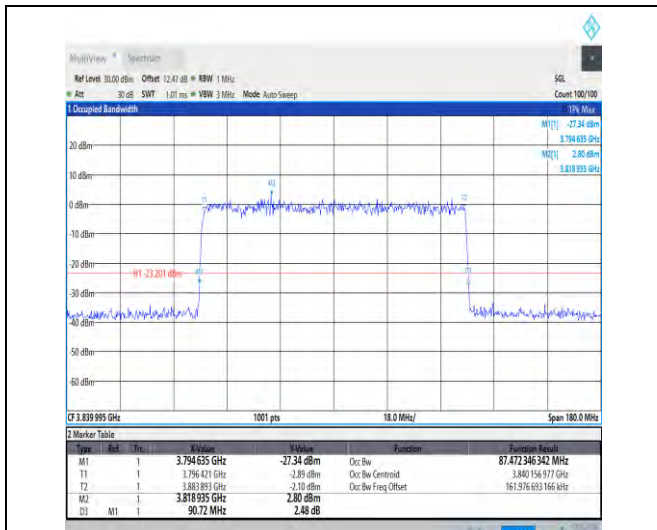
1-N77-3700-3980-30-90-M-9-CP-256QAM-Outer_Fu II-245@0-Ant3-87.472-90.720-≤90-PASS
