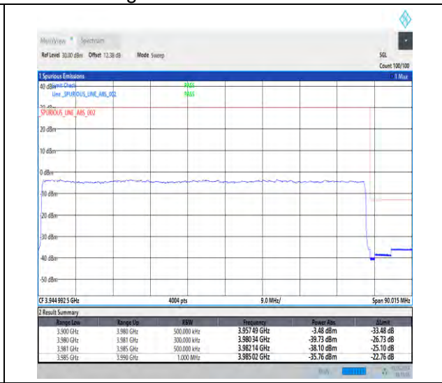
1-N77-3700-3980-30-80-H-3-DFT-PI2BPSK-Outer_Full-216@0-Ant3-1--PASS-see graph
