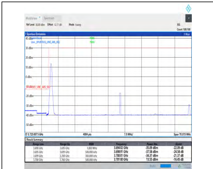
1-N77-3700-3980-30-60-L-1-DFT-PI2BPSK-Edge_1RB_Left-1@0-Ant3-1--PASS-see graph
