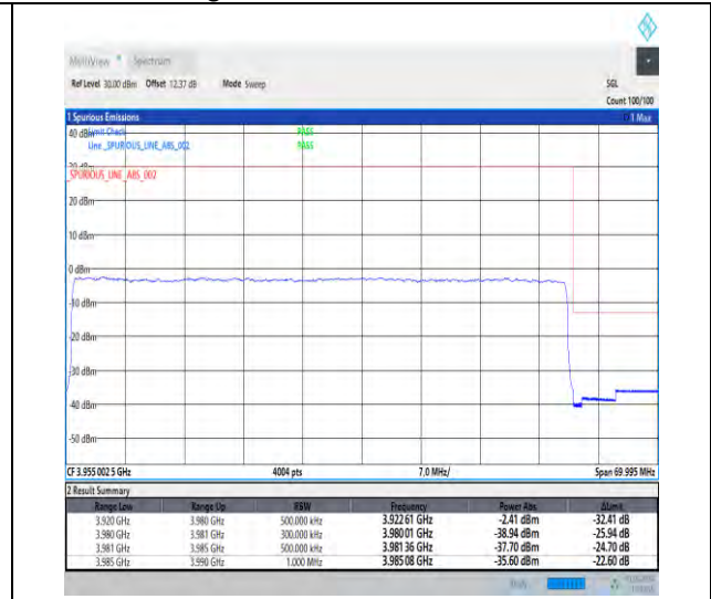
1-N77-3700-3980-30-60-H-3-DFT-PI2BPSK-Outer_Full-162@0-Ant3-1--PASS-see graph
