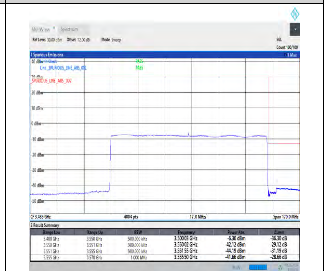
1-N77-3450-3550-30-100-H-6-CP-QPSK-Outer_Full-273@0-Ant3-1--PASS-see graph
