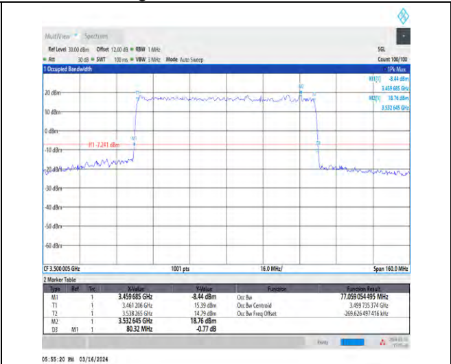
1-N77-3450-3550-30-80-M-3-DFT-16QAM-Outer_Full-216@0-Ant3-77.059-80.320-≤80-PASS
