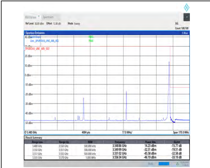
1-N77-3450-3550-30-90-H-2-DFT-PI2BPSK-Edge_1R_B_Right-1@244-Ant3-1--PASS-see graph
