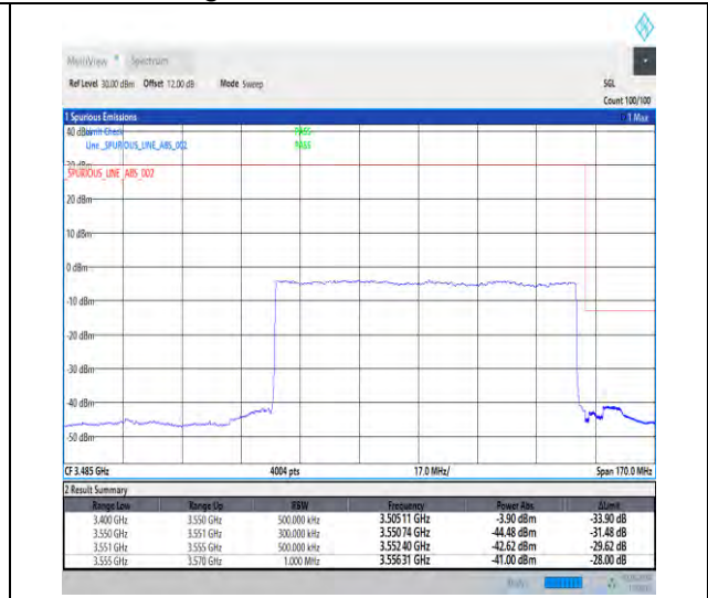
1-N77-3450-3550-30-90-H-3-DFT-PI2BPSK-Outer_Full-240@0-Ant3-1--PASS-see graph
