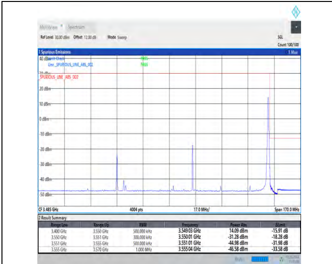
1-N77-3450-3550-30-100-H-2-DFT-PI2BPSK-Edge_1R_B_Right-1@272-Ant3-1--PASS-see graph
