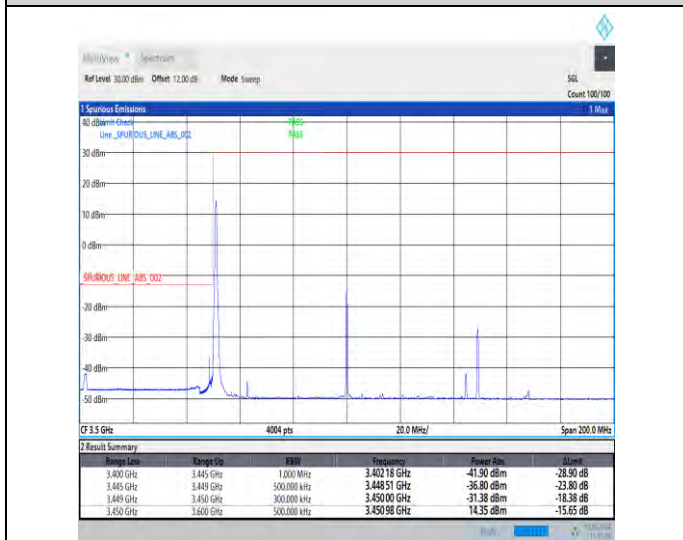
1-N77-3450-3550-30-100-L-4-CP-QPSK-Edge_1RB_Left-1@0-Ant3-1--PASS-see graph
