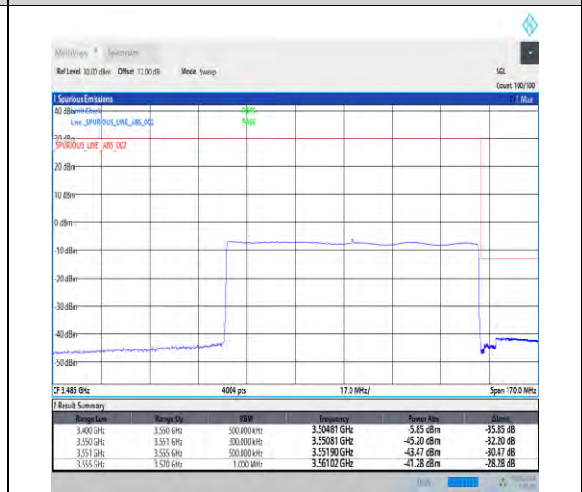
1-N77-3450-3550-30-90-H-6-CP-QPSK-Outer_Full-245@0-Ant3-1--PASS-see graph
