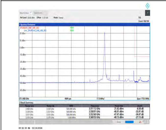
1-N77-3450-3550-30-40-H-5-CP-QPSK-Edge_1RB_Right-1@105-Ant3-1--PASS-see graph
