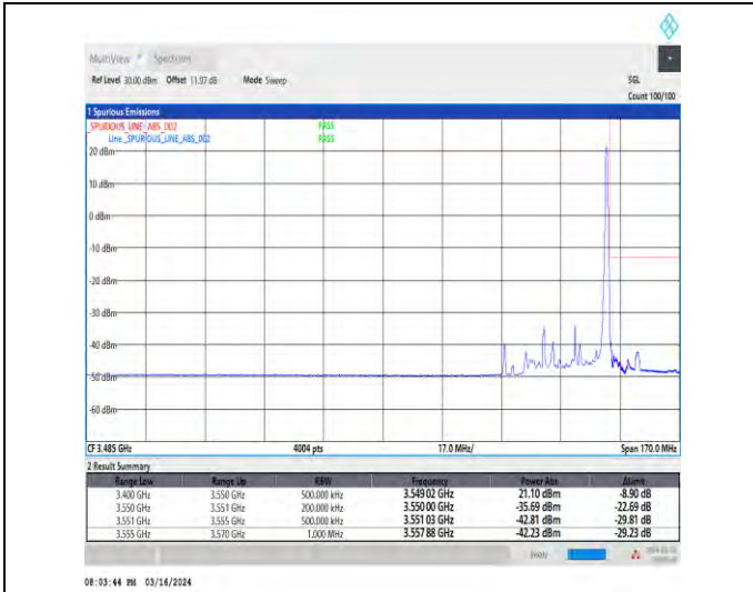
1-N77-3450-3550-30-20-H-2-DFT-PI2BPSK-Edge_1R_B_Right-1@50-Ant3-1--PASS-see graph
