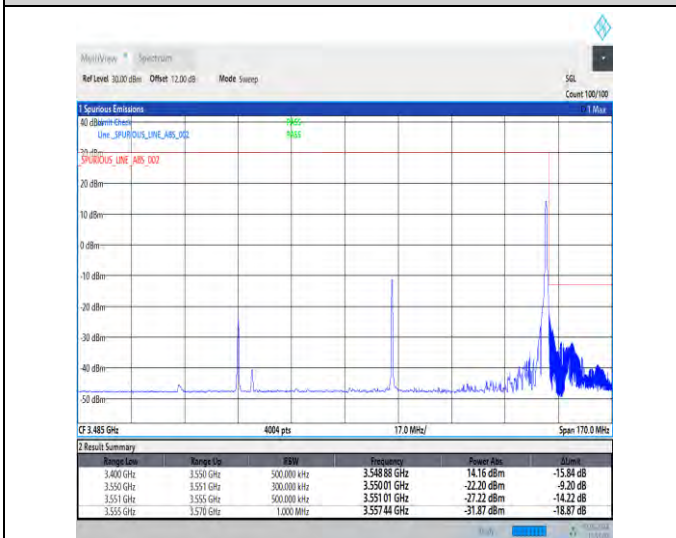
1-N77-3450-3550-30-100-H-5-CP-QPSK-Edge_1RB_Right-1@272-Ant3-1--PASS-see graph
