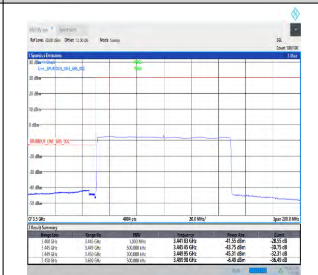
1-N77-3450-3550-30-100-L-6-CP-QPSK-Outer_Full-273@0-Ant3-1--PASS-see graph
