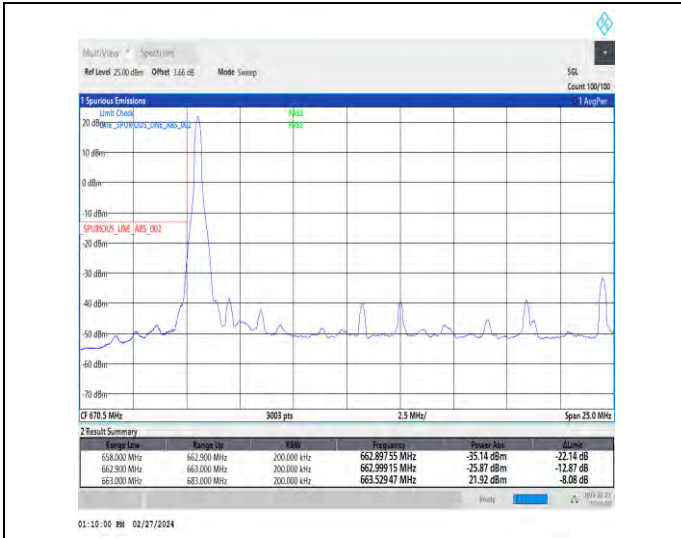
1-N71-15-20-L-1-DFT-PI2BPSK-Edge_1RB_Left-1@0-Ant1-1--PASS-see graph
