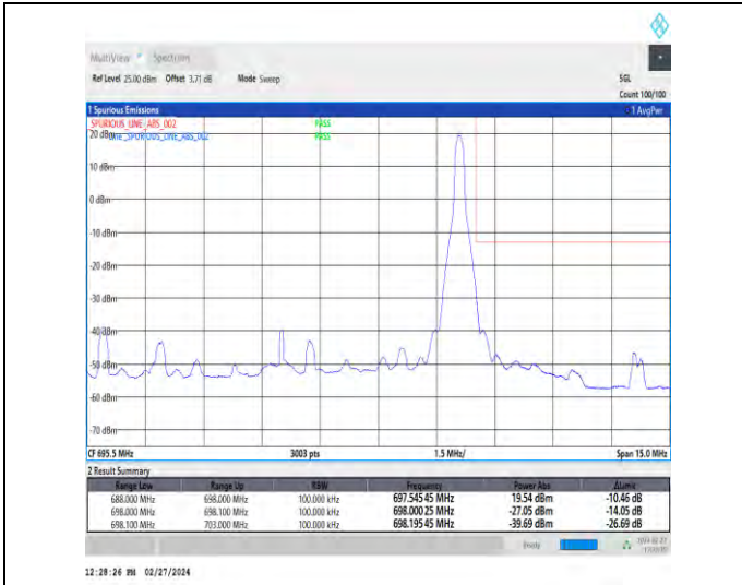
1-N71-15-10-H-2-DFT-PI2BPSK-Edge_1RB_Right-1@51-Ant1-1--PASS-see graph
