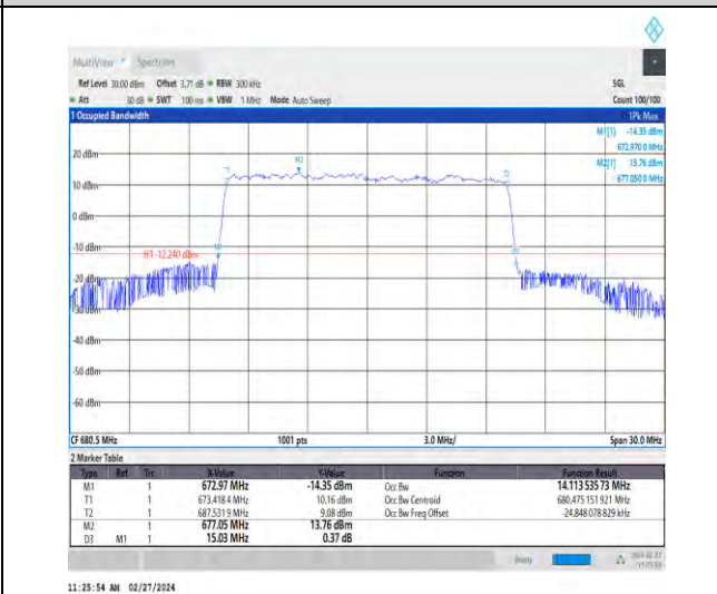
1-N71-15-15-M-6-CP-QPSK-Outer_Full-79@0-Ant1 14.114-15.030-≤15-PASS
