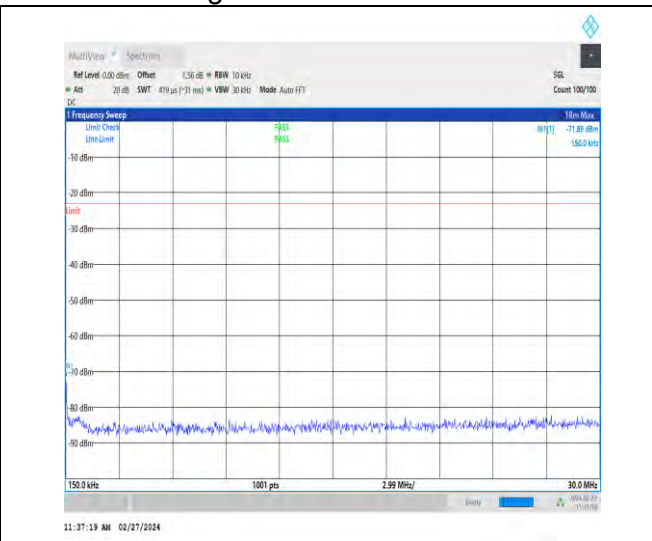
1-N71-15-20-H-1-DFT-PI2BPSK-Inner_1RB_Left-1 @ 1-0.15-30-Ant1-0.15--71.89--23-PASS
