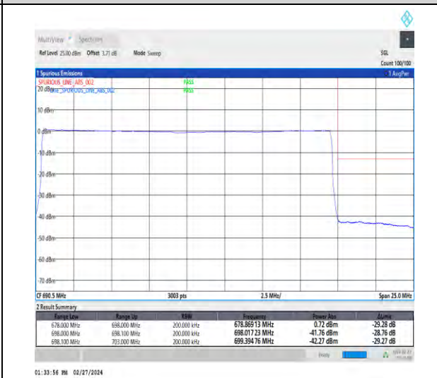
1-N71-15-20-H-6-CP-QPSK-Outer_Full-106@0-Ant1-1--PASS-see graph
