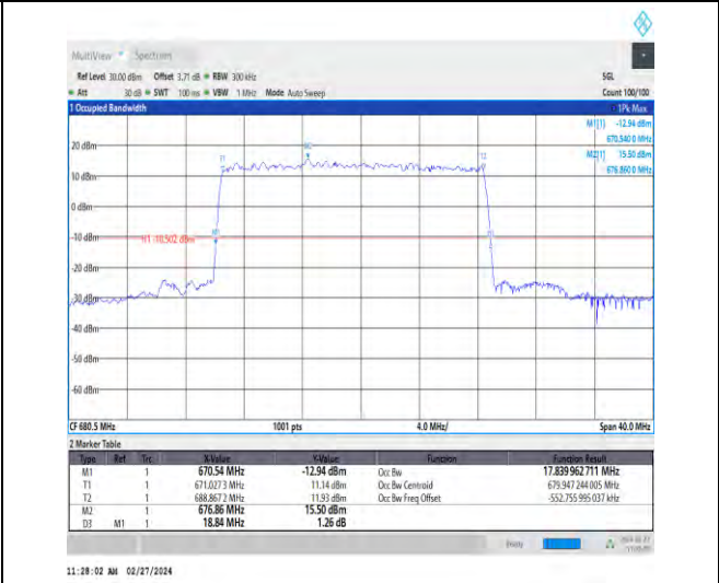
1-N71-15-20-M-1-DFT-QPSK-Outer_Full-100@0-Ant 1-17.84-18.840-≤20-PASS
