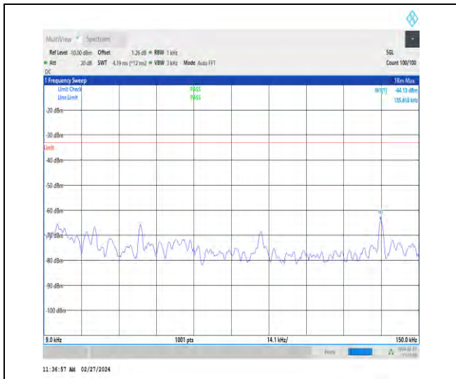
1-N71-15-20-H-1-DFT-PI2BPSK-Inner_1RB_Left-1 @ 1-0.009-0.15-Ant1-0.14--64.13--33-PASS
