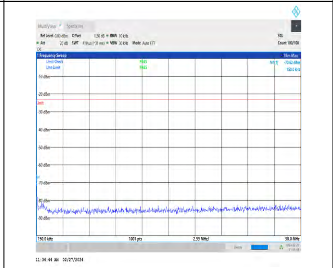
1-N71-15-20-M-1-DFT-PI2BPSK-Inner_1RB_Left-1 @ 1-0.15-30-Ant1-0.15--70.62--23-PASS
