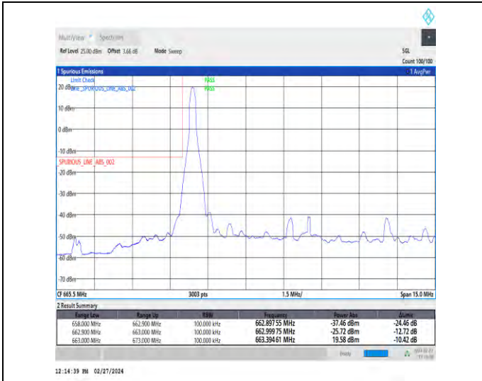
1-N71-15-10-L-1-DFT-PI2BPSK-Edge_1RB_Left-1@0-Ant1-1--PASS-see graph
