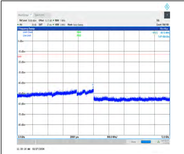
1-N71-15-20-L-1-DFT-PI2BPSK-Inner_1RB_Left-1 @ 1-3000-12000-Ant1-7471.65--45.12--13-PASS
