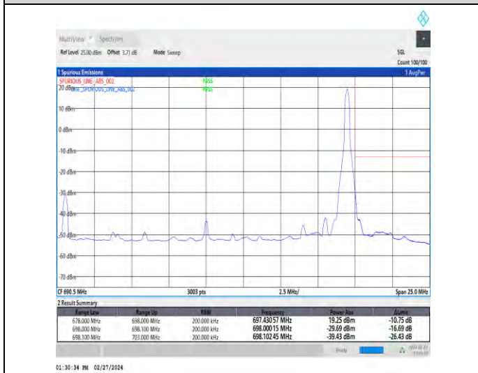
1-N71-15-20-H-5-CP-QPSK-Edge_1RB_Right-1@105-Ant1-1--PASS-see graph
