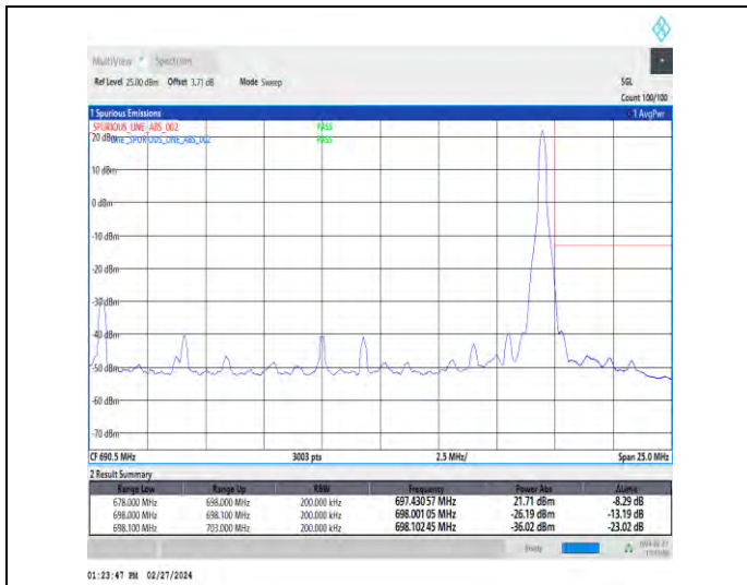
1-N71-15-20-H-2-DFT-PI2BPSK-Edge_1RB_Right-1@105-Ant1-1--PASS-see graph
