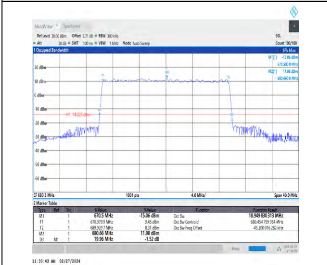
1-N71-15-20-M-8-CP-64QAM-Outer_Full-106@0-Ant1 1-18.95-19.960-≤20-PASS
