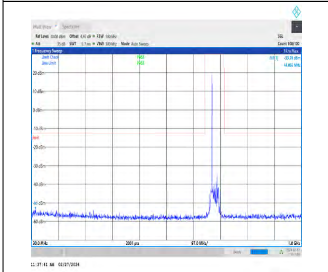
1-N71-15-20-H-1-DFT-PI2BPSK-Inner_1RB_Left-1 @ 1-30-1000-Ant1-44.07--53.78--13-PASS
