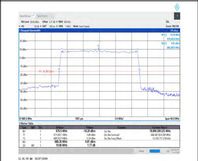
1-N71-15-20-M-9-CP-256QAM-Outer_Full-106@0-Ant1 -18.89-19.960-≤20-PASS
