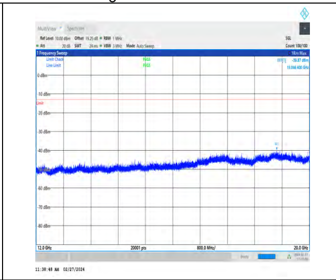
1-N71-15-20-H-1-DFT-PI2BPSK-Inner_1RB_Left-1@ 1-12000-20000-Ant1-19046.40--39.87--13-PASS
