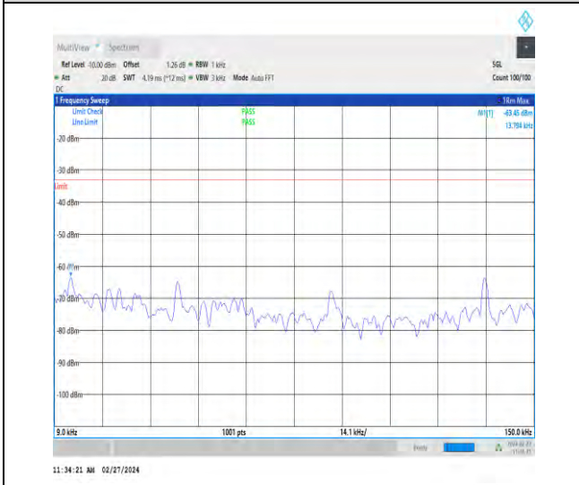
1-N71-15-20-M-1-DFT-PI2BPSK-Inner_1RB_Left-1 @ 1-0.009-0.15-Ant1-0.01--63.45--33-PASS
