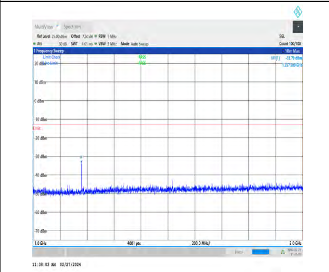
1-N71-15-20-H-1-DFT-PI2BPSK-Inner_1RB_Left-1 @ 1-1000-3000-Ant1-1357.50--33.79--13-PASS
