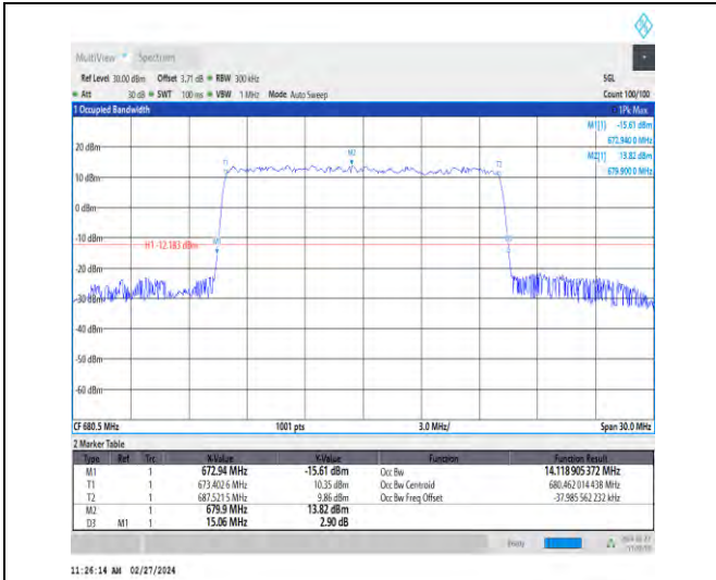
1-N71-15-15-M-7-CP-16QAM-Outer_Full-79@0-Ant1 -14.119-15.060-≤15-PASS
