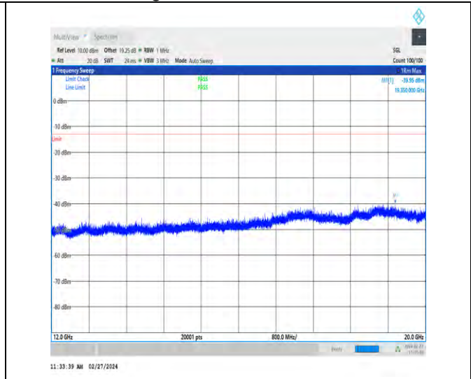
1-N71-15-20-L-1-DFT-PI2BPSK-Inner_1RB_Left-1 @ 1-12000-20000-Ant1-19350.00--39.95--13-PASS
