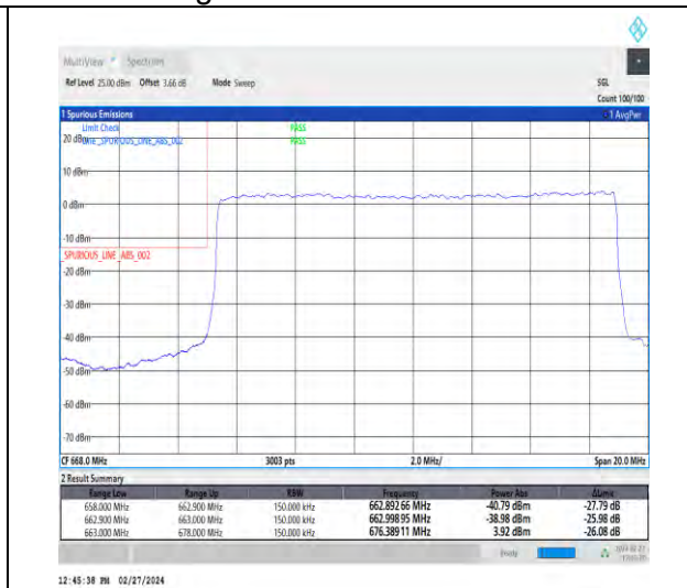
1-N71-15-15-L-3-DFT-PI2BPSK-Outer_Full-75@0-Ant1-1--PASS-see graph
