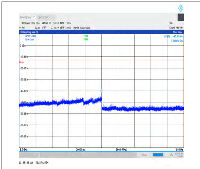
1-N71-15-20-H-1-DFT-PI2BPSK-Inner_1RB_Left-1 @1-3000-12000-Ant1-7485.60--43.43--13-PASS
