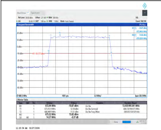
1-N71-15-15-M-1-DFT-QPSK-Outer_Full-75@0-Ant1 -13.436-14.370-≤15-PASS
