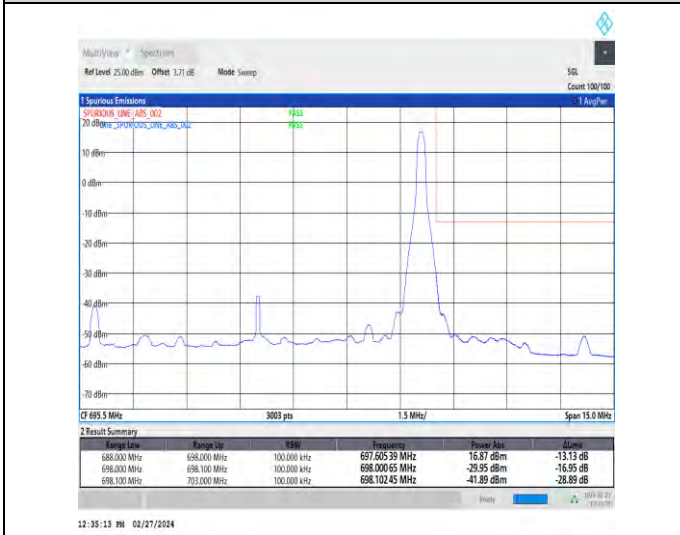
1-N71-15-10-H-5-CP-QPSK-Edge_1RB_Right-1@51-Ant1-1--PASS-see graph
