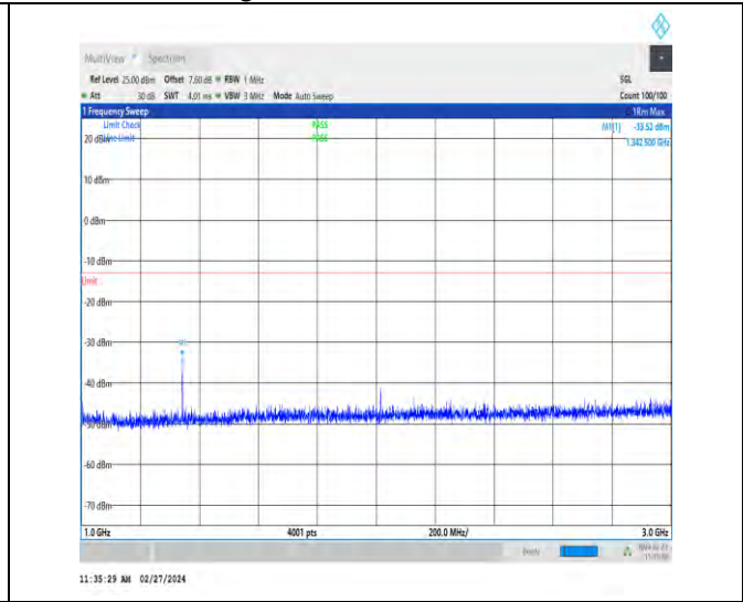
1-N71-15-20-M-1-DFT-PI2BPSK-Inner_1RB_Left-1@ 1-1000-3000-Ant1-1342.50--33.52--13-PASS
