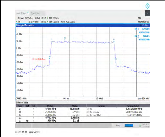
1-N71-15-10-M-7-CP-16QAM-Outer_Full-52@0-Ant 1-9.292-9.860-≤10-PASS
