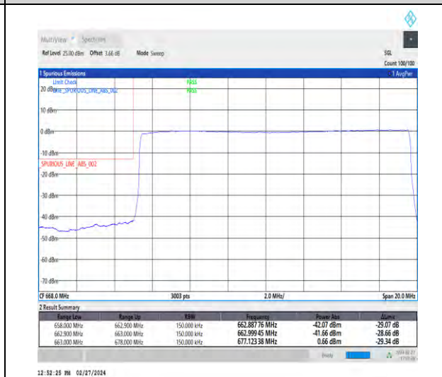
1-N71-15-15-L-6-CP-QPSK-Outer_Full-79@0-Ant1-1--PASS-see graph
