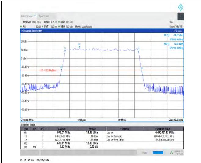
1-N71-15-5-M-5-DFT-256QAM-Outer_Full-25@0-Ant 1-4.495-4.920-≤5-PASS
