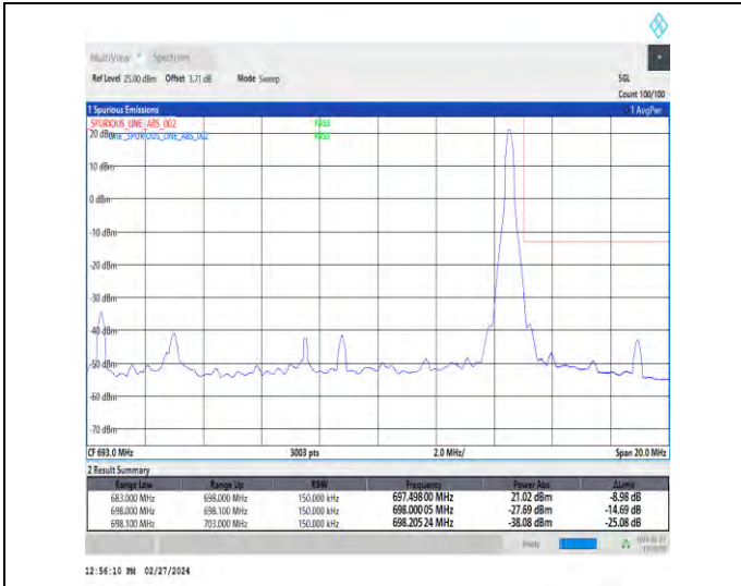
1-N71-15-15-H-2-DFT-PI2BPSK-Edge_1RB_Right-1@78-Ant1-1--PASS-see graph
