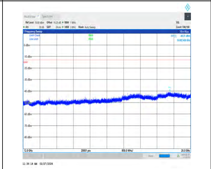
1-N71-15-20-M-1-DFT-PI2BPSK-Inner_1RB_Left-1@ 1-12000-20000-Ant1-19002.40--40.31--13-PASS
