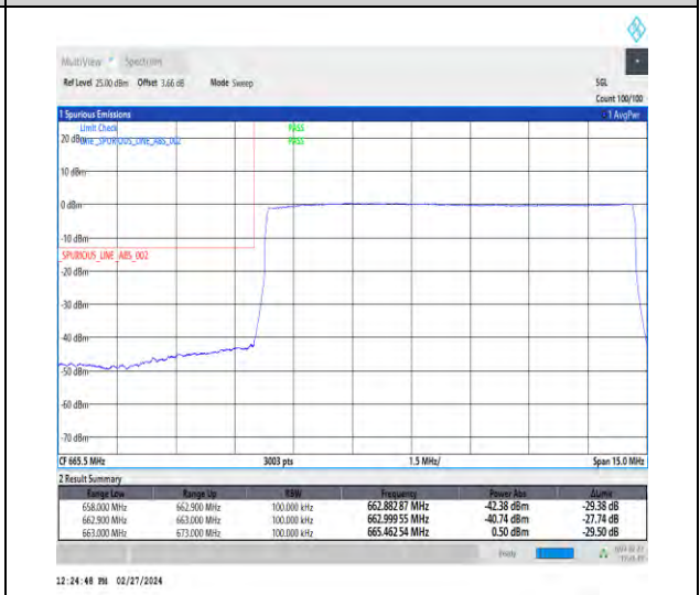
1-N71-15-10-L-6-CP-QPSK-Outer_Full-52@0-Ant1-1--PASS-see graph
