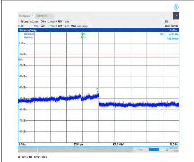
1-N71-15-20-M-1-DFT-PI2BPSK-Inner_1RB_Left-1 @1-3000-12000-Ant1-7438.35--44.91--13-PASS
