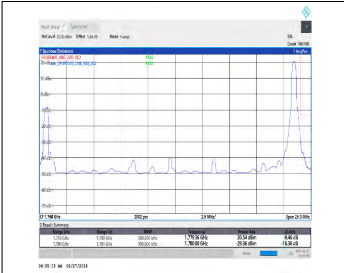
1-N66-15-25-H-2-DFT-PI2BPSK-Edge_1RB_Right-1@132-Ant4-1-seegraph-PASS-see graph
