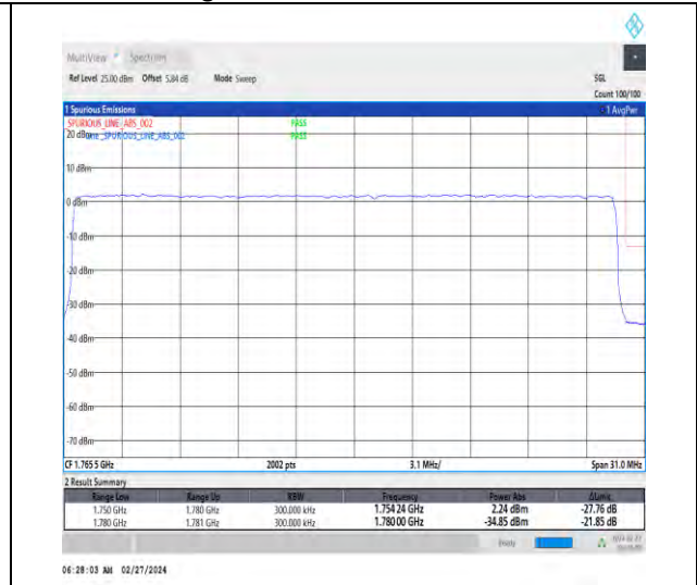
1-N66-15-30-H-3-DFT-PI2BPSK-Outer_Full-160@0-Ant4-1-seegraph-PASS-see graph
