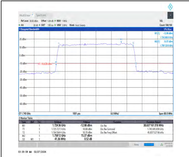
1-N66-15-40-M-3-DFT-16QAM-Outer_Full-216@0-A nt4-38.637-41.360-≤40-PASS
