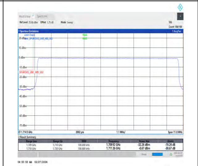
1-N66-15-10-L-6-CP-QPSK-Outer_Full-52@0-Ant4-1-seegraph-PASS-see graph
