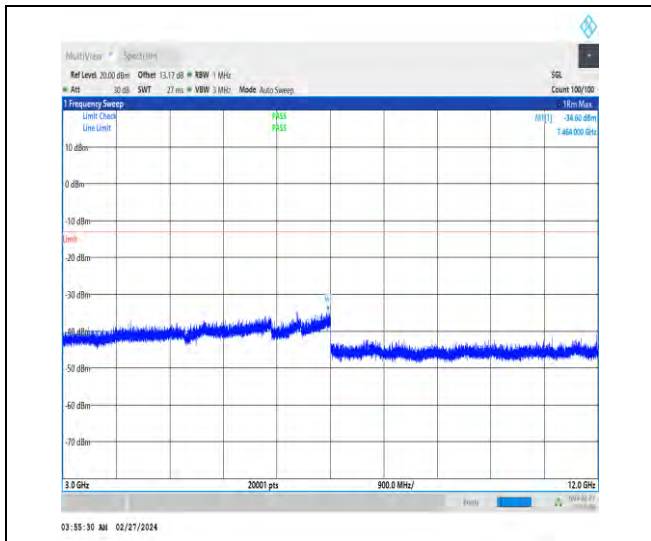
1-N66-15-40-H-1-DFT-PI2BPSK-Inner_1RB_Left-1 @1-3000-12000-Ant4-7464.00--34.60--13-PASS
