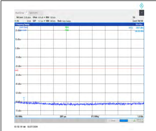
1-N66-15-40-M-1-DFT-PI2BPSK-Inner_1RB_Left-1 @1-30-1000-Ant4-100.33--59.01--23-PASS
