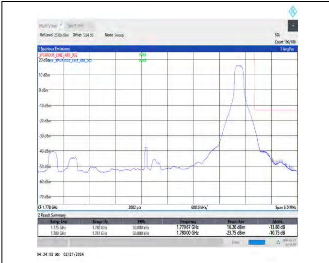
1-N66-15-5-H-2-DFT-PI2BPSK-Edge_1RB_Right-1@2 4-Ant4-1-seegraph-PASS-see graph
