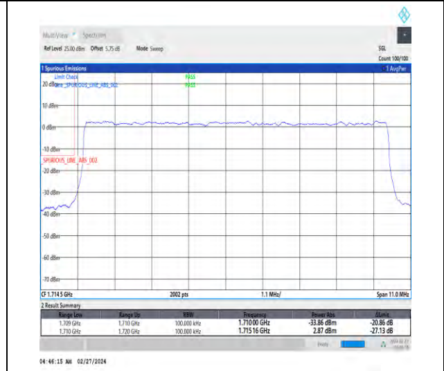
1-N66-15-10-L-3-DFT-PI2BPSK-Outer_Full-50@0-Ant4-1-seegraph-PASS-see graph
