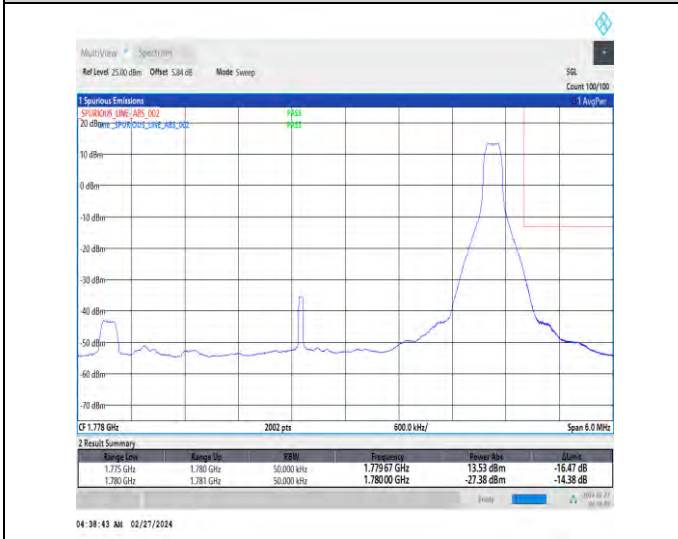
1-N66-15-5-H-5-CP-QPSK-Edge_1RB_Right-1@24-An t4-1-seegraph-PASS-see graph
