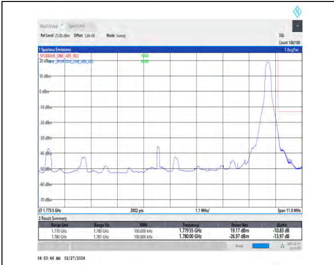
1-N66-15-10-H-2-DFT-PI2BPSK-Edge_1RB_Right-1@51-Ant4-1-seegraph-PASS-see graph
