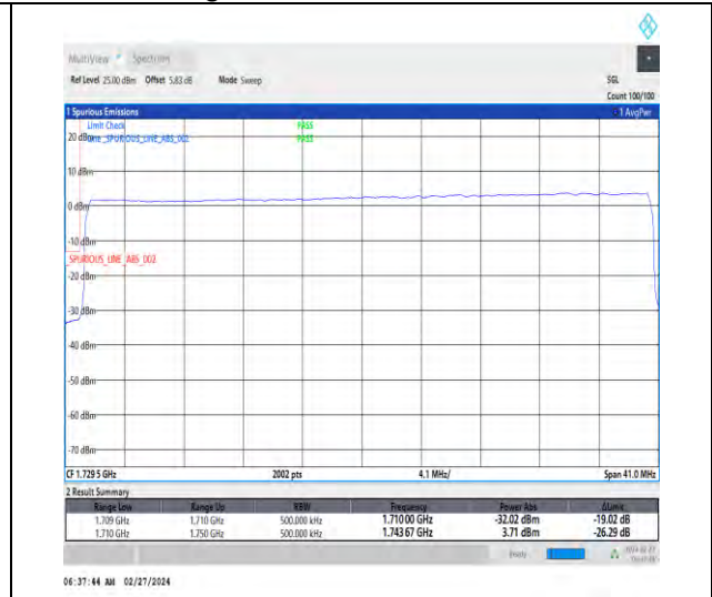
1-N66-15-40-L-3-DFT-PI2BPSK-Outer_Full-216@0-Ant4-1-seegraph-PASS-see graph
