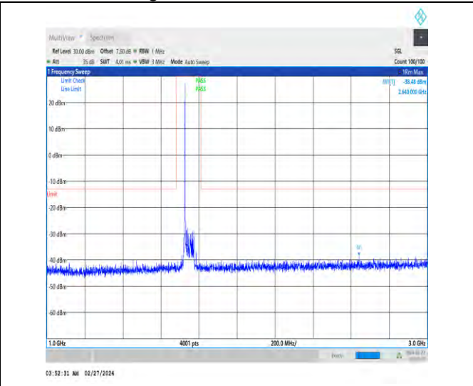
1-N66-15-40-M-1-DFT-PI2BPSK-Inner_1RB_Left-1@ 1-1000-3000-Ant4-2640.00--38.48--13-PASS
