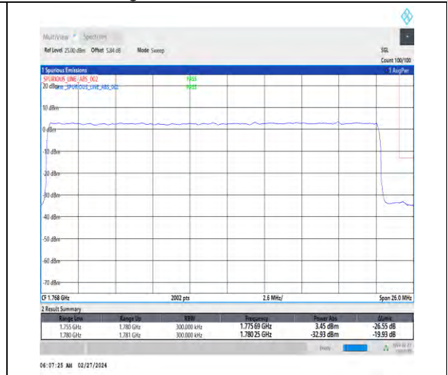
1-N66-15-25-H-3-DFT-PI2BPSK-Outer_Full-128@0-Ant4-1-seegraph-PASS-see graph
