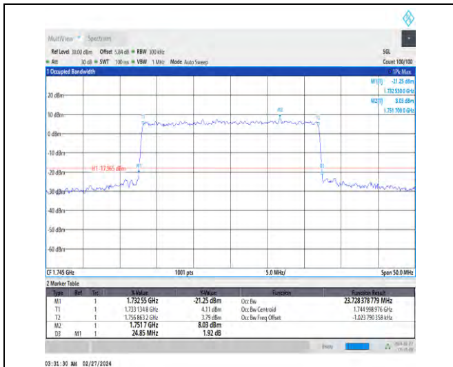
1-N66-15-25-M-9-CP-256QAM-Outer_Full-133@0-A nt4-23.728-24.850-≤25-PASS
