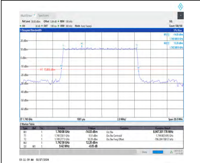
1-N66-15-10-M-2-DFT-PI2BPSK-Outer_Full-50@0-Ant4 8.947-9.420-≤10-PASS
