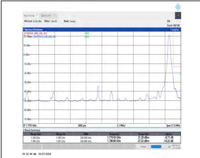
1-N66-15-20-H-2-DFT-PI2BPSK-Edge_1RB_Right-1@105-Ant4-1-seegraph-PASS-see graph
