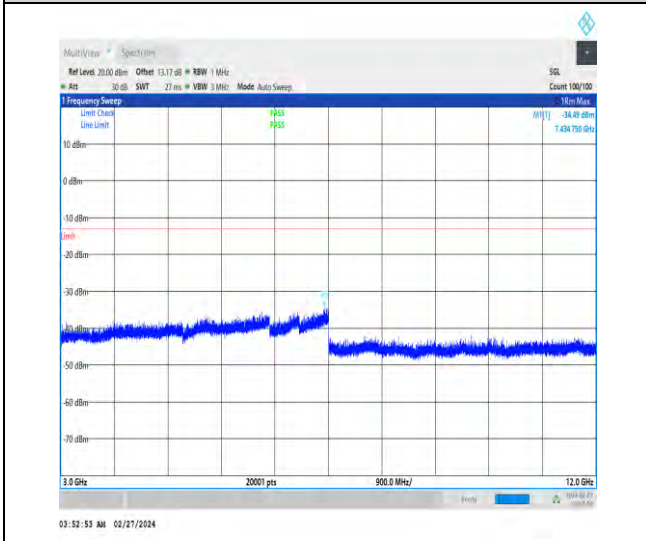
1-N66-15-40-M-1-DFT-PI2BPSK-Inner_1RB_Left-1 @1-3000-12000-Ant4-7434.75--34.49--13-PASS
