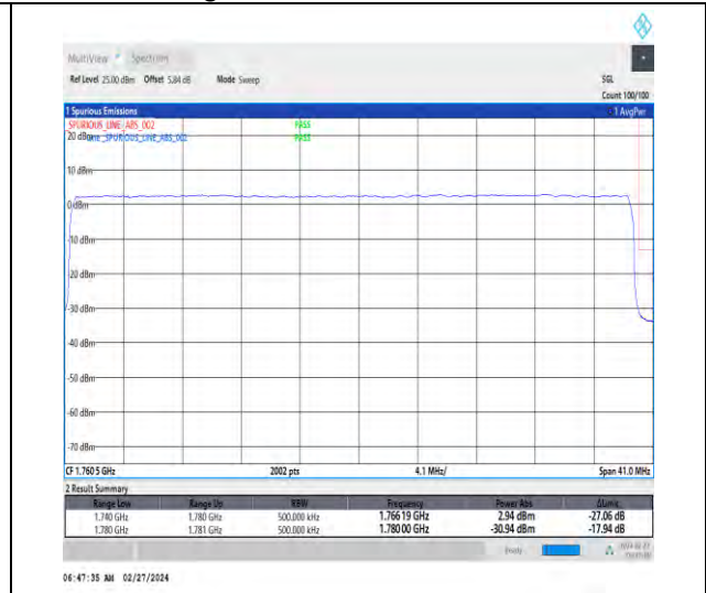
1-N66-15-40-H-3-DFT-PI2BPSK-Outer_Full-216@0-Ant4-1-seegraph-PASS-see graph
