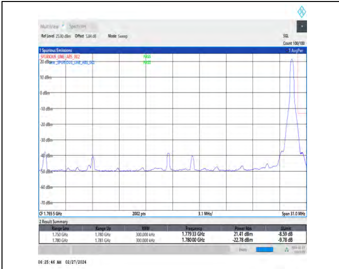
1-N66-15-30-H-2-DFT-PI2BPSK-Edge_1RB_Right-1@159-Ant4-1-seegraph-PASS-see graph
