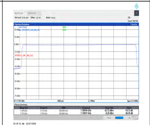
1-N66-15-20-L-6-CP-QPSK-Outer_Full-106@0-Ant4-1-seegraph-PASS-see graph
