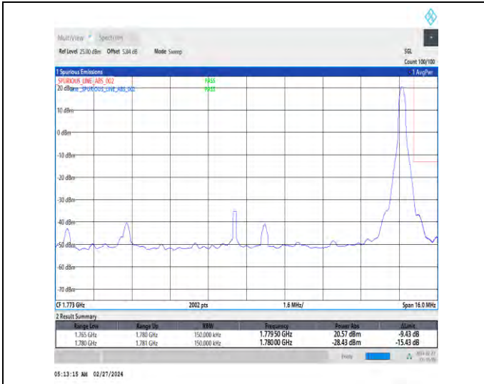
1-N66-15-15-H-2-DFT-PI2BPSK-Edge_1RB_Right-1@78-Ant4-1-seegraph-PASS-see graph
