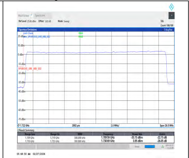
1-N66-15-25-L-3-DFT-PI2BPSK-Outer_Full-128@0-Ant4-1-seegraph-PASS-see graph
