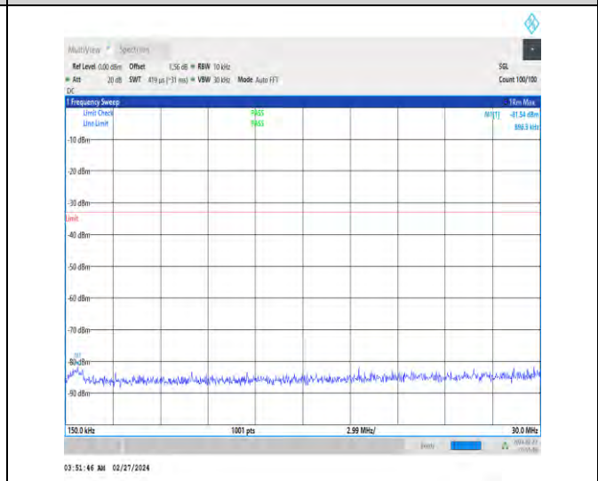
1-N66-15-40-M-1-DFT-PI2BPSK-Inner_1RB_Left-1@ 1-0.15-30-Ant4-0.90--81.54--33-PASS
