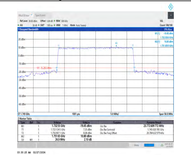
1-N66-15-25-M-6-CP-QPSK-Outer_Full-133@0-Ant4-23.773-24.900-≤25-PASS
