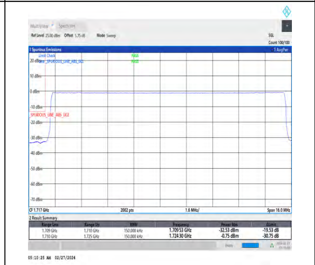
1-N66-15-15-L-6-CP-QPSK-Outer_Full-79@0-Ant4-1-seegraph-PASS-see graph
