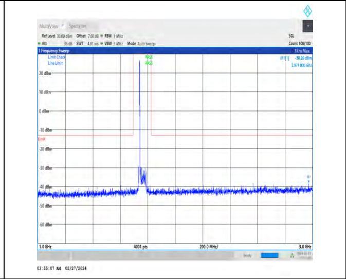
1-N66-15-40-H-1-DFT-PI2BPSK-Inner_1RB_Left-1 @ 1-1000-3000-Ant4-2971.00--38.20--13-PASS
