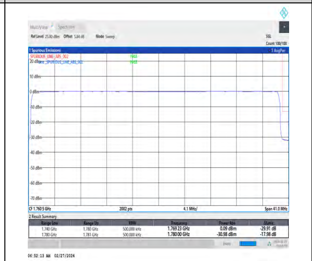
1-N66-15-40-H-6-CP-QPSK-Outer_Full-216@0-Ant4-1-seegraph-PASS-see graph
