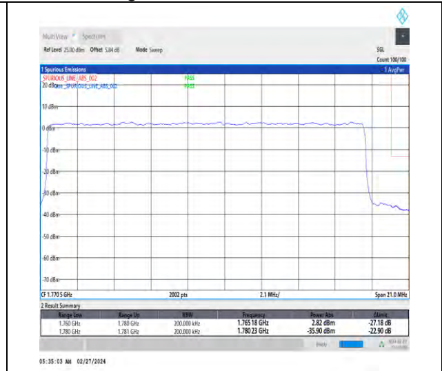
1-N66-15-20-H-3-DFT-PI2BPSK-Outer_Full-100@0-Ant4-1-seegraph-PASS-see graph
