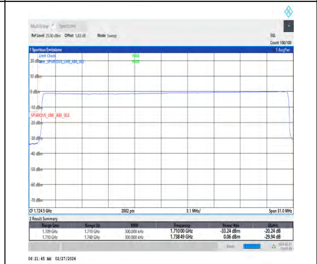
1-N66-15-30-L-6-CP-QPSK-Outer_Full-160@0-Ant4-1-seegraph-PASS-see graph
