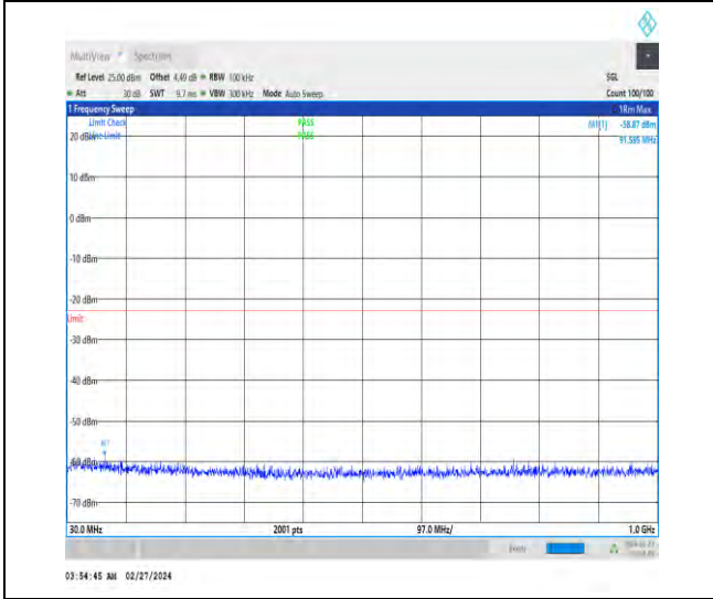
1-N66-15-40-H-1-DFT-PI2BPSK-Inner_1RB_Left-1 @ 1-30-1000-Ant4-91.60--58.87--23-PASS
