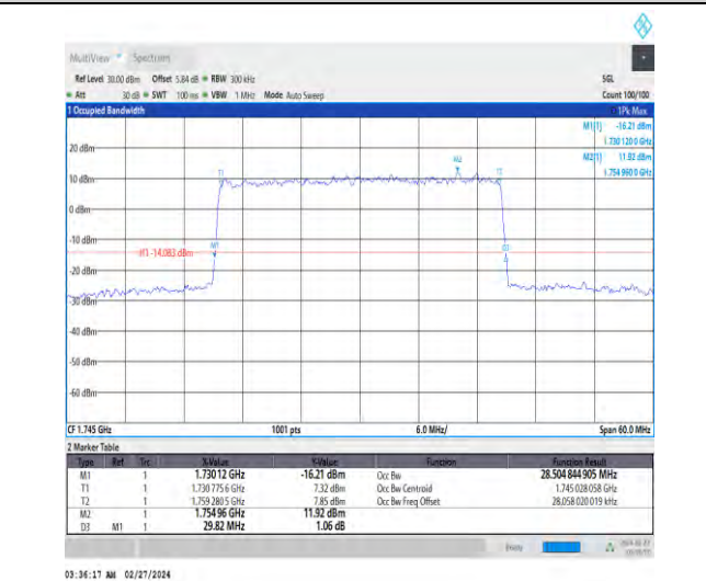
1-N66-15-30-M-3-DFT-16QAM-Outer_Full-160@0-A nt4-28.505-29.820-≤30-PASS
