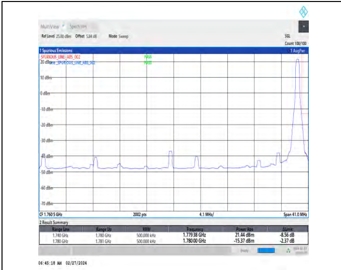
1-N66-15-40-H-2-DFT-PI2BPSK-Edge_1RB_Right-1@215-Ant4-1-seegraph-PASS-see graph
