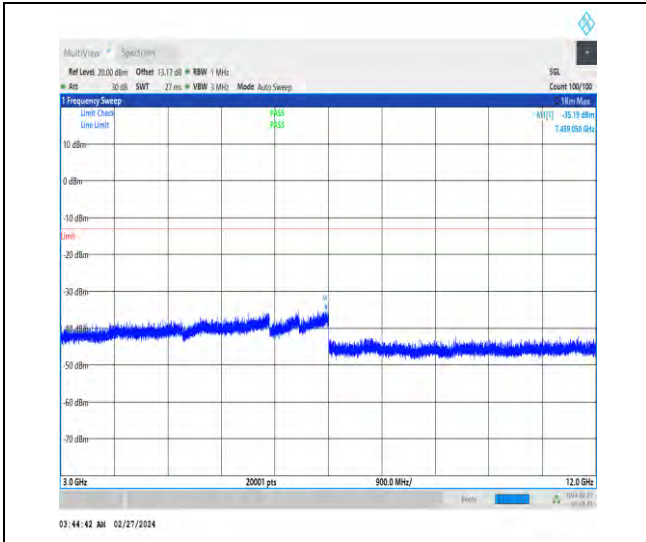
1-N66-15-40-L-1-DFT-PI2BPSK-Inner_1RB_Left-1 @1-3000-12000-Ant4-7459.05--35.19--13-PASS
