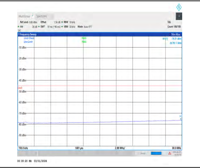
1-N41-30-100-M-1-DFT-PI2BPSK-Inner_1RB_Left-1 @1-0.15-30-Ant4-29.79--76.31--45-PASS
