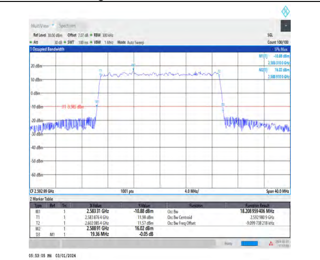
1-N41-30-20-M-8-CP-64QAM-Outer_Full-51@0-Ant4 -18.209-19.360-≤20-PASS
