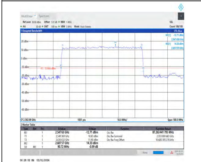
1-N41-30-90-M-8-CP-64QAM-Outer_Full-245@0-Ant4 t4-87.263-90.720-≤90-PASS
