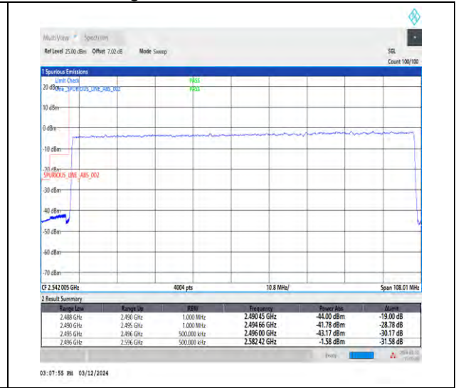
1-N41-30-100-L-3-DFT-PI2BPSK-Outer_Full-270@0-Ant4-1--PASS-see graph
