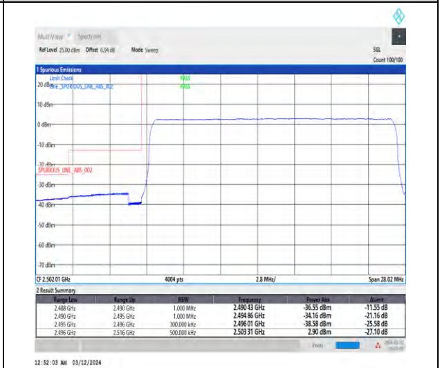
1-N41-30-20-L-6-CP-QPSK-Outer_Full-51@0-Ant4-1--PASS-see graph
