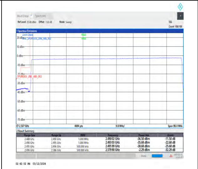
1-N41-30-90-L-6-CP-QPSK-Outer_Full-245@0-Ant4-1--PASS-see graph
