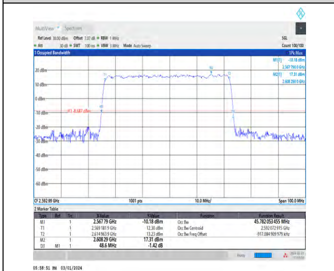
1-N41-30-50-M-3-DFT-16QAM-Outer_Full-128@0-Ant 4-45.782-48.600-≤50-PASS
