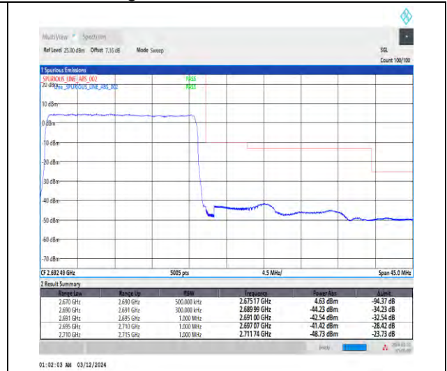
1-N41-30-20-H-3-DFT-PI2BPSK-Outer_Full-50@0-Ant4-1--PASS-see graph
