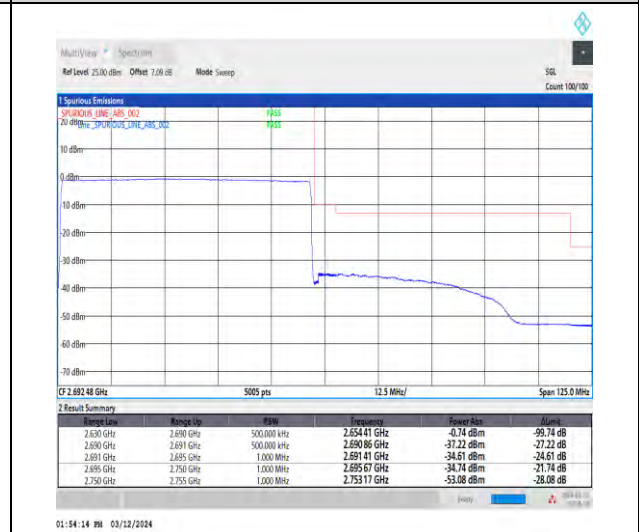
1-N41-30-60-H-6-CP-QPSK-Outer_Full-162@0-Ant4-1--PASS-see graph
