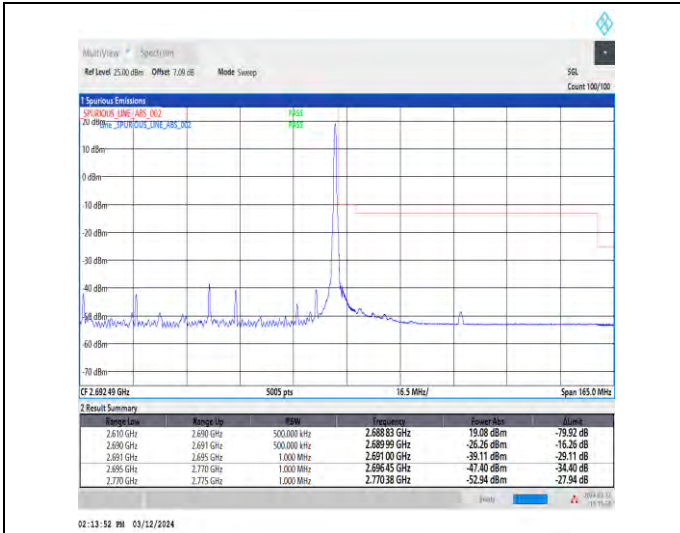
1-N41-30-80-H-2-DFT-PI2BPSK-Edge_1RB_Right-1@216-Ant4-1--PASS-see graph
