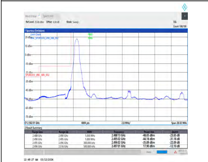
1-N41-30-20-L-4-CP-QPSK-Edge_1RB_Left-1@0-Ant4-1--PASS-see graph
