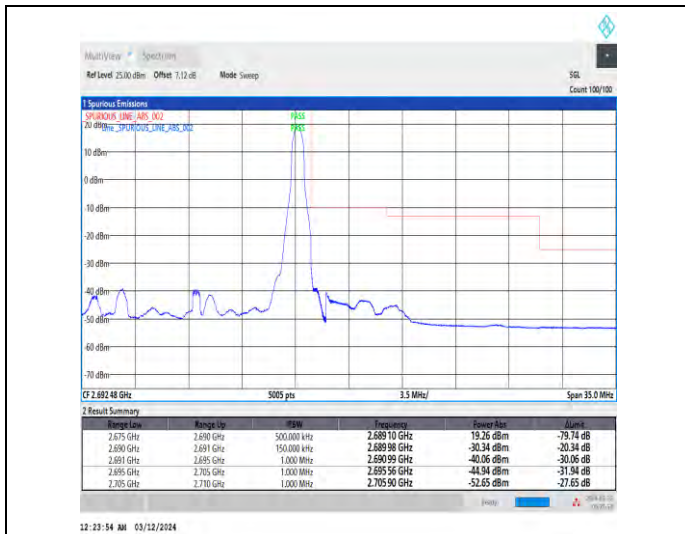
1-N41-30-15-H-2-DFT-PI2BPSK-Edge_1RB_Right-1@37-Ant4-1--PASS-see graph
