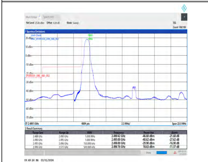
1-N41-30-15-L-4-CP-QPSK-Edge_1RB_Left-1@0-Ant4-1--PASS-see graph
