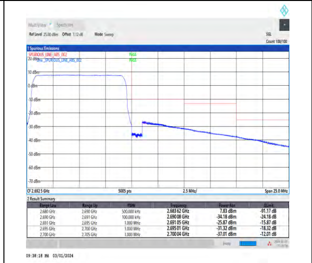
1-N41-30-10-H-6-CP-QPSK-Outer_Full-24@0-Ant4-1--PASS-see graph
