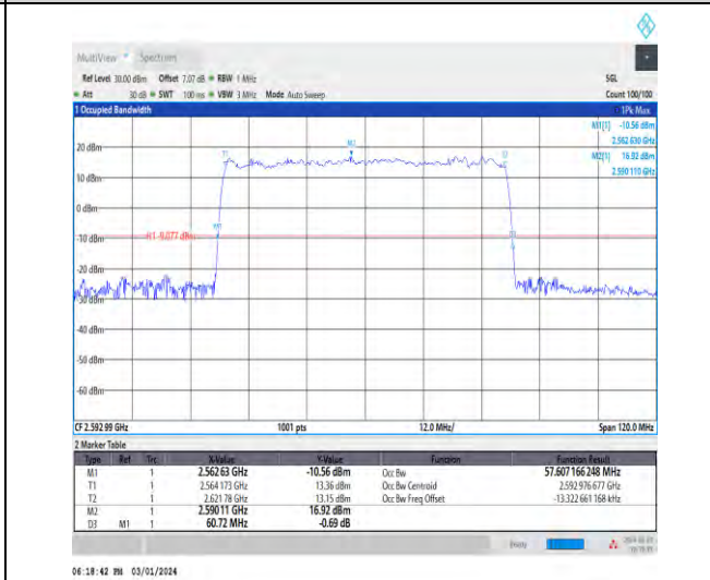
1-N41-30-60-M-3-DFT-16QAM-Outer_Full-162@0-A nt4-57.607-60.720-≤60-PASS
