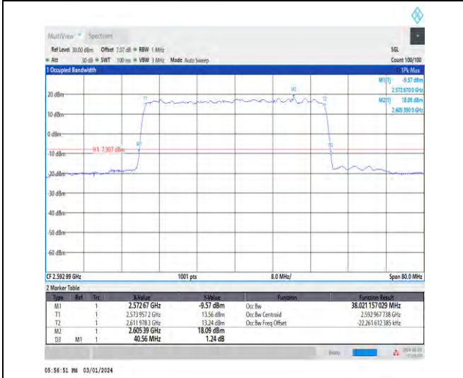
1-N41-30-40-M-8-CP-64QAM-Outer_Full-106@0-Ant4 t4-38.021-40.560-≤40-PASS
