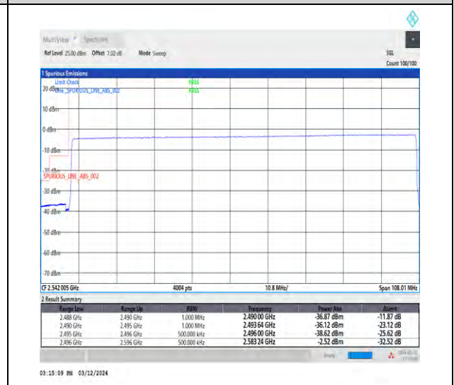
1-N41-30-100-L-6-CP-QPSK-Outer_Full-273@0-Ant4-1--PASS-see graph
