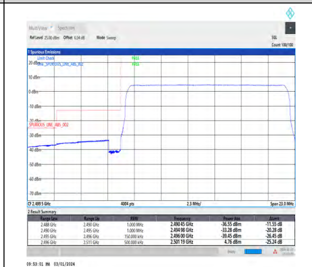
1-N41-30-15-L-6-CP-QPSK-Outer_Full-38@0-Ant4-1--PASS-see graph
