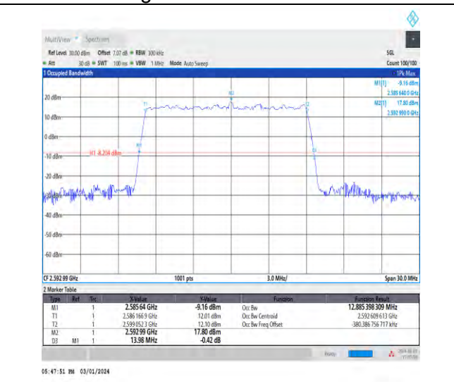
1-N41-30-15-M-5-DFT-256QAM-Outer_Full-36@0-A nt4-12.885-13.980-≤15-PASS
