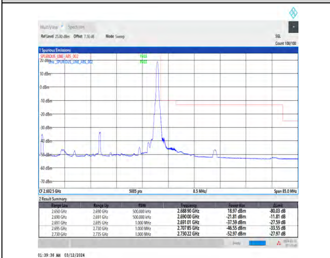
1-N41-30-40-H-5-CP-QPSK-Edge_1RB_Right-1@105-Ant4-1--PASS-see graph
