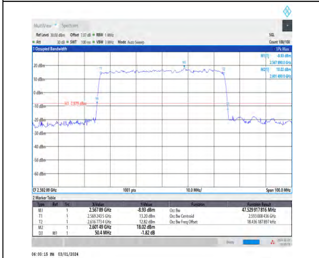
1-N41-30-50-M-7-CP-16QAM-Outer_Full-133@0-Ant4-47.53-50.400-≤50-PASS
