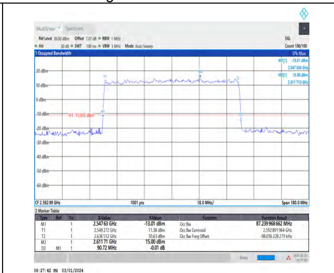
1-N41-30-90-M-7-CP-16QAM-Outer_Full-245@0-Ant4 4-87.24-90.720-≤90-PASS
