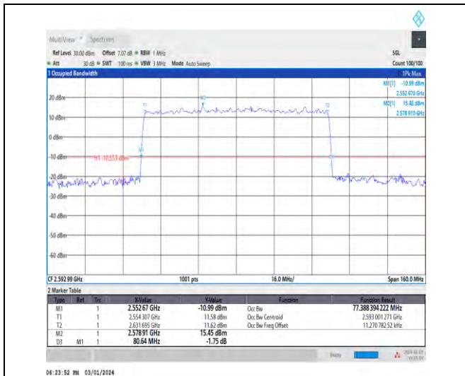
1-N41-30-80-M-7-CP-16QAM-Outer_Full-217@0-An t4-77.388-80.640-<=80-PASS
