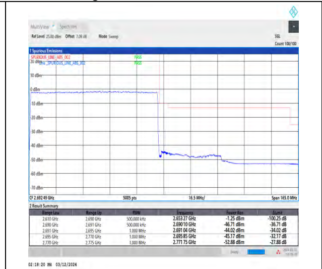
1-N41-30-80-H-3-DFT-PI2BPSK-Outer_Full-216@0-Ant4-1--PASS-see graph
