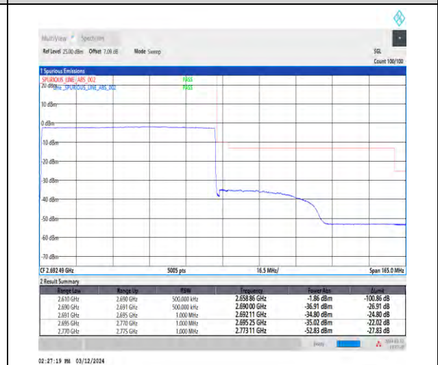
1-N41-30-80-H-6-CP-QPSK-Outer_Full-217@0-Ant4-1--PASS-see graph
