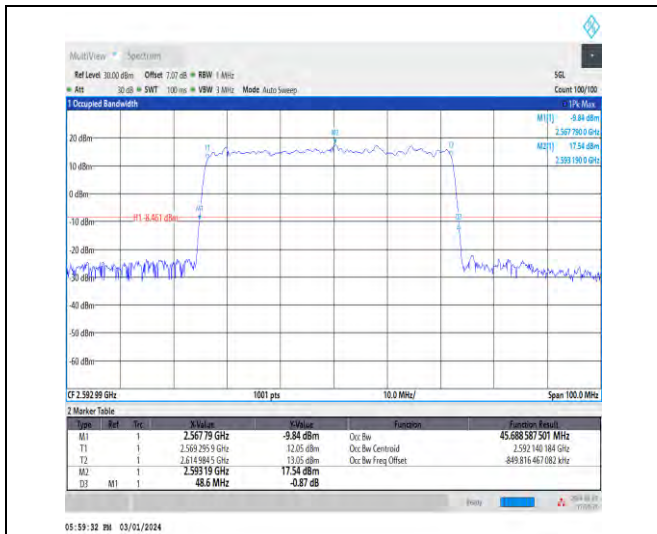
1-N41-30-50-M-5-DFT-256QAM-Outer_Full-128@0-Ant4-45.689-48.600-≤50-PASS
