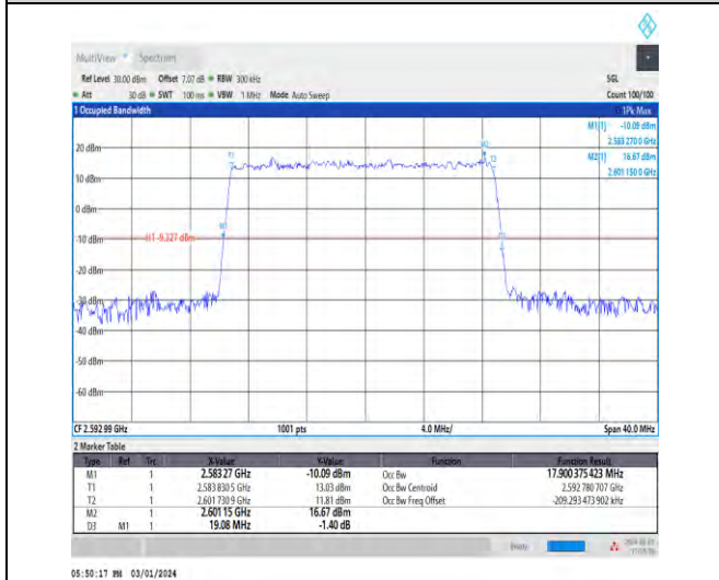
1-N41-30-20-M-1-DFT-QPSK-Outer_Full-50@0-Ant4 -17.9-19.080-≤20-PASS
