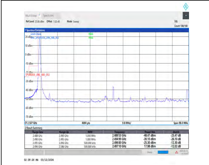
1-N41-30-90-L-4-CP-QPSK-Edge_1RB_Left-1@0-Ant4-1--PASS-see graph
