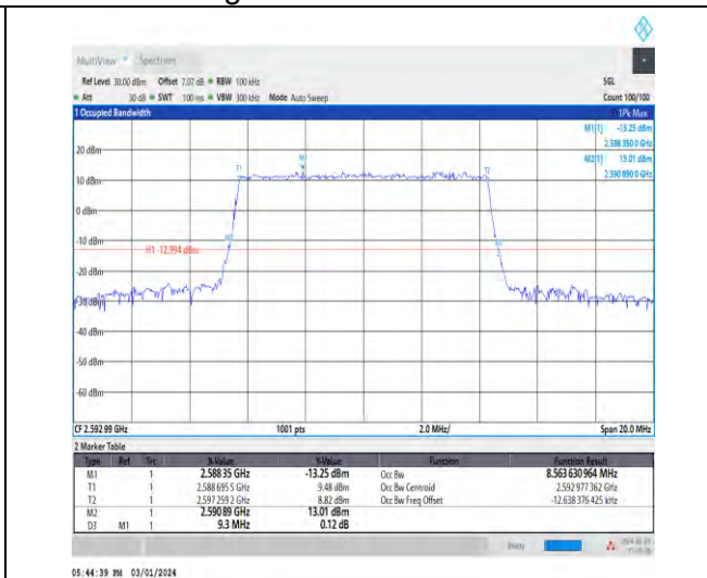
1-N41-30-10-M-6-CP-QPSK-Outer_Full-24@0-Ant4- 8.564-9.300-≤10-PASS
