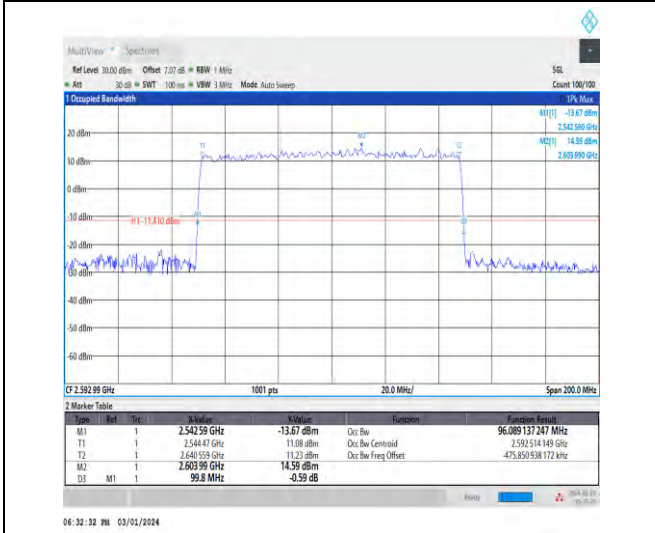
1-N41-30-100-M-3-DFT-16QAM-Outer_Full-270@0-A Ant4-96.089-99.800-≤100-PASS
