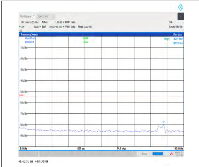
1-N41-30-100-H-1-DFT-PI2BPSK-Inner_1RB_Left-1 @1-0.009-0.15-Ant4-0.13--80.97--55-PASS
