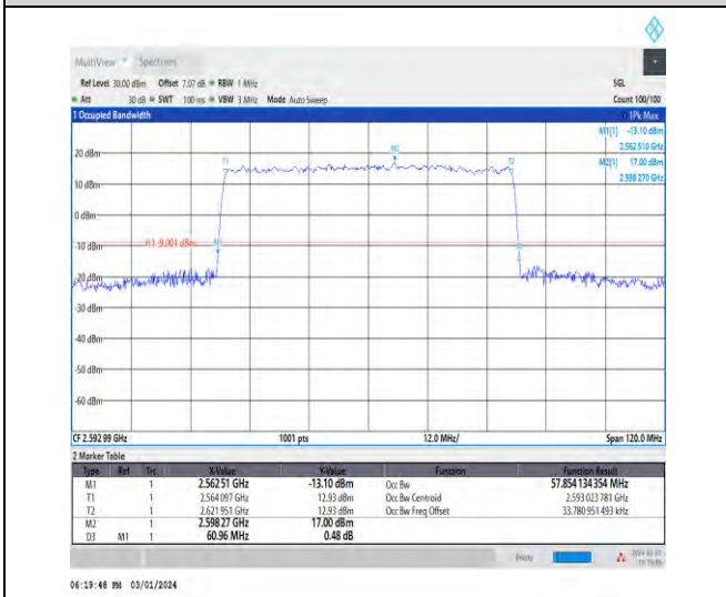
1-N41-30-60-M-6-CP-QPSK-Outer_Full-162@0-Ant4 -57.854-60.960-≤60-PASS
