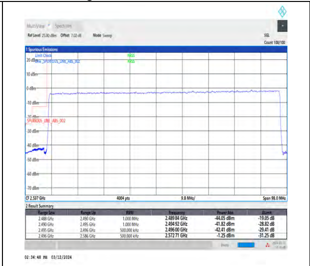
1-N41-30-90-L-3-DFT-PI2BPSK-Outer_Full-240@0-Ant4-1--PASS-see graph
