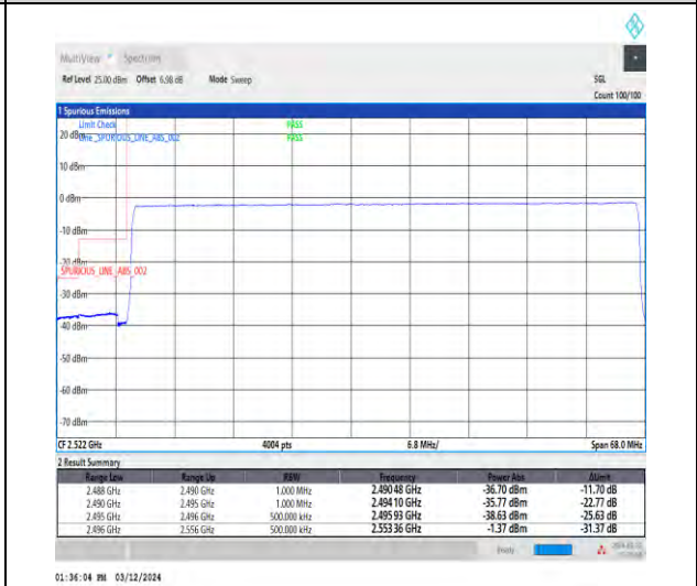
1-N41-30-60-L-6-CP-QPSK-Outer_Full-162@0-Ant4-1--PASS-see graph
