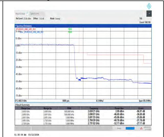
1-N41-30-40-H-3-DFT-PI2BPSK-Outer_Full-100@0-Ant4-1--PASS-see graph
