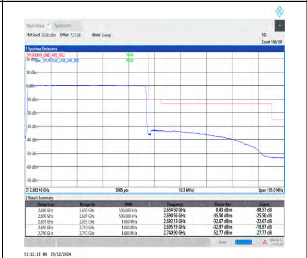
1-N41-30-50-H-6-CP-QPSK-Outer_Full-133@0-Ant4-1--PASS-see graph
