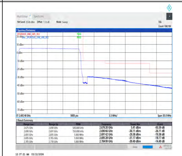
1-N41-30-15-H-6-CP-QPSK-Outer_Full-38@0-Ant4-1--PASS-see graph
