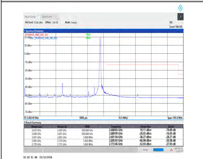
1-N41-30-80-H-5-CP-QPSK-Edge_1RB_Right-1@216-Ant4-1--PASS-see graph
