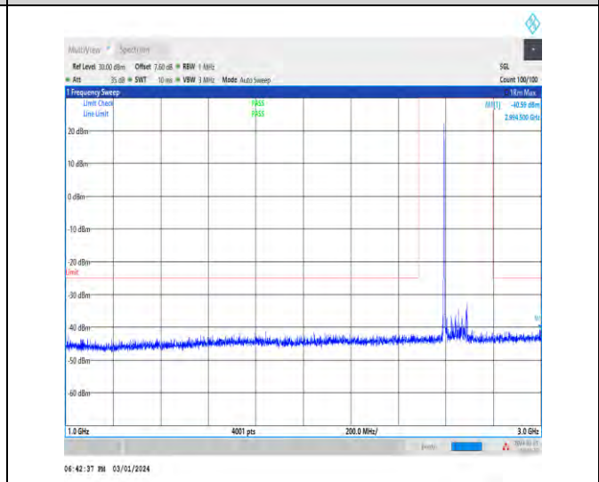
1-N41-30-100-H-1-DFT-PI2BPSK-Inner_1RB_Left-1 @1-1000-3000-Ant4-2994.50--40.59--25-PASS
