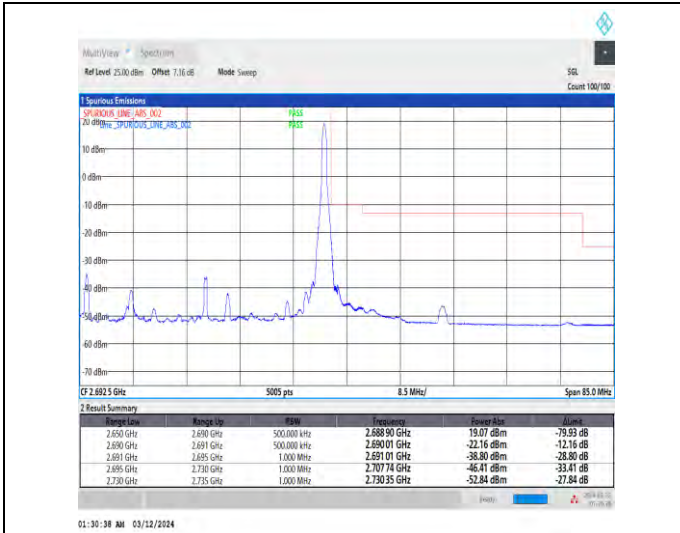
1-N41-30-40-H-2-DFT-PI2BPSK-Edge_1RB_Right-1@105-Ant4-1--PASS-see graph
