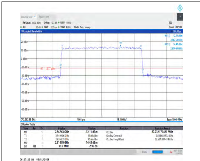
1-N41-30-90-M-6-CP-QPSK-Outer_Full-245@0-Ant4 -87.232-90.900-≤90-PASS
