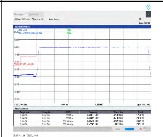
1-N41-30-40-L-6-CP-QPSK-Outer_Full-106@0-Ant4-1--PASS-see graph
