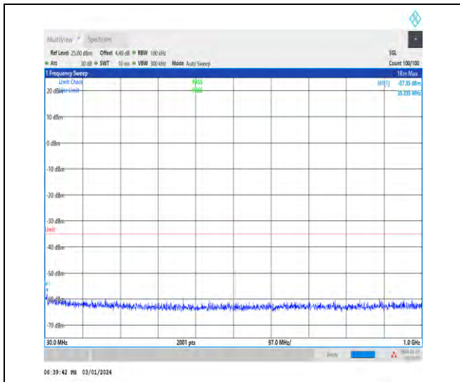
1-N41-30-100-M-1-DFT-PI2BPSK-Inner_1RB_Left-1 @1-30-1000-Ant4-35.34--57.35--35-PASS
