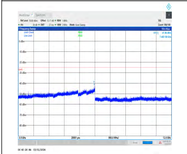
1-N41-30-100-M-1-DFT-PI2BPSK-Inner_1RB_Left-1 @1-3000-12000-Ant4-7463.10--41.96--25-PASS
