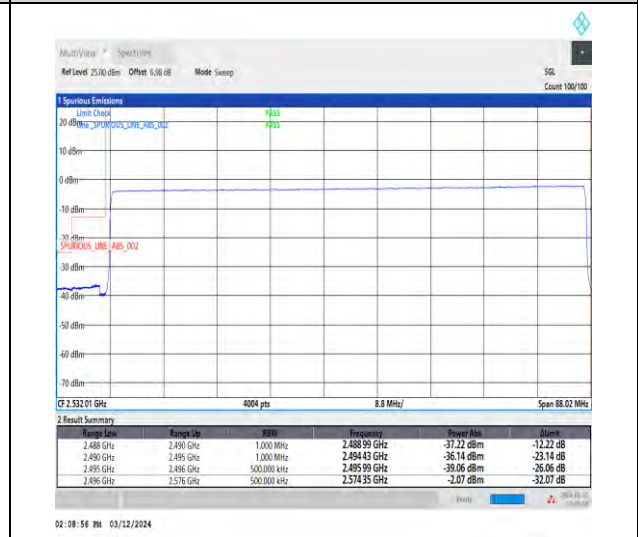
1-N41-30-80-L-6-CP-QPSK-Outer_Full-217@0-Ant4-1--PASS-see graph
