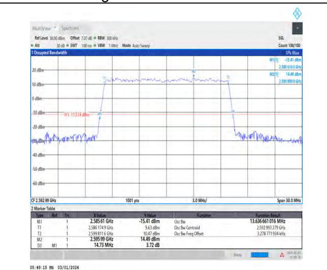
1-N41-30-15-M-9-CP-256QAM-Outer_Full-38@0-Ant 4-13.637-14.730-≤15-PASS
