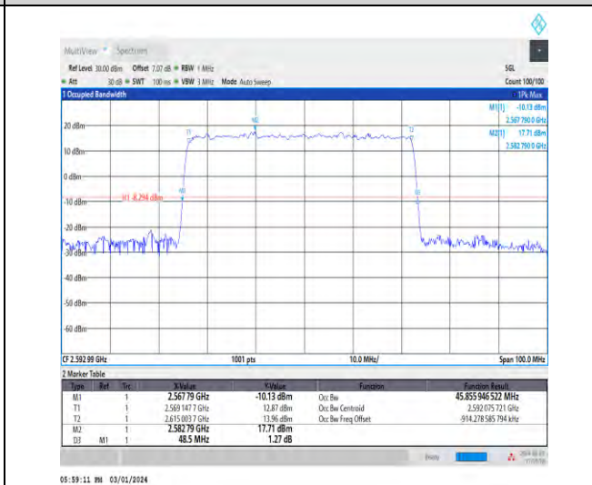
1-N41-30-50-M-4-DFT-64QAM-Outer_Full-128@0-Ant 4-45.856-48.500-≤50-PASS
