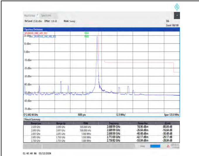
1-N41-30-60-H-2-DFT-PI2BPSK-Edge_1RB_Right-1@161-Ant4-1--PASS-see graph
