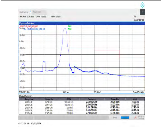
1-N41-30-10-H-5-CP-QPSK-Edge_1RB_Right-1@23-Ant4-1--PASS-see graph
