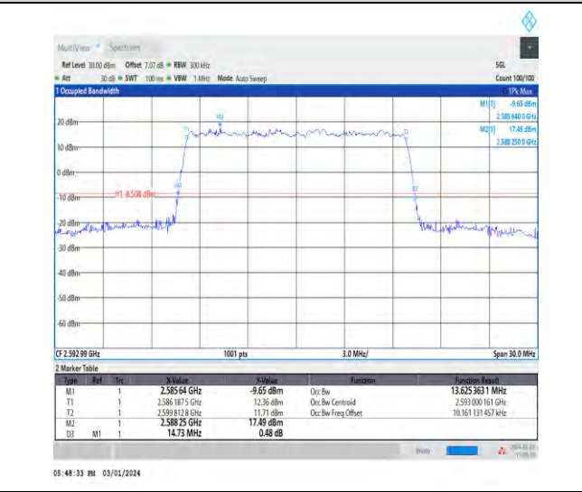
1-N41-30-15-M-7-CP-16QAM-Outer_Full-38@0-Ant4 -13.625-14.730-≤15-PASS
