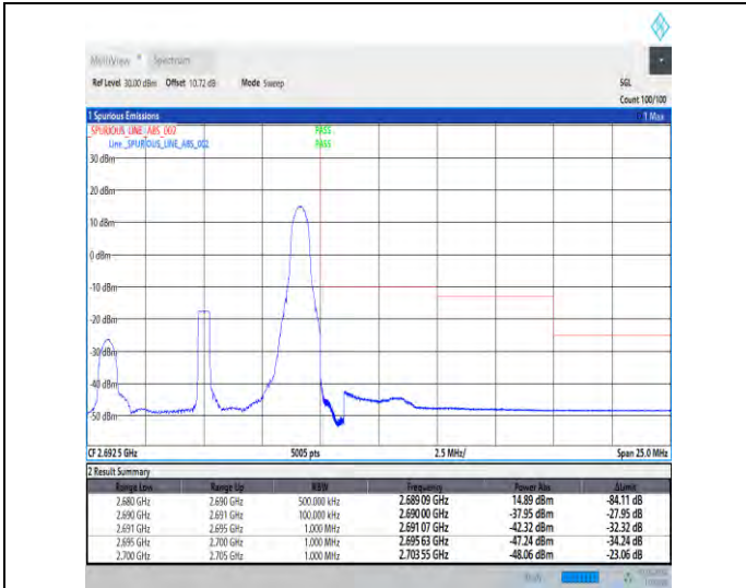
1-N41-30-10-H-2-DFT-PI2BPSK-Edge_1RB_Right-1@23-Ant4-1--PASS-see graph
