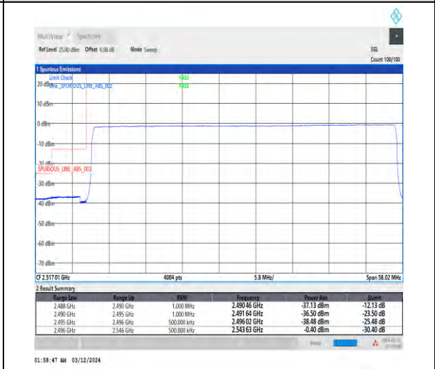
1-N41-30-50-L-6-CP-QPSK-Outer_Full-133@0-Ant4-1--PASS-see graph
