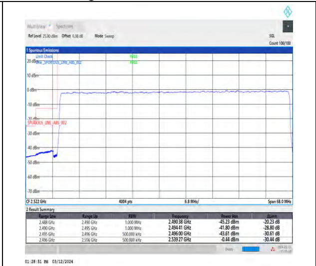
1-N41-30-60-L-3-DFT-PI2BPSK-Outer_Full-162@0-Ant4-1--PASS-see graph
