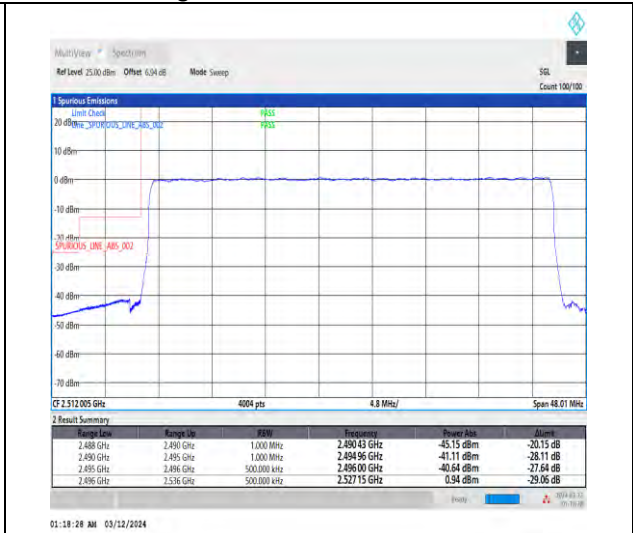
1-N41-30-40-L-3-DFT-PI2BPSK-Outer_Full-100@0-Ant4-1--PASS-see graph
