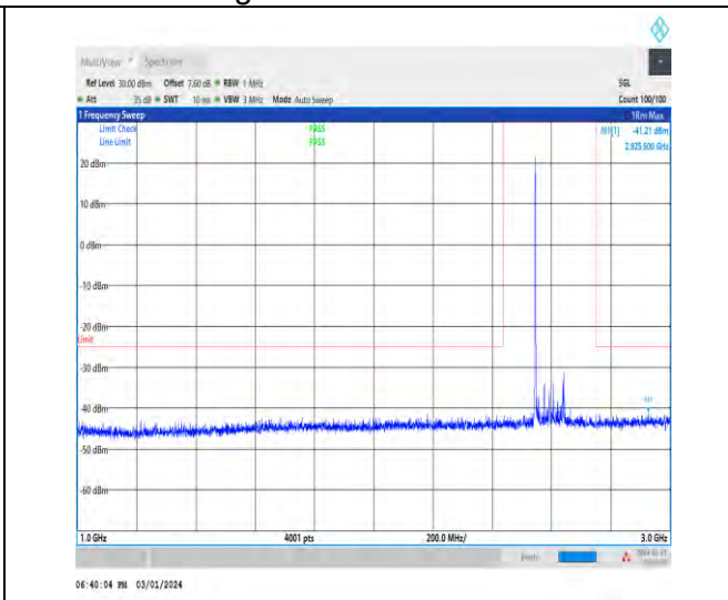
1-N41-30-100-M-1-DFT-PI2BPSK-Inner_1RB_Left-1 @1-1000-3000-Ant4-2925.50--41.21--25-PASS
