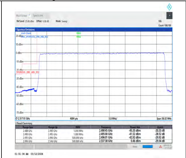
1-N41-30-50-L-3-DFT-PI2BPSK-Outer_Full-128@0-Ant4-1--PASS-see graph
