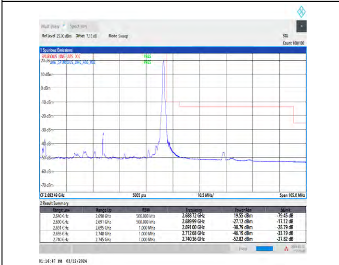
1-N41-30-50-H-5-CP-QPSK-Edge_1RB_Right-1@132-Ant4-1--PASS-see graph
