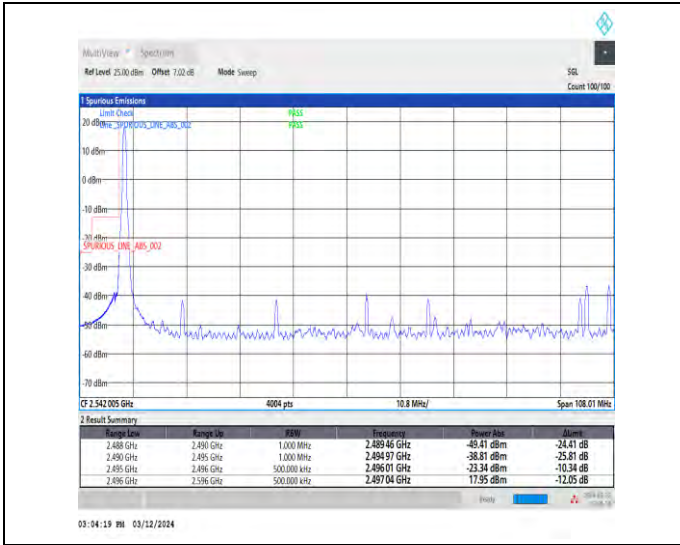
1-N41-30-100-L-1-DFT-PI2BPSK-Edge_1RB_Left-1@0-Ant4-1--PASS-see graph
