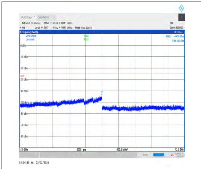
1-N41-30-100-L-1-DFT-PI2BPSK-Inner_1RB_Left-1 @1-3000-12000-Ant4-7490.10--44.36--25-PASS
