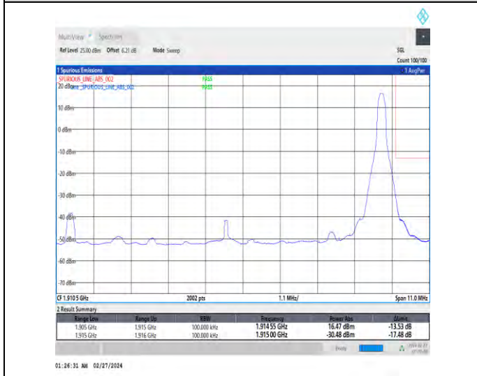
1-N25-15-10-H-5-CP-QPSK-Edge_1RB_Right-1@51-Ant4-1-seegraph-PASS-see graph
