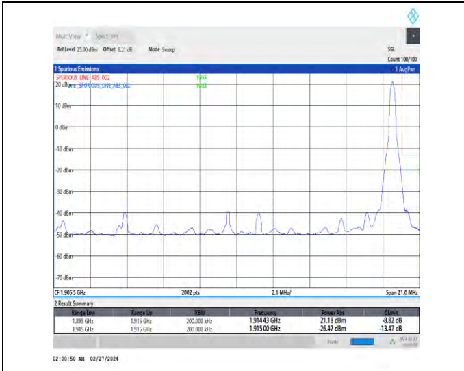
1-N25-15-20-H-2-DFT-PI2BPSK-Edge_1RB_Right-1@105-Ant4-1-seegraph-PASS-see graph
