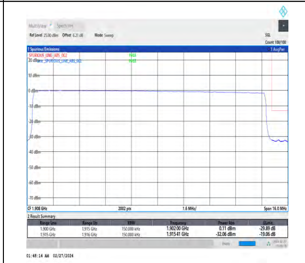
1-N25-15-15-H-6-CP-QPSK-Outer_Full-79@0-Ant4-1-seegraph-PASS-see graph
