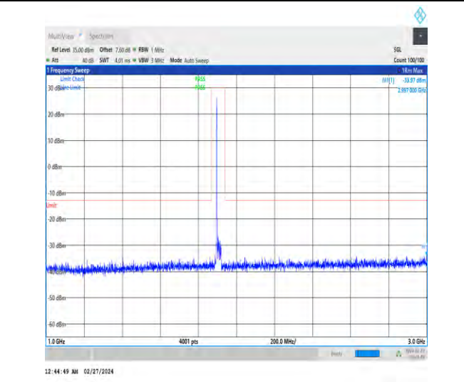
1-N25-15-20-H-1-DFT-PI2BPSK-Inner_1RB_Left-1 @ 1-1000-3000-Ant4-2997.00--33.97--13-PASS
