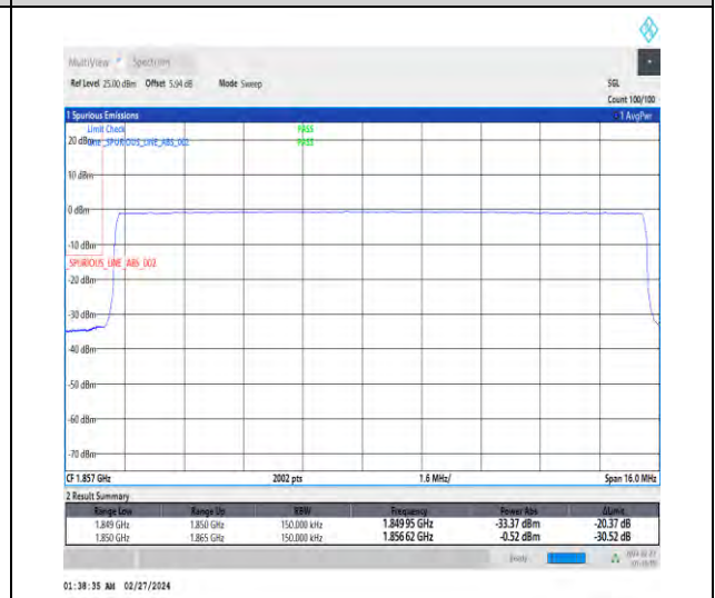
1-N25-15-15-L-6-CP-QPSK-Outer_Full-79@0-Ant4-1-seegraph-PASS-see graph
