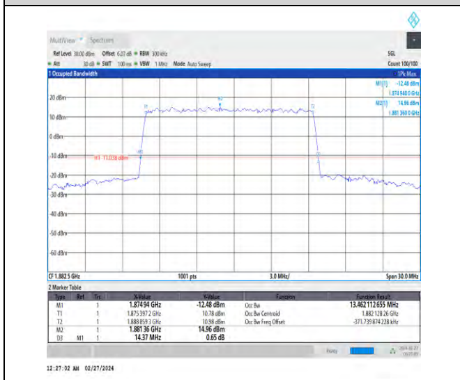
1-N25-15-15-M-1-DFT-QPSK-Outer_Full-75@0-Ant4 -13.462-14.370-≤15-PASS
