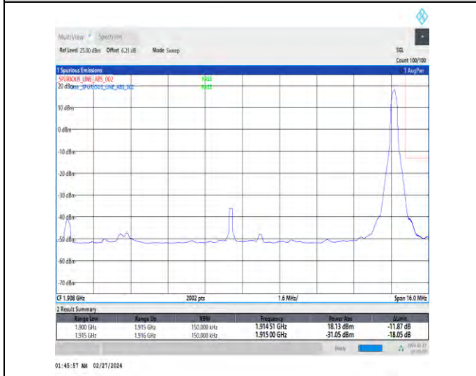
1-N25-15-15-H-5-CP-QPSK-Edge_1RB_Right-1@78-Ant4-1-seegraph-PASS-see graph
