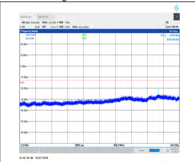
1-N25-15-20-H-1-DFT-PI2BPSK-Inner_1RB_Left-1@ 1-12000-20000-Ant4-18947.60--24.96--13-PASS
