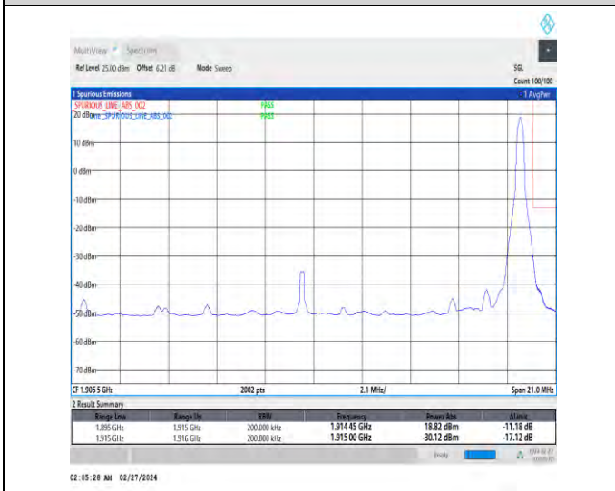
1-N25-15-20-H-5-CP-QPSK-Edge_1RB_Right-1@105-Ant4-1-seegraph-PASS-see graph
