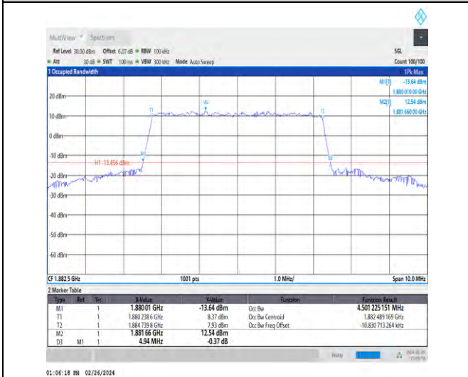
1-N25-15-5-M-7-CP-16QAM-Outer_Full-25@0-Ant4-4 4.501-4.940-≤5-PASS
