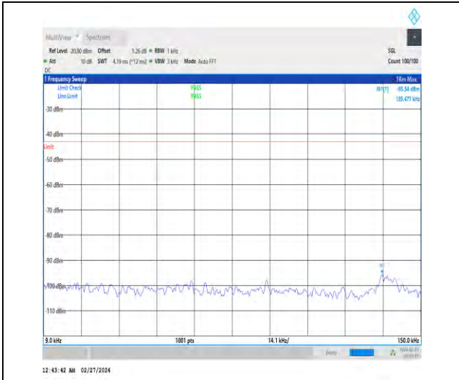
1-N25-15-20-H-1-DFT-PI2BPSK-Inner_1RB_Left-1 @ 1-0.009-0.15-Ant4-0.14--95.54--43-PASS
