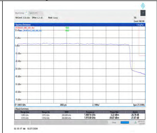
1-N25-15-20-H-3-DFT-PI2BPSK-Outer_Full-100@0-Ant4-1-seegraph-PASS-see graph
