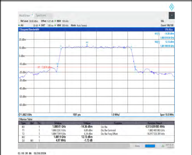
1-N25-15-5-M-8-CP-64QAM-Outer_Full-25@0-Ant4-4 4.514-4.970-≤5-PASS
