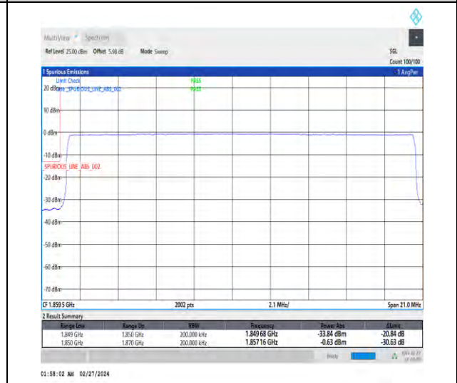
1-N25-15-20-L-6-CP-QPSK-Outer_Full-106@0-Ant4-1-seegraph-PASS-see graph
