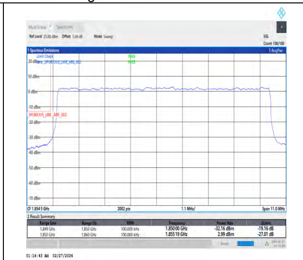
1-N25-15-10-L-3-DFT-PI2BPSK-Outer_Full-50@0-Ant4-1-seegraph-PASS-see graph
