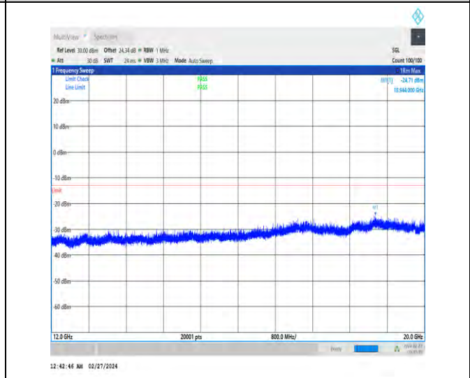
1-N25-15-20-M-1-DFT-PI2BPSK-Inner_1RB_Left-1 @ 1-12000-20000-Ant4-18944.00--24.71--13-PASS
