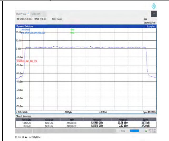
1-N25-15-20-L-3-DFT-PI2BPSK-Outer_Full-100@0-Ant4-1-seegraph-PASS-see graph
