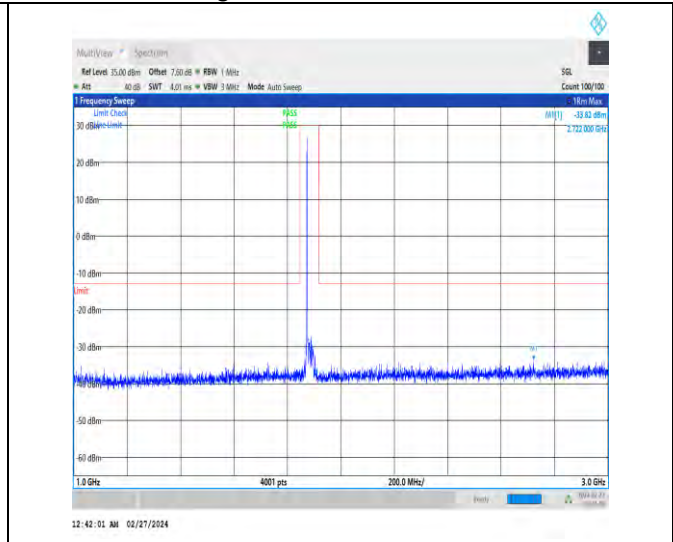
1-N25-15-20-M-1-DFT-PI2BPSK-Inner_1RB_Left-1 @ 1-1000-3000-Ant4-2722.00--33.82--13-PASS
