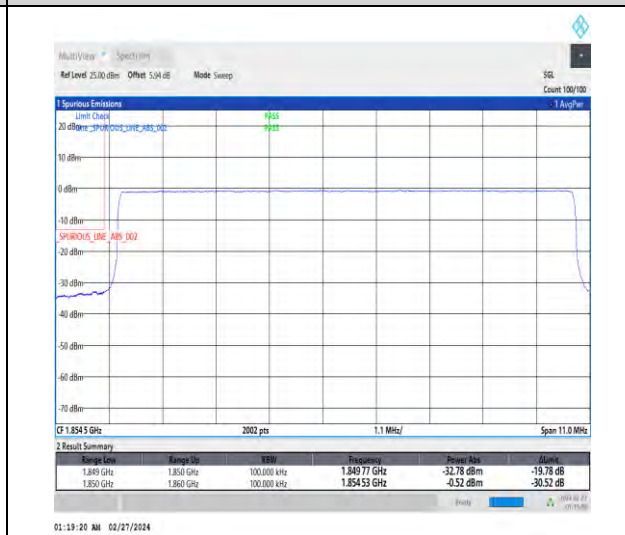
1-N25-15-10-L-6-CP-QPSK-Outer_Full-52@0-Ant4-1-seegraph-PASS-see graph
