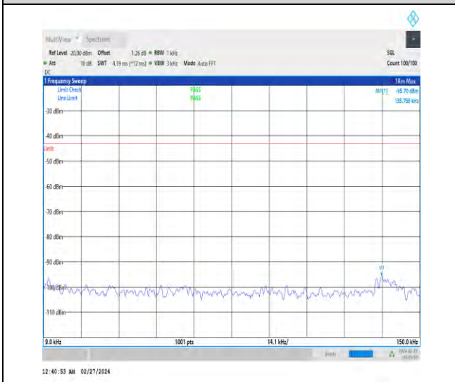
1-N25-15-20-M-1-DFT-PI2BPSK-Inner_1RB_Left-1 @ 1-0.009-0.15-Ant4-0.14--95.70--43-PASS
