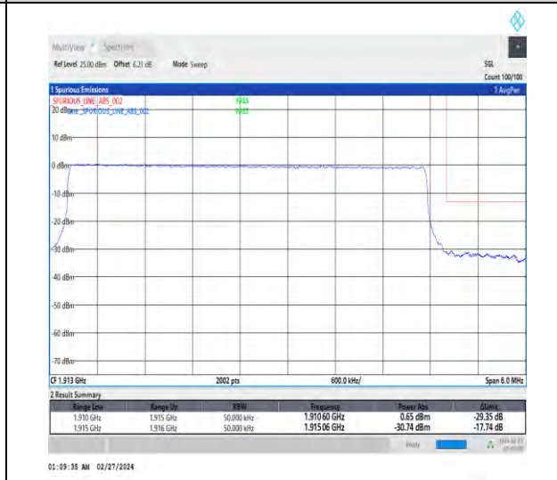
1-N25-15-5-H-6-CP-QPSK-Outer_Full-25@0-Ant4-1-seegraph-PASS-see graph
