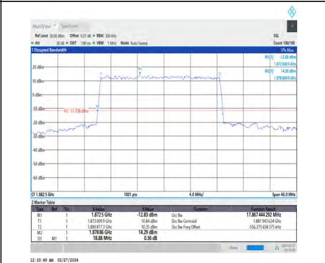
1-N25-15-20-M-1-DFT-QPSK-Outer_Full-100@0-Ant4 4-17.867-18.880-≤20-PASS
