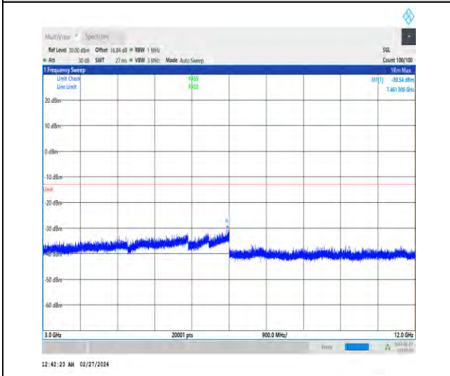
1-N25-15-20-M-1-DFT-PI2BPSK-Inner_1RB_Left-1 @ 1-3000-12000-Ant4-7461.30--30.54--13-PASS
