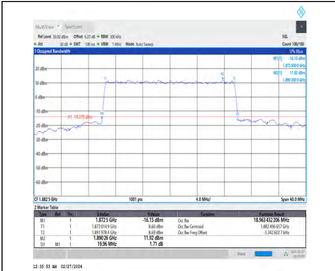
1-N25-15-20-M-6-CP-QPSK-Outer_Full-106@0-Ant4 -18.963-19.960-≤20-PASS
