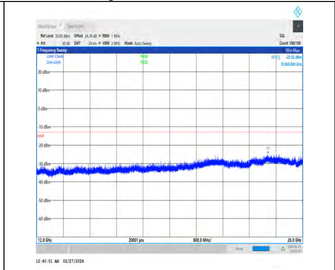
1-N25-15-20-L-1-DFT-PI2BPSK-Inner_1RB_Left-1@ 1-12000-20000-Ant4-18965.60--25.02--13-PASS
