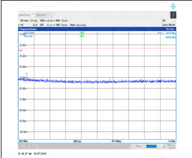
1-N25-15-20-H-1-DFT-PI2BPSK-Inner_1RB_Left-1 @ 1-30-1000-Ant4-80.93--49.70--23-PASS
