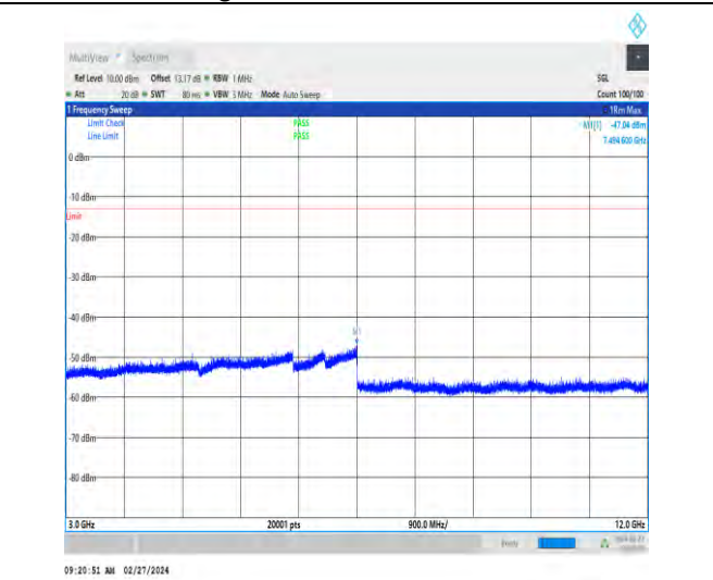
1-N5-15-20-M-1-DFT-PI2BPSK-Inner_1RB_Left-1@ 1-3000-12000-Ant1-7494.60--47.04--13-PASS
