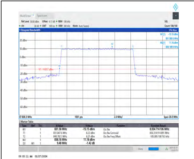
1-N5-15-10-M-4-DFT-64QAM-Outer_Full-50@0-Ant 1-8.935-9.480-≤10-PASS
