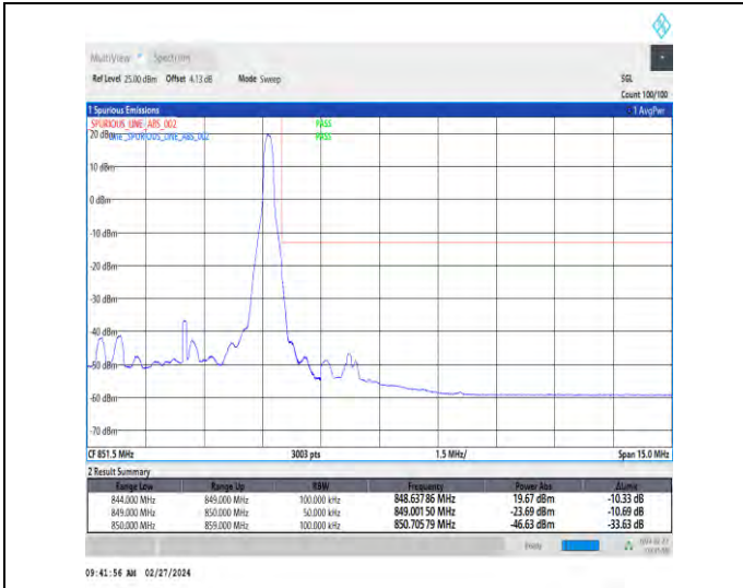
1-N5-15-5-H-2-DFT-PI2BPSK-Edge_1RB_Right-1@24-Ant1-1--PASS-see graph
