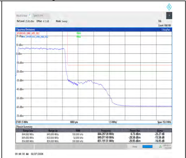
1-N5-15-5-H-3-DFT-PI2BPSK-Outer_Full-25@0-Ant1-1--PASS-see graph
