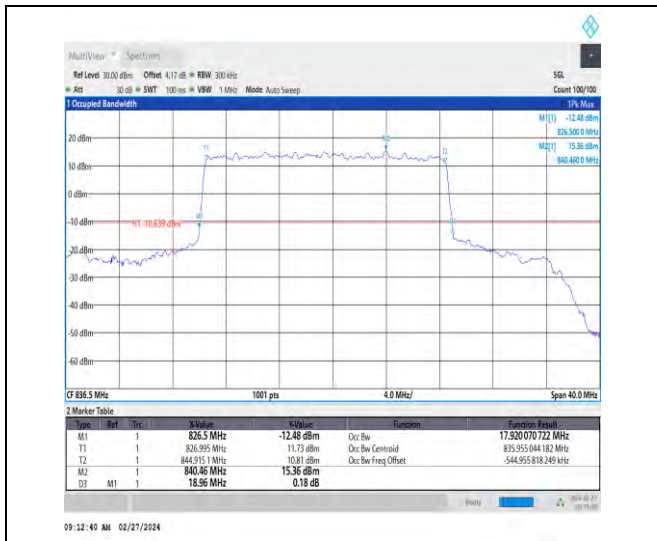
1-N5-15-20-M-2-DFT-P12BPSK-Outer_Full-100@0-A nt1-17.92-18.960-≤20-PASS
