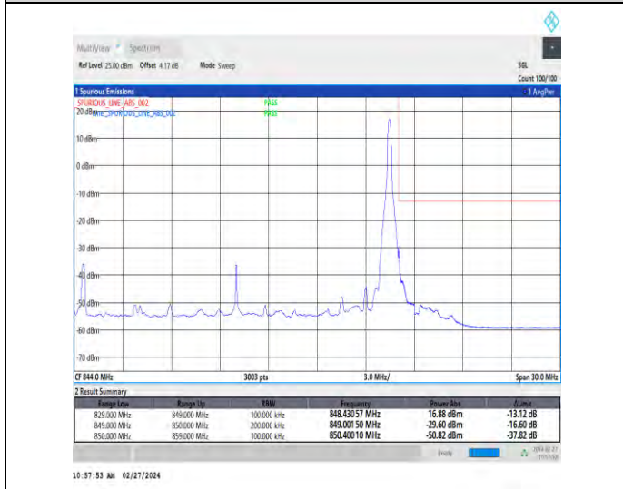
1-N5-15-20-H-5-CP-QPSK-Edge_1RB_Right-1@105-Ant1-1--PASS-see graph
