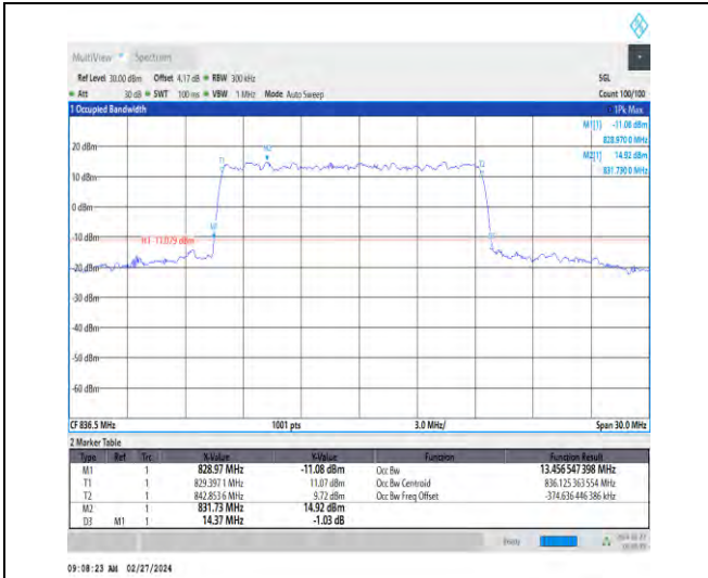
1-N5-15-15-M-3-DFT-16QAM-Outer_Full-75@0-Ant 1-13.457-14.370≤15-PASS
