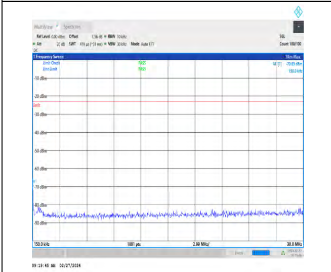
1-N5-15-20-M-1-DFT-PI2BPSK-Inner_1RB_Left-1@ 1-0.15-30-Ant1-0.15--70.63--23-PASS
