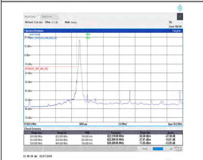
1-N5-15-20-L-4-CP-QPSK-Edge_1RB_Left-1@0-Ant1-1--PASS-see graph
