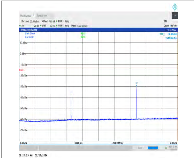
1-N5-15-20-M-1-DFT-PI2BPSK-Inner_1RB_Left-1@ 1-1000-3000-Ant1-2482.00--30.39--13-PASS
