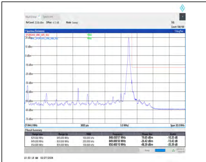
1-N5-15-20-H-2-DFT-PI2BPSK-Edge_1RB_Right-1@105-Ant1-1--PASS-see graph
