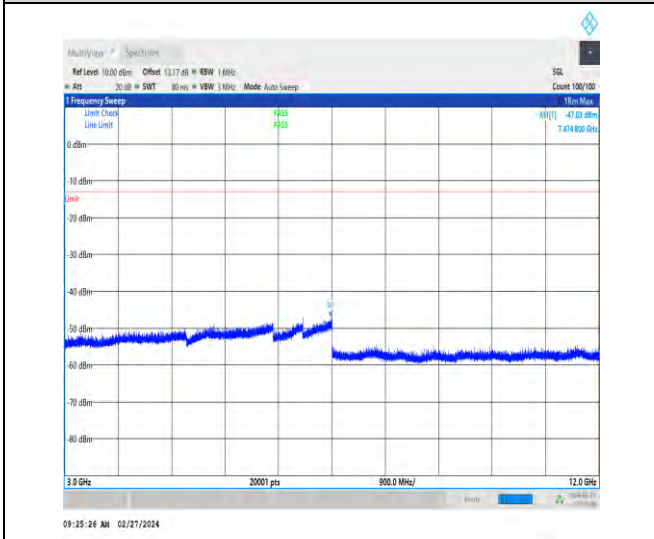
1-N5-15-20-H-1-DFT-PI2BPSK-Inner_1RB_Left-1@1 -3000-12000-Ant1-7474.80--47.03--13-PASS
