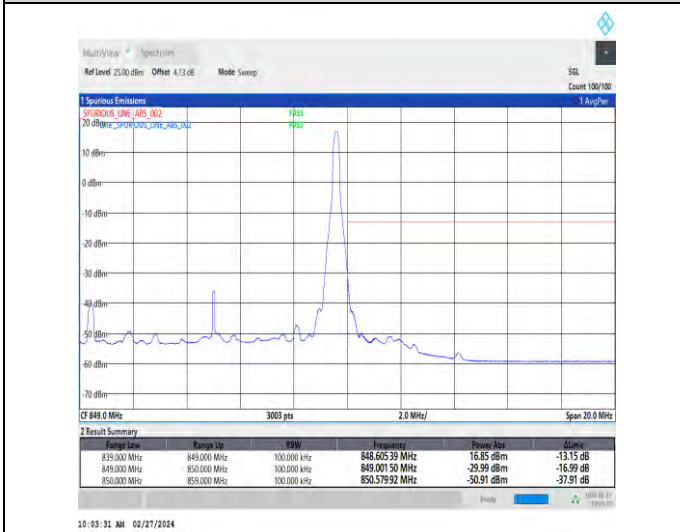
1-N5-15-10-H-5-CP-QPSK-Edge_1RB_Right-1@51-Ant1-1--PASS-see graph
