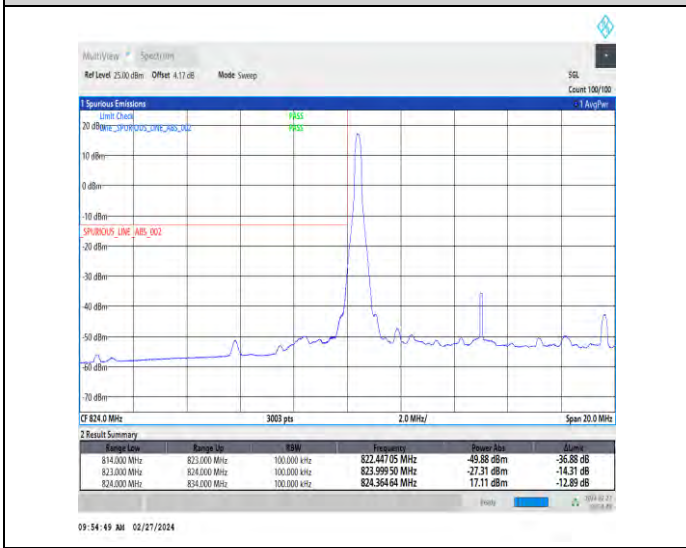
1-N5-15-10-L-4-CP-QPSK-Edge_1RB_Left-1@0-Ant1-1--PASS-see graph
