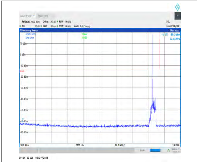
1-N5-15-20-H-1-DFT-PI2BPSK-Inner_1RB_Left-1@1 -30-1000-Ant1-50.86--61.43--13-PASS
