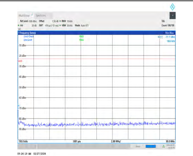
1-N5-15-20-H-1-DFT-PI2BPSK-Inner_1RB_Left-1@1 -0.15-30-Ant1-0.15--71.11--23-PASS
