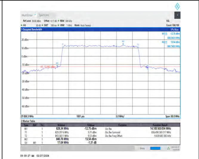
1-N5-15-15-M-6-CP-QPSK-Outer_Full-79@0-Ant1-1 4.186-17.040≤15-PASS
