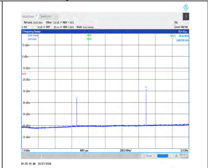
1-N5-15-20-H-1-DFT-PI2BPSK-Inner_1RB_Left-1@1 -1000-3000-Ant1-2489.50--29.92--13-PASS
