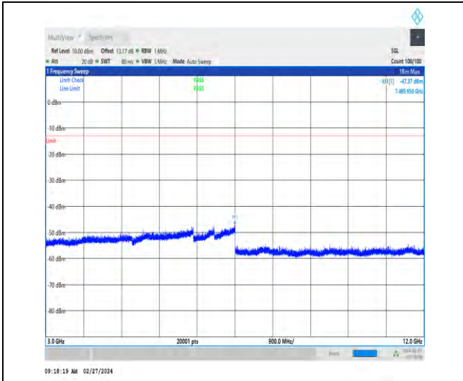
1-N5-15-20-L-1-DFT-PI2BPSK-Inner_1RB_Left-1@ -3000-12000-Ant1-7495.95--47.37--13-PASS
