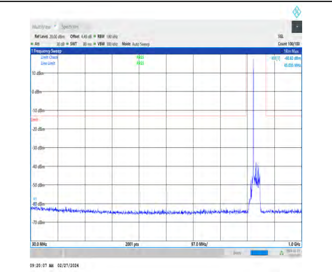
1-N5-15-20-M-1-DFT-PI2BPSK-Inner_1RB_Left-1@ 1-30-1000-Ant1-45.04--60.82--13-PASS
