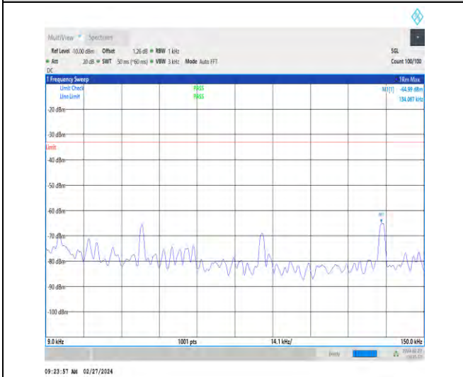
1-N5-15-20-H-1-DFT-PI2BPSK-Inner_1RB_Left-1@1 -0.009-0.15-Ant1-0.13--64.99--33-PASS
