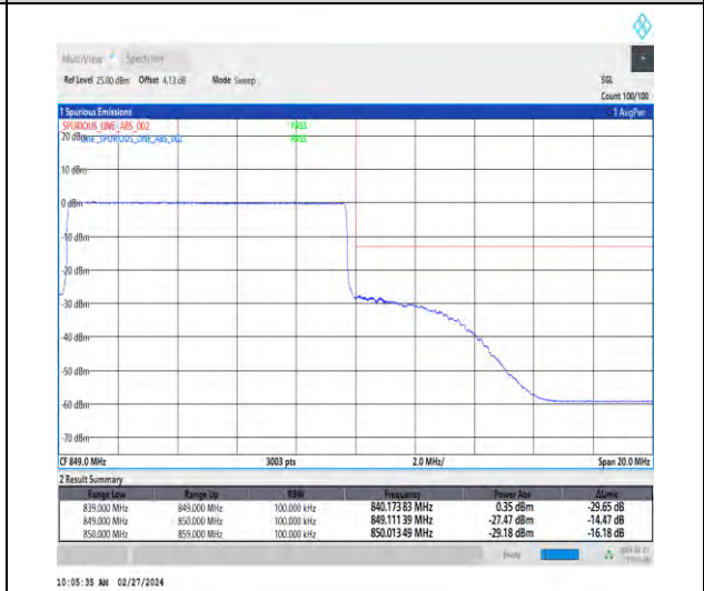
1-N5-15-10-H-6-CP-QPSK-Outer_Full-52@0-Ant1-1--PASS-see graph
