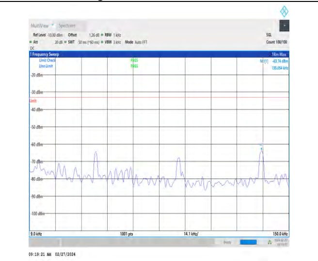
1-N5-15-20-M-1-DFT-PI2BPSK-Inner_1RB_Left-1@ 1-0.009-0.15-Ant1-0.14--63.74--33-PASS
