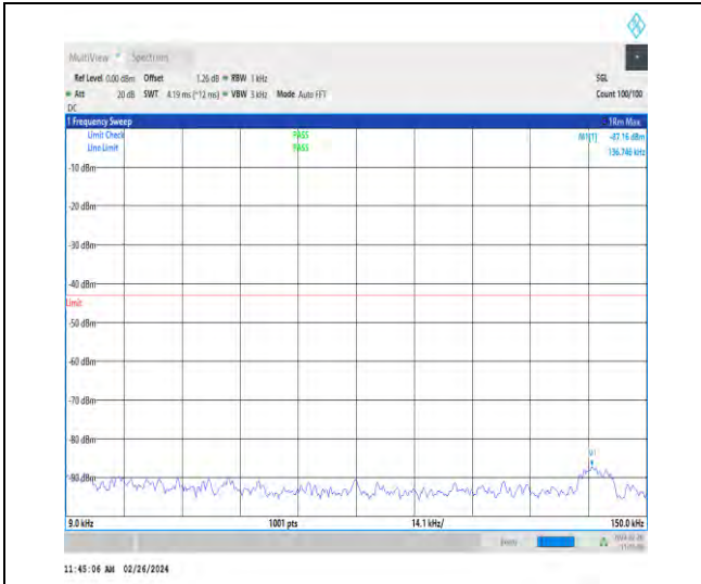
1-N2-15-20-H-1-DFT-PI2BPSK-Inner_1RB_Left-1@ 1-0.009-0.15-Ant4-0.14--87.16--43-PASS
