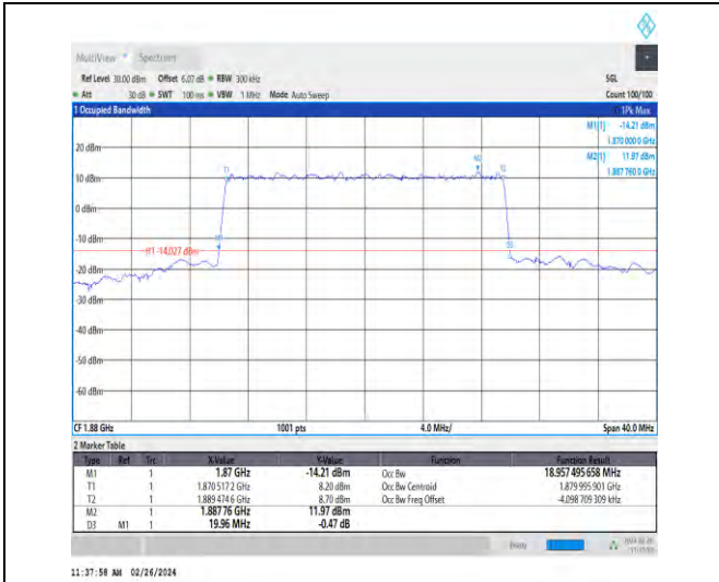
1-N2-15-20-M-6-CP-QPSK-Outer_Full-106@0-Ant4-18.957-19.960-≤20-PASS
