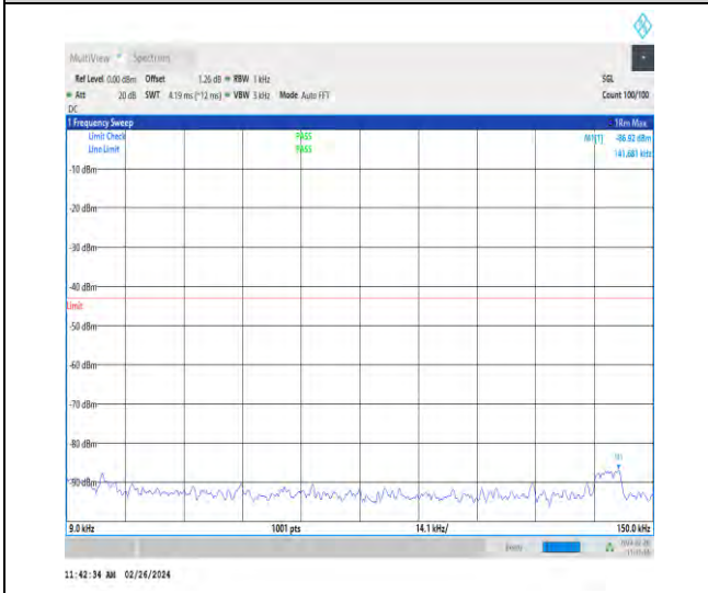
1-N2-15-20-M-1-DFT-PI2BPSK-Inner_1RB_Left-1@ 1-0.009-0.15-Ant4-0.14--86.92--43-PASS
