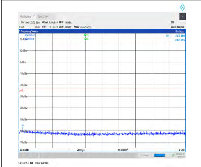
1-N2-15-20-H-1-DFT-PI2BPSK-Inner_1RB_Left-1@ 1-30-1000-Ant4-51.83--58.75--23-PASS
