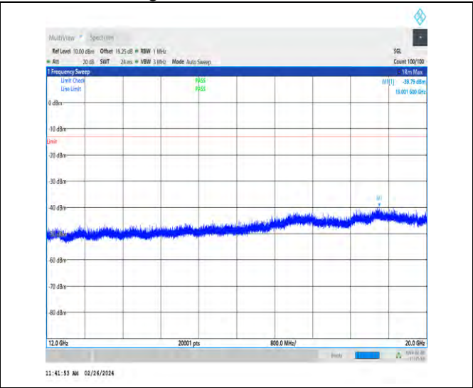
1-N2-15-20-L-1-DFT-PI2BPSK-Inner_1RB_Left-1@1- 12000-20000-Ant4-19001.60--39.79--13-PASS
