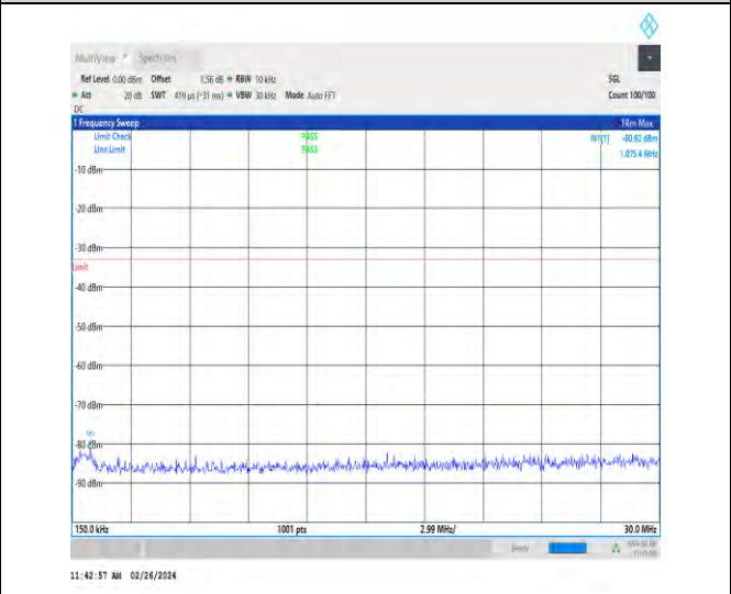
1-N2-15-20-M-1-DFT-PI2BPSK-Inner_1RB_Left-1@1- 0.15-30-Ant4-1.08--80.92--33-PASS
