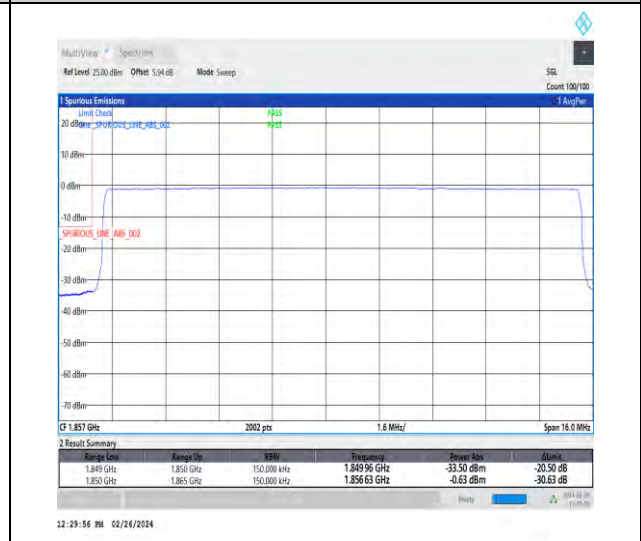
1-N2-15-15-L-6-CP-QPSK-Outer_Full-79@0-Ant4-1-seegraph-PASS-see graph
