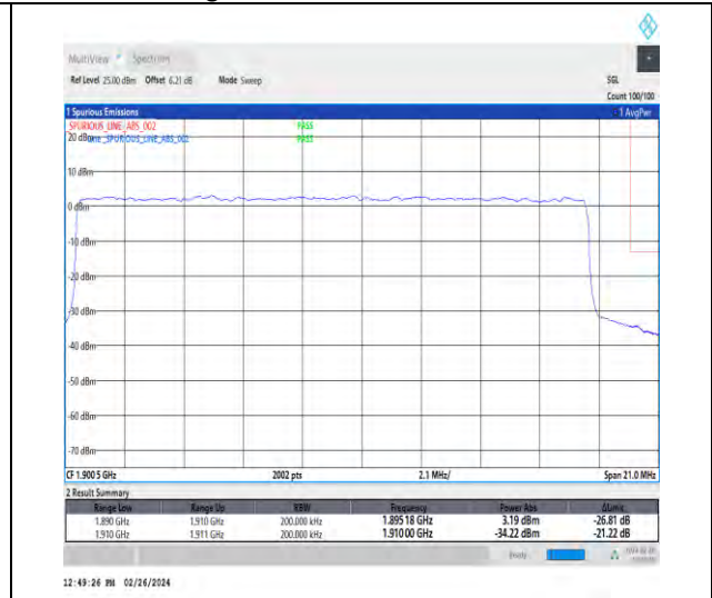
1-N2-15-20-H-3-DFT-PI2BPSK-Outer_Full-100@0-Ant4-1-seegraph-PASS-see graph
