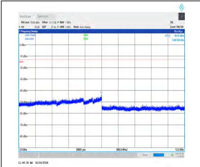
1-N2-15-20-H-1-DFT-PI2BPSK-Inner_1RB_Left-1@ 1-3000-12000-Ant4-7483.35--45.05--13-PASS
