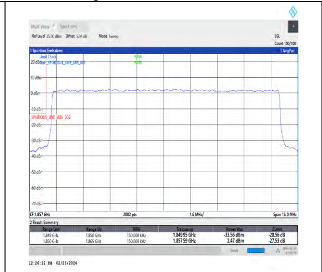
1-N2-15-15-L-3-DFT-PI2BPSK-Outer_Full-75@0-Ant4-1-seegraph-PASS-see graph
