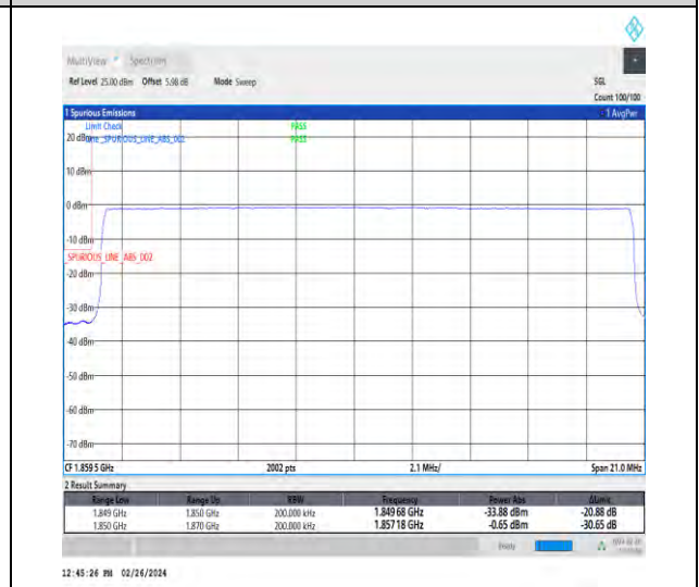
1-N2-15-20-L-6-CP-QPSK-Outer_Full-106@0-Ant 4-1-seegraph-PASS-see graph
