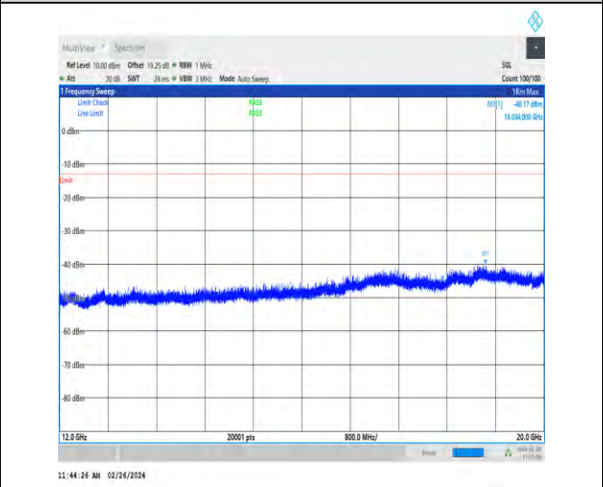
1-N2-15-20-M-1-DFT-PI2BPSK-Inner_1RB_Left-1@ -12000-20000-Ant4-19034.00--40.17--13-PASS
