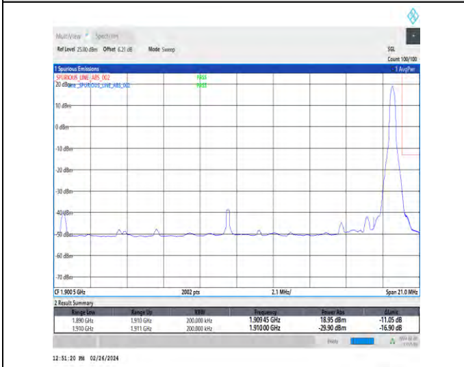
1-N2-15-20-H-5-CP-QPSK-Edge_1RB_Right-1@105-Ant4-1-seegraph-PASS-see graph
