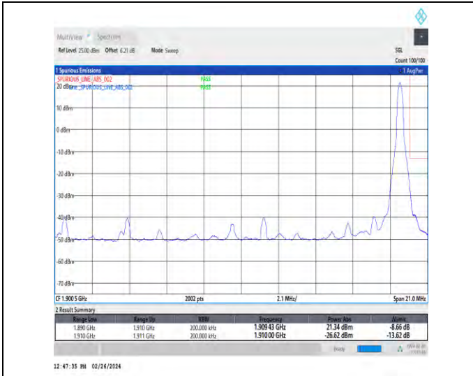
1-N2-15-20-H-2-DFT-PI2BPSK-Edge_1RB_Right-1@105-Ant4-1-seegraph-PASS-see graph
