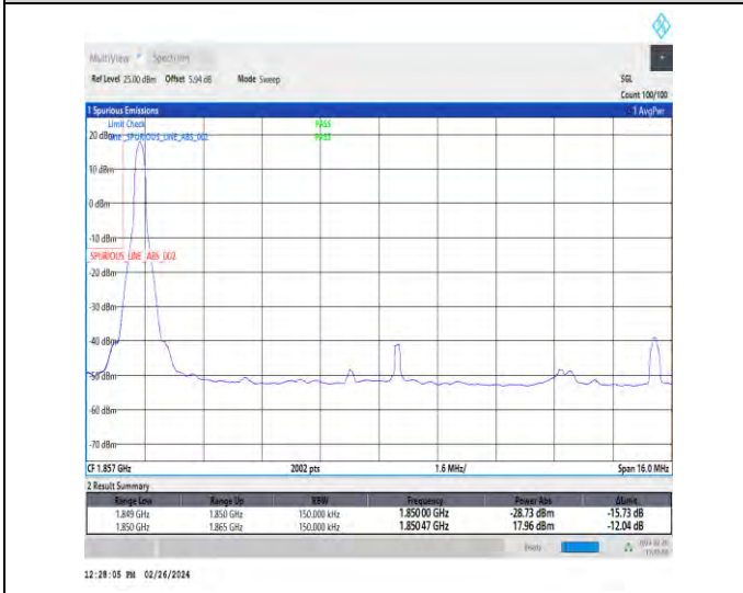
1-N2-15-15-L-4-CP-QPSK-Edge_1RB_Left-1@0-Ant4-1-seegraph-PASS-see graph
