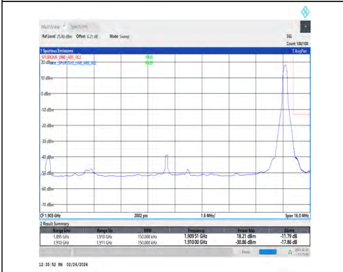
1-N2-15-15-H-5-CP-QPSK-Edge_1RB_Right-1@78-Ant4-1-seegraph-PASS-see graph
