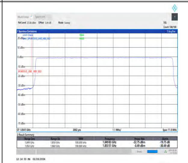
1-N2-15-10-L-6-CP-QPSK-Outer_Full-52@0-Ant4-1-seegraph-PASS-see graph
