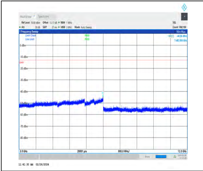
1-N2-15-20-L-1-DFT-PI2BPSK-Inner_1RB_Left-1@ 1-3000-12000-Ant4-7482.00--44.58--13-PASS
