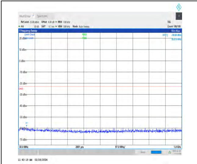
1-N2-15-20-M-1-DFT-PI2BPSK-Inner_1RB_Left-1@ 1-30-1000-Ant4-78.02--58.68--23-PASS
