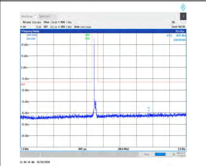
1-N2-15-20-H-1-DFT-PI2BPSK-Inner_1RB_Left-1@ -1000-3000-Ant4-2549.50--38.97--13-PASS
