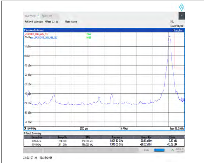
1-N2-15-15-H-2-DFT-PI2BPSK-Edge_1RB_Right-1@78-Ant4-1-seegraph-PASS-see graph
