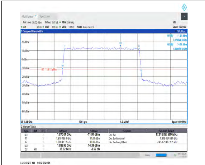
1-N2-15-20-M-2-DFT-PI2BPSK-Outer_Full-100@0-A nt4-17.917-18.920-≤20-PASS
