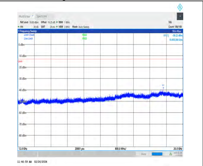
1-N2-15-20-H-1-DFT-PI2BPSK-Inner_1RB_Left-1@ -12000-20000-Ant4-19053.20--39.22--13-PASS
