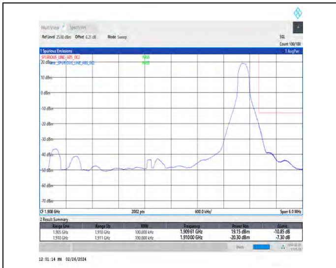
1-N2-15-5-H-2-DFT-PI2BPSK-Edge_1RB_Right-1@24-Ant4-1-see graph-PASS-see graph
