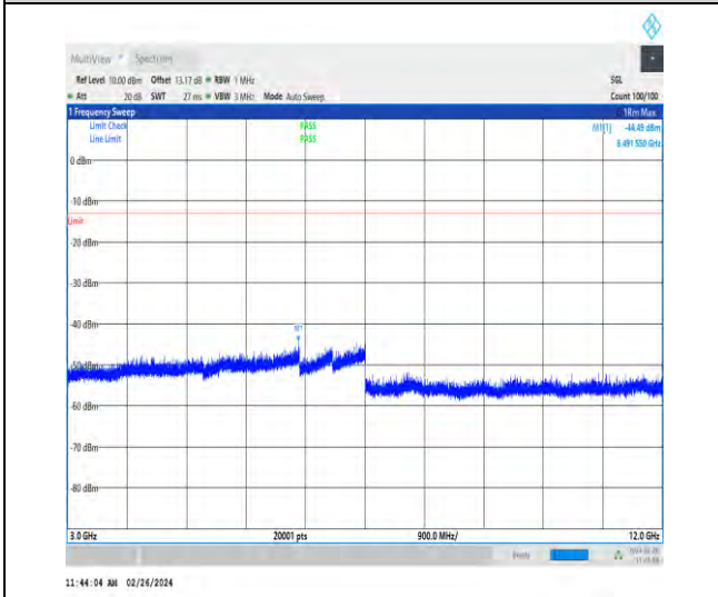
1-N2-15-20-M-1-DFT-PI2BPSK-Inner_1RB_Left-1@ 1-3000-12000-Ant4-6491.55--44.49--13-PASS
