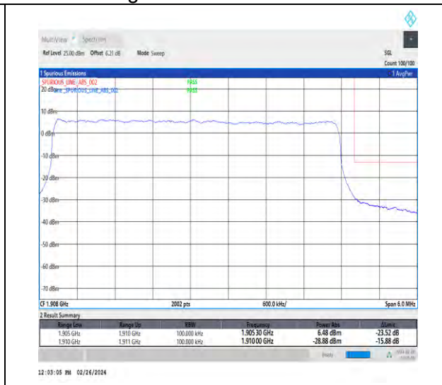
1-N2-15-5-H-3-DFT-PI2BPSK-Outer_Full-25@0-Ant4-1-see graph-PASS-see graph
