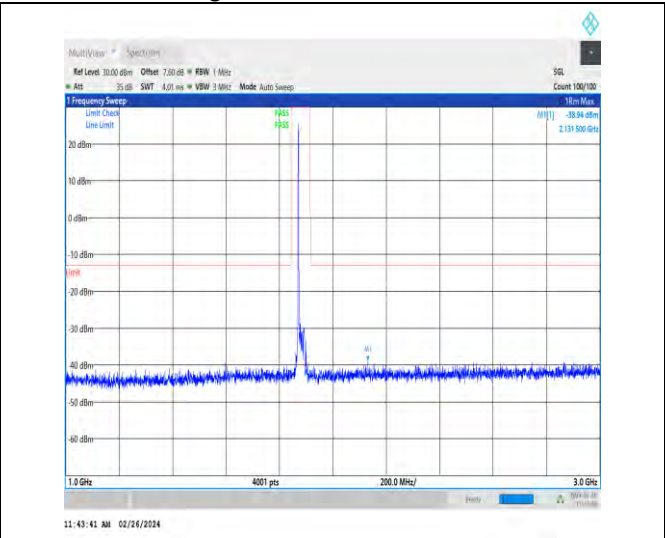
1-N2-15-20-M-1-DFT-PI2BPSK-Inner_1RB_Left-1@ -1000-3000-Ant4-2131.50--38.94--13-PASS
