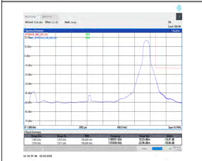
1-N2-15-5-H-5-CP-QPSK-Edge_1RB_Right-1@24-Ant4-1-see graph-PASS-see graph
