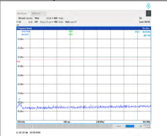
1-N2-15-20-H-1-DFT-PI2BPSK-Inner_1RB_Left-1@ -0.15-30-Ant4-0.81--80.04--33-PASS
