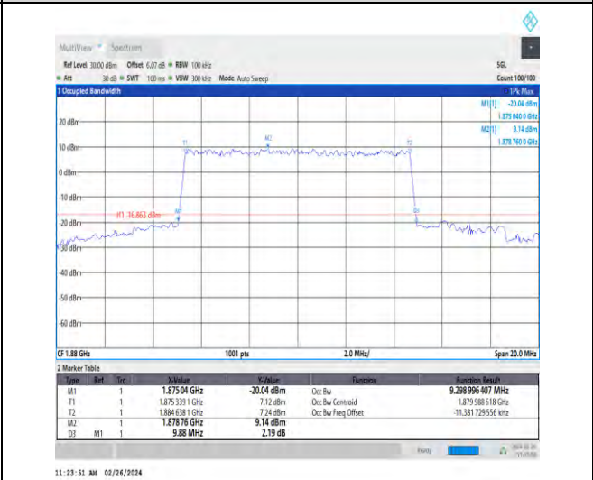
1-N2-15-10-M-7-CP-16QAM-Outer_Full-52@0-Ant4-9. 9.299-9.880≤10-PASS
