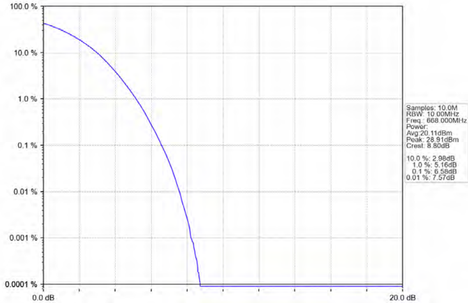
Band71_10MHz_64QAM_LCH_668MHz_RB_50_0_NTNV
