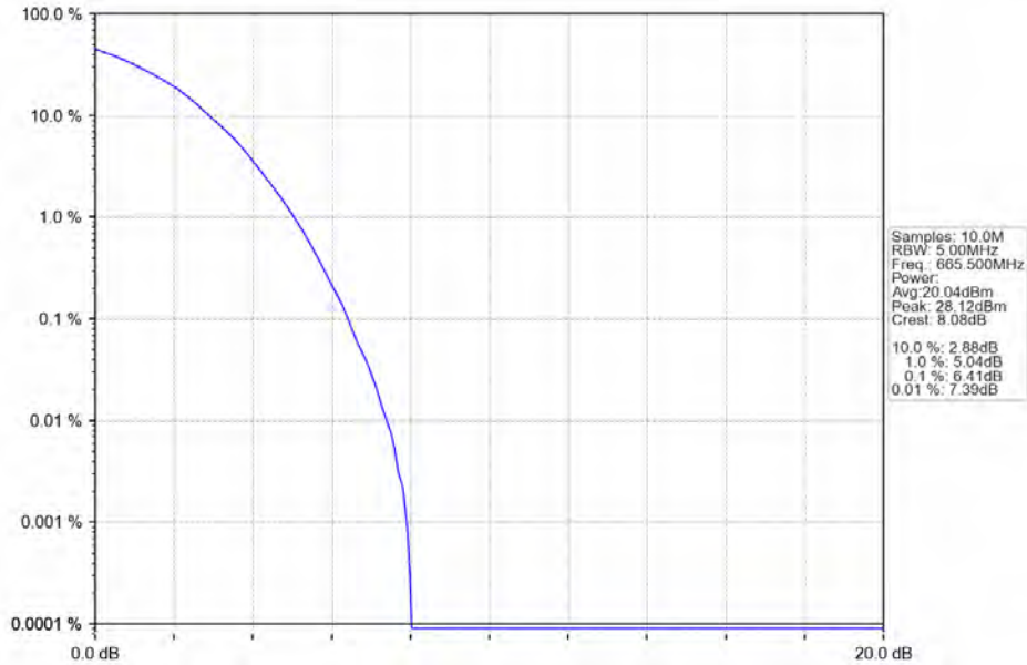
Band71_5MHz_64QAM_LCH_665.5MHz_RB_25_0_NTNV
