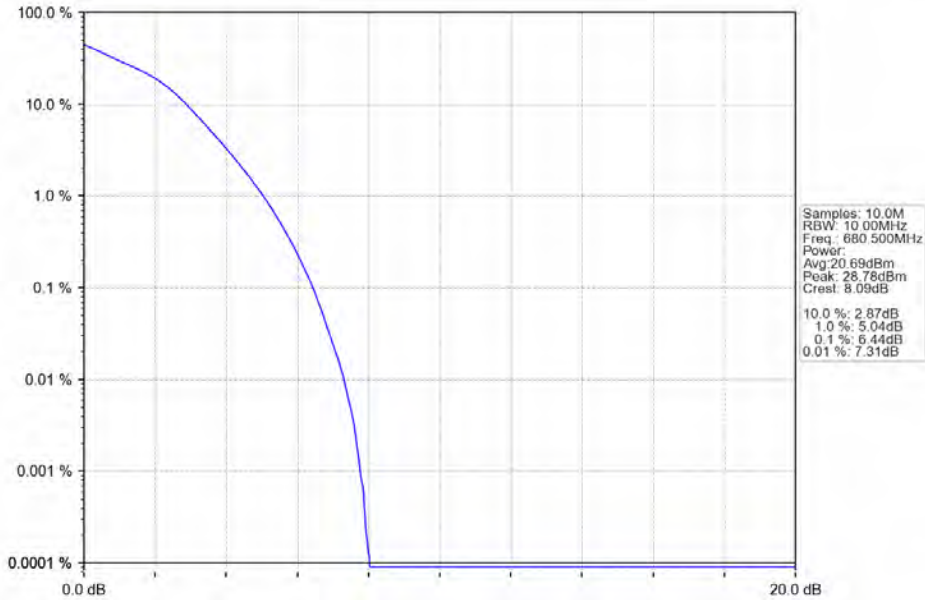
Band71_10MHz_16QAM_MCH_680.5MHz_RB_50_0_NTNV
