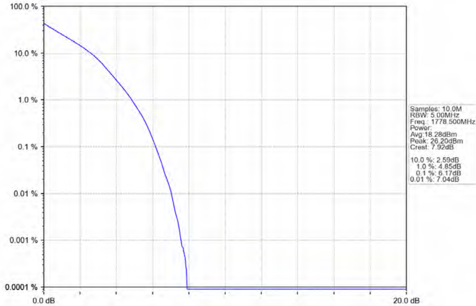
Band66_3MHz_QPSK_HCH_1778.5MHz_RB_15_0_NTNV
