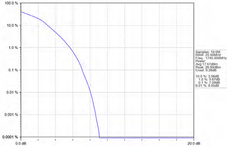
Band66_15MHz_16QAM_MCH_1745MHz_RB_75_0_NTNV
