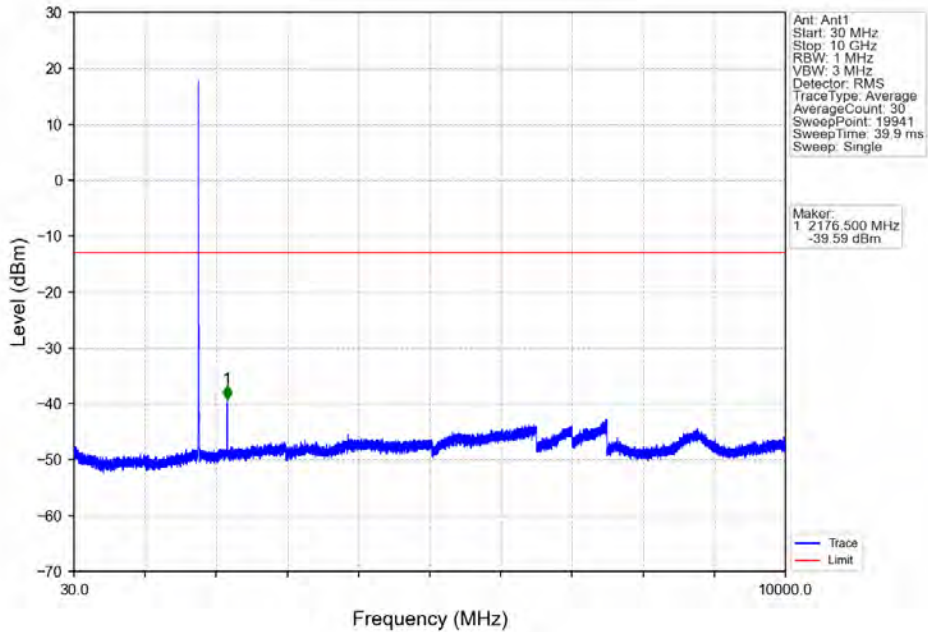
Band66_5MHz_QPSK_HCH_1777.5MHz_RB_1_0_NTNV
