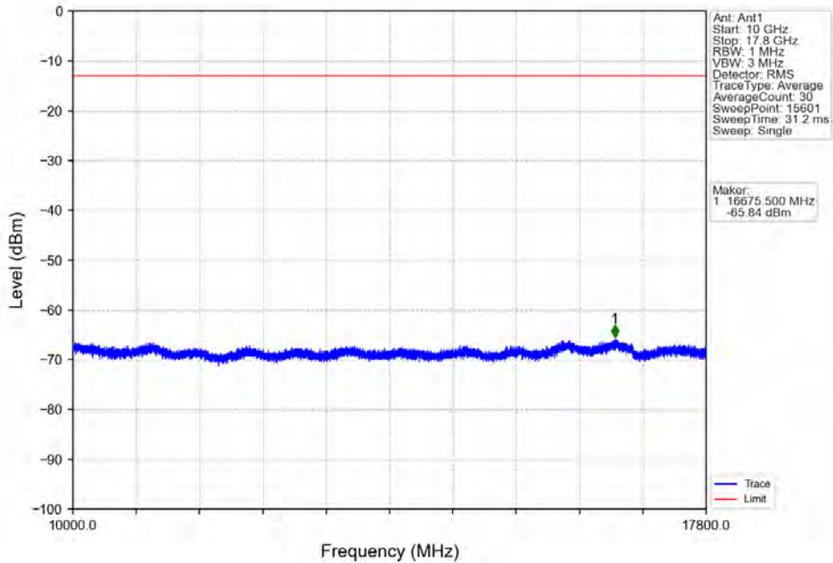
Band66_1.4MHz_QPSK_LCH_1710.7MHz_RB_6_0_NTNV
