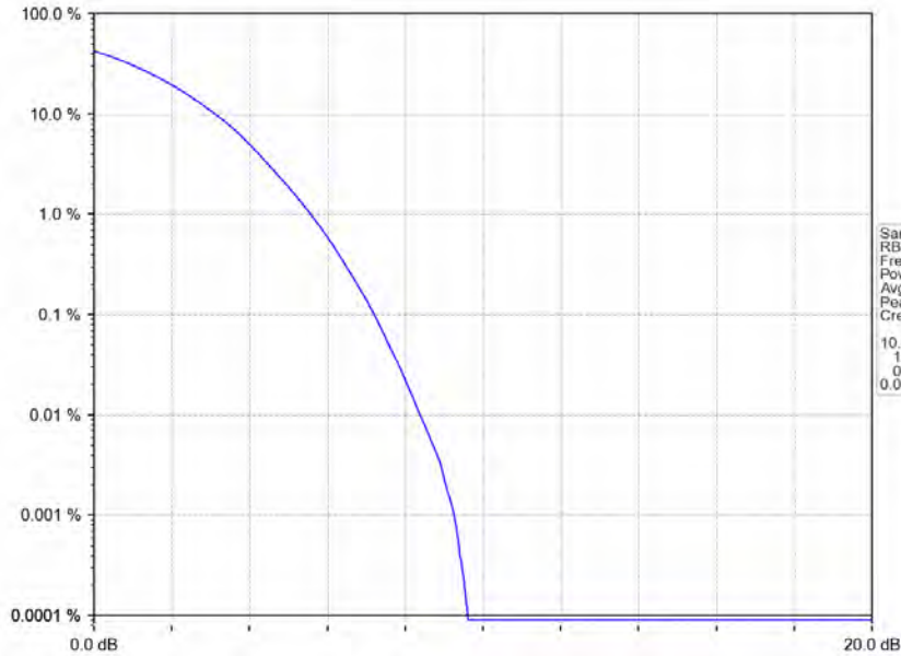
Band66_20MHz_64QAM_LCH_1720MHz_RB_100_0_NTNV
