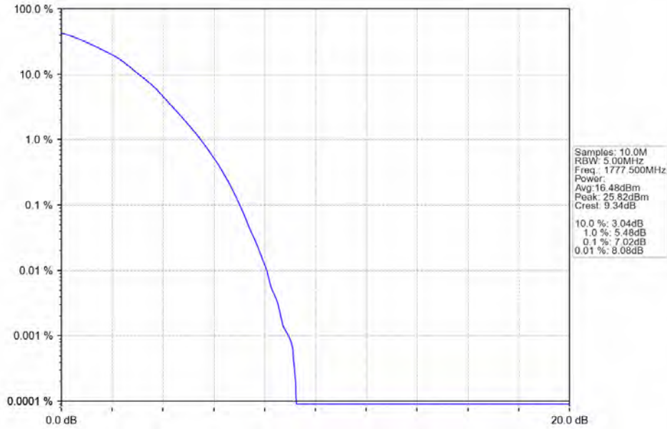
Band66_5MHz_64QAM_HCH_1777.5MHz_RB_25_0_NTNV
