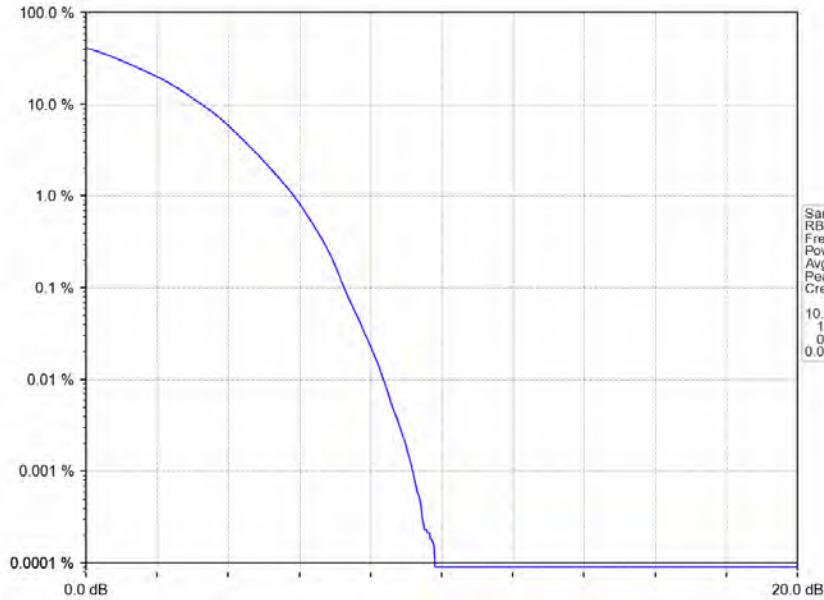
Band66_15MHz_64QAM_LCH_1717.5MHz_RB_75_0_NTNV
