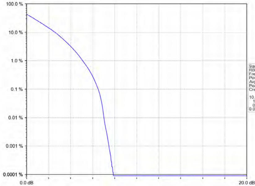
Band66_15MHz_QPSK_HCH_1772.5MHz_RB_75_0_NTNV
