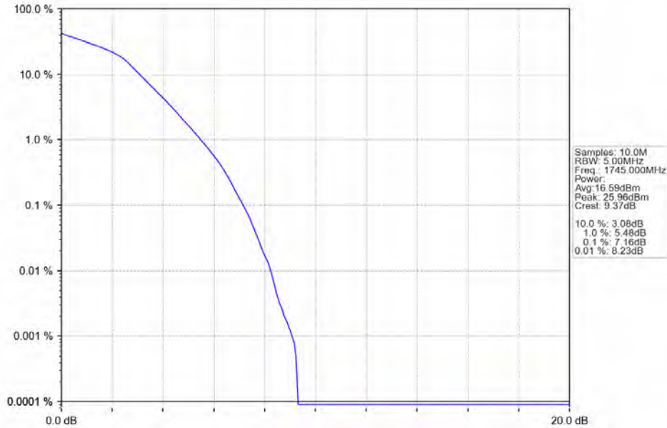
Band66_1.4MHz_16QAM_MCH_1745MHz_RB_6_0_NTNV
