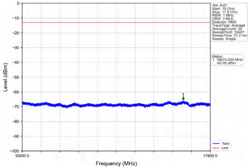
Band66_10MHz_QPSK_LCH_1715MHz_RB_50_0_NTNV
