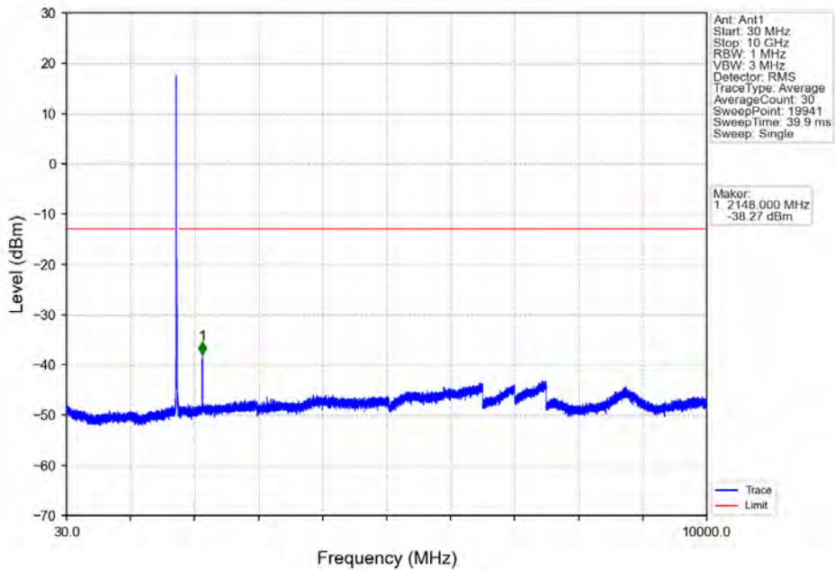
Band66_15MHz_QPSK_MCH_1745MHz_RB_1_0_NTNV
