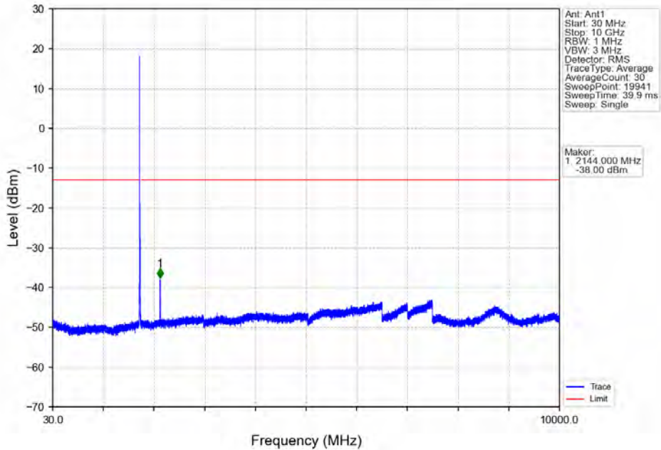
Band66_10MHz_QPSK_MCH_1745MHz_RB_1_0_NTNV
