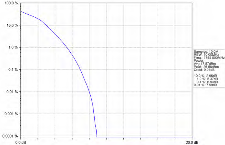
Band66_10MHz_16QAM_MCH_1745MHz_RB_50_0_NTNV
