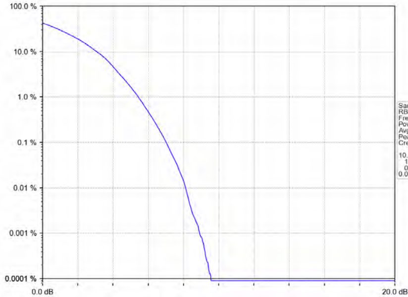
Band66_10MHz_64QAM_HCH_1775MHz_RB_50_0_NTNV
