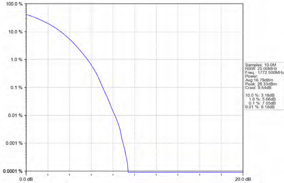
Band66_15MHz_64QAM_HCH_1772.5MHz_RB_75_0_NTNV
