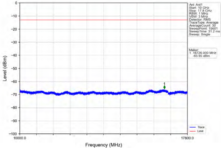
Band66_15MHz_QPSK_LCH_1717.5MHz_RB_75_0_NTNV
