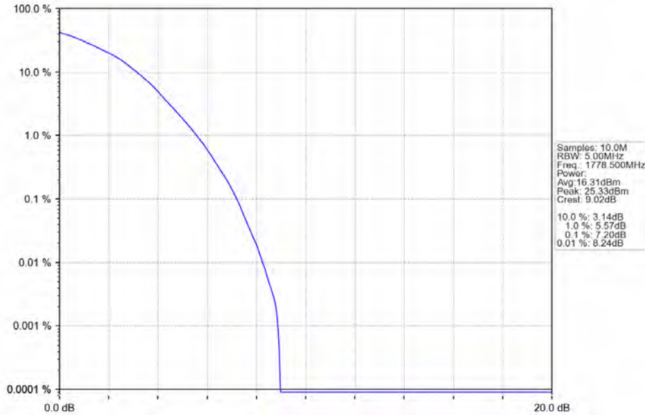
Band66_3MHz_64QAM_HCH_1778.5MHz_RB_15_0_NTNV
