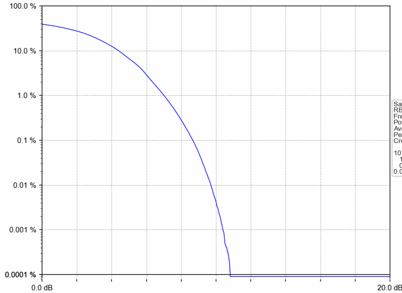
Band41_20MHz_64QAM_LCH_2506MHz_RB_100_0_NTNV
