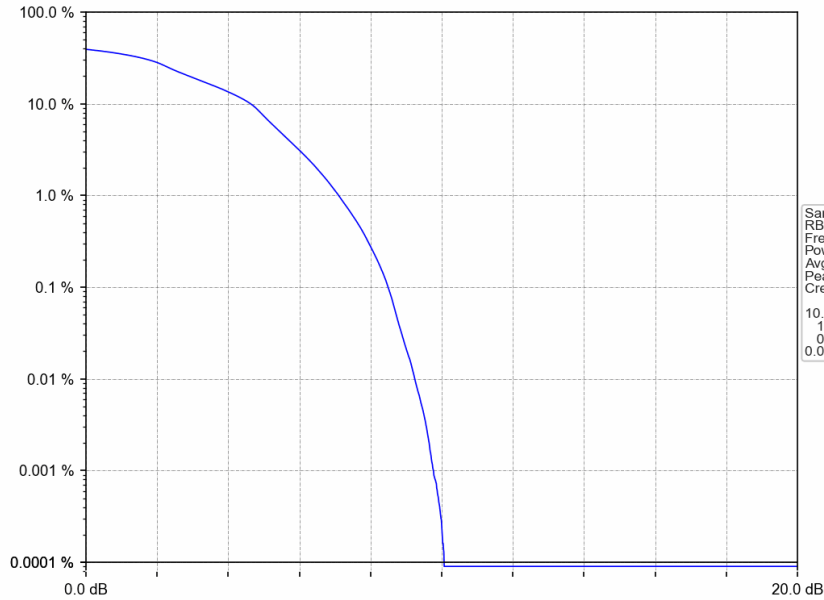
Band41_15MHz_16QAM_MCH_2593MHz_RB_75_0_NTNV
