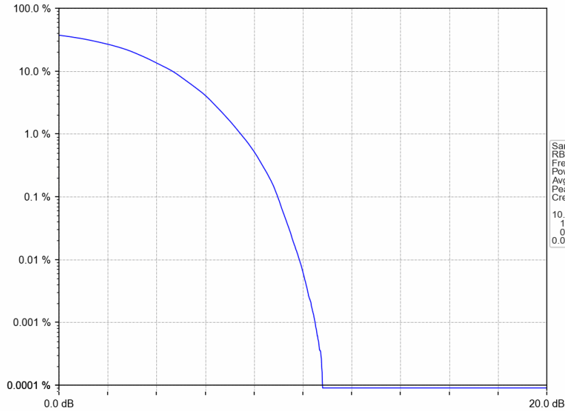
Band41_15MHz_64QAM_LCH_2503.5MHz_RB_75_0_NTNV
