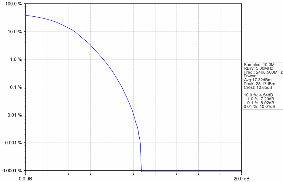
Band41_5MHz_64QAM_LCH_2498.5MHz_RB_25_0_NTNV
