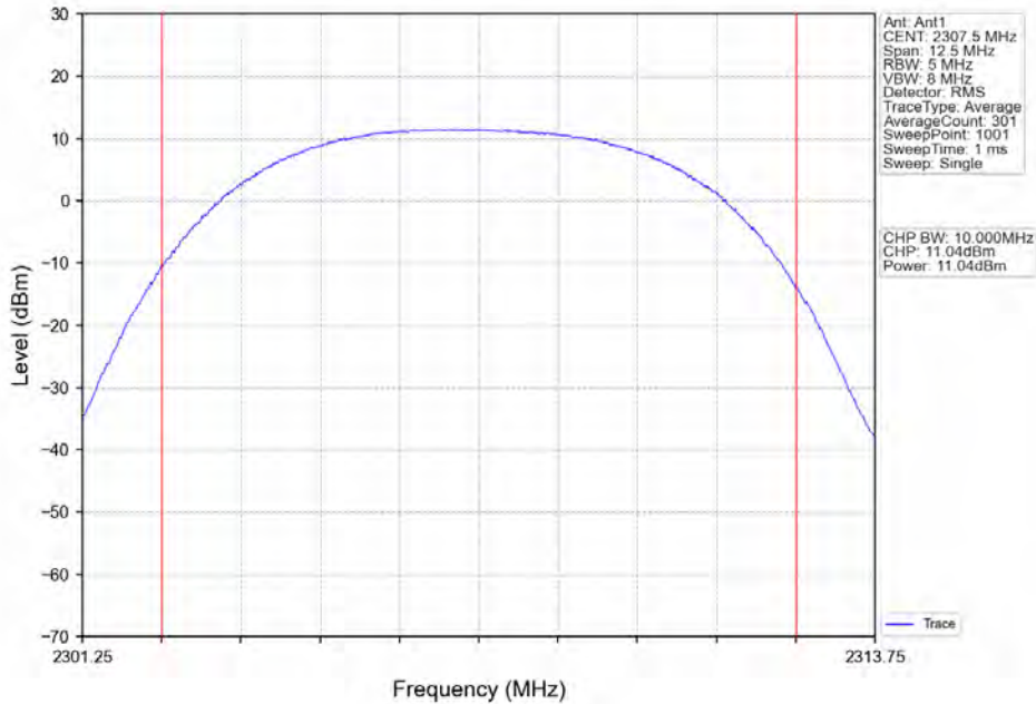
Band30_5MHz_64QAM_LCH_2307.5MHz_RB_12_13_NTNV
