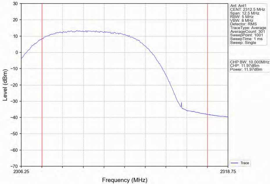
Band30_5MHz_64QAM_HCH_2312.5MHz_RB_1_13_NTNV
