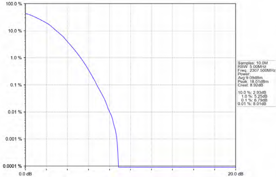
Band30_5MHz_64QAM_LCH_2307.5MHz_RB_25_0_NTNV
