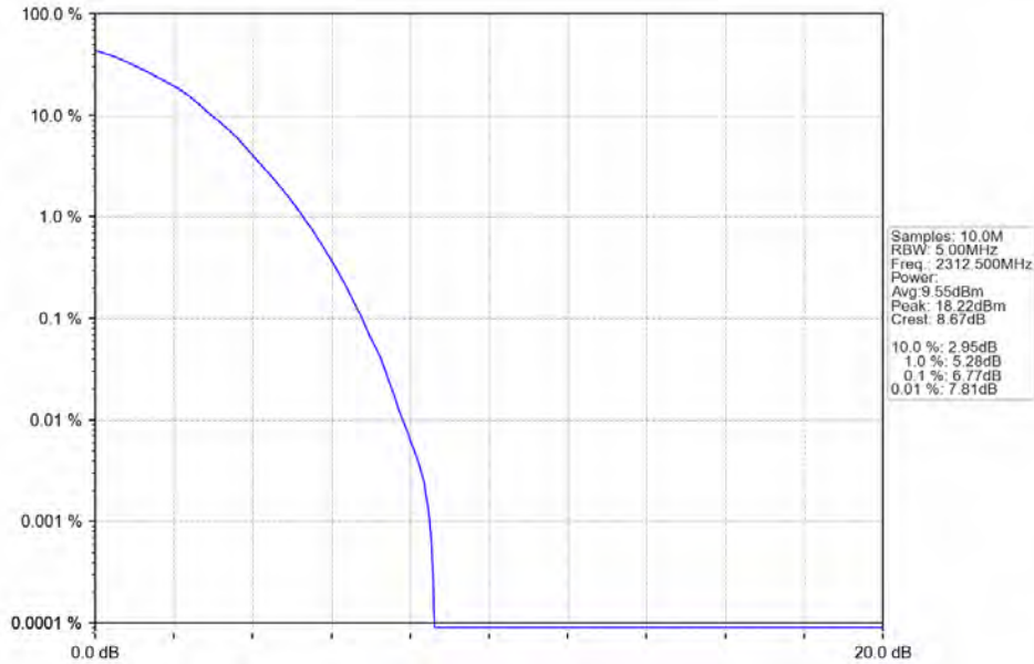
Band30_5MHz_64QAM_HCH_2312.5MHz_RB_25_0_NTNV
