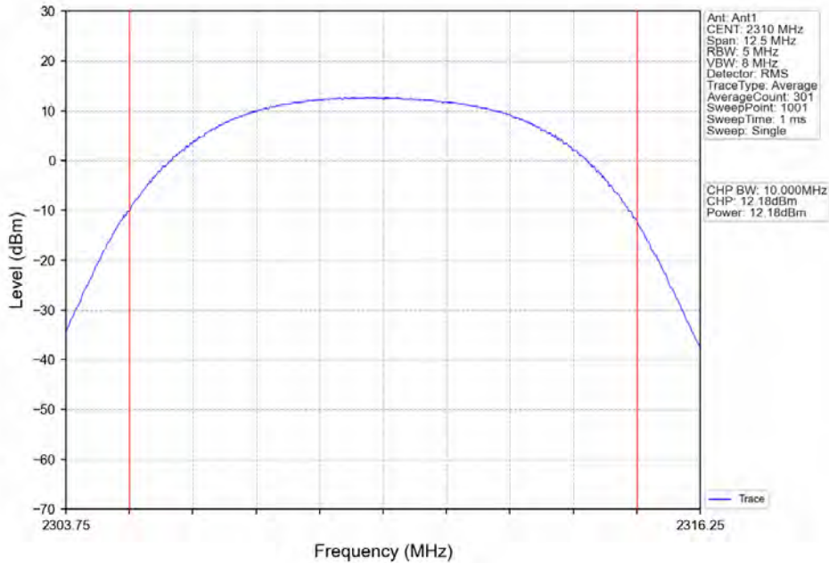
Band30_5MHz_16QAM_MCH_2310MHz_RB_12_13_NTNV
