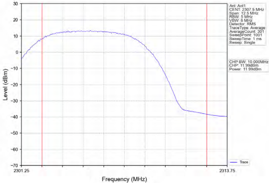
Band30_5MHz_64QAM_LCH_2307.5MHz_RB_1_13_NTNV
