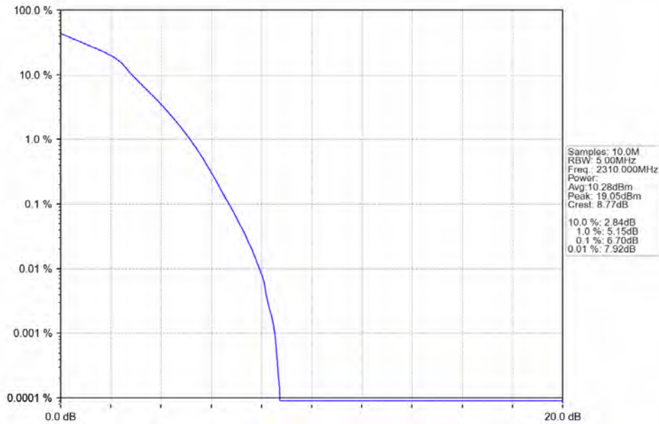
Band30_5MHz_16QAM_MCH_2310MHz_RB_25_0_NTNV
