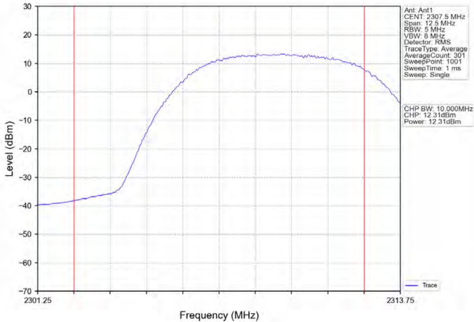
Band30_5MHz_64QAM_LCH_2307.5MHz_RB_12_0_NTNV
