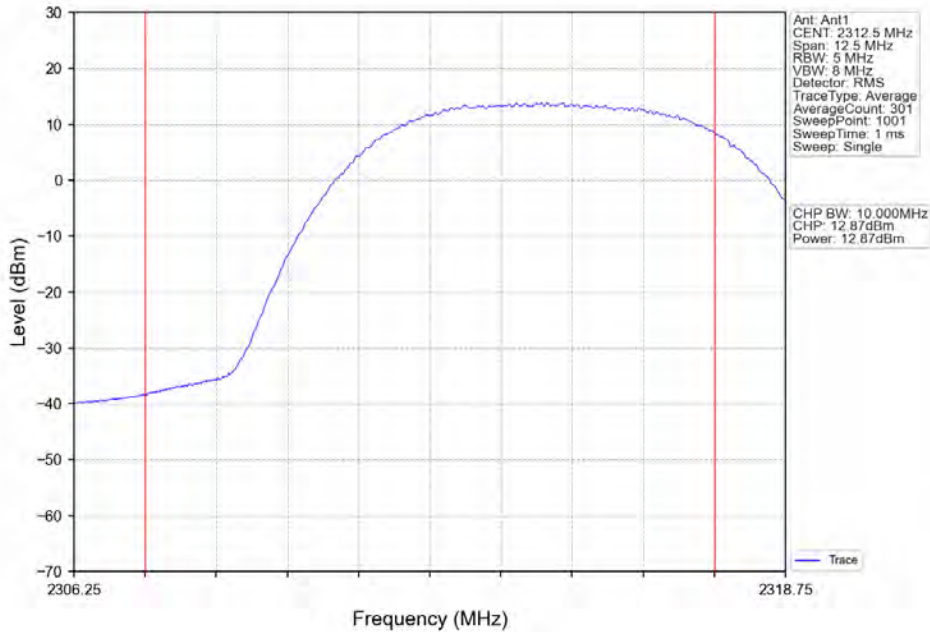
Band30_5MHz_64QAM_HCH_2312.5MHz_RB_12_0_NTNV
