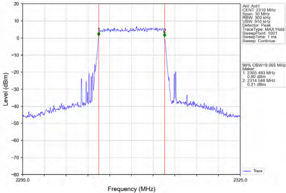
Band30_10MHz_64QAM_MCH_2310MHz_RB_50_0_NTNV
