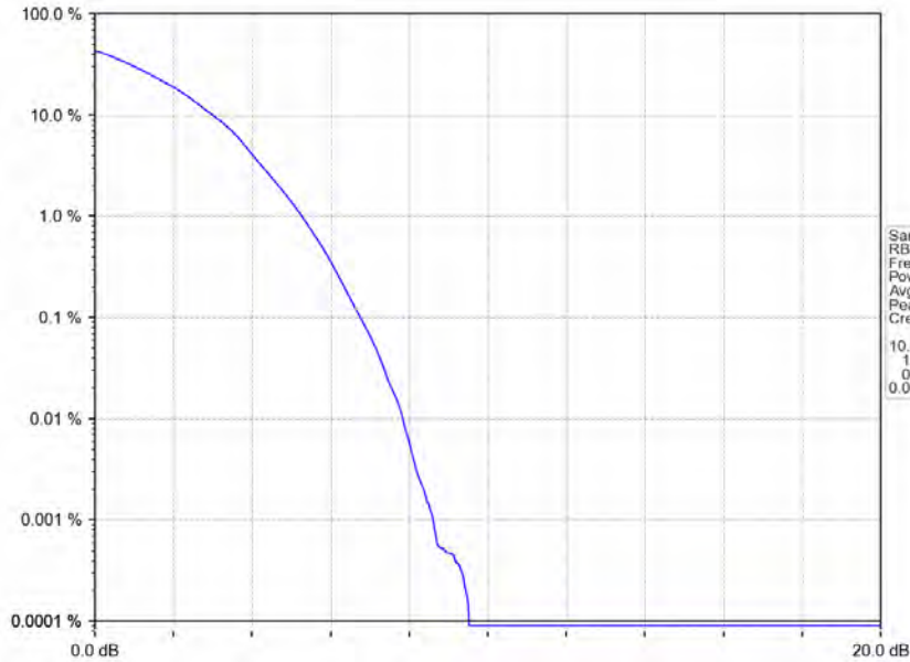
Band30_10MHz_64QAM_MCH_2310MHz_RB_50_0_NTNV
