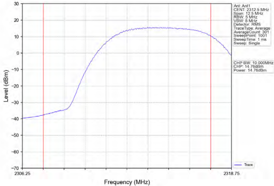
Band30_5MHz_QPSK_HCH_2312.5MHz_RB_12_0_NTNV
