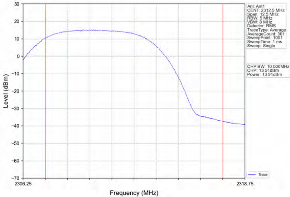
Band30_5MHz_QPSK_HCH_2312.5MHz_RB_1_13_NTNV
