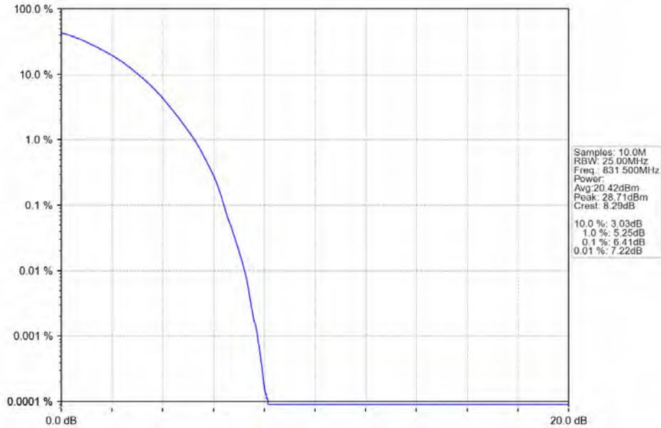
Band26b_15MHz_64QAM_LCH_831.5MHz_RB_75_0_NTNV
