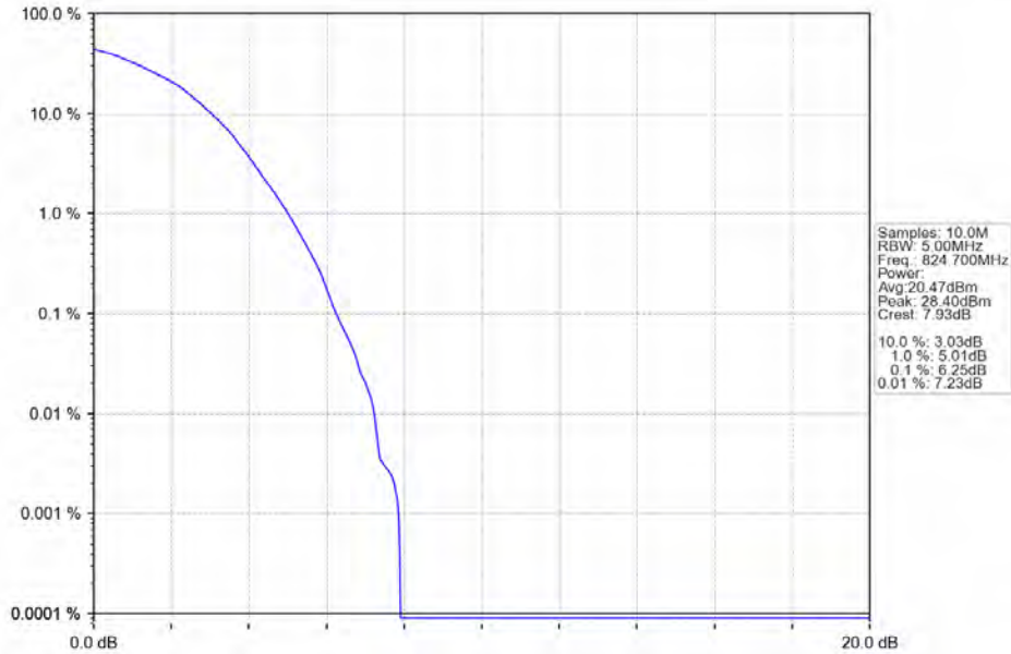
Band26b_1.4MHz_64QAM_LCH_824.7MHz_RB_6_0_NTNV
