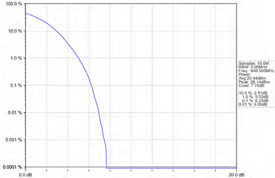
Band26b_5MHz_64QAM_HCH_846.5MHz_RB_25_0_NTNV
