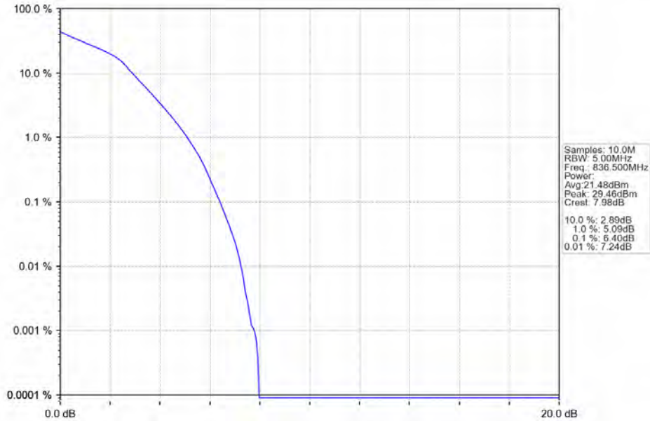
Band26b_3MHz_16QAM_MCH_836.5MHz_RB_15_0_NTNV
