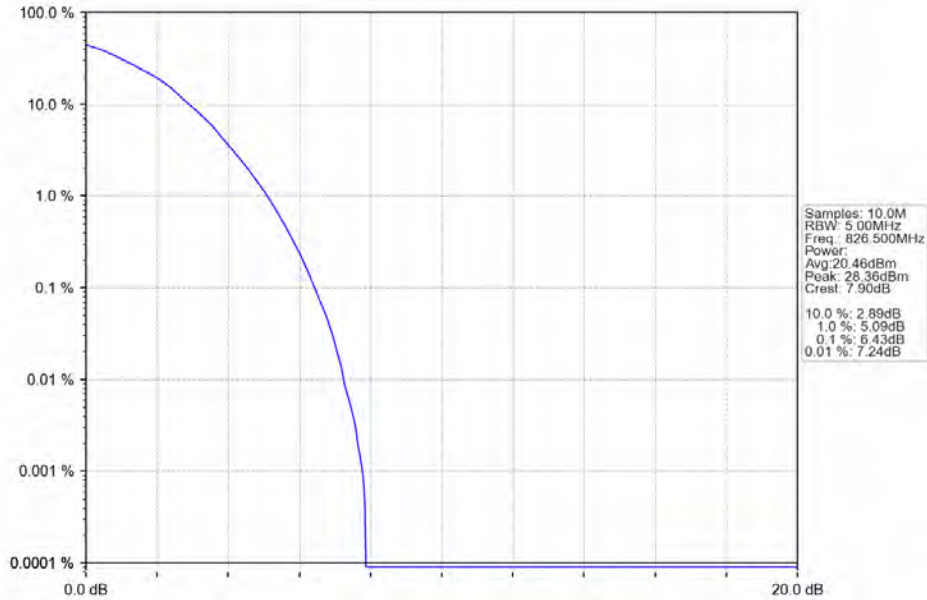
Band26b_5MHz_64QAM_LCH_826.5MHz_RB_25_0_NTNV
