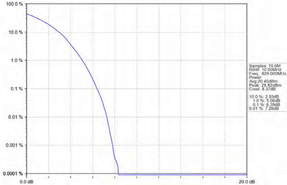
Band26b_10MHz_64QAM_LCH_829MHz_RB_50_0_NTNV
