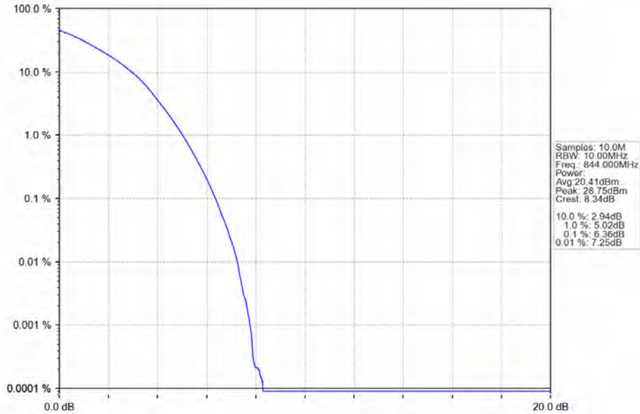
Band26b_10MHz_64QAM_HCH_844MHz_RB_50_0_NTNV
