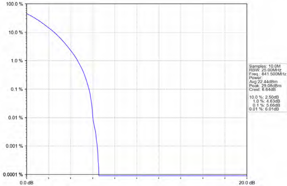
Band26b_15MHz_QPSK_HCH_841.5MHz_RB_75_0_NTNV
