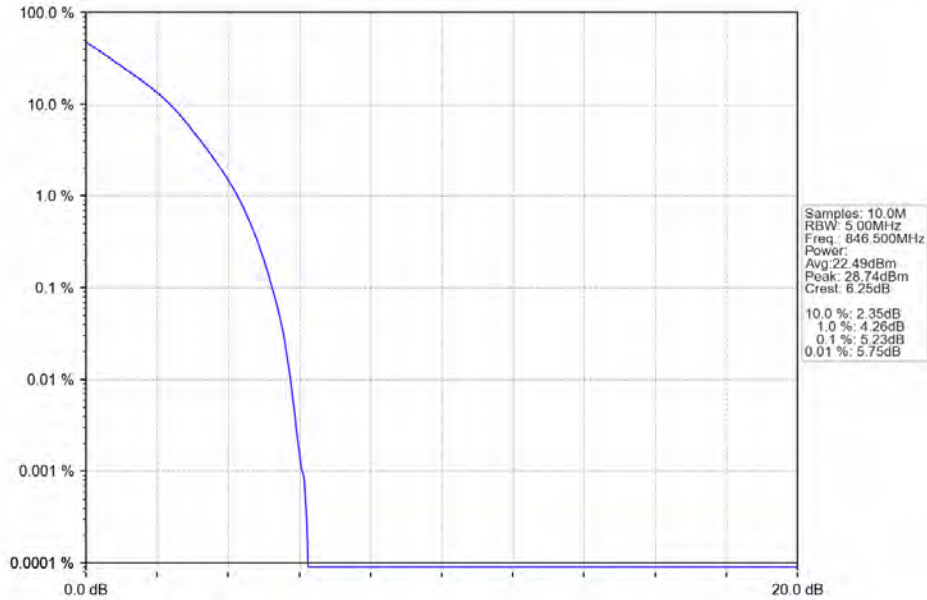
Band26b_5MHz_QPSK_HCH_846.5MHz_RB_25_0_NTNV
