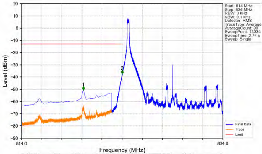
Band26b_10MHz_QPSK_LCH_829MHz_RB_1_0_NTNV
