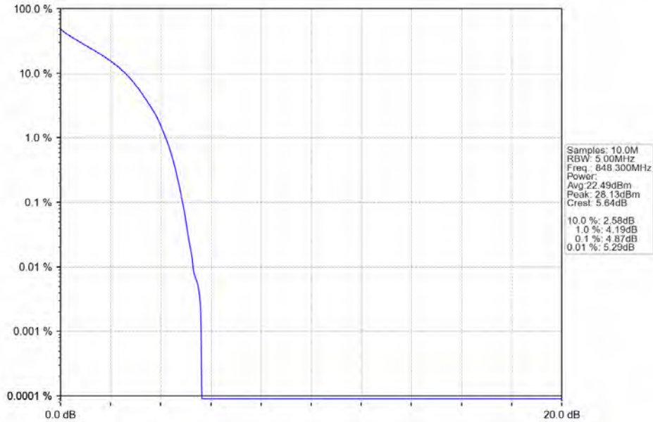
Band26b_1.4MHz_QPSK_HCH_848.3MHz_RB_6_0_NTNV
