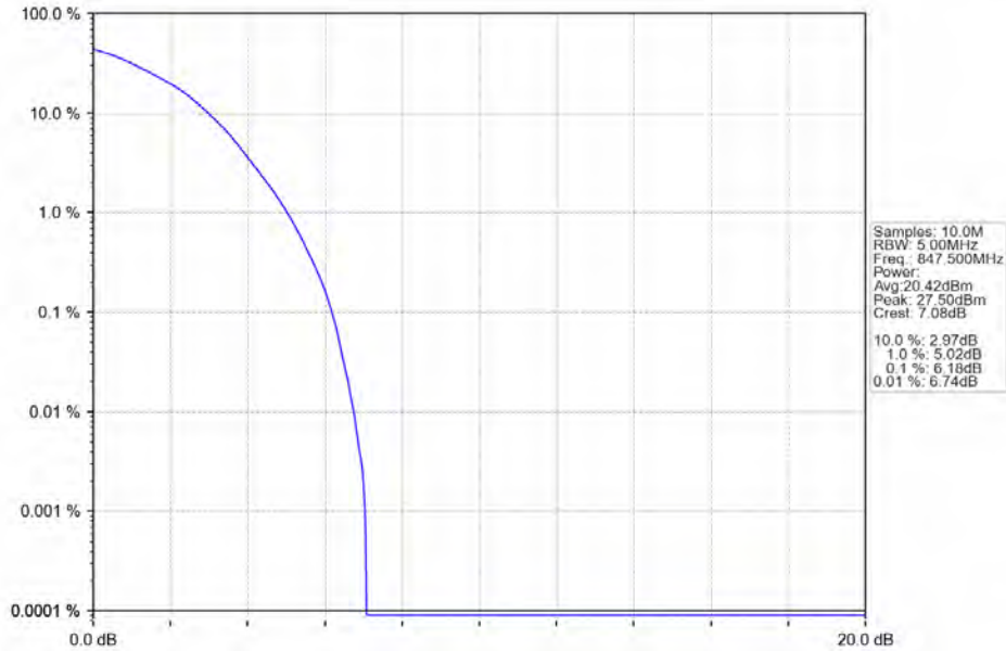
Band26b_3MHz_64QAM_HCH_847.5MHz_RB_15_0_NTNV
