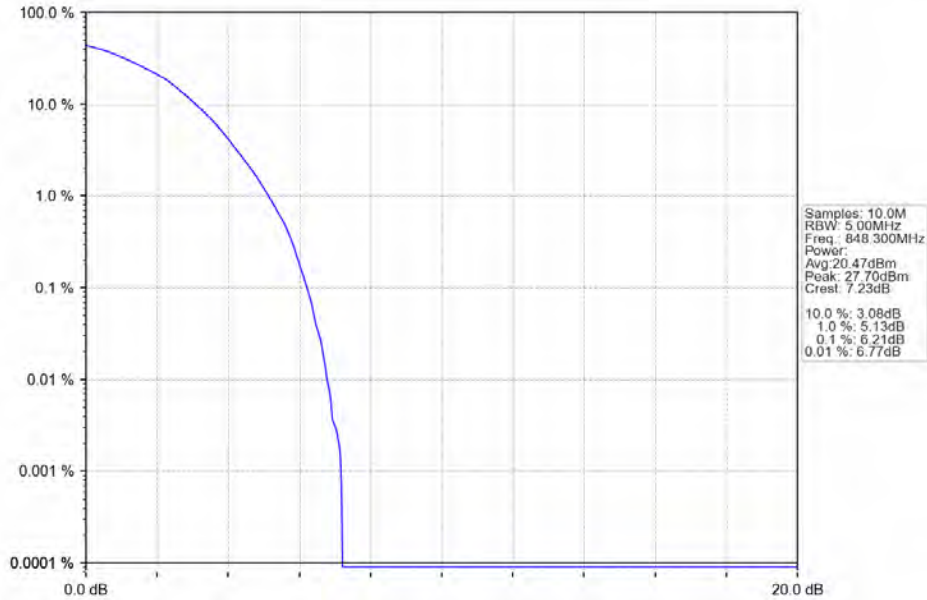
Band26b_1.4MHz_64QAM_HCH_848.3MHz_RB_6_0_NTNV
