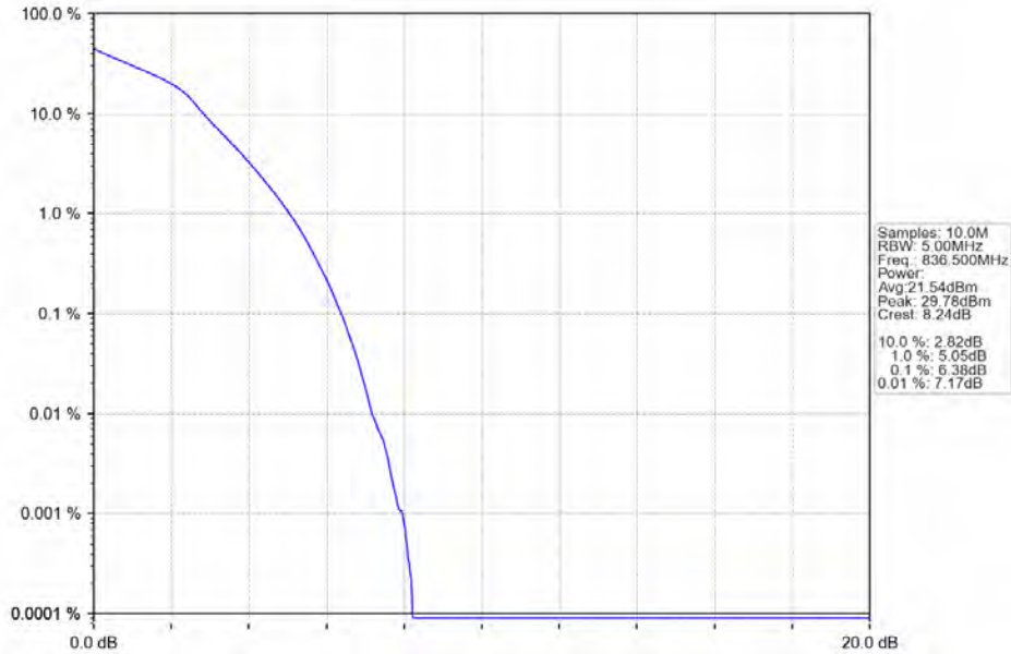
Band26b_5MHz_16QAM_MCH_836.5MHz_RB_25_0_NTNV
