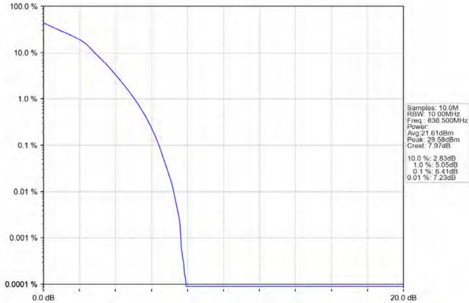
Band26b_10MHz_16QAM_MCH_836.5MHz_RB_50_0_NTNV
