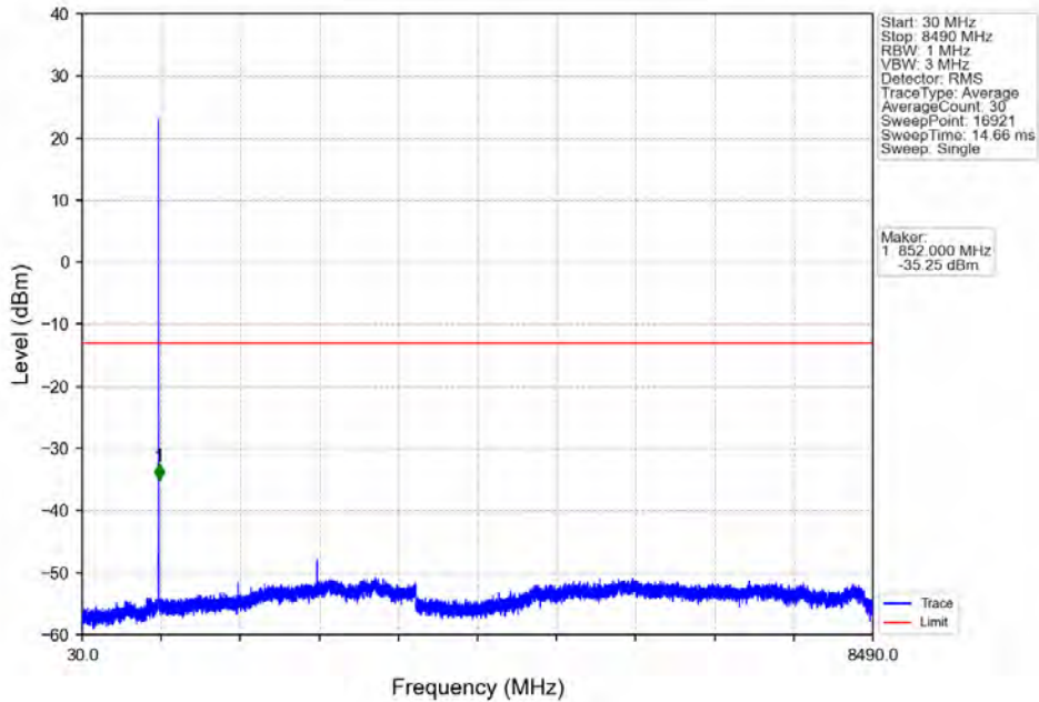
Band26b_1.4MHz_QPSK_HCH_848.3MHz_RB_1_5_NTNV
