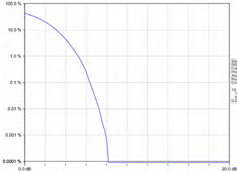
Band26b_15MHz_64QAM_HCH_841.5MHz_RB_75_0_NTNV
