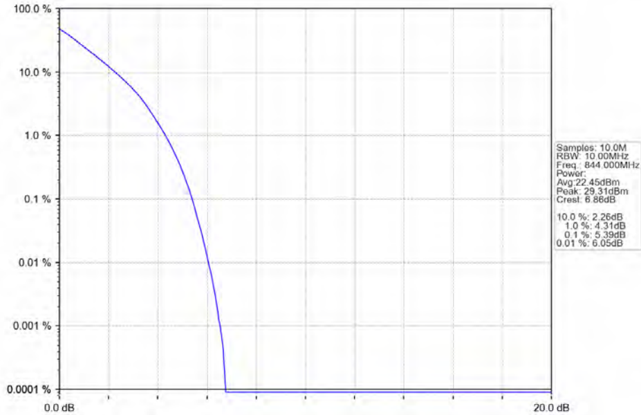
Band26b_10MHz_QPSK_HCH_844MHz_RB_50_0_NTNV
