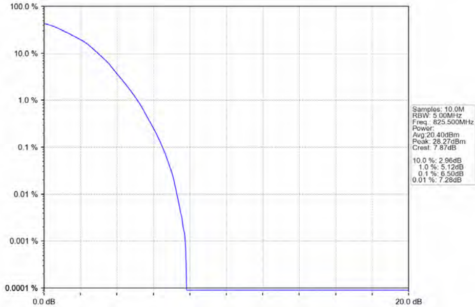
Band26b_3MHz_64QAM_LCH_825.5MHz_RB_15_0_NTNV
