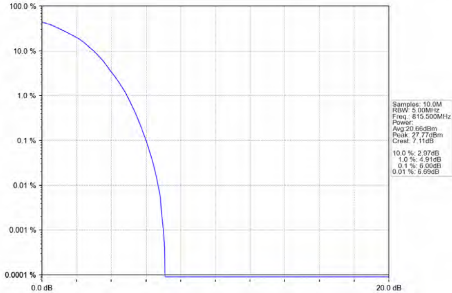
Band26a_3MHz_64QAM_LCH_815.5MHz_RB_15_0_NTNV
