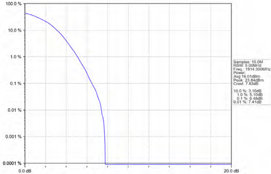
Band25_1.4MHz_64QAM_HCH_1914.3MHz_RB_6_0_NTNV
