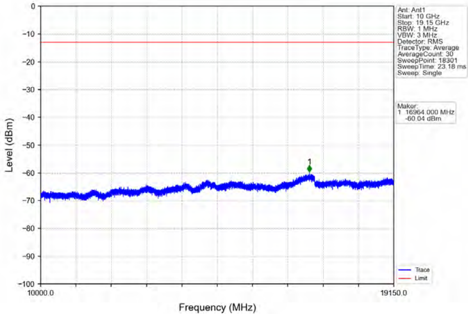
Band25_3MHz_QPSK_LCH_1851.5MHz_RB_15_0_NTNV
