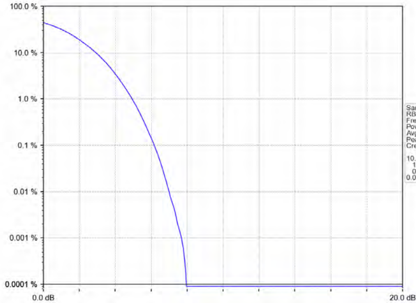
Band25_20MHz_64QAM_HCH_1905MHz_RB_100_0_NTNV
