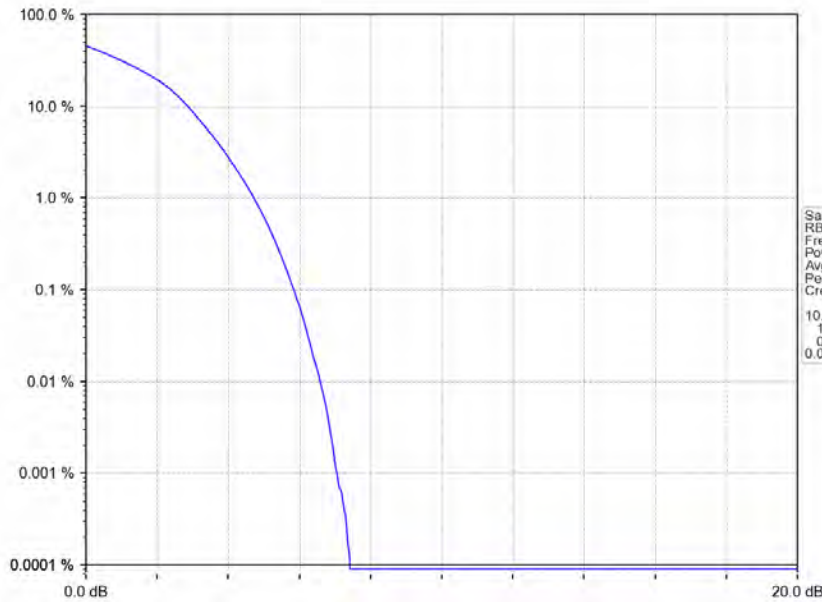
Band25_20MHz_16QAM_MCH_1882.5MHz_RB_100_0_NTNV
