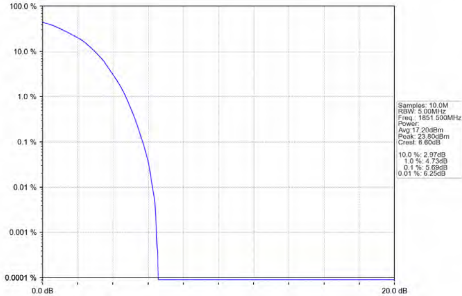
Band25_3MHz_64QAM_LCH_1851.5MHz_RB_15_0_NTNV
