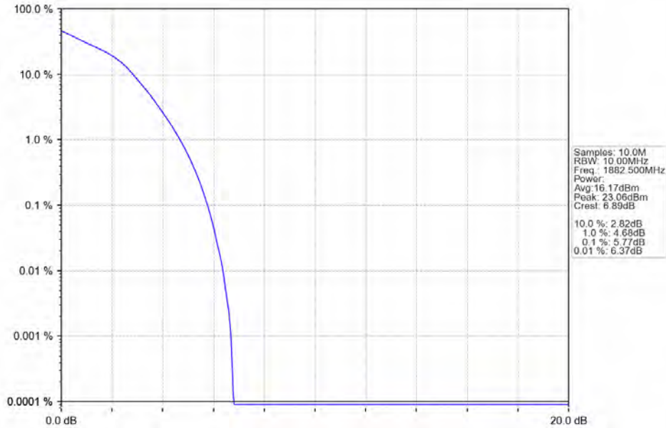
Band25_10MHz_16QAM_MCH_1882.5MHz_RB_50_0_NTNV
