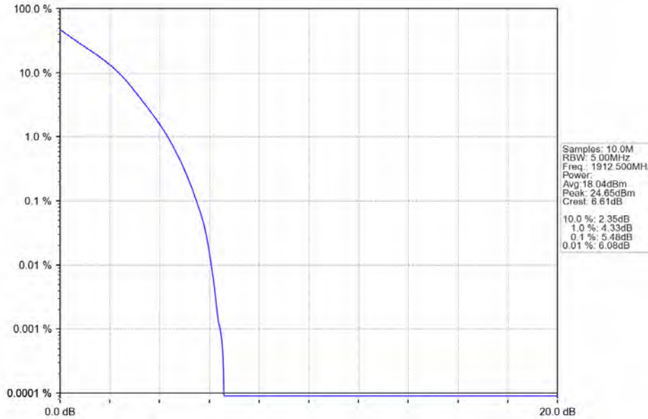
Band25_5MHz_QPSK_HCH_1912.5MHz_RB_25_0_NTNV
