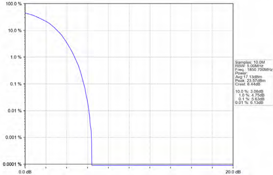
Band25_1.4MHz_64QAM_LCH_1850.7MHz_RB_6_0_NTNV
