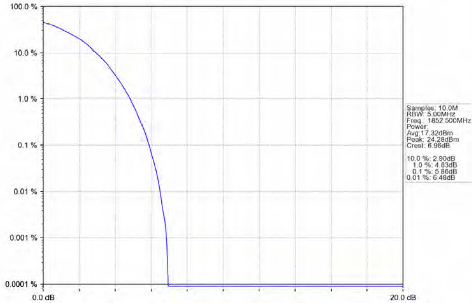
Band25_5MHz_64QAM_LCH_1852.5MHz_RB_25_0_NTNV
