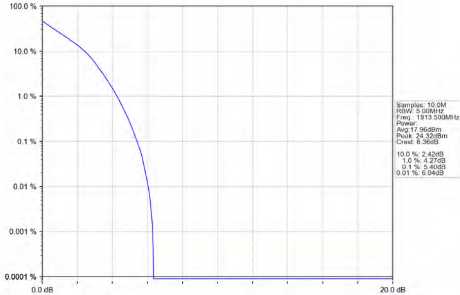
Band25_3MHz_QPSK_HCH_1913.5MHz_RB_15_0_NTNV
