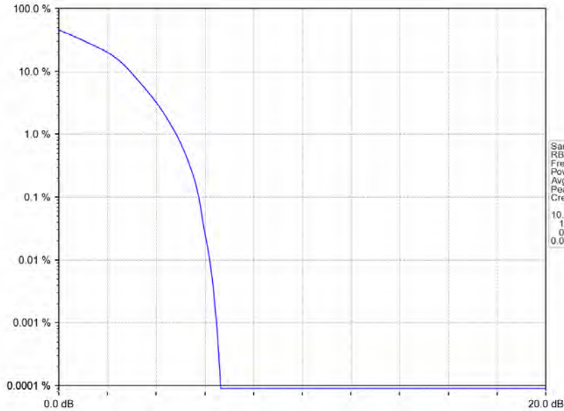
Band25_15MHz_16QAM_MCH_1882.5MHz_RB_75_0_NTNV
