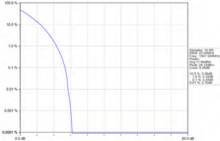
Band25_15MHz_QPSK_HCH_1907.5MHz_RB_75_0_NTNV
