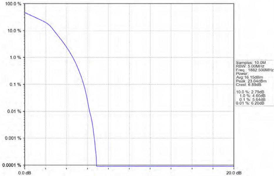
Band25_5MHz_16QAM_MCH_1882.5MHz_RB_25_0_NTNV
