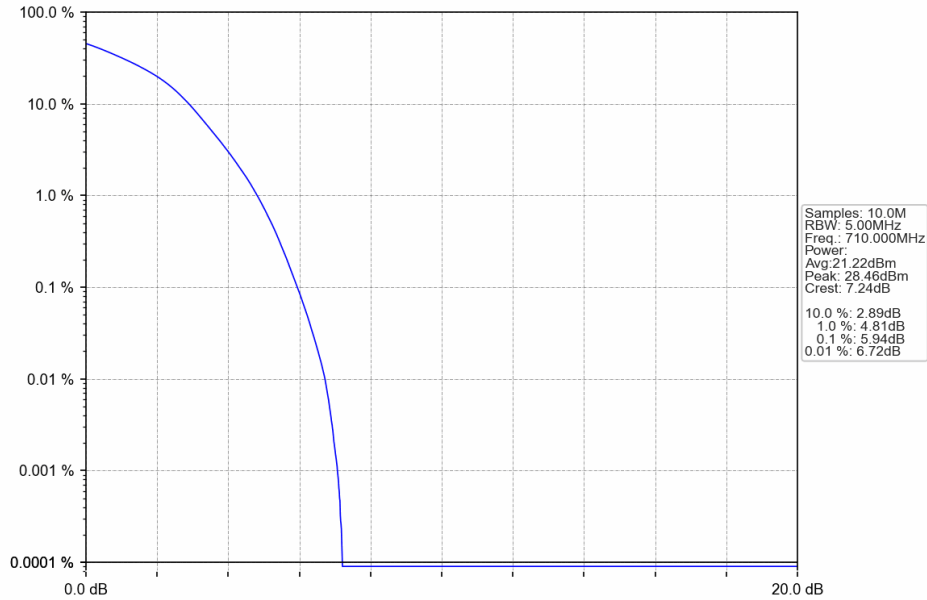
Band17_5MHz_16QAM_MCH_710MHz_RB_25_0_NTNV
