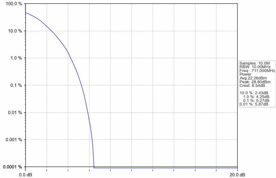
Band17_10MHz_QPSK_HCH_711MHz_RB_50_0_NTNV
