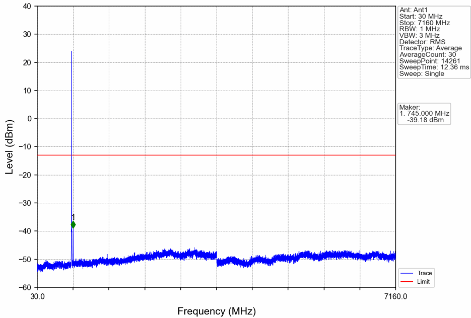
Band17_5MHz_QPSK_HCH_713.5MHz_RB_1_24_NTNV
