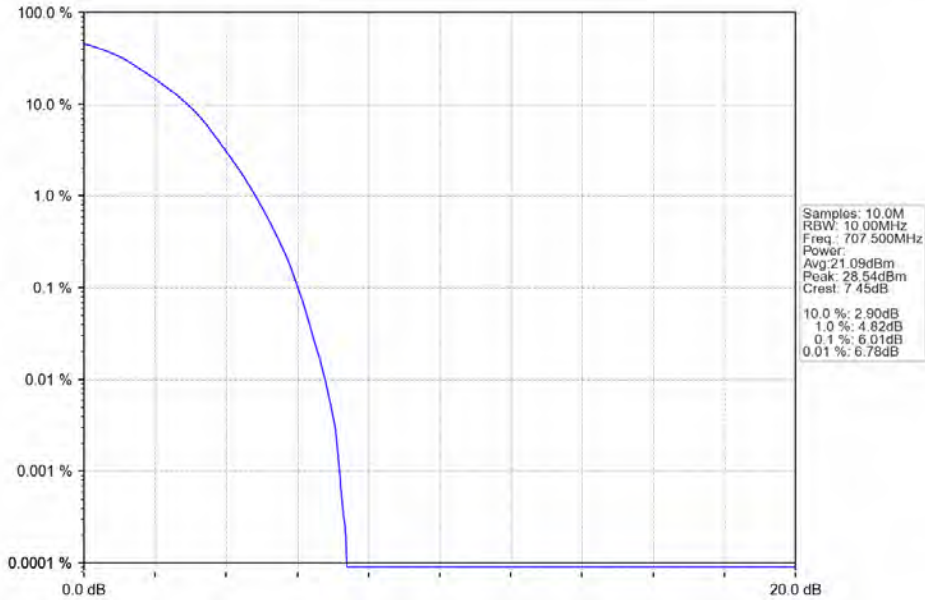
Band12_10MHz_16QAM_MCH_707.5MHz_RB_50_0_NTNV
