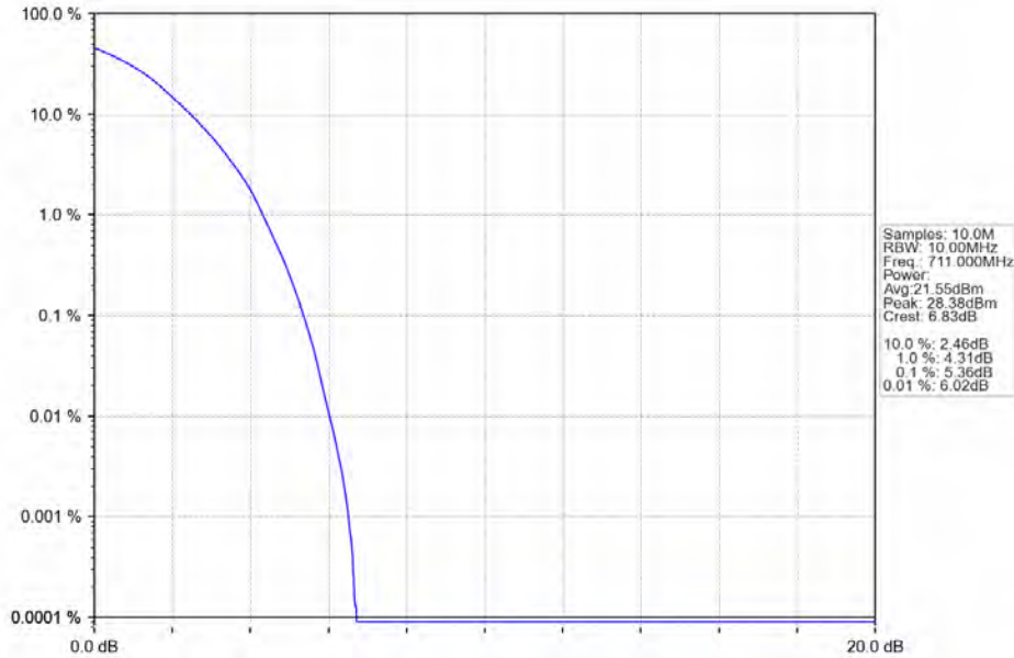
Band12_10MHz_QPSK_HCH_711MHz_RB_50_0_NTNV
