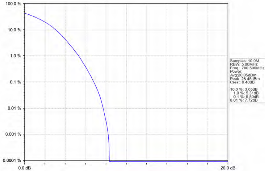
Band12_3MHz_64QAM_LCH_700.5MHz_RB_15_0_NTNV
