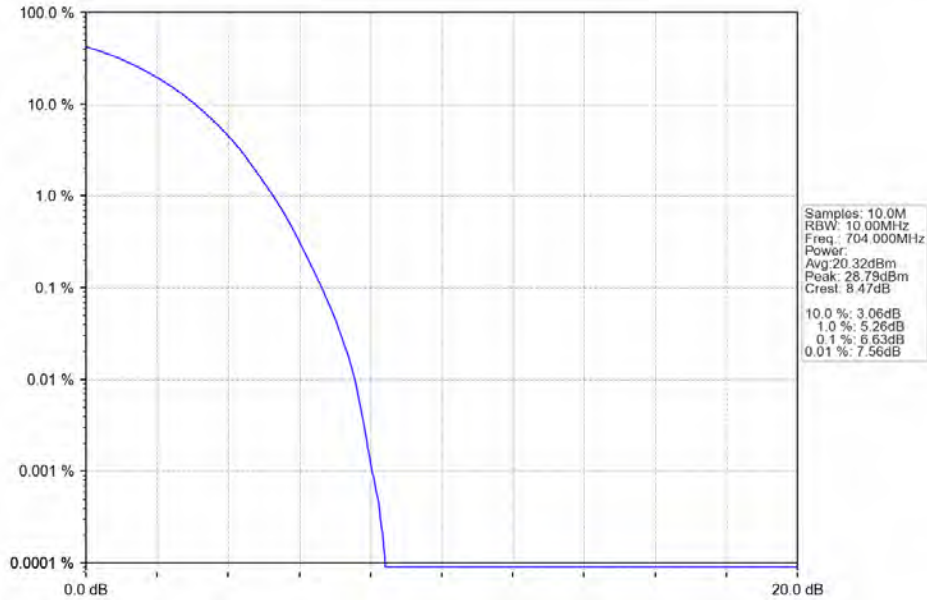
Band12_10MHz_64QAM_LCH_704MHz_RB_50_0_NTNV
