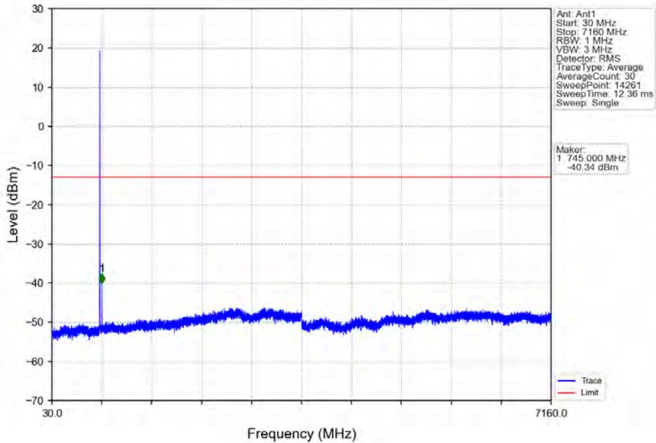
Band12 3MHz QPSK HCH 714.5MHz_RB_1_14_NTNV
