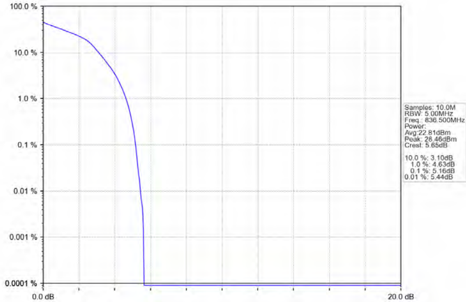
Band5_1.4MHz_16QAM_MCH_836.5MHz_RB_6_0_NTNV
