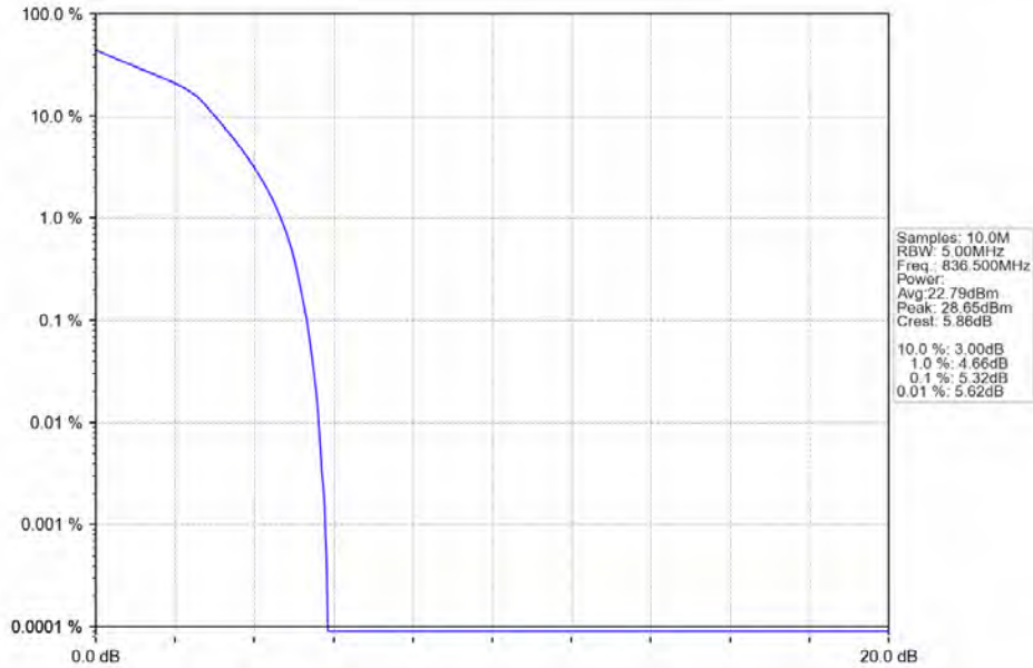
Band5_3MHz_16QAM_MCH_836.5MHz_RB_15_0_NTNV
