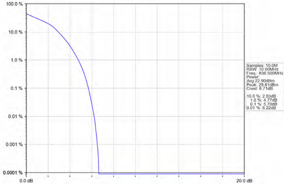
Band5_10MHz_16QAM_MCH_836.5MHz_RB_50_0_NTNV
