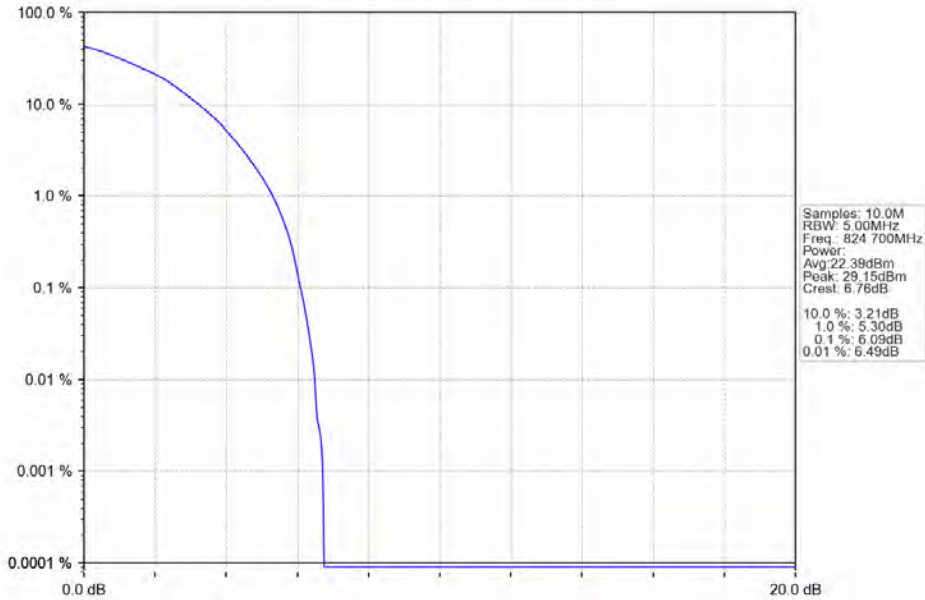
Band5_1.4MHz_64QAM_LCH_824.7MHz_RB_6_0_NTNV
