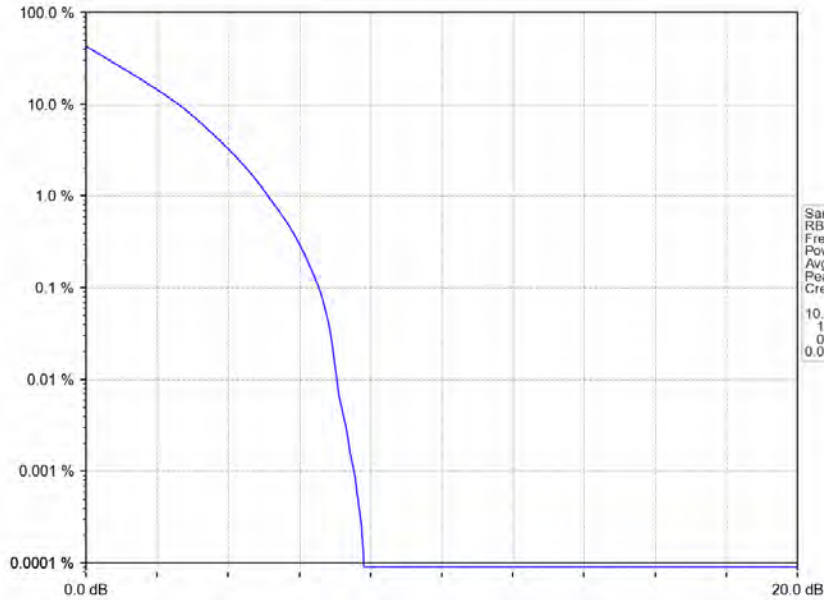
Band4_15MHz_QPSK_HCH_1747.5MHz_RB_75_0_NTNV
