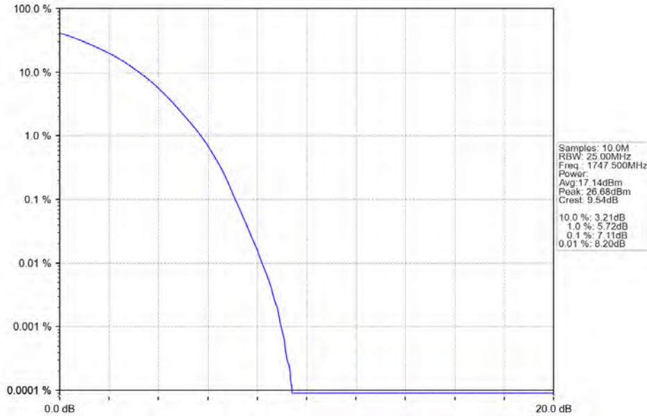
Band4 15MHz_64QAM_HCH_1747.5MHz_RB_75_0_NTNV
