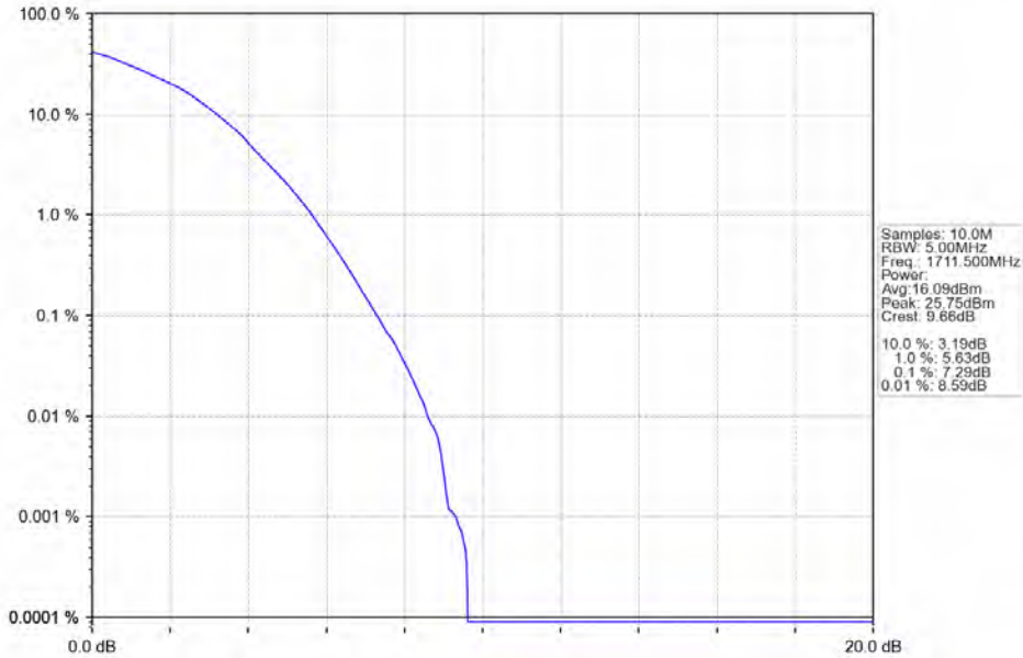
Band4_3MHz_64QAM_LCH_1711.5MHz_RB_15_0_NTNV
