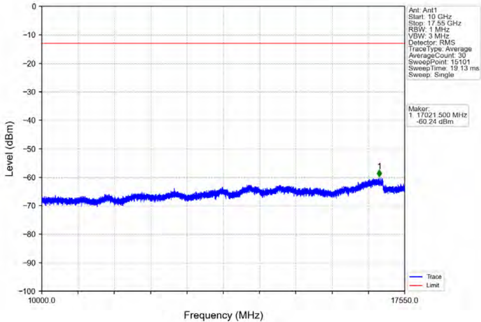
Band4_5MHz_QPSK_LCH_1712.5MHz_RB_25_0_NTNV
