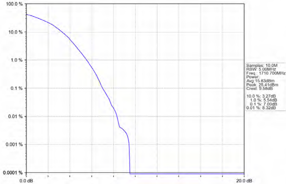
Band4_1.4MHz_64QAM_LCH_1710.7MHz_RB_6_0_NTNV
