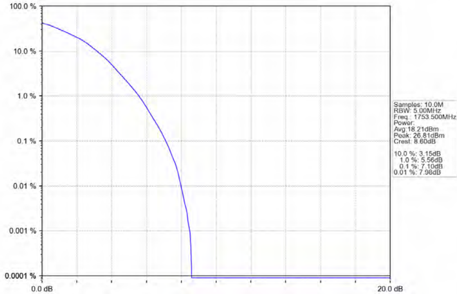
Band4_3MHz_64QAM_HCH_1753.5MHz_RB_15_0_NTNV
