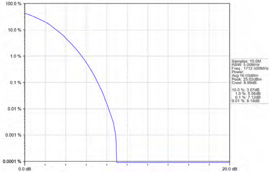
Band4_5MHz_64QAM_LCH_1712.5MHz_RB_25_0_NTNV
