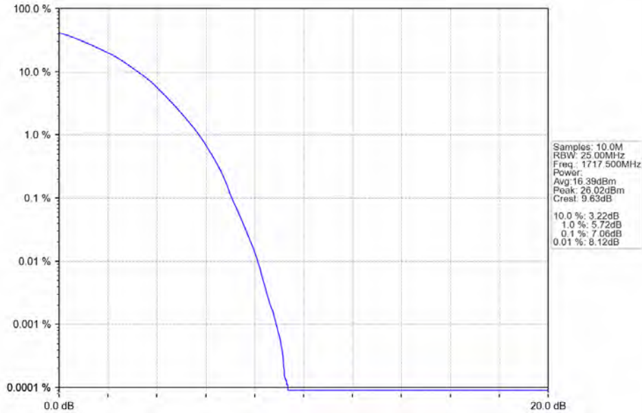
Band4_15MHz_64QAM_LCH_1717.5MHz_RB_75_0_NTNV
