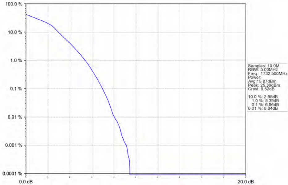
Band4_5MHz_16QAM_MCH_1732.5MHz_RB_25_0_NTNV
