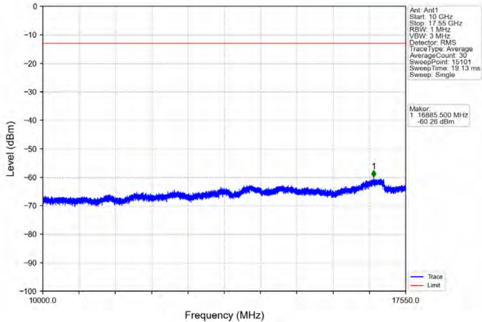
Band4_15MHz_QPSK_LCH_1717.5MHz_RB_75_0_NTNV
