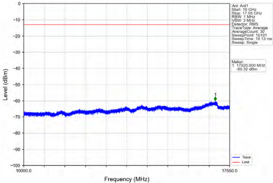
Band4_3MHz_QPSK_LCH_1711.5MHz_RB_15_0_NTNV
