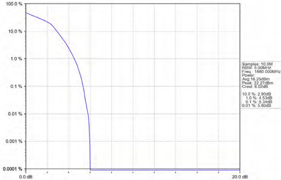
Band2_1.4MHz_16QAM_MCH_1880MHz_RB_6_0_NTNV
