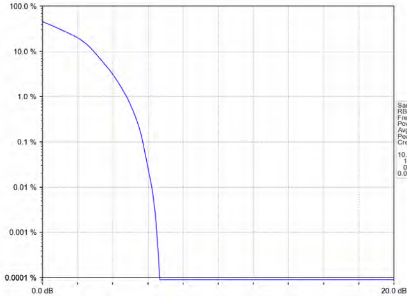
Band2_15MHz_16QAM_MCH_1880MHz_RB_75_0_NTNV
