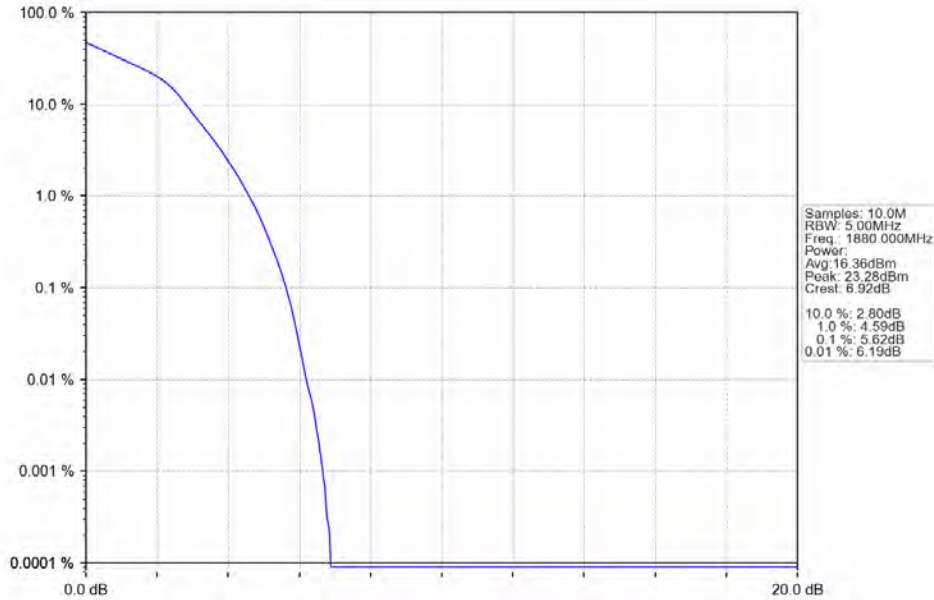
Band2_5MHz_16QAM_MCH_1880MHz_RB_25_0_NTNV
