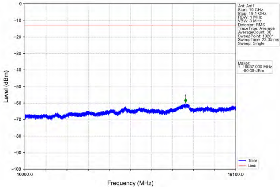
Band2_1.4MHz_QPSK_LCH_1850.7MHz_RB_6_0_NTNV
