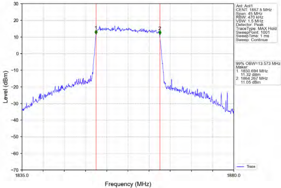
Band2_15MHz_QPSK_LCH_1857.5MHz_RB_75_0_NTNV
