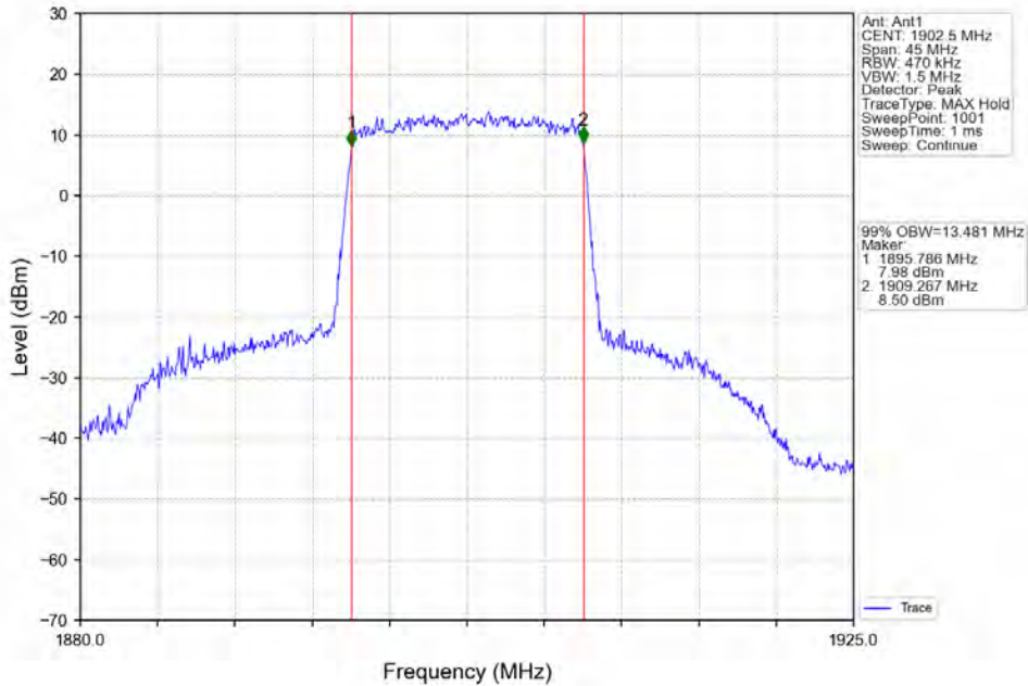
Band2_15MHz_16QAM_HCH_1902.5MHz_RB_75_0_NTNV
