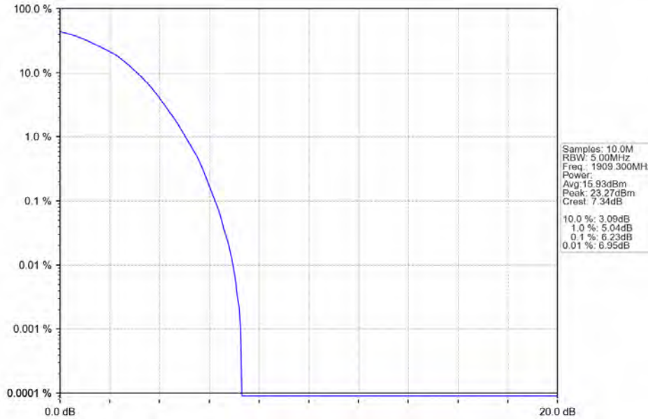
Band2_1.4MHz_64QAM_HCH_1909.3MHz_RB_6_0_NTNV
