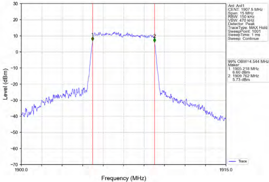
Band2_5MHz_64QAM_HCH_1907.5MHz_RB_25_0_NTNV
