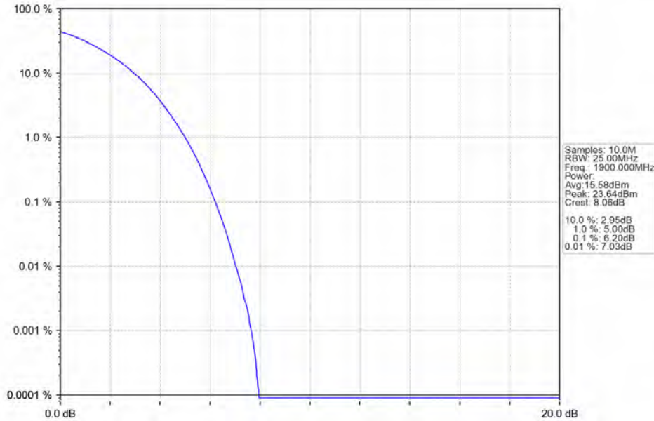
Band2_20MHz_64QAM_HCH_1900MHz_RB_100_0_NTNV
