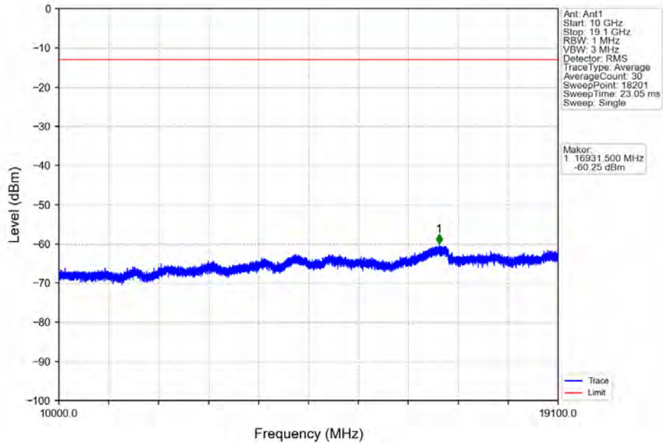
Band2_3MHz_QPSK_LCH_1851.5MHz_RB_15_0_NTNV
