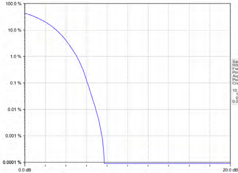
Band2_15MHz_64QAM_HCH_1902.5MHz_RB_75_0_NTNV
