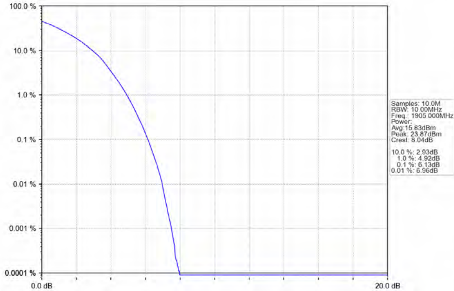
Band2_10MHz_64QAM_HCH_1905MHz_RB_50_0_NTNV
