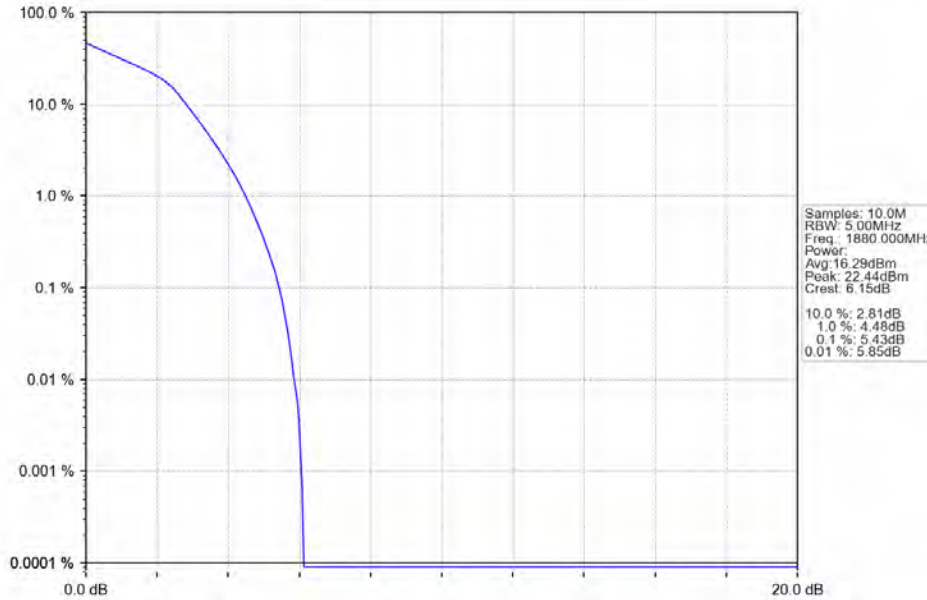
Band2_3MHz_16QAM_MCH_1880MHz_RB_15_0_NTNV
