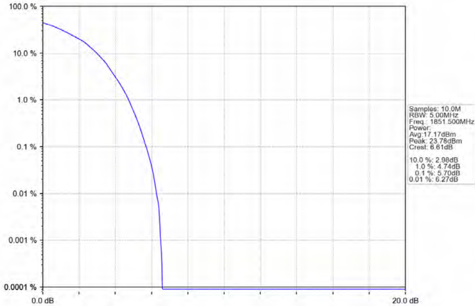
Band2_3MHz_64QAM_LCH_1851.5MHz_RB_15_0_NTNV
