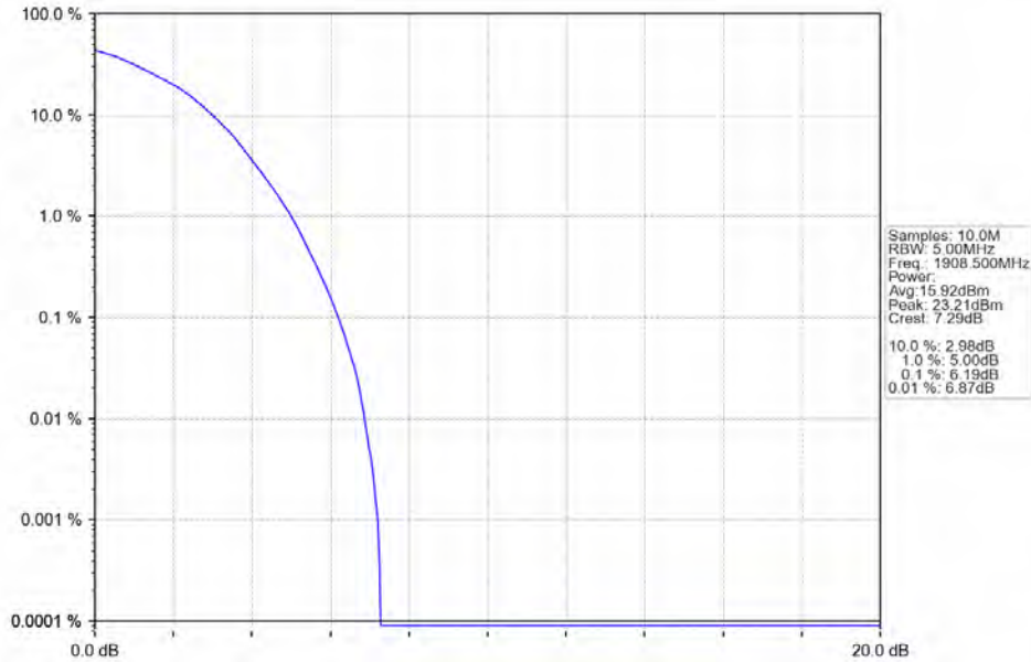
Band2_3MHz_64QAM_HCH_1908.5MHz_RB_15_0_NTNV
