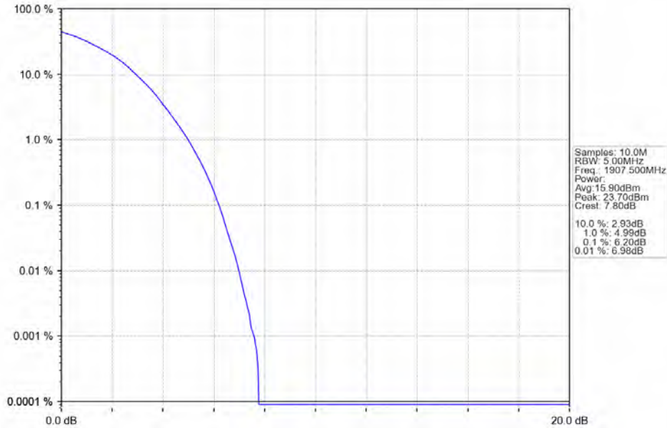
Band2_5MHz_64QAM_HCH_1907.5MHz_RB_25_0_NTNV
