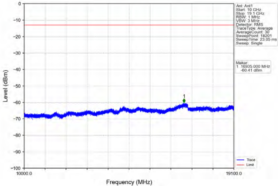
Band2_5MHz_QPSK_LCH_1852.5MHz_RB_25_0_NTNV
