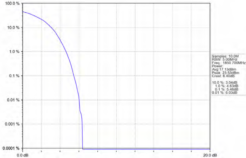
Band2_1.4MHz_64QAM_LCH_1850.7MHz_RB_6_0_NTNV
