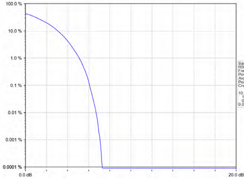
Band2_15MHz_64QAM_LCH_1857.5MHz_RB_75_0_NTNV
