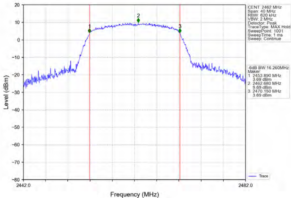
802.11g_HCH_2462MHz_Ant7 (SISO) NTN
