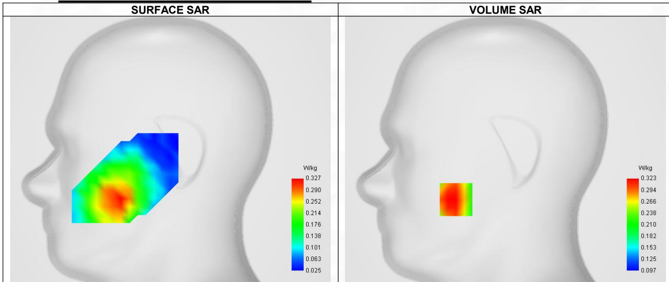
Maximum location: X=-48.00, Y=-49.00 ; SAR Peak: 0.42 W/kg
