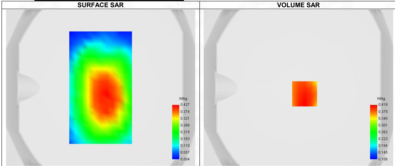
Maximum location: X=8.00, Y=-8.00 ; SAR Peak: 0.52 W/kg
