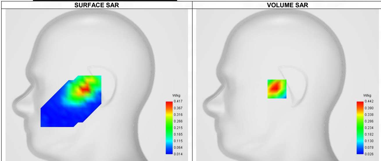
Maximum location: X=-18.00, Y=-7.00 ; SAR Peak: 0.86 W/kg
