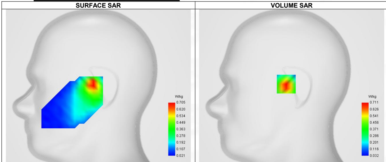
Maximum location: X=-9.00, Y=3.00 ; SAR Peak: 1.09 W/kg
