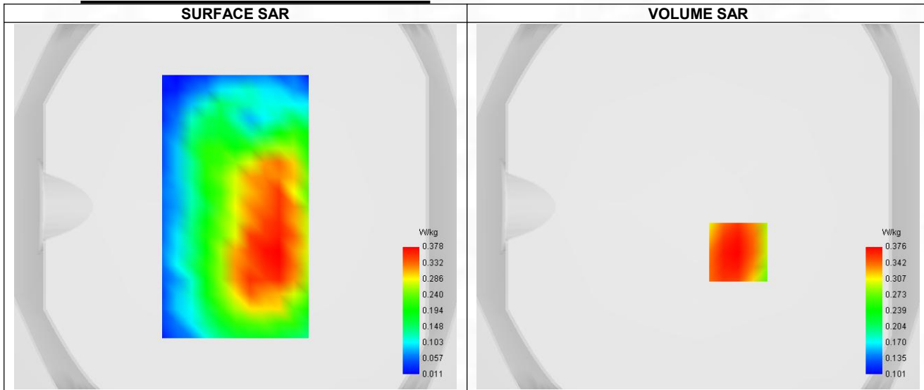
Maximum location: X=22.00, Y=-25.00 ; SAR Peak: 0.47 W/kg
