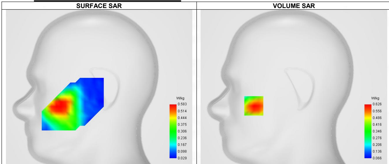
Maximum location: X=-67.00, Y=-31.00 ; SAR Peak: 0.91 W/kg
