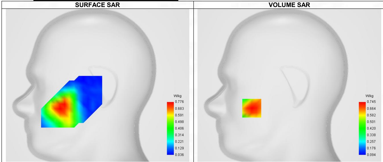
Maximum location: X=-64.00, Y=-39.00 ; SAR Peak: 0.97 W/kg
