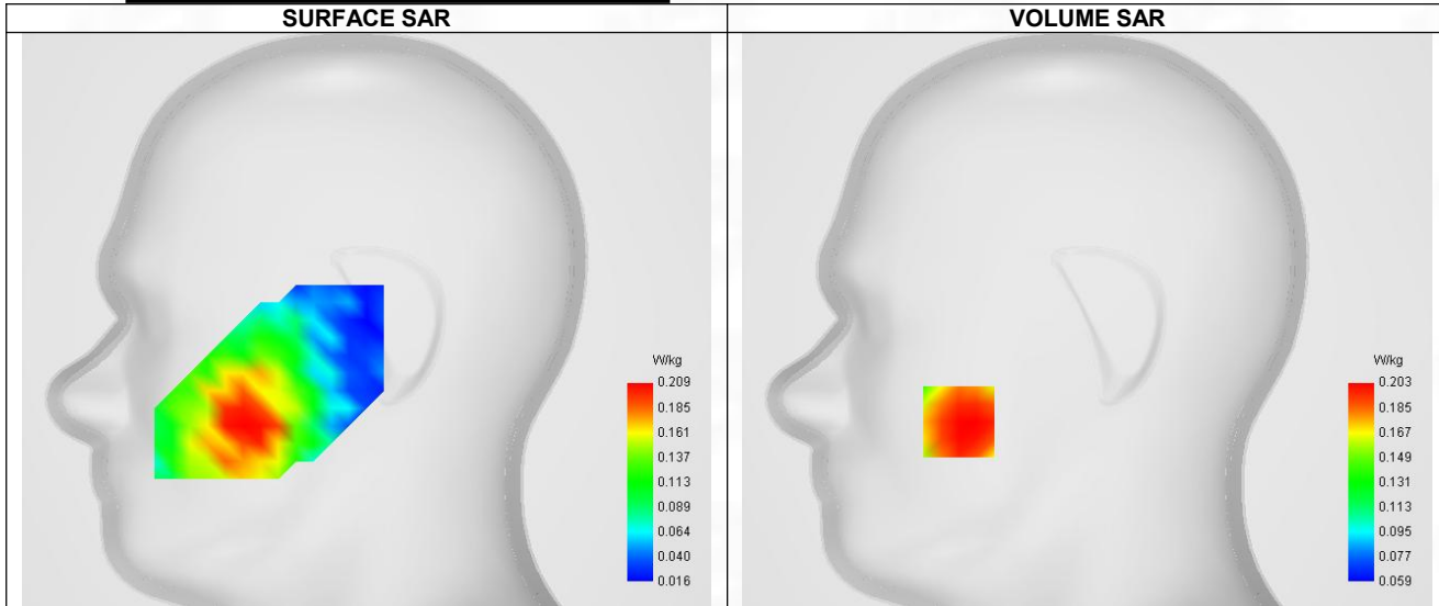
Maximum location: X=-58.00, Y=-46.00 ; SAR Peak: 0.27 W/kg
