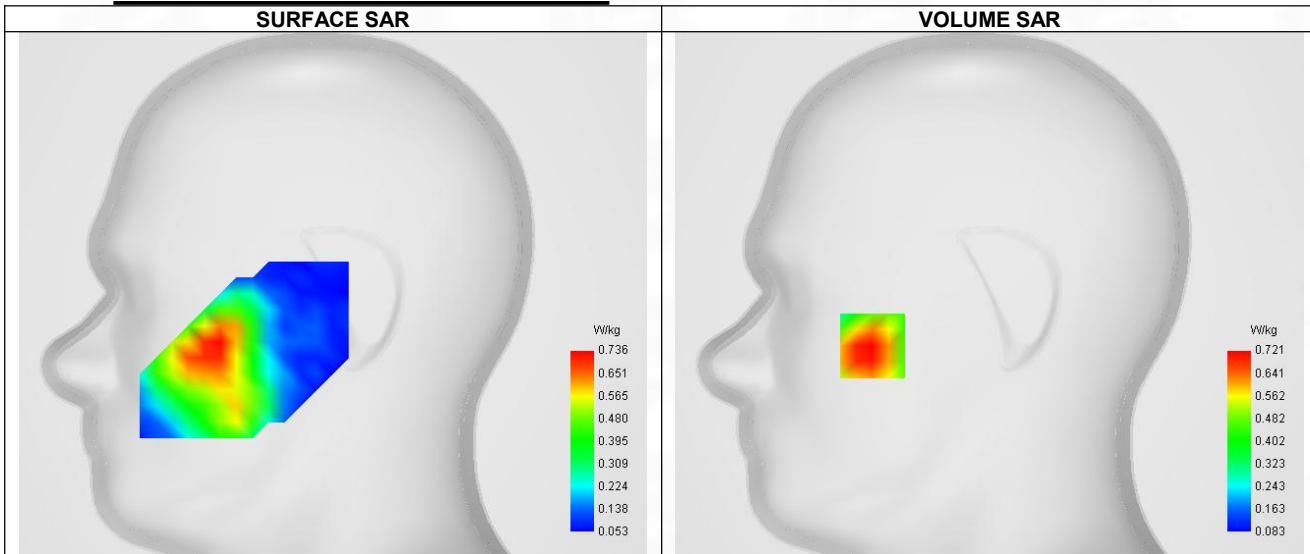
Maximum location: X=-58.00, Y=-26.00 ; SAR Peak: 0.98 W/kg
