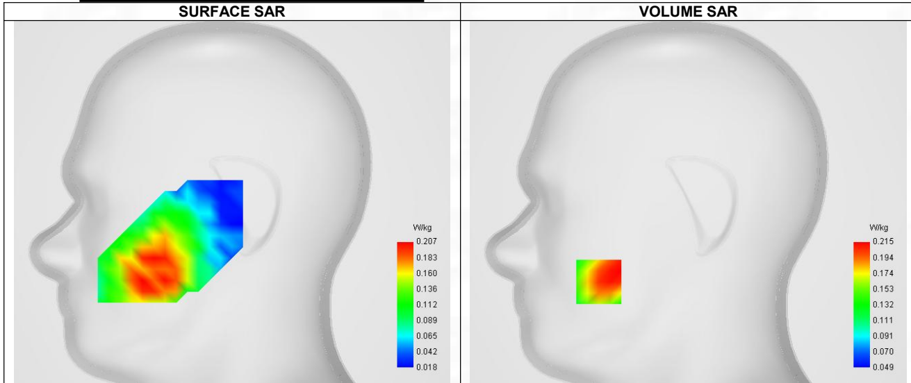
Maximum location: X=-64.00, Y=-57.00 ; SAR Peak: 0.28 W/kg
