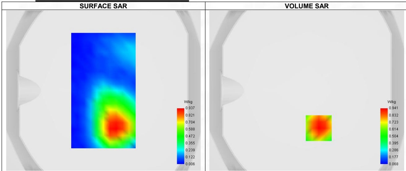
Maximum location: X=15.00, Y=-47.00 ; SAR Peak: 1.32 W/kg
