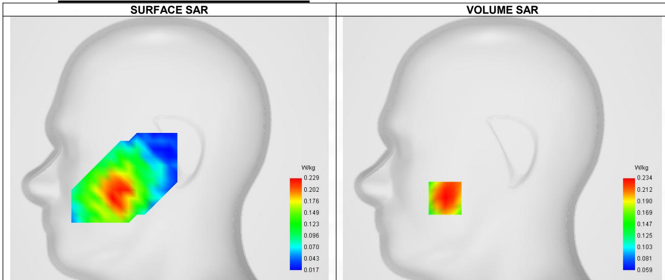
Maximum location: X=-56.00, Y=-48.00 ; SAR Peak: 0.31 W/kg
