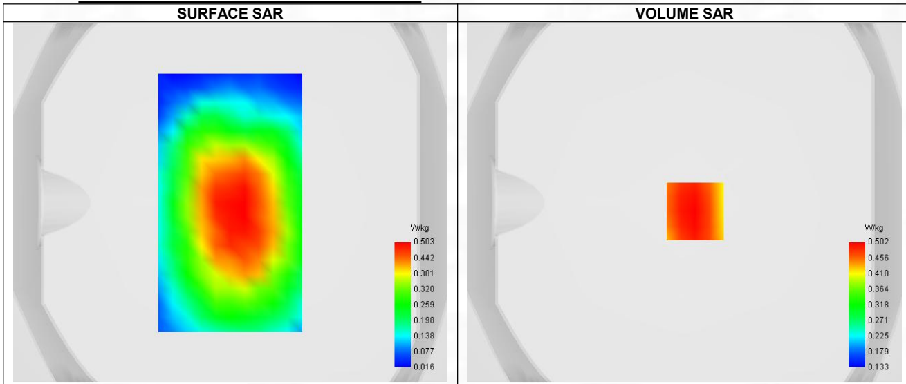
Maximum location: X=6.00, Y=-5.00 ; SAR Peak: 0.62 W/kg
