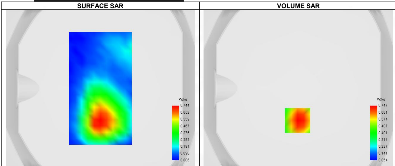
Maximum location: X=-1.00, Y=-41.00 ; SAR Peak: 1.09 W/kg
