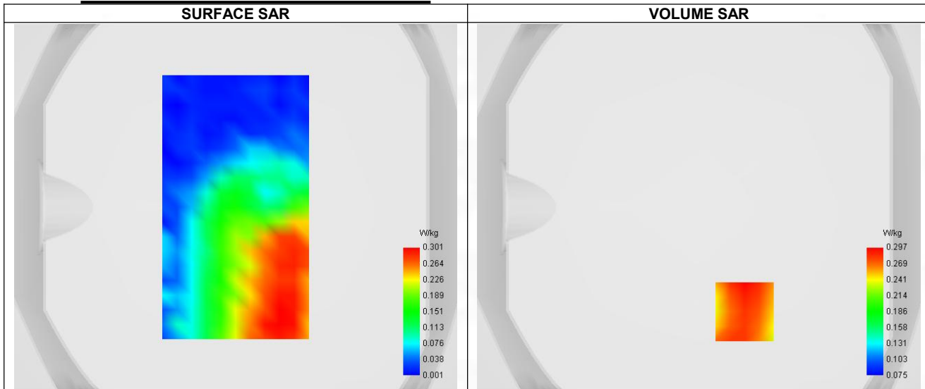
Maximum location: X=25.00, Y=-57.00 ; SAR Peak: 0.36 W/kg
