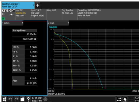
B2&B66_N5(20M)_DFT-s-OFDM_PI_2-BPSK_Outer_Full_Mid_CH
