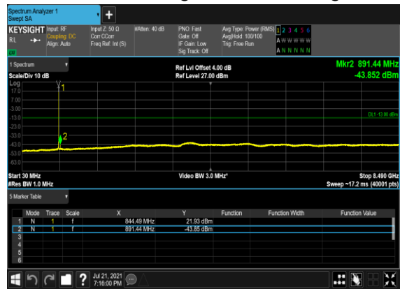
B2&B66_N5(5M)_DFT-s-OFDM_QPSK_Edge_1RB_Left_High_CH
