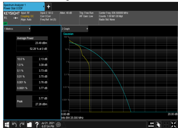
B2&B66_N5(20M)_DFT-s-OFDM_PI_2-BPSK_Edge_1RB_Left_Mid_CH
