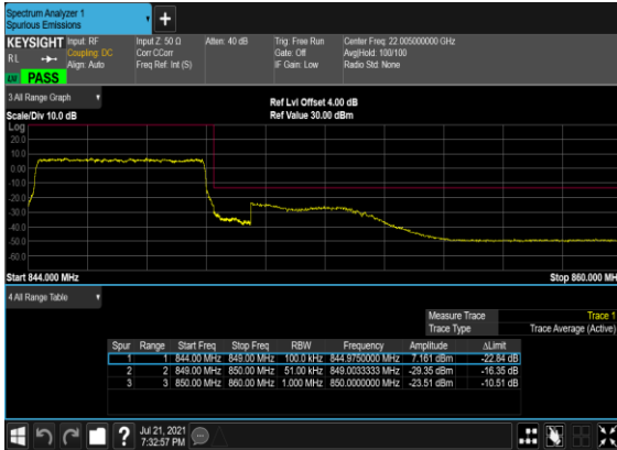
B2&B66_N5(5M)_DFT-s- OFDM_QPSK_Outer_Full_High_CH
