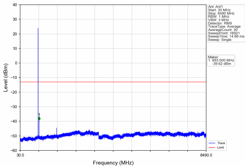
B26_5MHz_16QAM_HCH_846.5MHz_RB_1_0_NTNV
