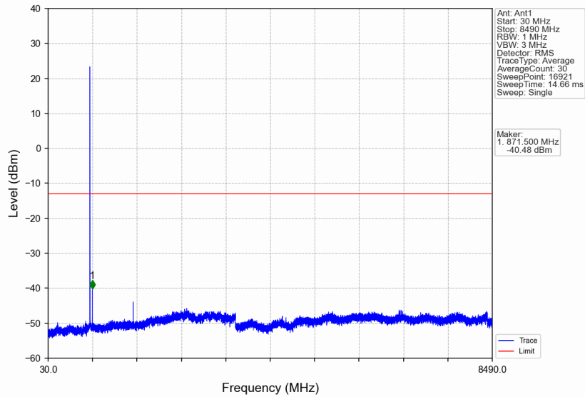
B26_3MHz_16QAM_LCH_825.5MHz_RB_15_0_NTNV
