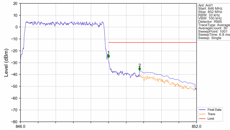
B26_3MHz_64QAM_HCH_847.5MHz_RB_15_0_NTNV
