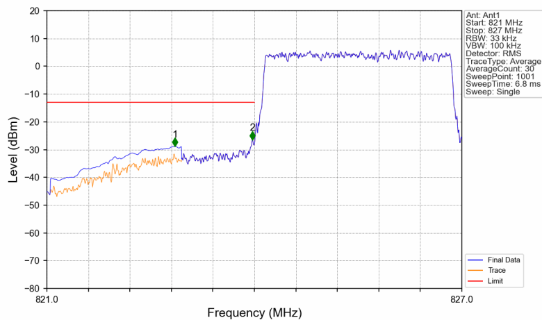
B26_3MHz_16QAM_LCH_825.5MHz_RB_15_0_NTNV
