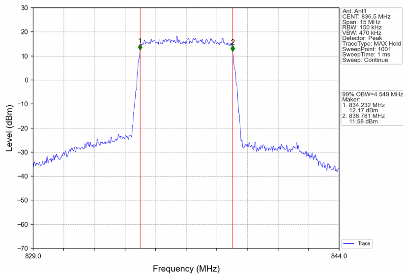
B26_5MHz_64QAM_MCH_836.5MHz_RB_25_0_NTNV
