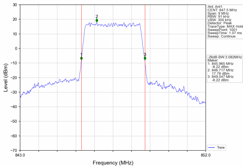
B26_3MHz_64QAM_HCH_847.5MHz_RB_15_0_NTNV
