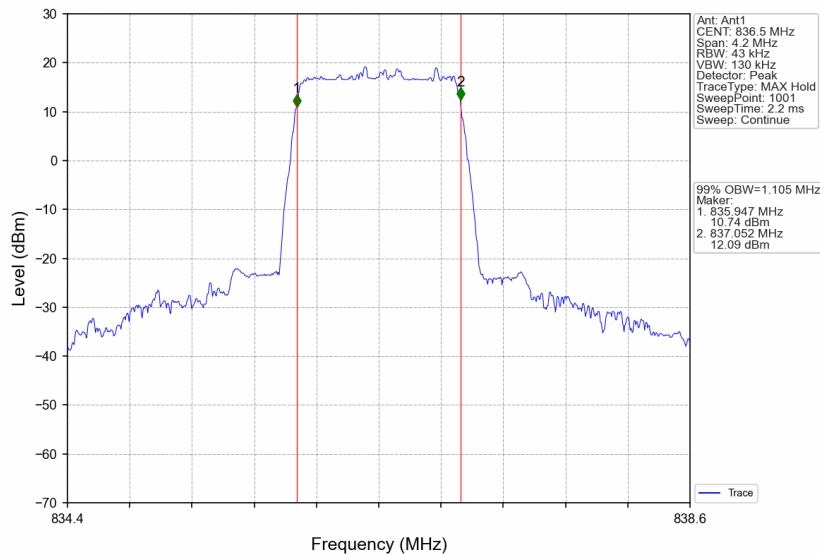
B26_1.4MHz_64QAM_MCH_836.5MHz_RB_6_0_NTNV
