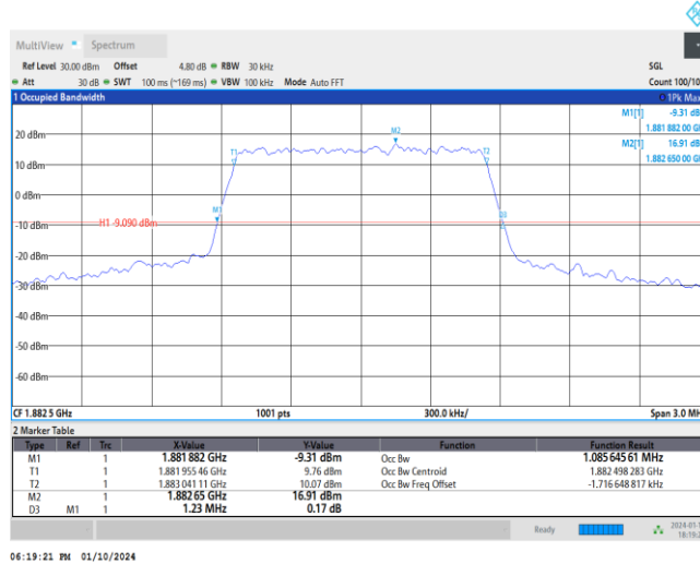
Band25-1.4MHz-16QAM-26365-6RB#0
