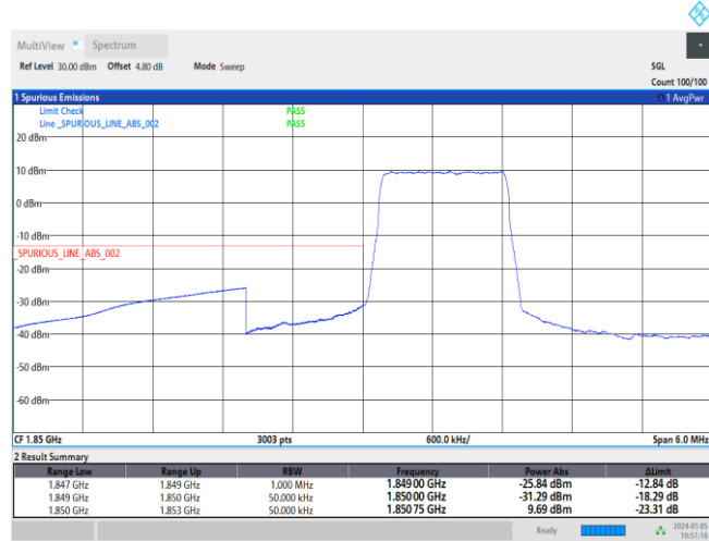
Band2-1.4MHz-QPSK-18607-6RB#0
