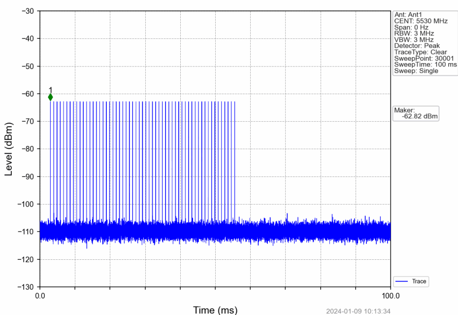
Signal Calibration_802.11ac(VHT80)_2C_5530MHz_RadarType1_Trial0
