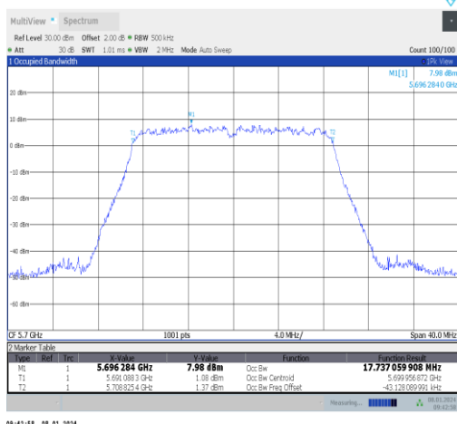
11ac20MIMO-Ant1-5700
