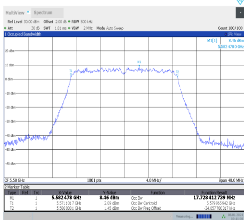
11ac20MIMO-Ant1-5580
