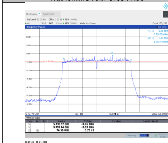
11ac80MIMO-Ant1-5775-PASS
