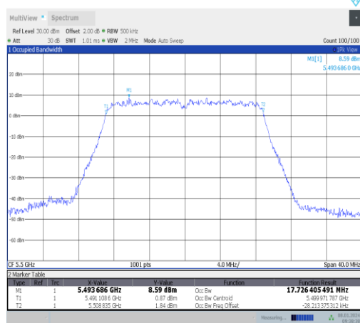
11ac20MIMO-Ant0-5500
