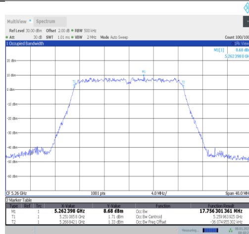
11ac20MIMO-Ant0-5260
