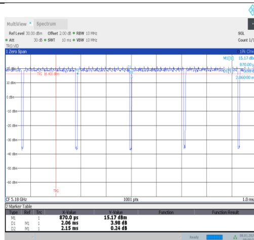
NTNV-11a-Ant1-5180
