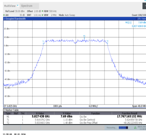
11ac20MIMO-Ant0-5825
