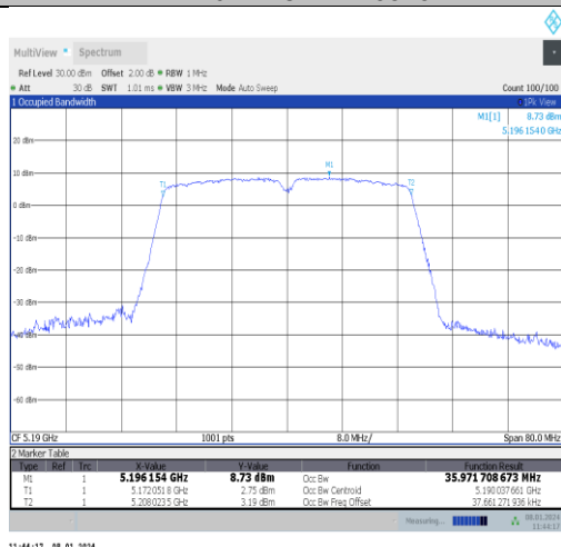
11ac40MIMO-Ant1-5190
