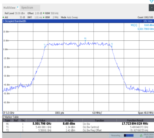
11ac20MIMO-Ant1-5500
