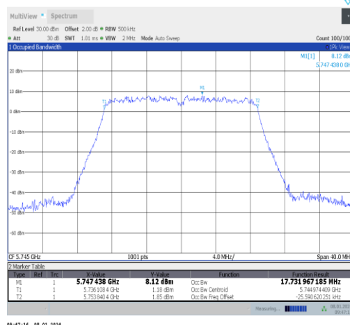
11ac20MIMO-Ant0-5745
