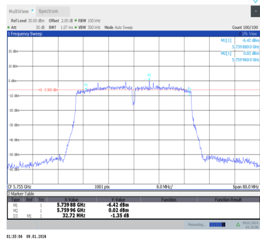
11ac40MIMO-Ant0-5755-PASS
