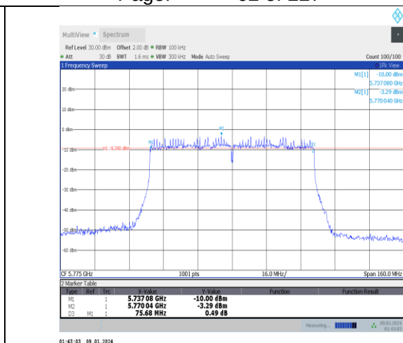
11ac80MIMO-Ant0-5775-PASS
