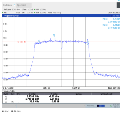
11ac40MIMO-Ant1-5755-PASS
