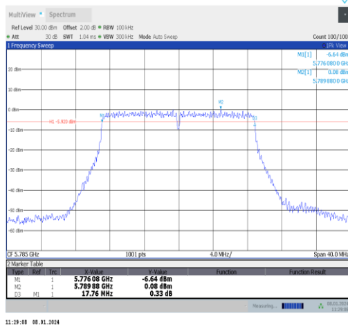
11ac20MIMO-Ant1-5785-PASS
