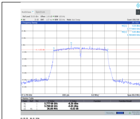
11ac40MIMO-Ant1-5795-PASS
