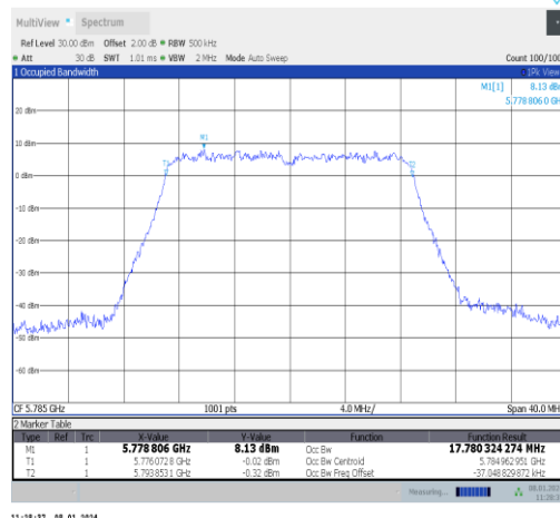
11ac20MIMO-Ant0-5785
