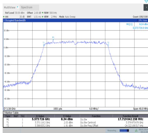
11ac20MIMO-Ant0-5580
