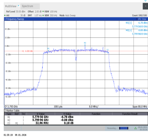
11ac40MIMO-Ant0-5795-PASS
