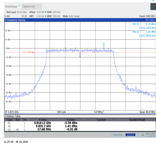
11ac20MIMO-Ant0-5825-PASS
