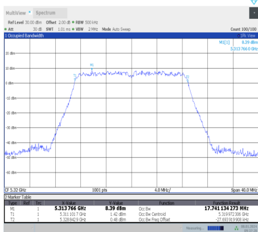
11ac20MIMO-Ant1-5320
