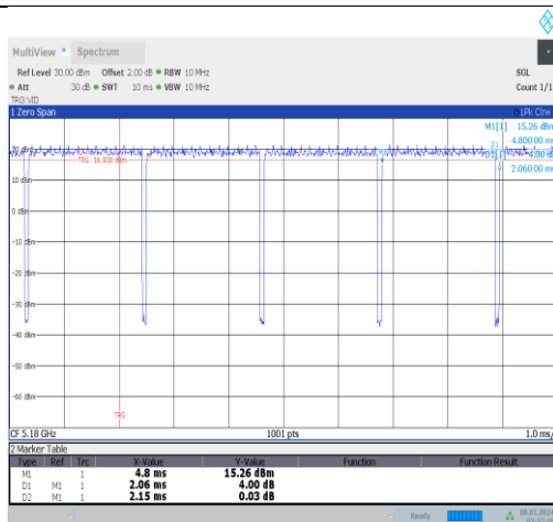
NTNV-11a-Ant0-5180
