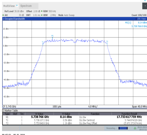
11ac20MIMO-Ant1-5745
