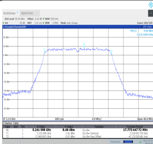
11ac20MIMO-Ant1-5240
