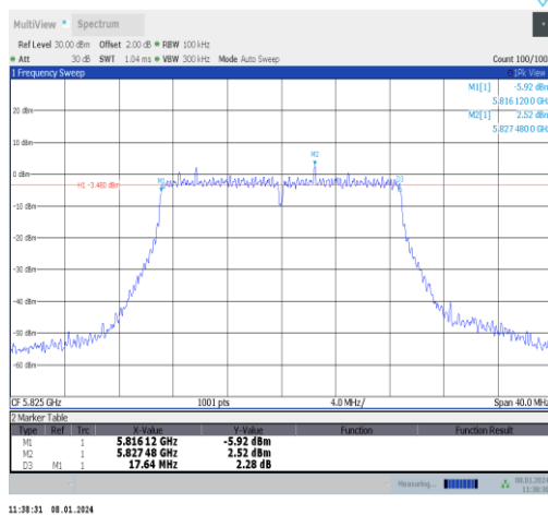
11ac20MIMO-Ant1-5825-PASS
