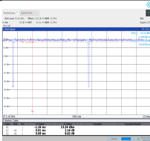
NTNV-11n20MIMO-Ant0-5180
