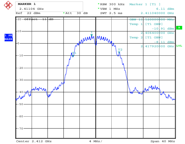
ANT 2(802.11b)
