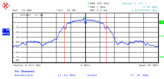
ANT 1(802.11b)
