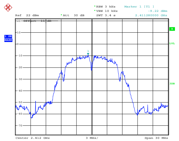
ANT 2(802.11b)
