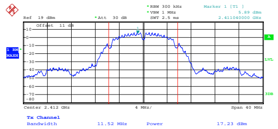
ANT 2(802.11b)
