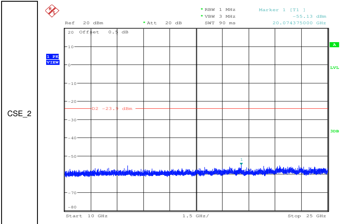
RF Conducted Spurious Emissions_11N40SISO_2452_Ant1
