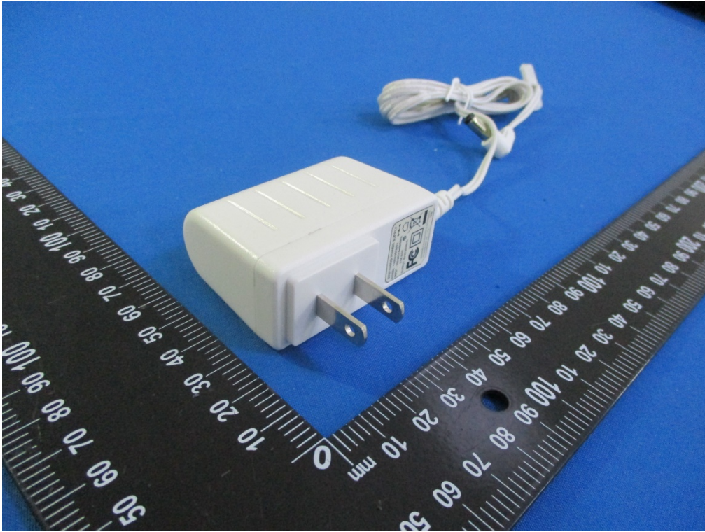
EUT – Adapter
