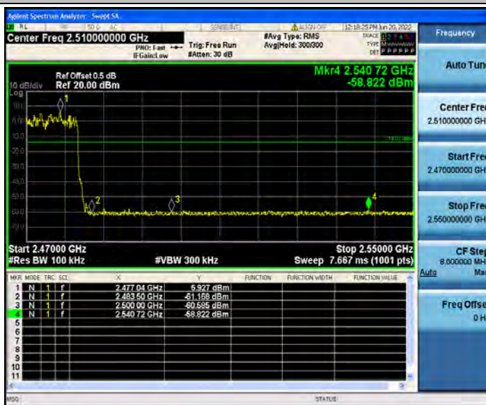
8-DPSK_Hop_2480
