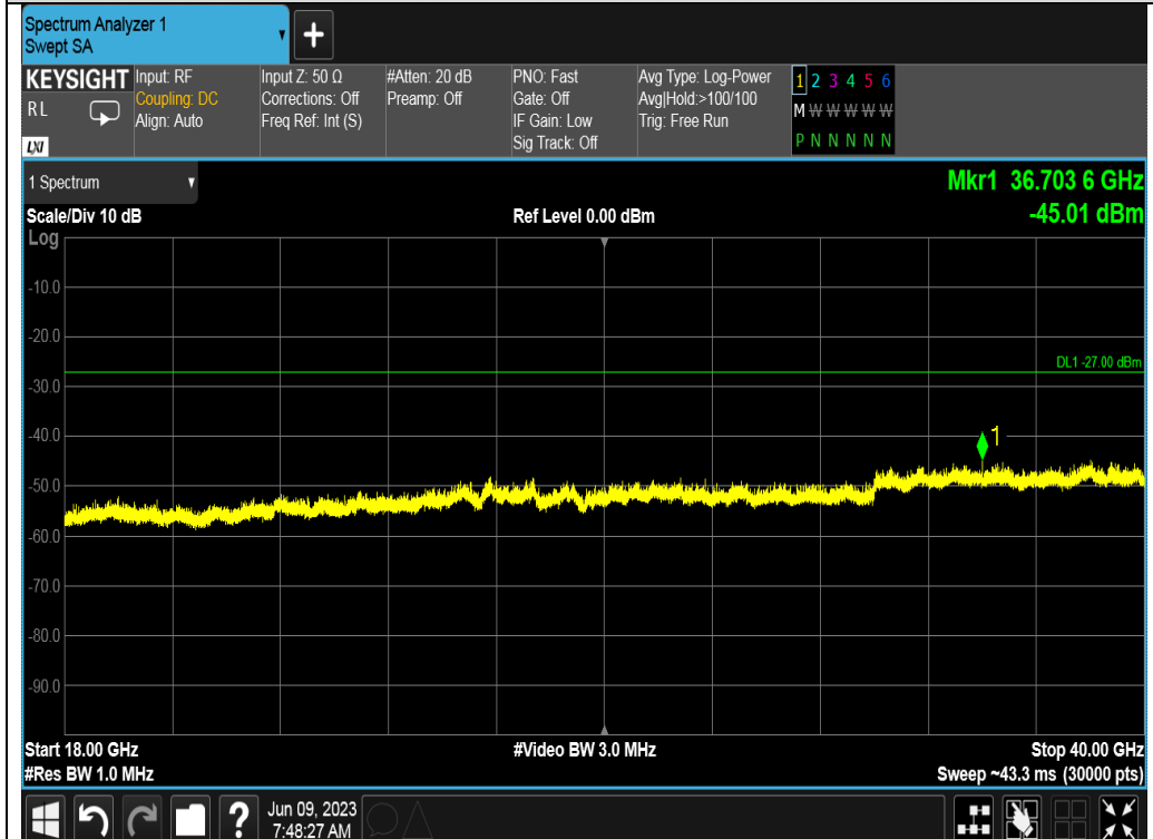
Test_Graph_802.11n40_ANT1_5795_MCS0_Frequency Band5
