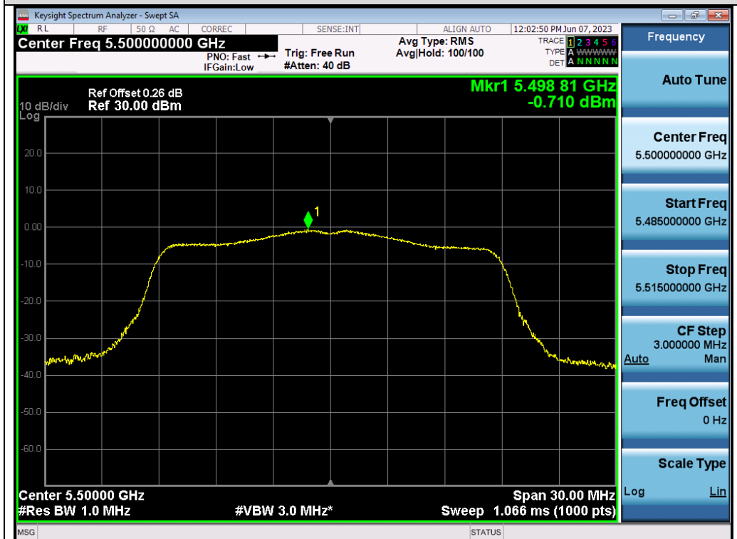
Test_Graph_802.11ac20_ANT1_5500_MCS0_PSD
