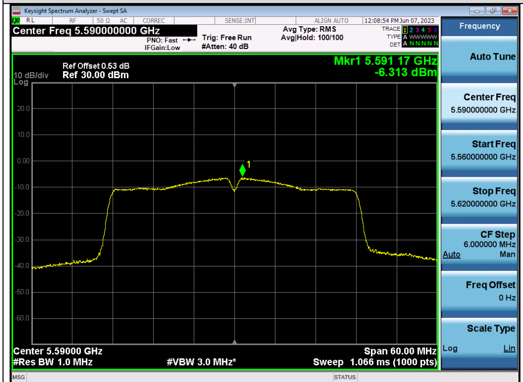
Test_Graph_802.11ac40_ANT1_5590_MCS9_PSD
