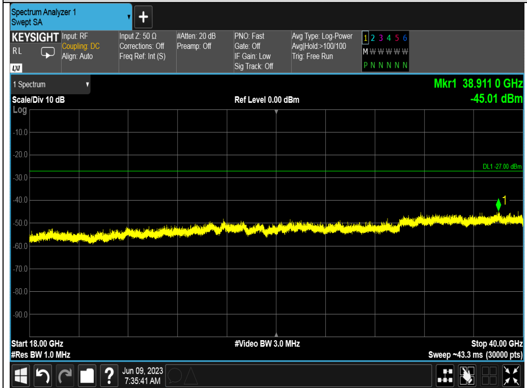
Test_Graph_802.11a_ANT1_5320_6Mbps_Frequency Band 5
