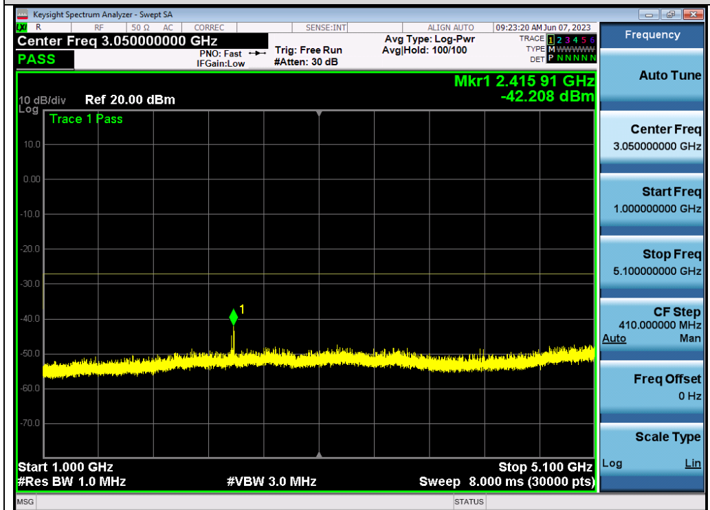
Test_Graph_802.11a_ANT1_5180_6Mbps_Frequency Band 2
