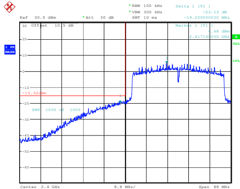
802.11ax40_2422MHz_RU_Full 23.13dB
