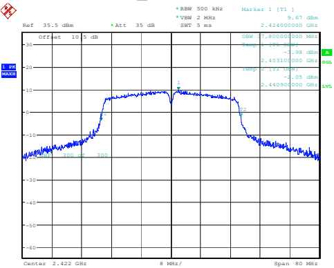
802.11n40_2422MHz 37.800MHz
