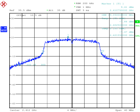
802.11n20_2412MHz 19.050MHz
