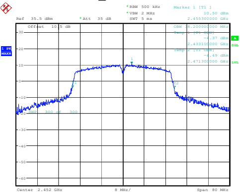
802.11n40_2452MHz 38.200MHz
