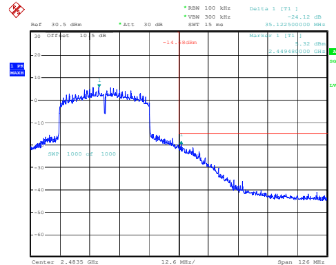
802.11ax40_2452MHz_RU_Full 24.12dB
