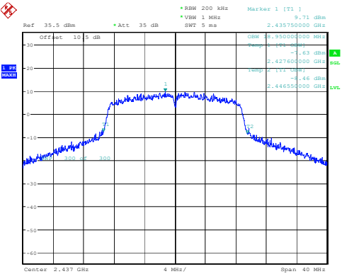
802.11n20_2437MHz 18.950MHz
