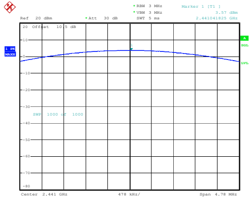
DH1_Middle 3.57dBm
