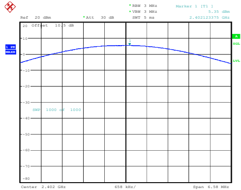
2DH1_Low 5.35dBm
