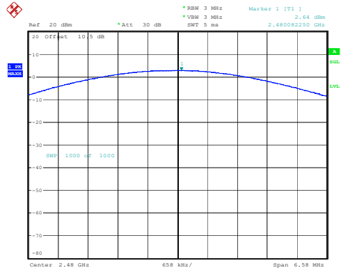
2DH1_High 2.64dBm
