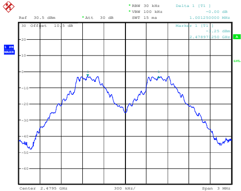
DH1_High 1.001MHz
