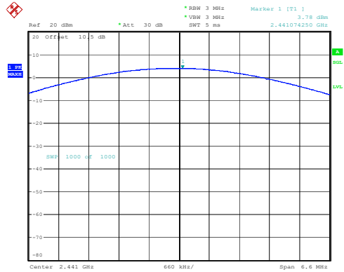
2DH1_Middle 3.78dBm
