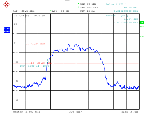
2DH1_Low 1.316MHz
