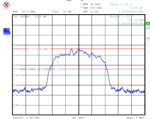
3DH1_High 1.290MHz
