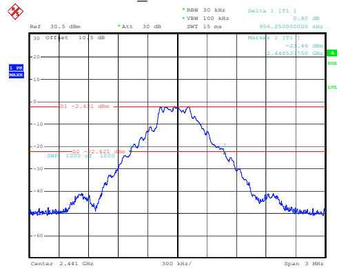
DH1_Middle 0.956MHz
