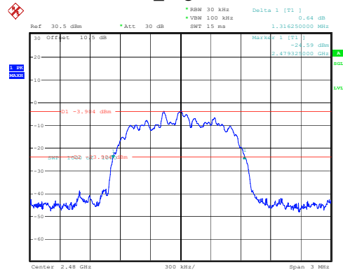
2DH1_High 1.316MHz
