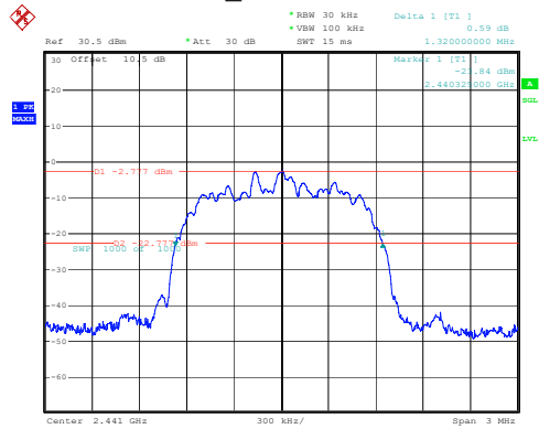
2DH1_Middle 1.320MHz
