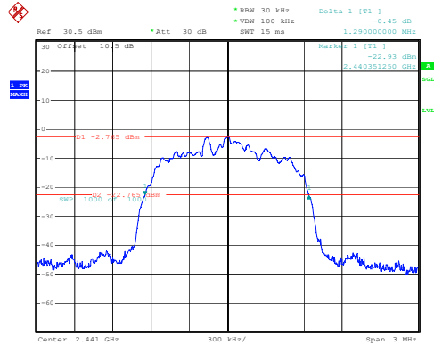
3DH1_Middle 1.290MHz
