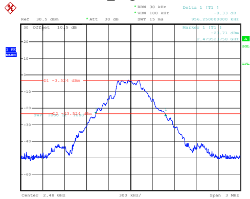
DH1_High 0.956MHz
