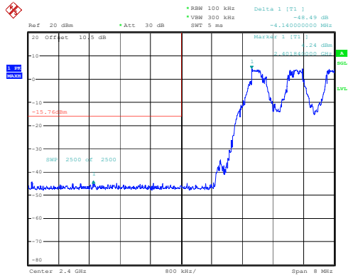
DH1_Hopping_Lower
