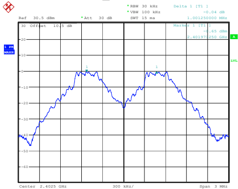
DH1_Low 1.001MHz
