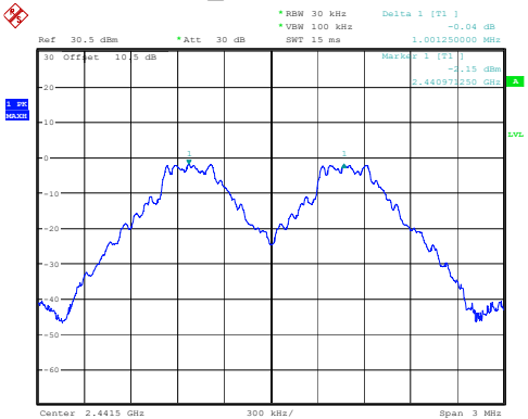
DH1_Middle 1.001MHz
