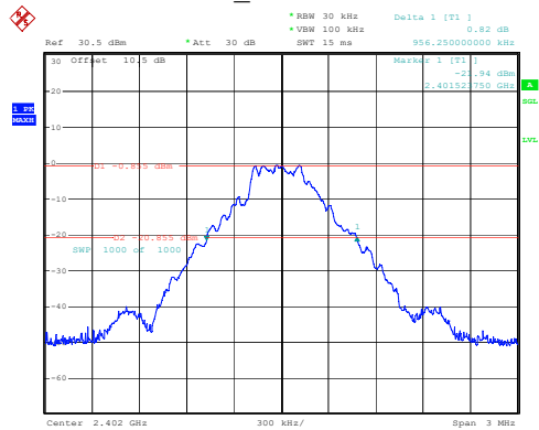
DH1_Low 0.956MHz
