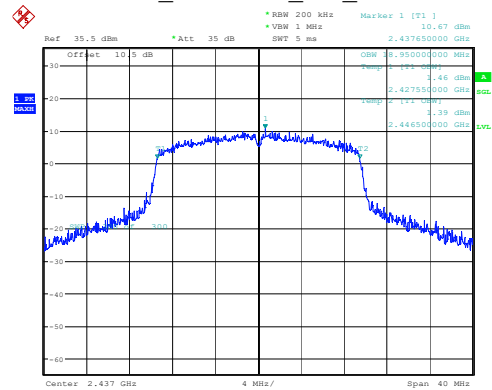
802.11ax20_2437MHz_RU_Full 18.950MHz
