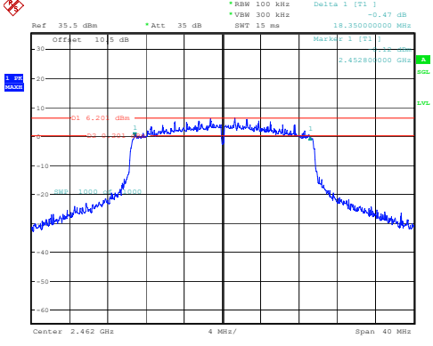
802.11ax20_2462MHz_RU_Full 18.350MHz
