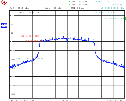
802.11ax20_2437MHz_RU_Full 18.100MHz
