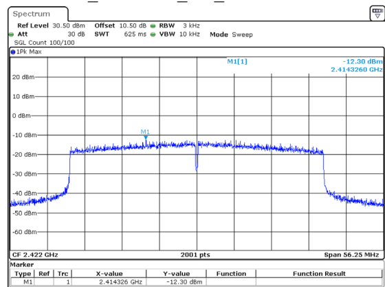
802.11ax40_2422MHz_RU_Full -12.30dBm/3kHz
