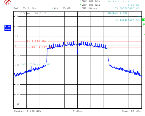
802.11ax40_2452MHz_RU_Full 35.300MHz
