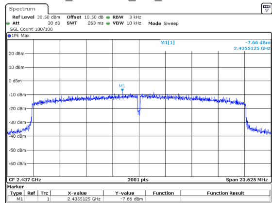
802.11ax20_2437MHz_RU_Full -7.66dBm/3kHz
