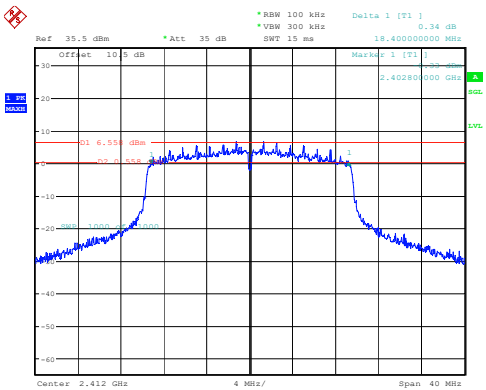
802.11ax20_2412MHz_RU_Full 18.400MHz
