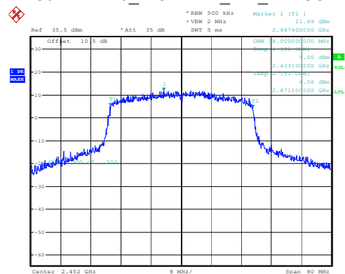
802.11ax40_2452MHz_RU_Full 38MHz
