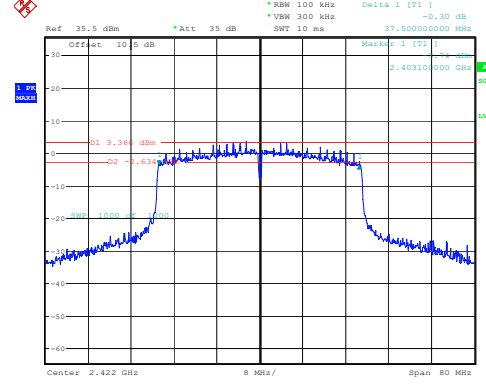
802.11ax40_2422MHz_RU_Full 37.500MHz
