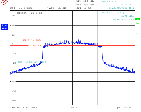
802.11ax40_2437MHz_RU_Full 35.300MHz
