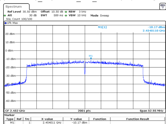
802.11ax40_2452MHz_RU_Full -10.17dBm/3kHz
