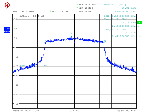
802.11ax40_2422MHz_RU_Full 38.100MHz
