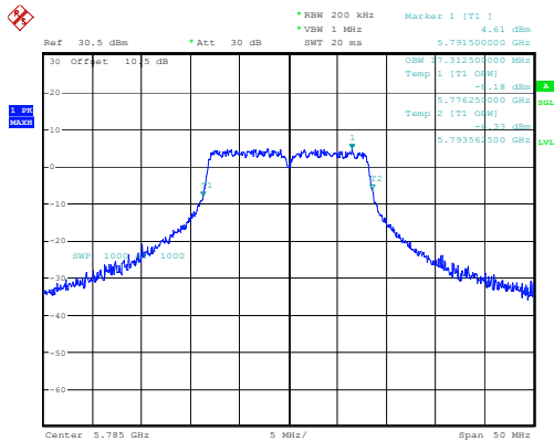
802.11a_5785MHz 17.313MHz
