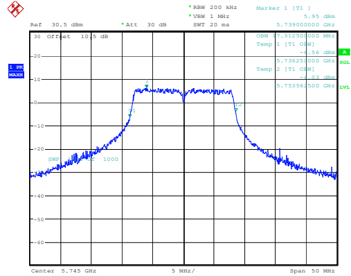
802.11a_5745MHz 17.313MHz
