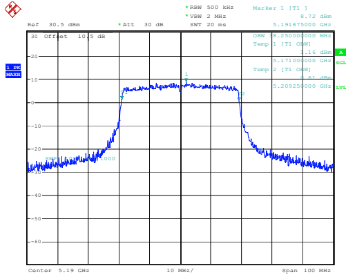
802.11ax40_5190MHz_RU_Full 38.250MHz
