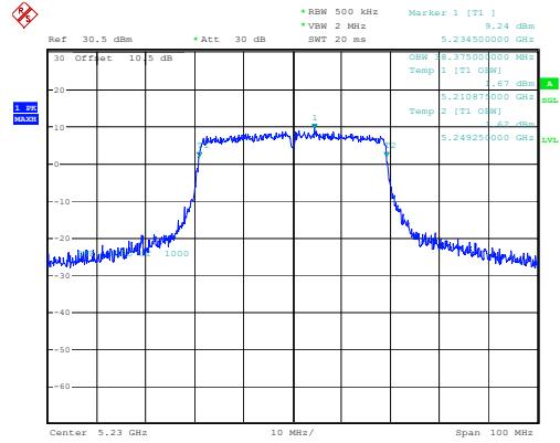
802.11ax40_5230MHz_RU_Full 38.375MHz
