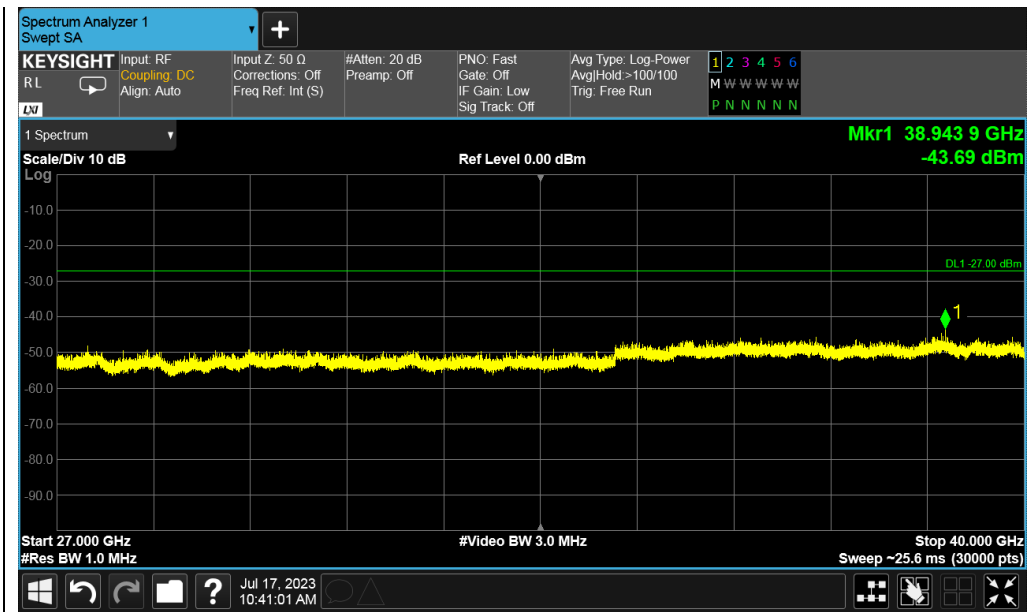
Test_Graph_802.11n40_ANT1_5310_MCS0_Frequency Band 5
