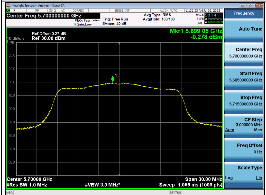
Test_Graph_802.11ac20_ANT1_5700_MCS9_PSD
