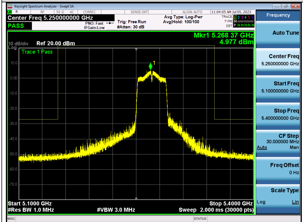
Test_Graph_802.11n40_ANT1_5270_MCS0_Frequency Band 3
