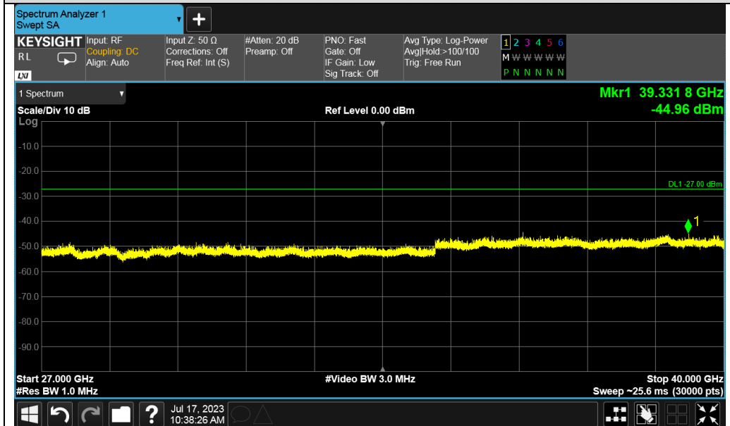
Test_Graph_802.11a_ANT1_5260_6Mbps_Frequency Band 5
