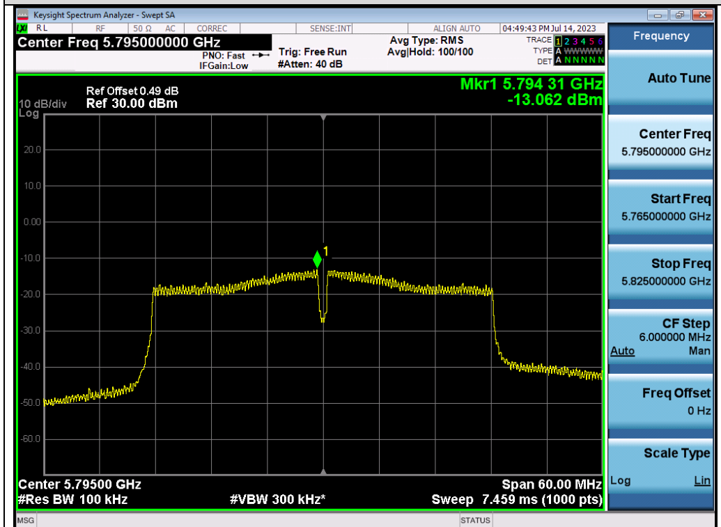
Test_Graph_802.11ac40_ANT1_5795_MCS9_PSD
