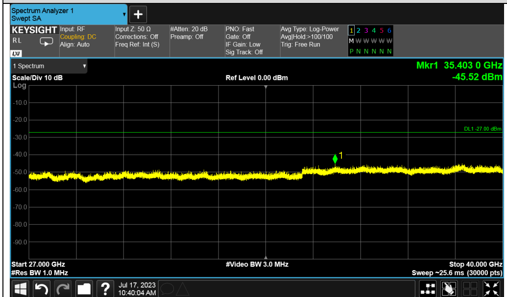
Test_Graph_802.11n40_ANT1_5270_MCS0_Frequency Band 5
