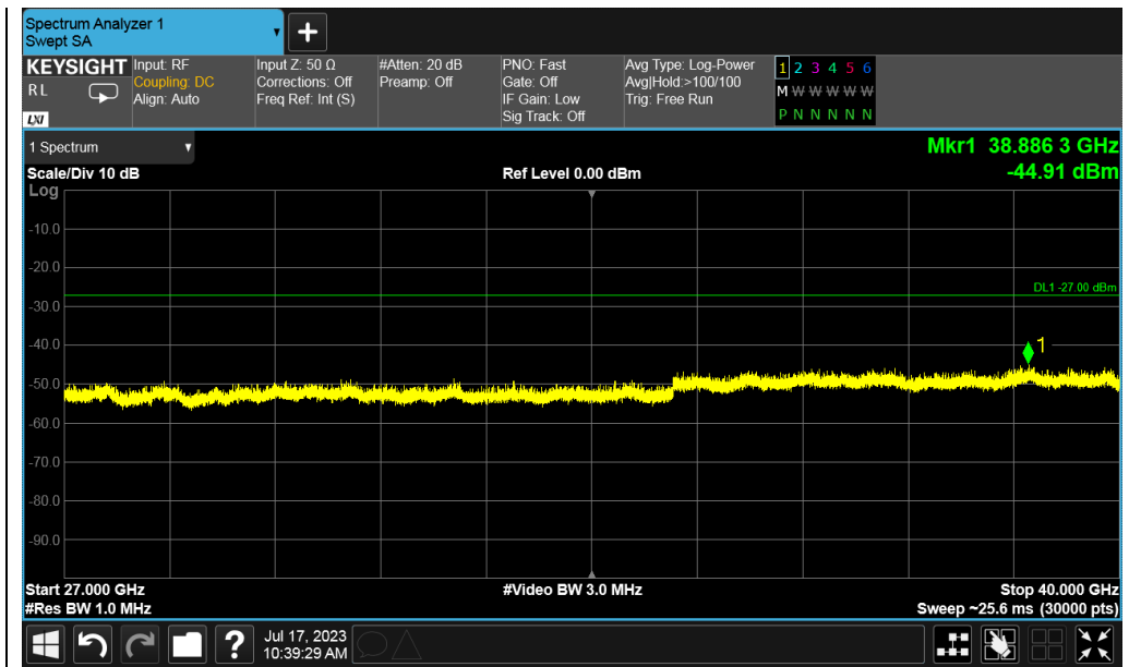
Test_Graph_802.11a_ANT1_5320_6Mbps_Frequency Band 5
