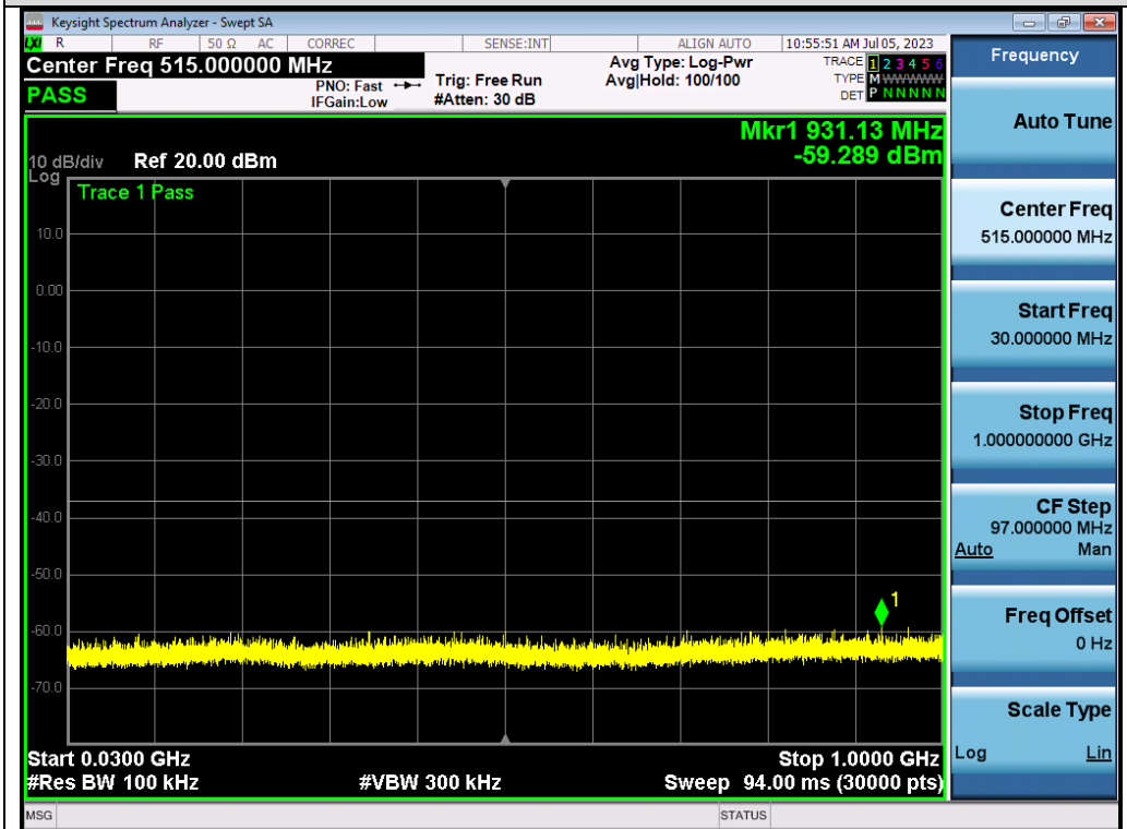
Test_Graph_802.11ac80_ANT1_5290_MCS9_Frequency Band 1
