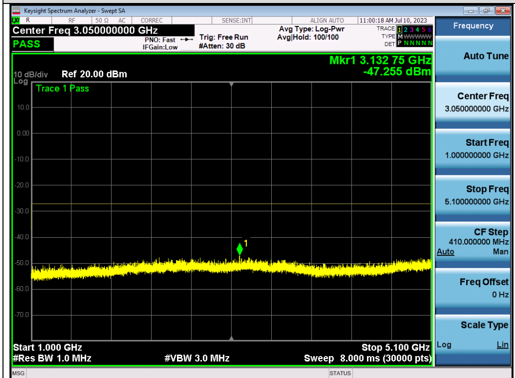
Test_Graph_802.11a_ANT1_5180_6Mbps_Frequency Band 2
