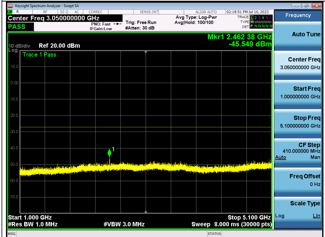
Test_Graph_802.11a_ANT1_5260_6Mbps_Frequency Band 2
