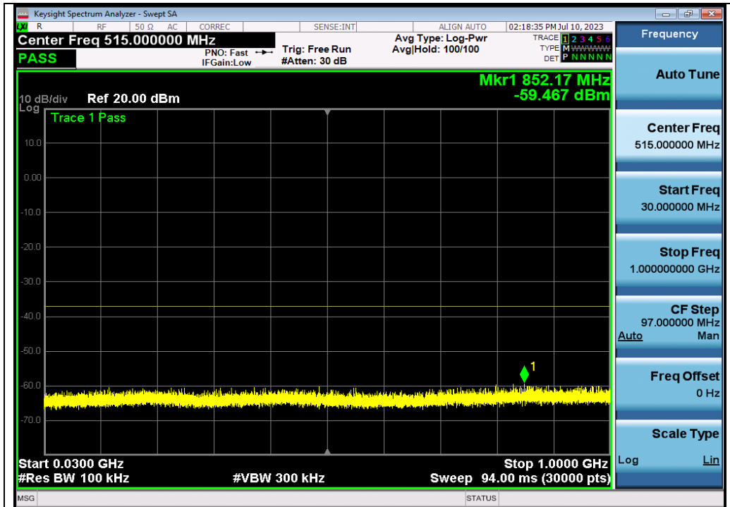
Test_Graph_802.11a_ANT1_5260_6Mbps_Frequency Band 1
