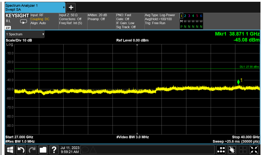
Test_Graph_802.11n40_ANT1_5270_MCS0_Frequency Band 5
