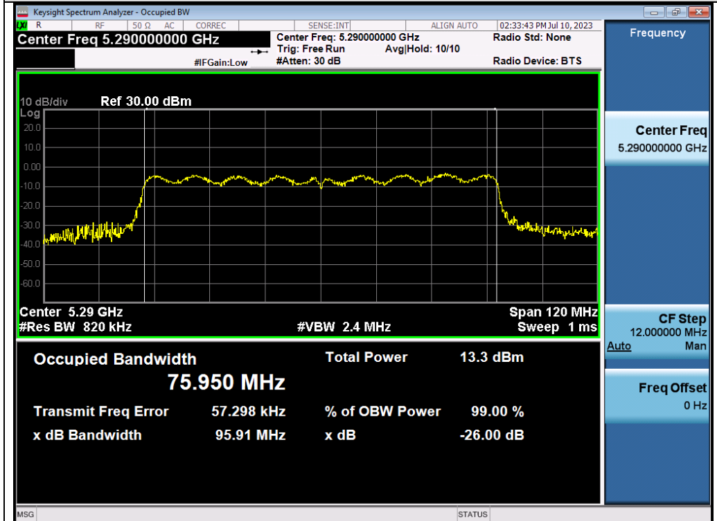
Test_Graph_802.11ac80_ANT1_5290_MCS9_OBW
