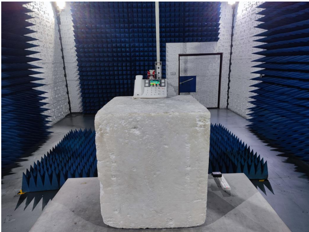
RADIATED EMISSION TEST SETUP ABOVE 1GHz (by Adapter)
