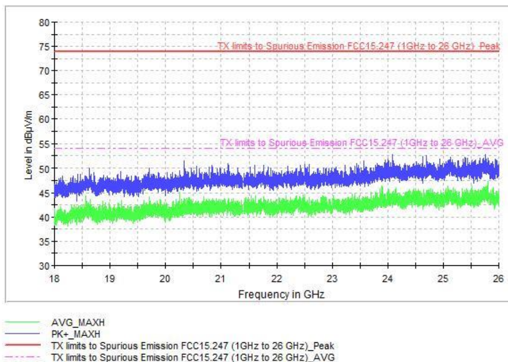
18GHz_26GHz_HP_CH High
