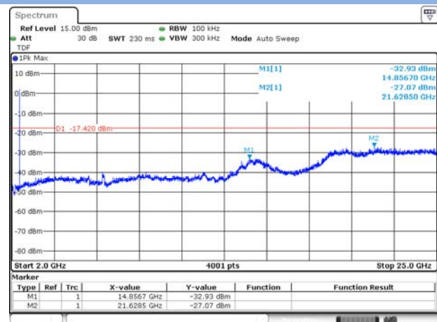
GFSK (BLE) LOW CHANNEL, SPURIOUS 2 GHz ~ 25 GHz
