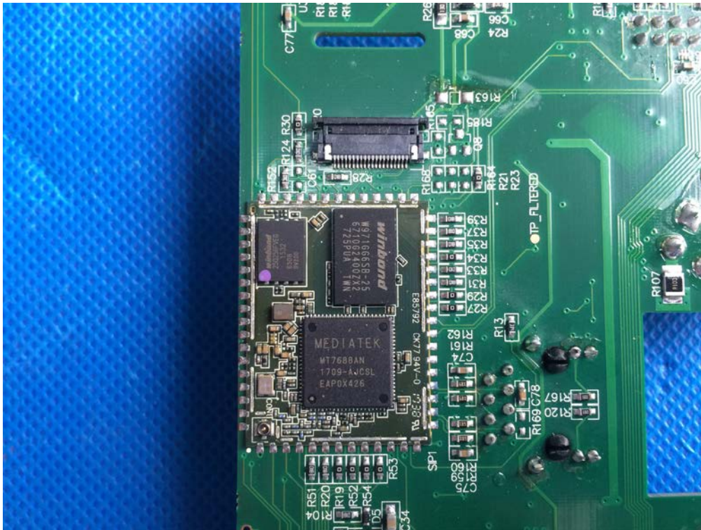
EUT – WIFI module View 4
