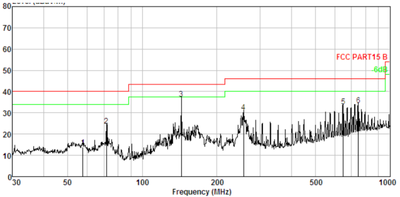
Test plot for Horizontal: GFSK(2402MHz)
