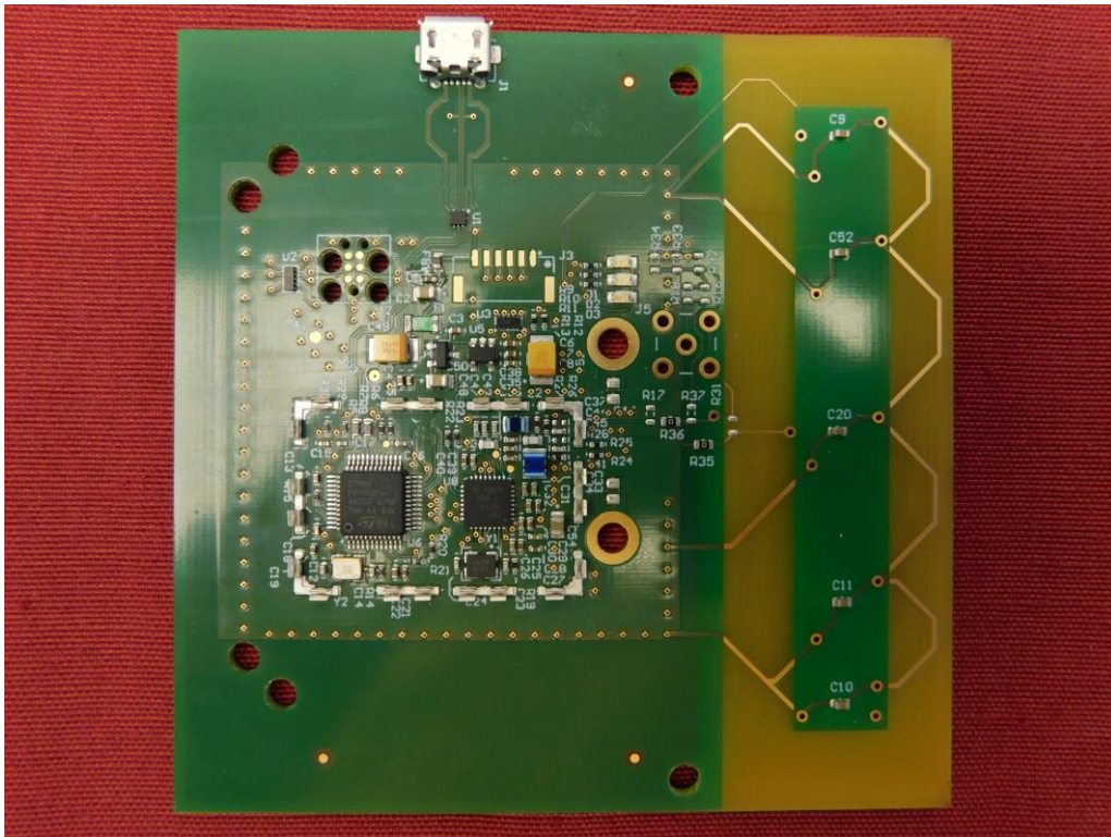
Picture 1: EUT - bottom side, without shielding
